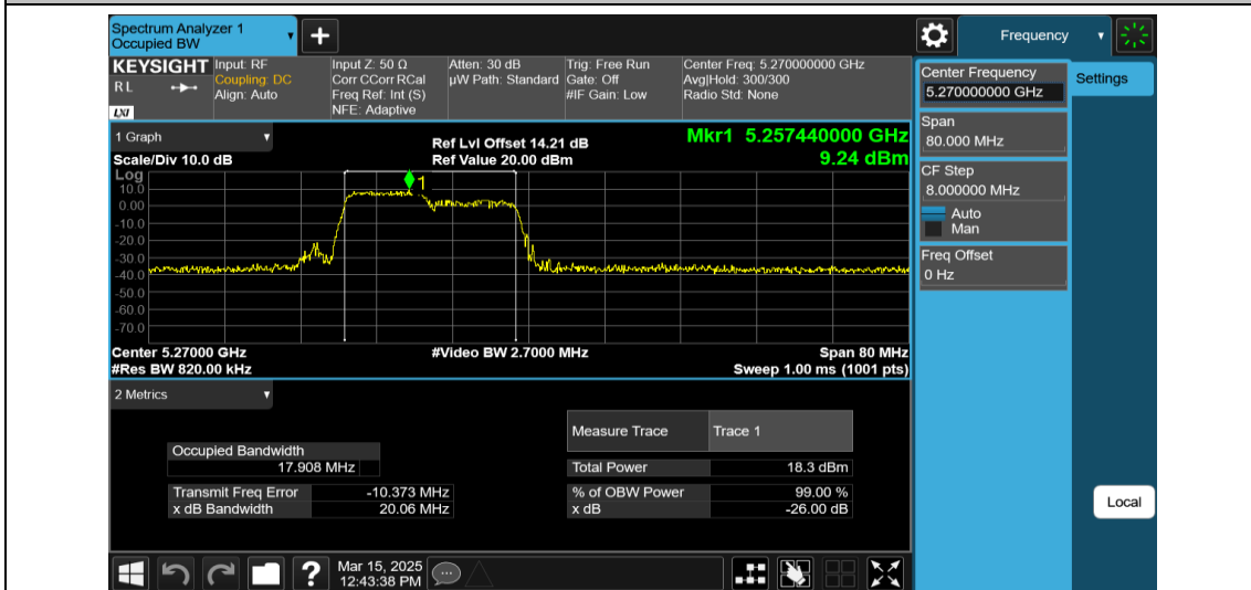
11AX40MIMO-Ant2-5270-106Tone-RU53
