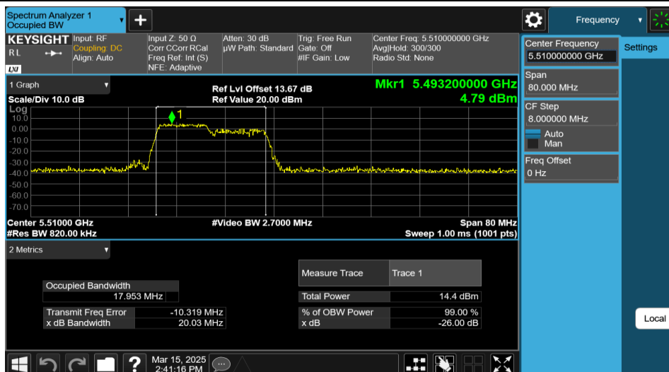
11AX40MIMO-Ant2-5510-106Tone-RU53
