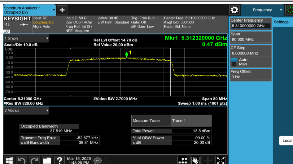
11AX40MIMO-Ant1-5310-484Tone-RU65
