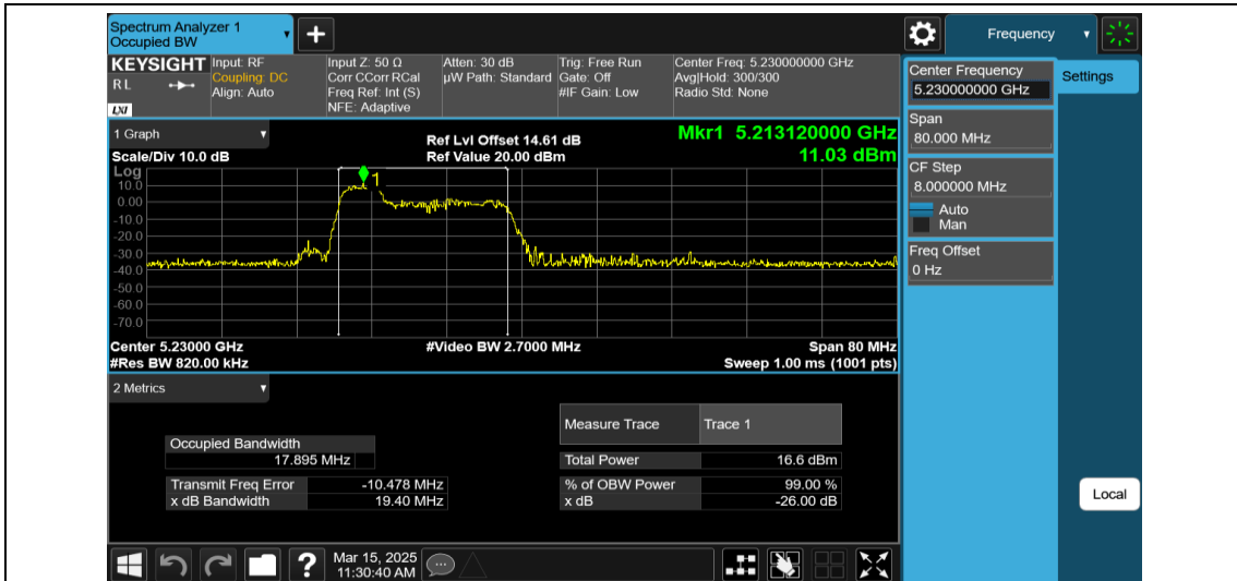
11AX40MIMO-Ant1-5230-52Tone-RU37
