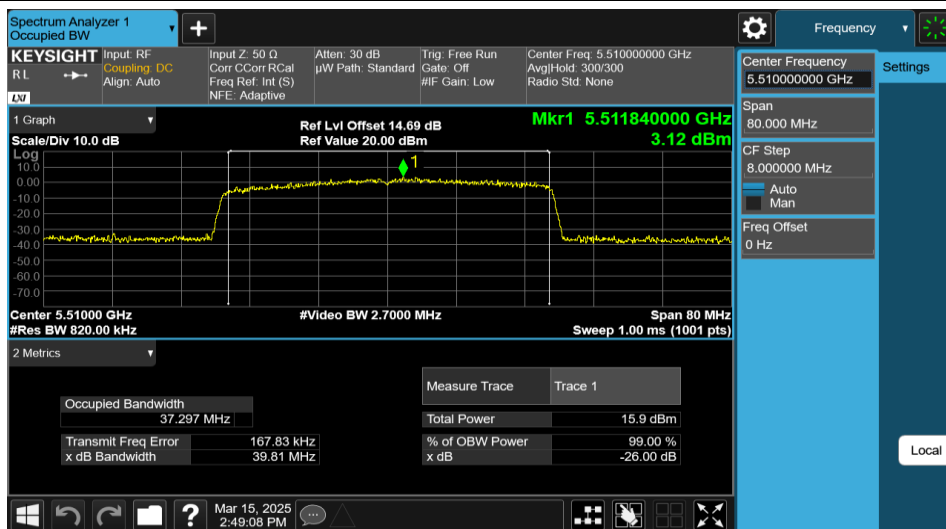
11AX40MIMO-Ant1-5510-484Tone-RU65
