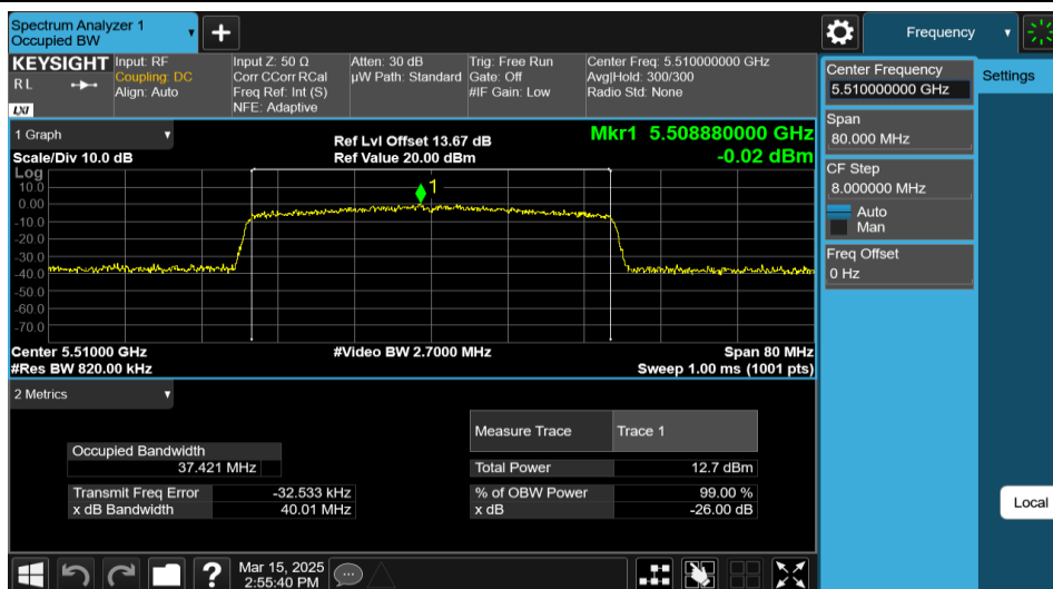
11AX40MIMO-Ant2-5510-484Tone-RU65
