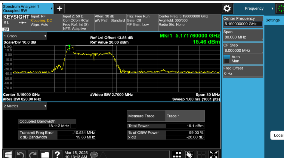
11AX40MIMO-Ant2-5190-26Tone-RU0
