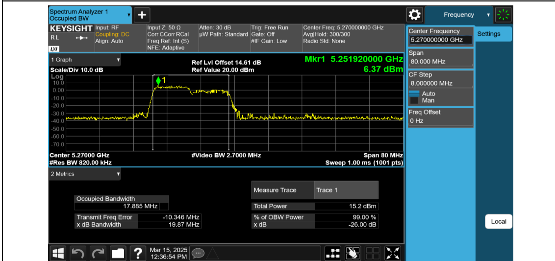
11AX40MIMO-Ant1-5270-106Tone-RU53
