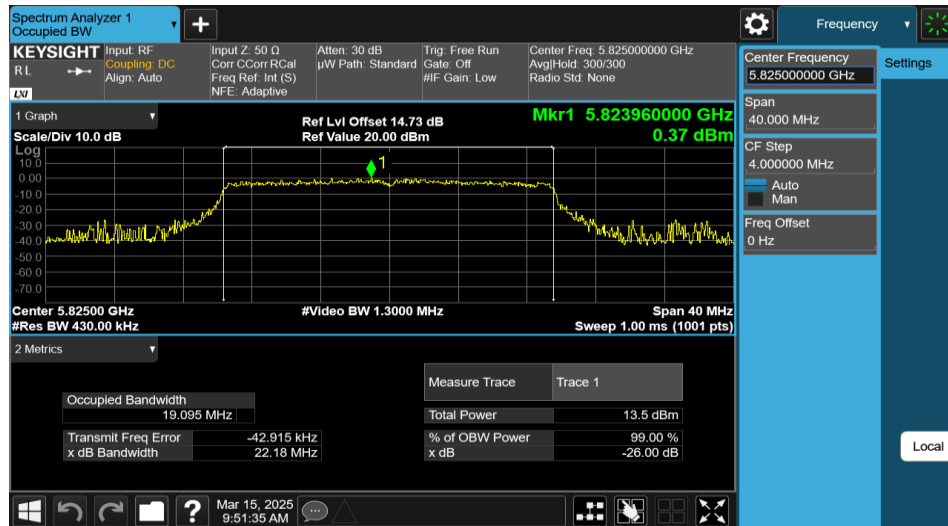
11AX20MIMO-Ant1-5825-242Tone-RU61
