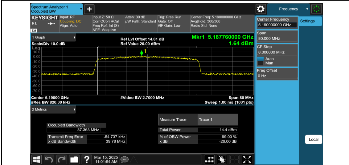
11AX40MIMO-Ant1-5190-484Tone-RU65
