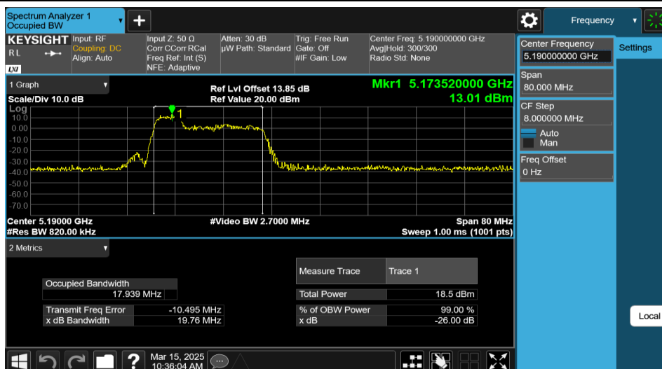
11AX40MIMO-Ant2-5190-52Tone-RU37
