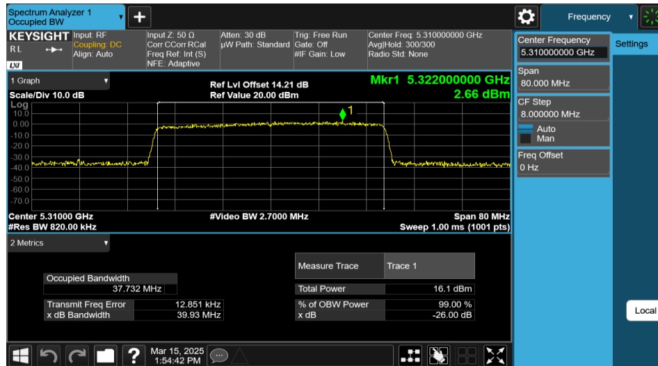
11AX40MIMO-Ant2-5310-484Tone-RU65
