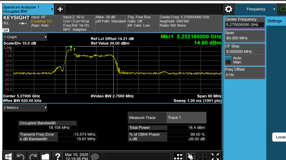
11AX40MIMO-Ant2-5270-26Tone-RU0
