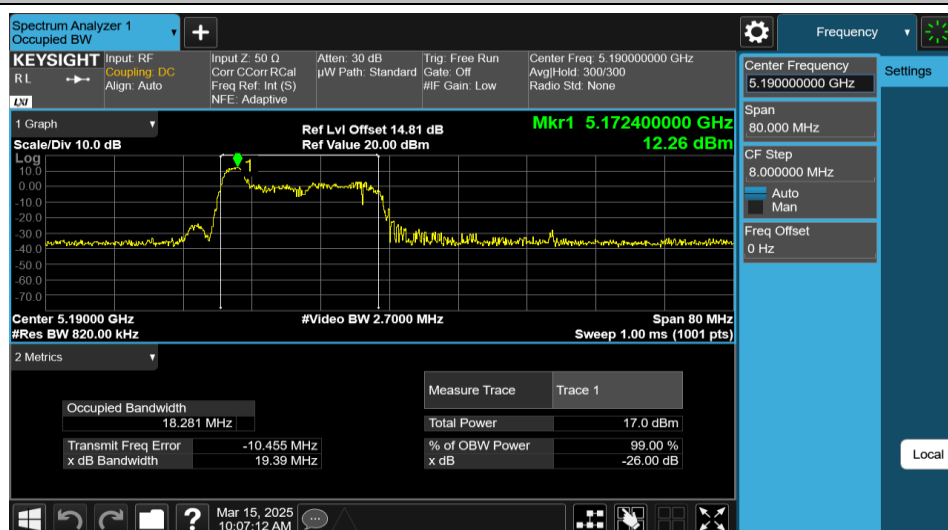
11AX40MIMO-Ant1-5190-26Tone-RU0
