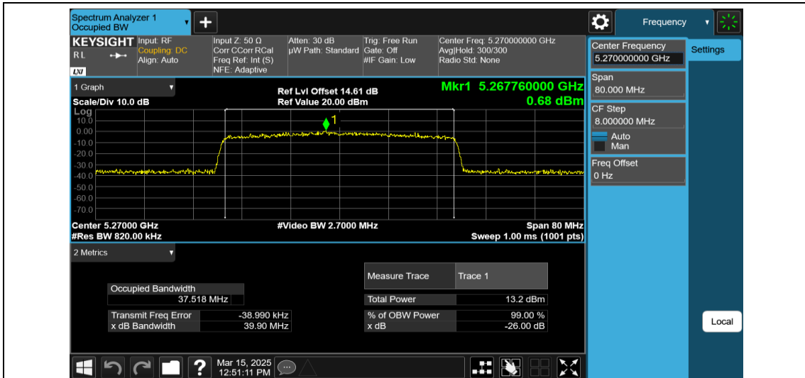
11AX40MIMO-Ant1-5270-484Tone-RU65
