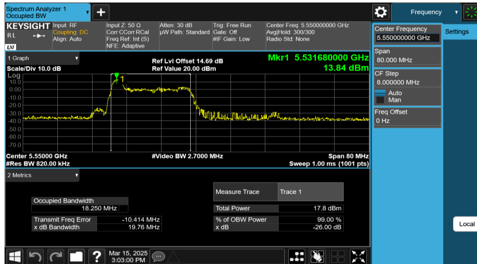
11AX40MIMO-Ant1-5550-26Tone-RU0
