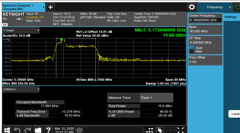
11AX40MIMO-Ant1-5190-52Tone-RU37
