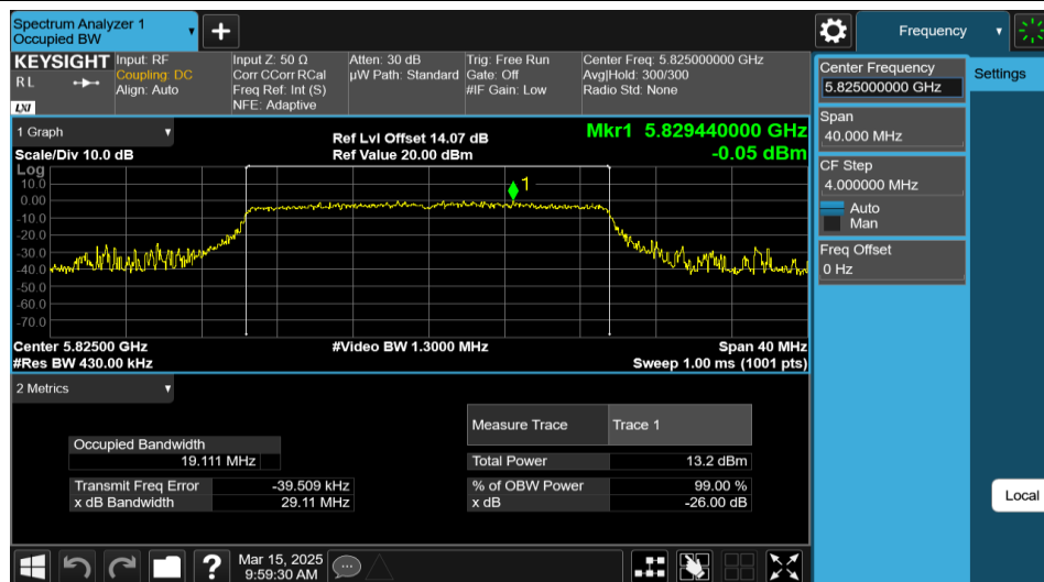
11AX20MIMO-Ant2-5825-242Tone-RU61
