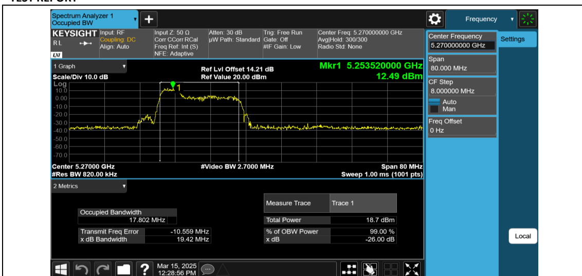
11AX40MIMO-Ant2-5270-52Tone-RU37
