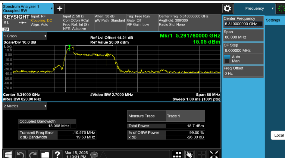
11AX40MIMO-Ant2-5310-26Tone-RU0
