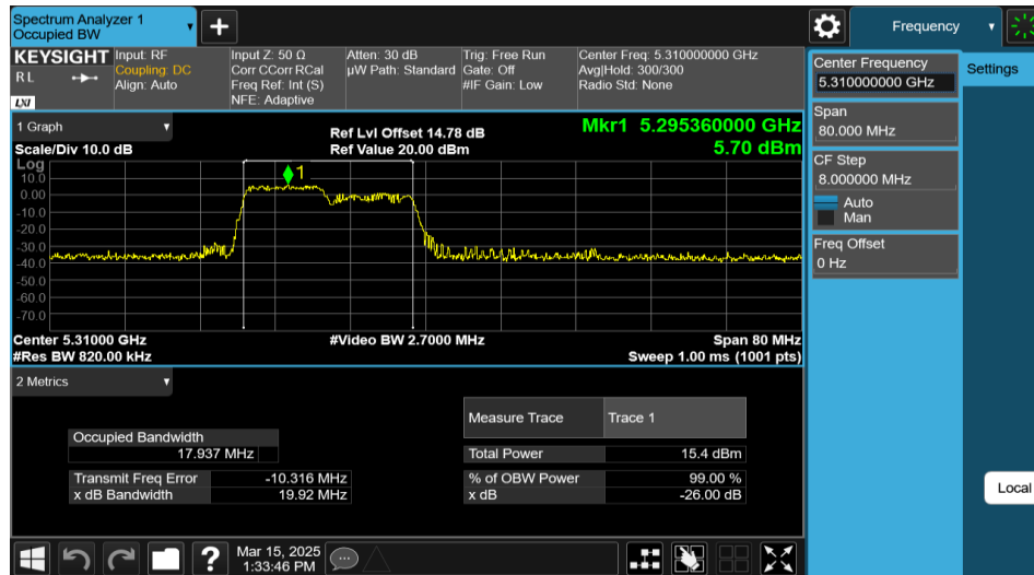
11AX40MIMO-Ant1-5310-106Tone-RU53
