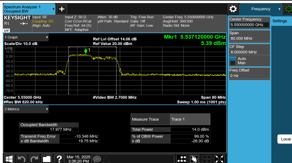
11AX40MIMO-Ant2-5550-106Tone-RU53
