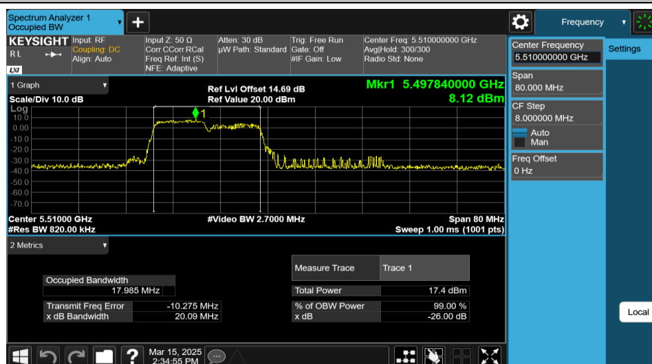
11AX40MIMO-Ant1-5510-106Tone-RU53
