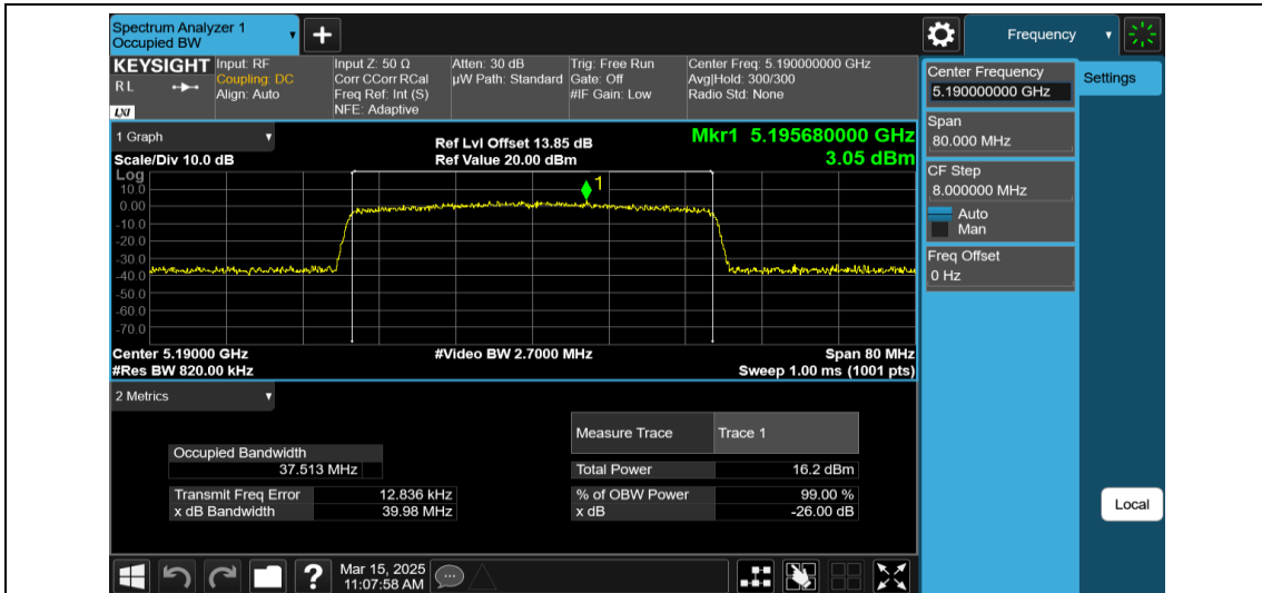
11AX40MIMO-Ant2-5190-484Tone-RU65
