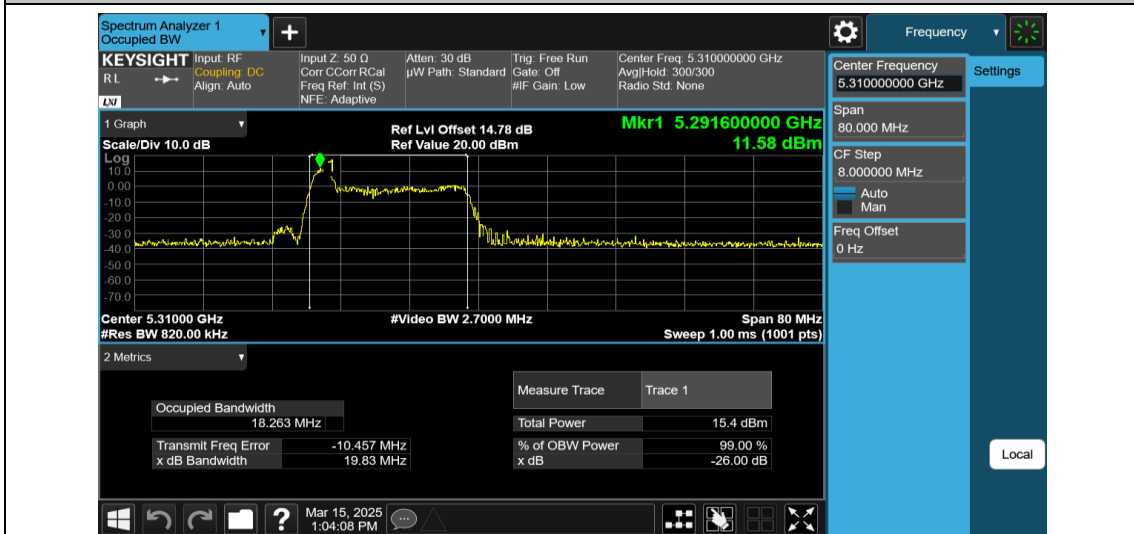
11AX40MIMO-Ant1-5310-26Tone-RU0
