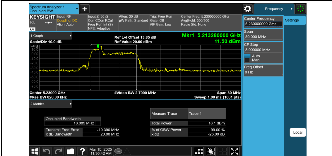
11AX40MIMO-Ant2-5230-52Tone-RU37
