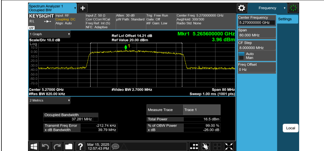
11AX40MIMO-Ant2-5270-484Tone-RU65
