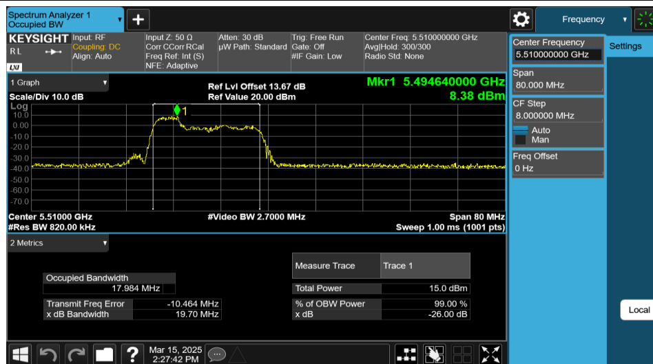
11AX40MIMO-Ant2-5510-52Tone-RU37
