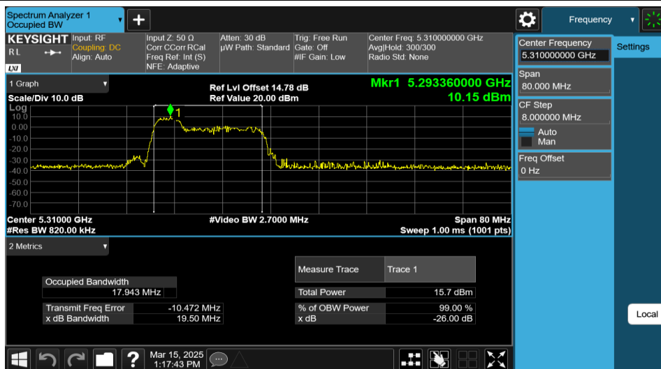
11AX40MIMO-Ant1-5310-52Tone-RU37
