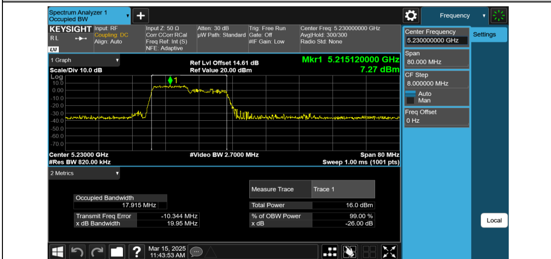
11AX40MIMO-Ant1-5230-106Tone-RU53
