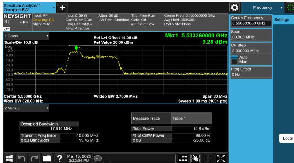
11AX40MIMO-Ant2-5550-52Tone-RU37
