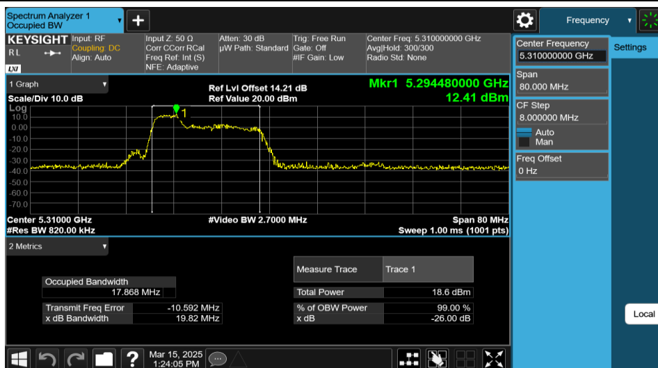
11AX40MIMO-Ant2-5310-52Tone-RU37
