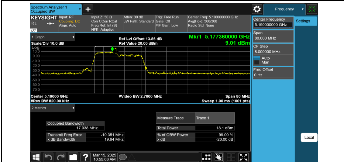
11AX40MIMO-Ant2-5190-106Tone-RU53
