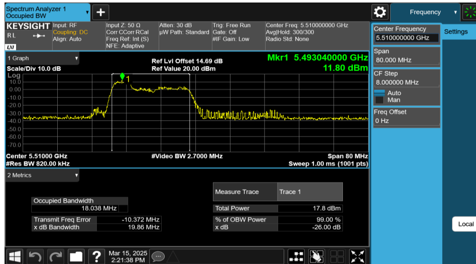
11AX40MIMO-Ant1-5510-52Tone-RU37
