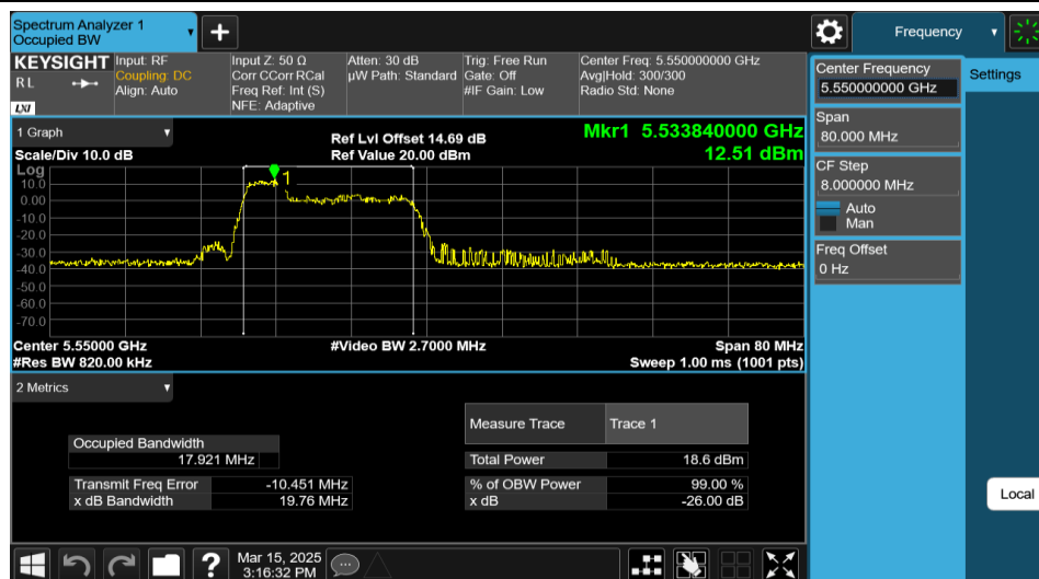
11AX40MIMO-Ant1-5550-52Tone-RU37
