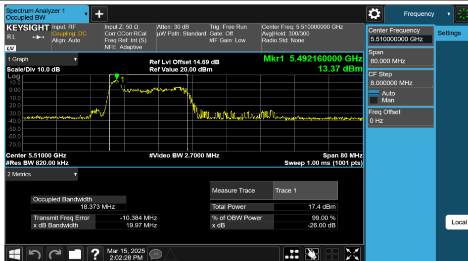
11AX40MIMO-Ant1-5510-26Tone-RU0
