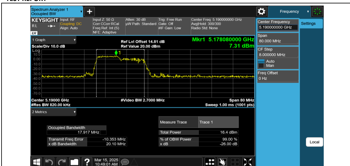
11AX40MIMO-Ant1-5190-106Tone-RU53
