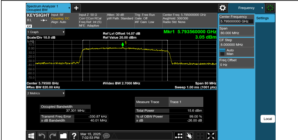
11AX40MIMO-Ant2-5795-484Tone-RU65
