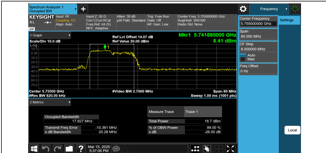
11AX40MIMO-Ant2-5755-106Tone-RU53
