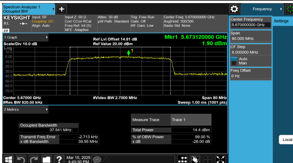
11AX40MIMO-Ant1-5670-484Tone-RU65
