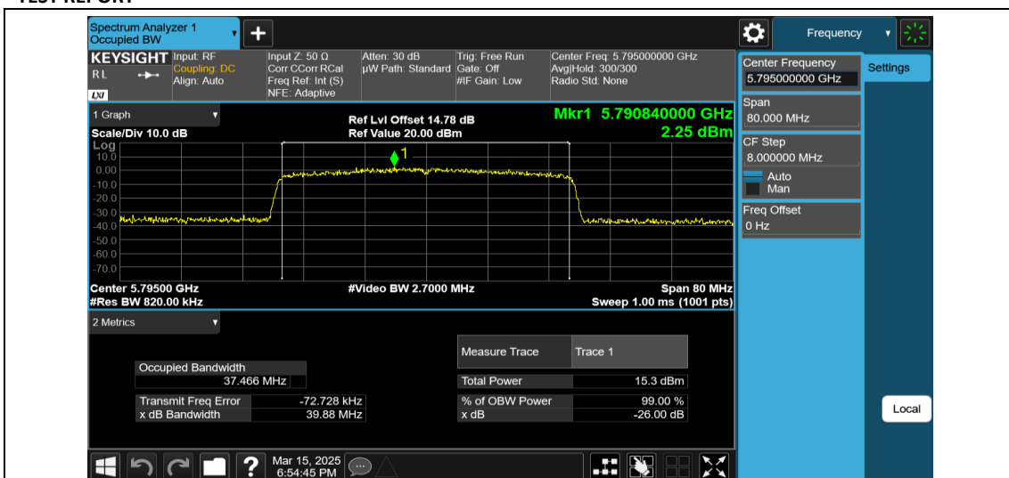
11AX40MIMO-Ant1-5795-484Tone-RU65
