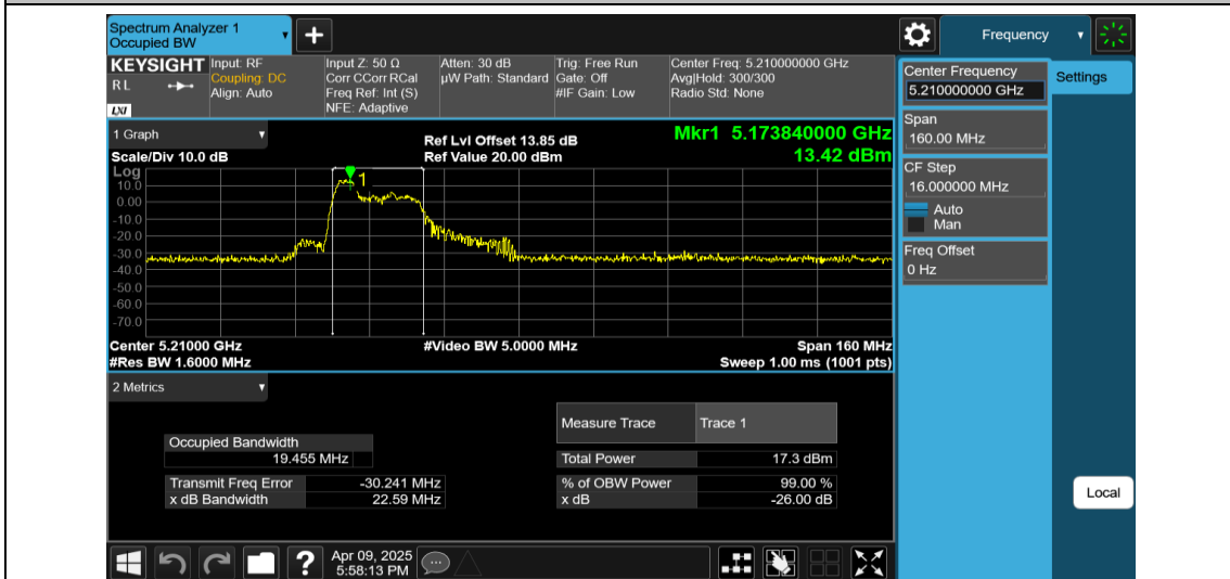
11AX80MIMO-Ant2-5210-52Tone-RU37
