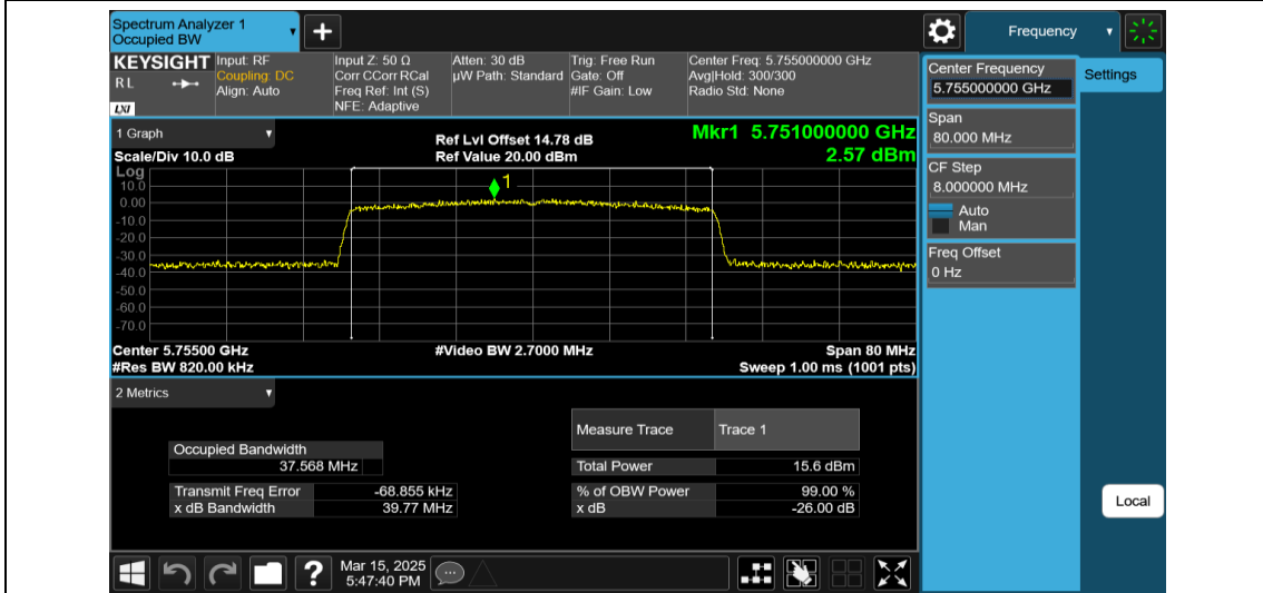
11AX40MIMO-Ant1-5755-484Tone-RU65
