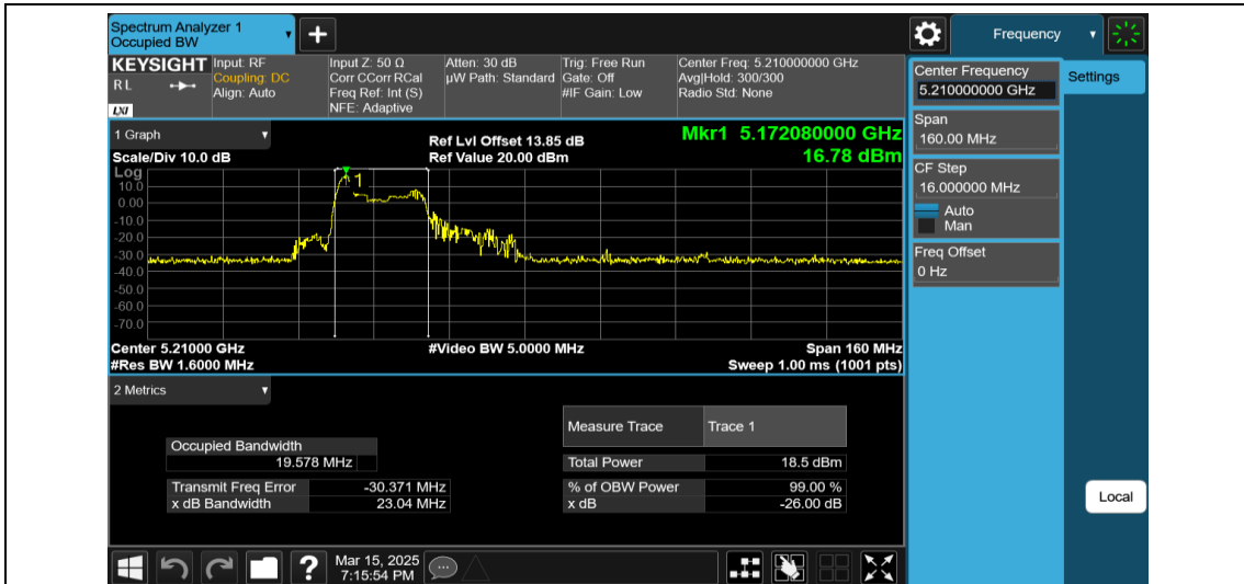
11AX80MIMO-Ant2-5210-26Tone-RU0
