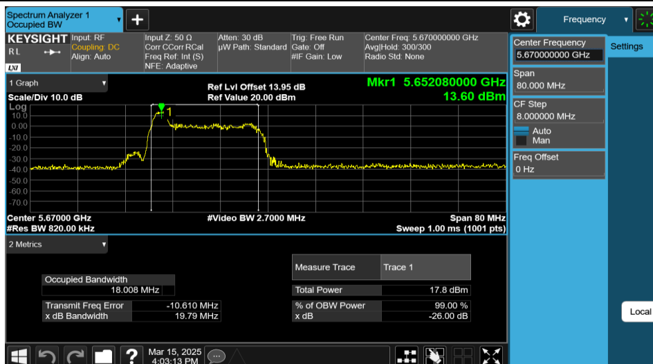
11AX40MIMO-Ant2-5670-26Tone-RU0
