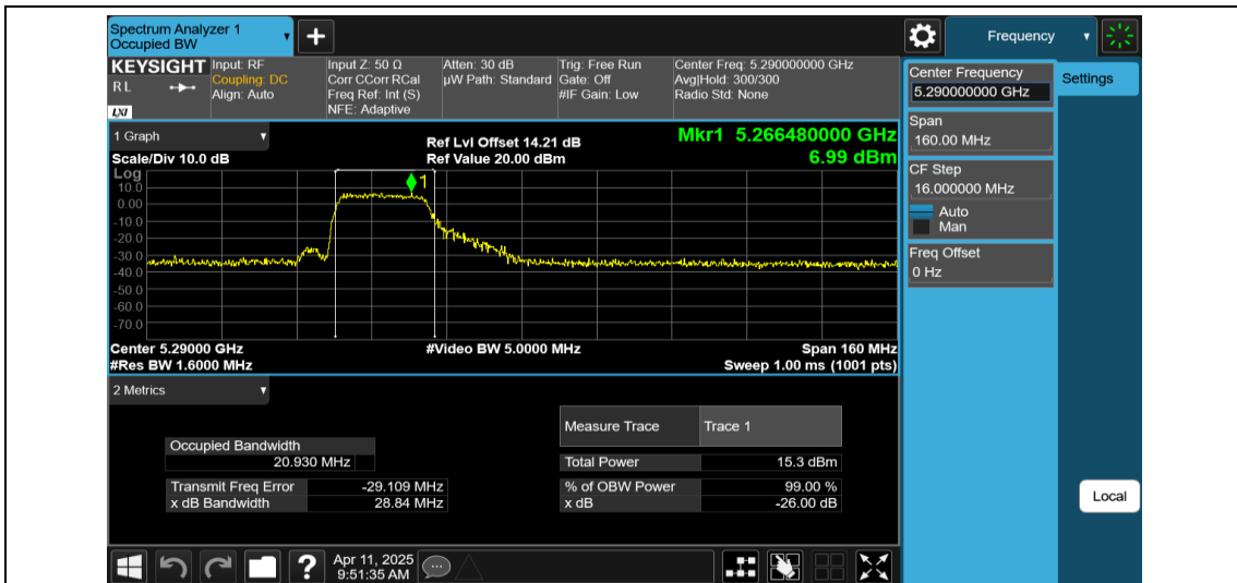
11AX80MIMO-Ant2-5290-242Tone-RU61
