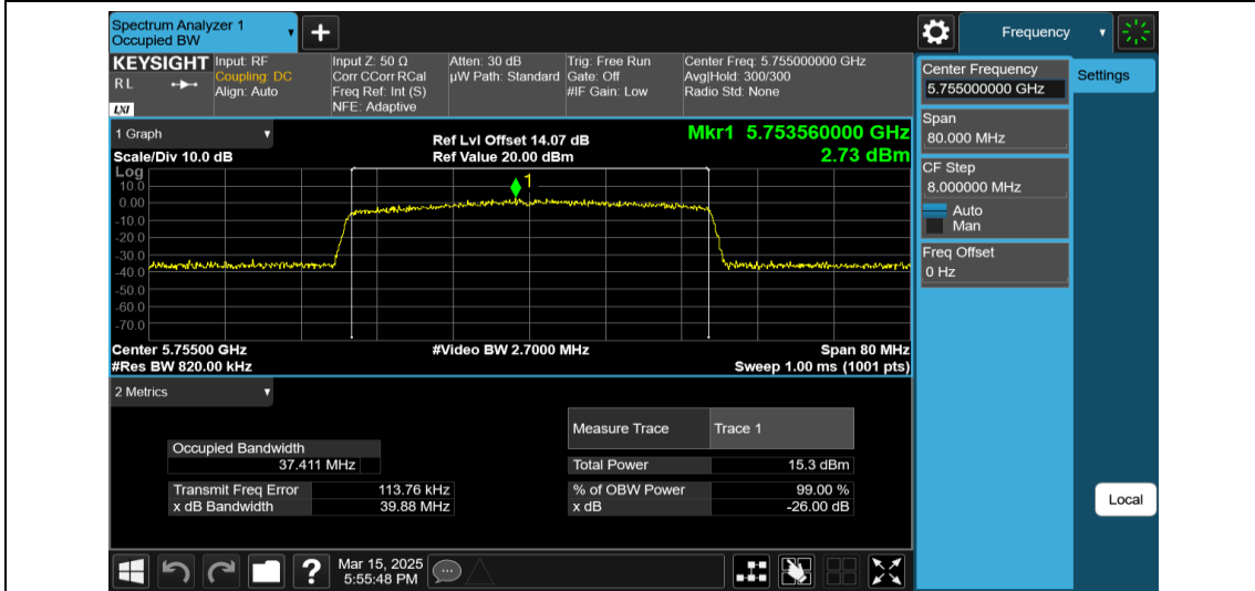
11AX40MIMO-Ant2-5755-484Tone-RU65
