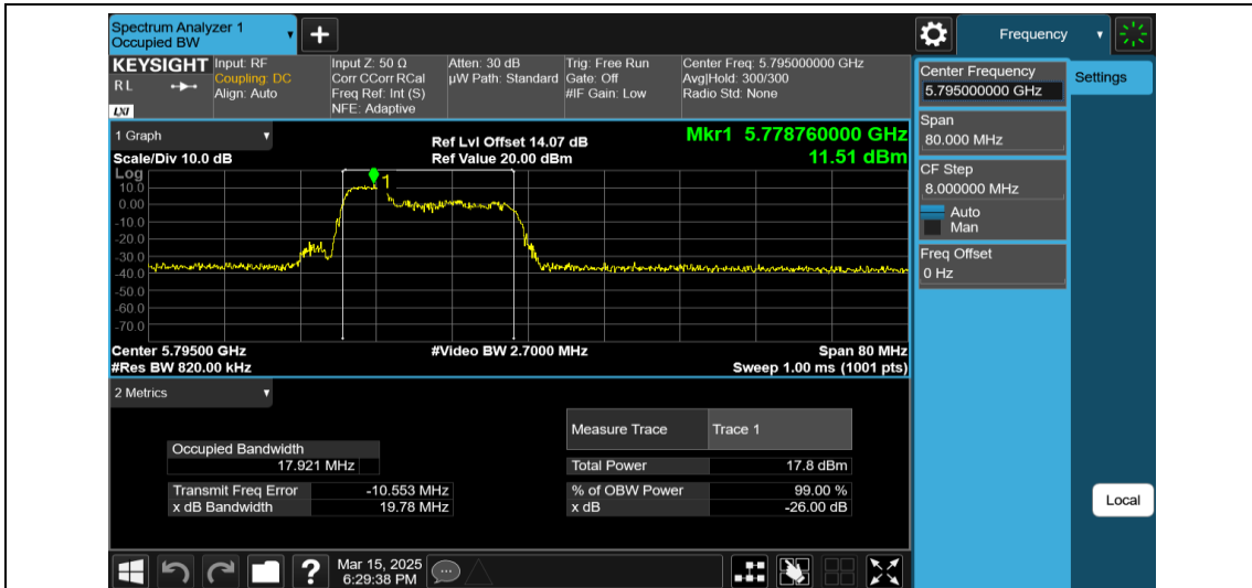
11AX40MIMO-Ant2-5795-52Tone-RU37
