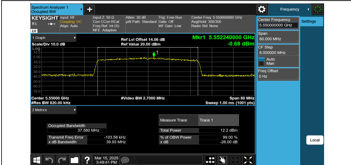
11AX40MIMO-Ant2-5550-484Tone-RU65
