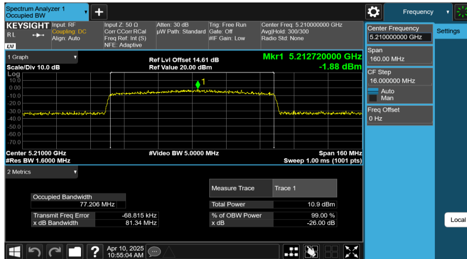
11AX80MIMO-Ant1-5210-996Tone-RU67
