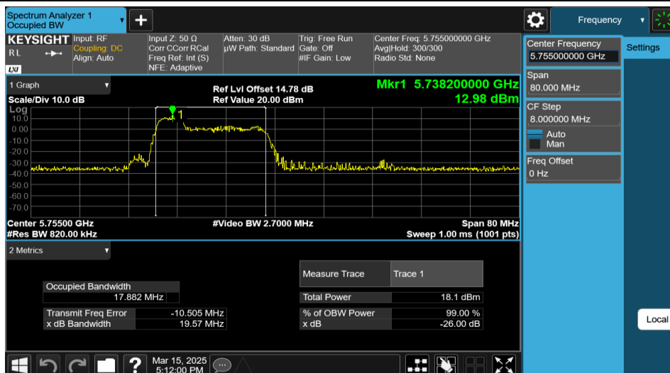
11AX40MIMO-Ant1-5755-52Tone-RU37
