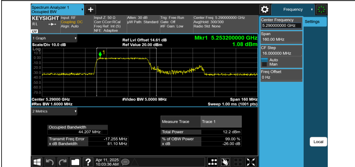
11AX80MIMO-Ant1-5290-484Tone-RU65
