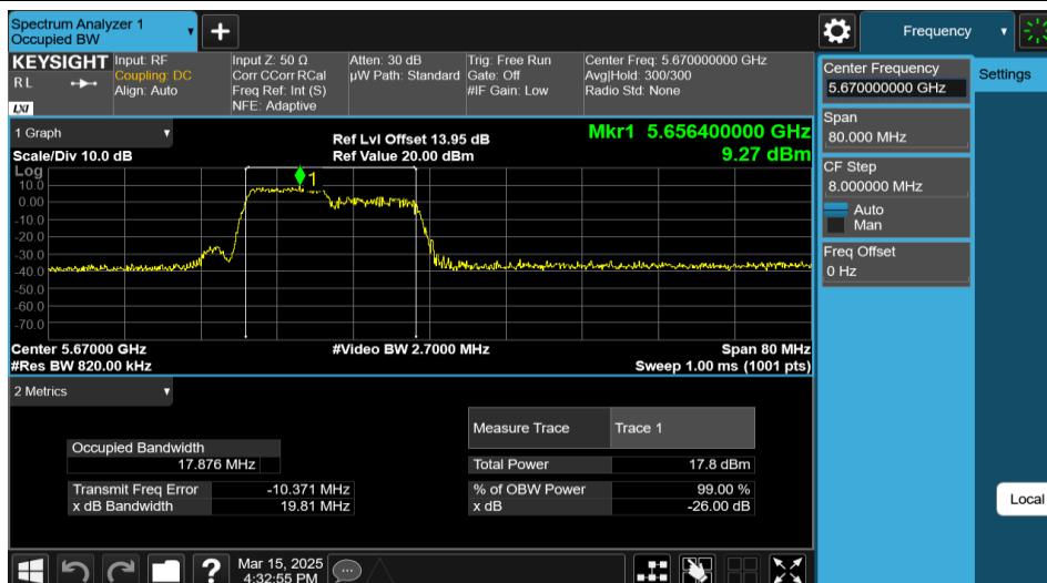
11AX40MIMO-Ant2-5670-106Tone-RU53
