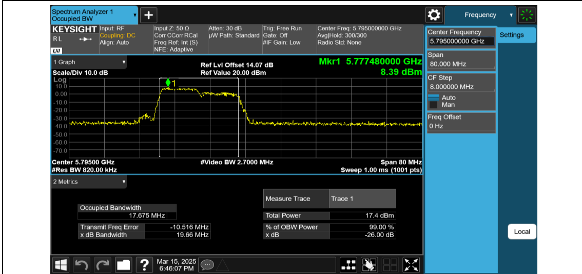
11AX40MIMO-Ant2-5795-106Tone-RU53
