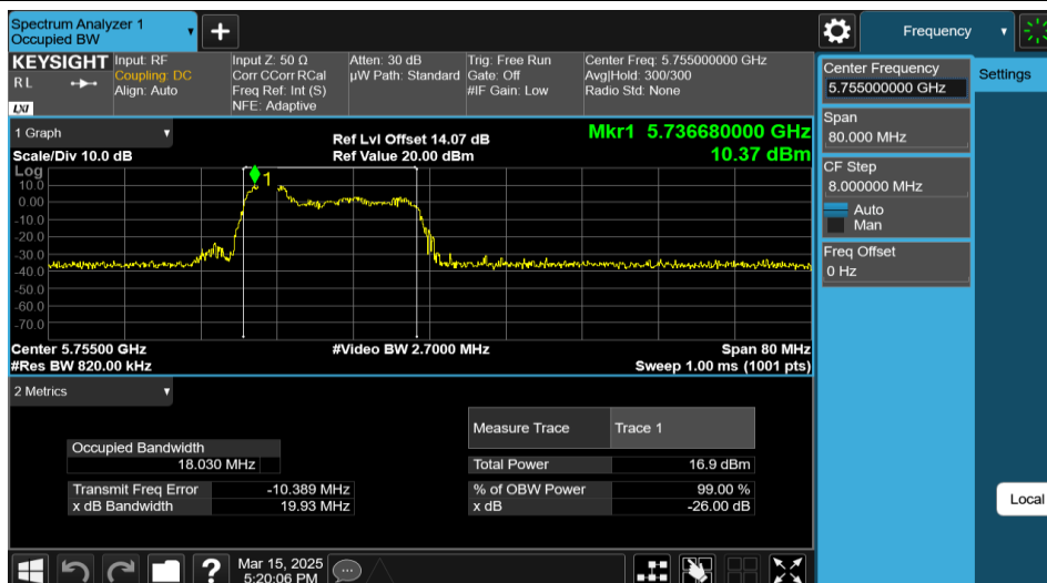
11AX40MIMO-Ant2-5755-52Tone-RU37
