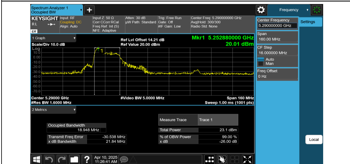
11AX80MIMO-Ant2-5290-52Tone-RU37
