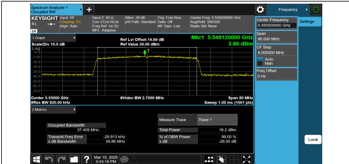
11AX40MIMO-Ant1-5550-484Tone-RU65
