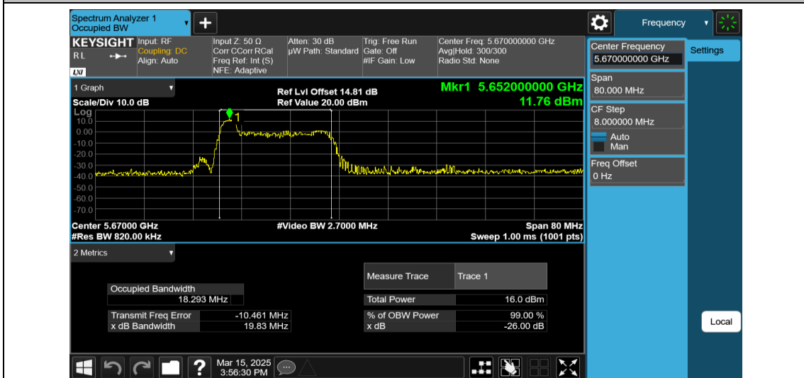
11AX40MIMO-Ant1-5670-26Tone-RU0
