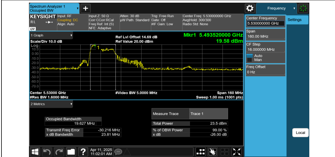
11AX80MIMO-Ant1-5530-52Tone-RU37
