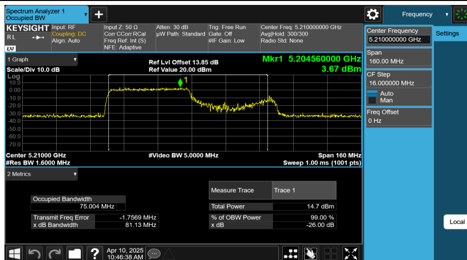
11AX80MIMO-Ant2-5210-484Tone-RU65
