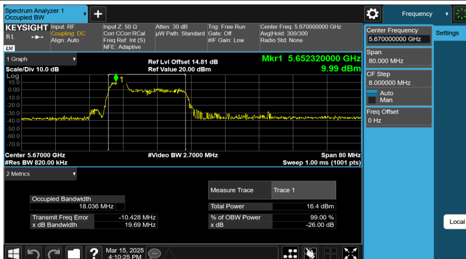
11AX40MIMO-Ant1-5670-52Tone-RU37
