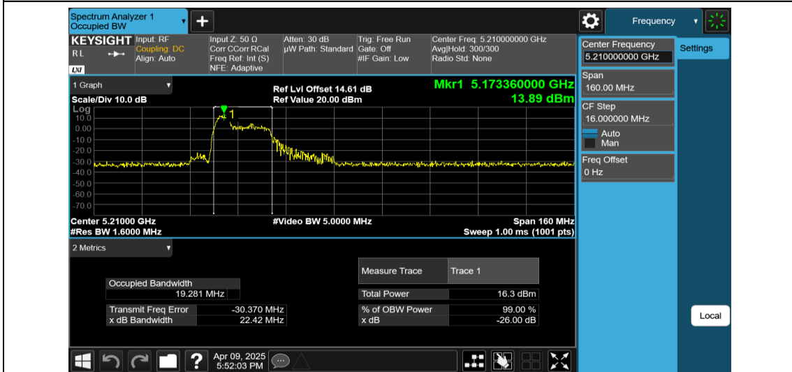
11AX80MIMO-Ant1-5210-52Tone-RU37
