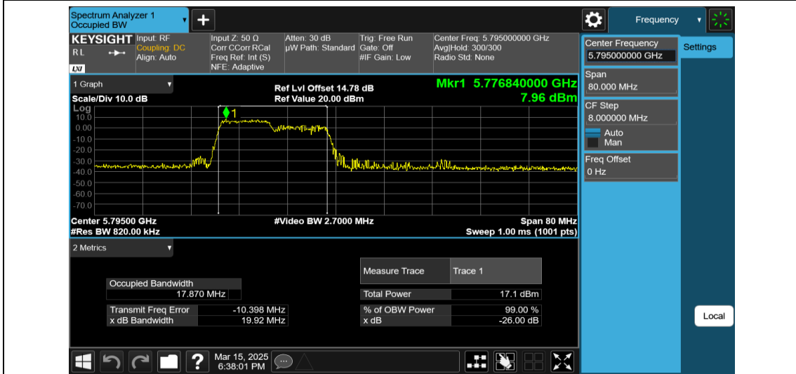
11AX40MIMO-Ant1-5795-106Tone-RU53
