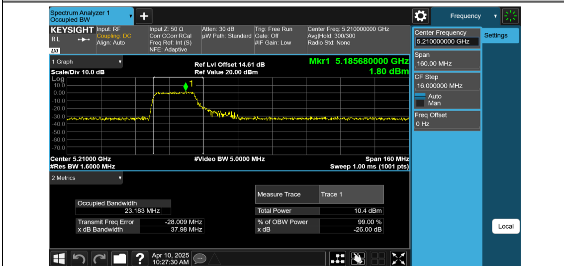
11AX80MIMO-Ant1-5210-242Tone-RU61
