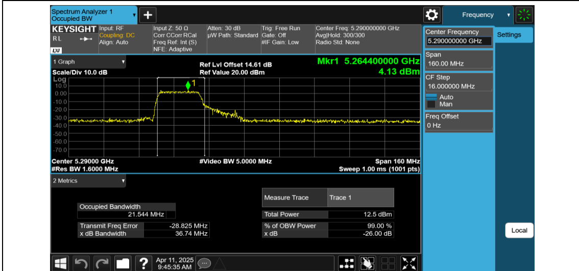
11AX80MIMO-Ant1-5290-242Tone-RU61
