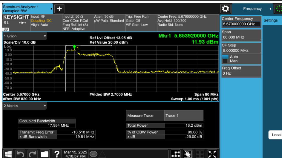
11AX40MIMO-Ant2-5670-52Tone-RU37
