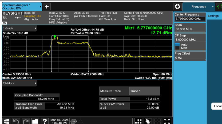
11AX40MIMO-Ant1-5795-26Tone-RU0
