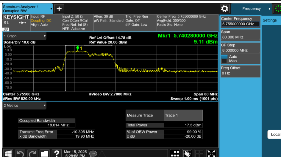
11AX40MIMO-Ant1-5755-106Tone-RU53
