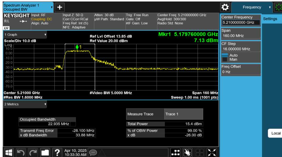
11AX80MIMO-Ant2-5210-242Tone-RU61
