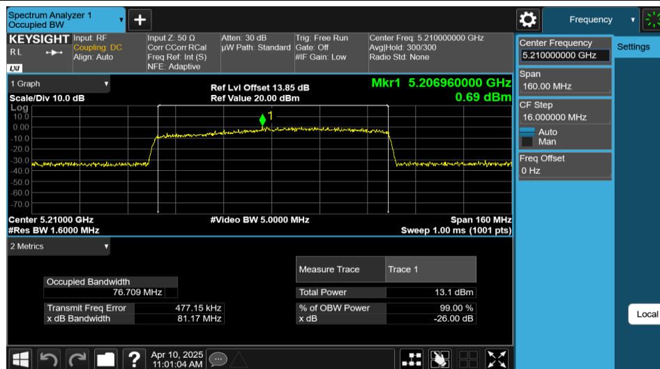
11AX80MIMO-Ant2-5210-996Tone-RU67
