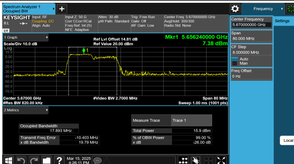
11AX40MIMO-Ant1-5670-106Tone-RU53
