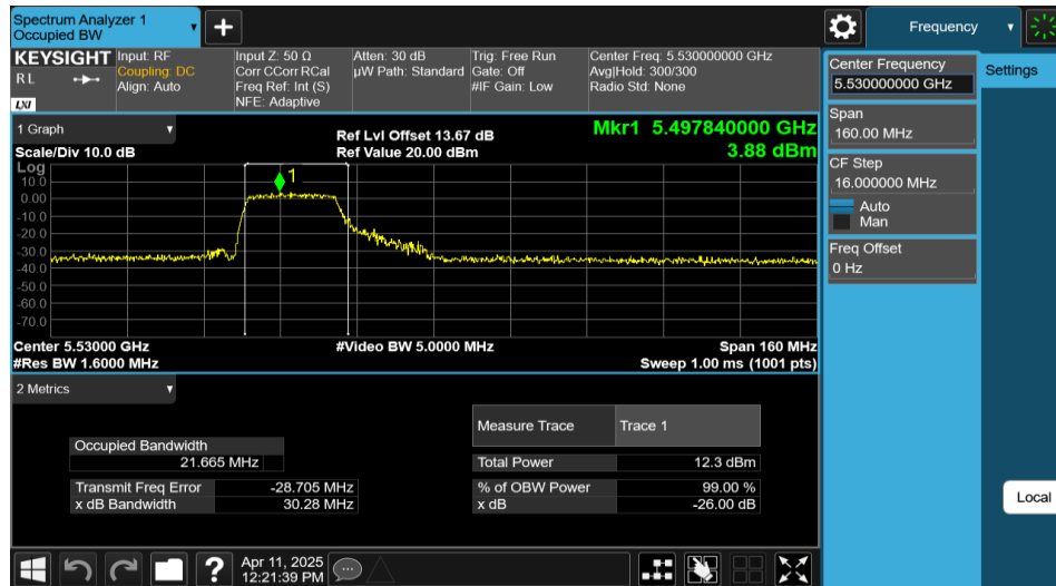
11AX80MIMO-Ant2-5530-242Tone-RU61
