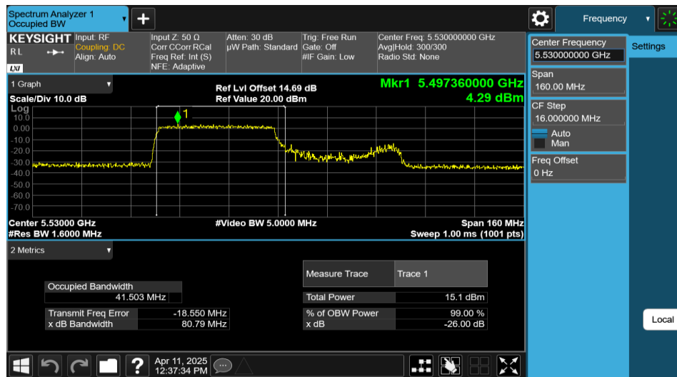
11AX80MIMO-Ant1-5530-484Tone-RU65
