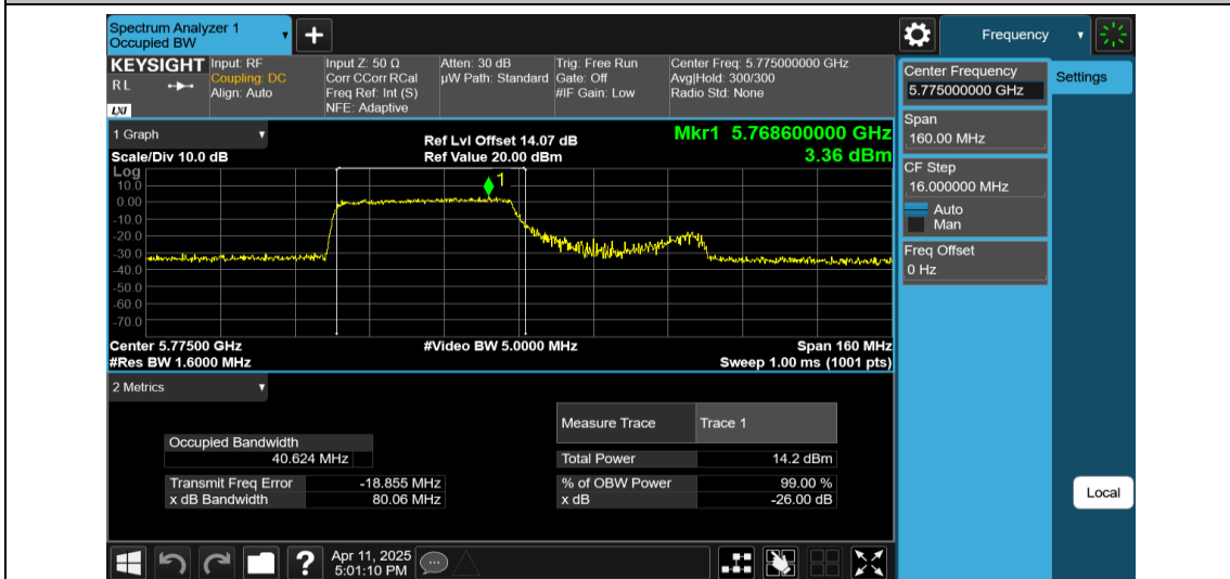
11AX80MIMO-Ant2-5775-484Tone-RU65
