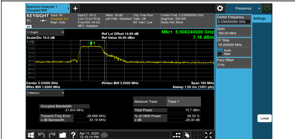
11AX80MIMO-Ant1-5530-242Tone-RU61
