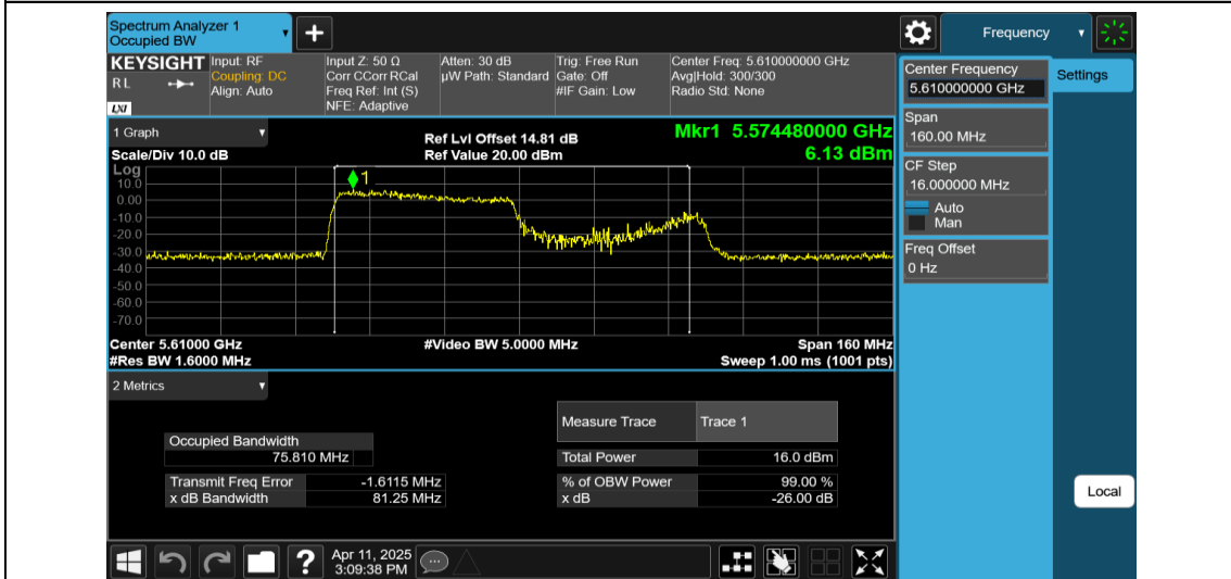
11AX80MIMO-Ant1-5610-484Tone-RU65
