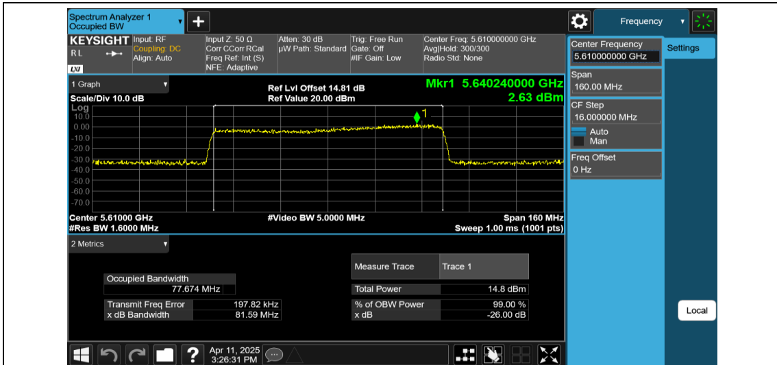
11AX80MIMO-Ant1-5610-996Tone-RU67
