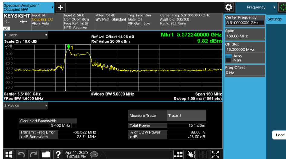
11AX80MIMO-Ant2-5610-26Tone-RU0
