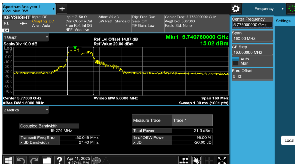
11AX80MIMO-Ant2-5775-106Tone-RU53
