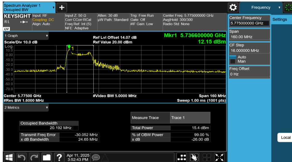
11AX80MIMO-Ant2-5775-26Tone-RU0
