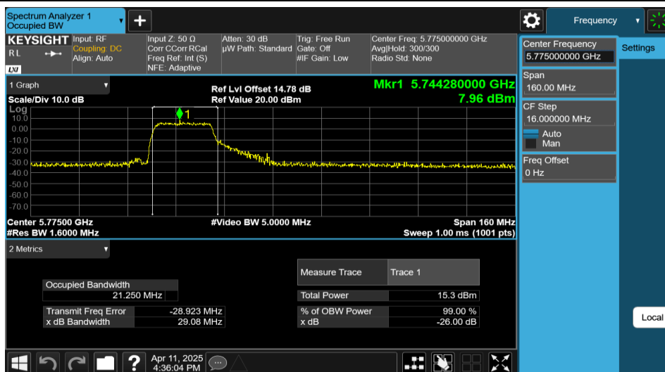
11AX80MIMO-Ant1-5775-242Tone-RU61
