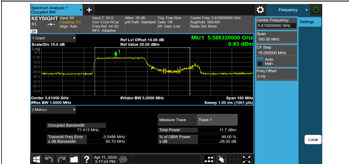
11AX80MIMO-Ant2-5610-484Tone-RU65
