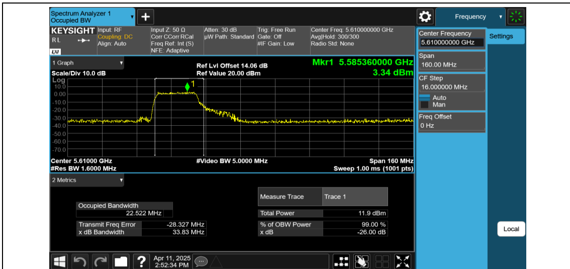
11AX80MIMO-Ant2-5610-242Tone-RU61
