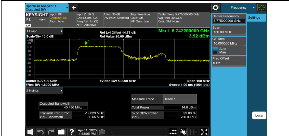
11AX80MIMO-Ant1-5775-484Tone-RU65
