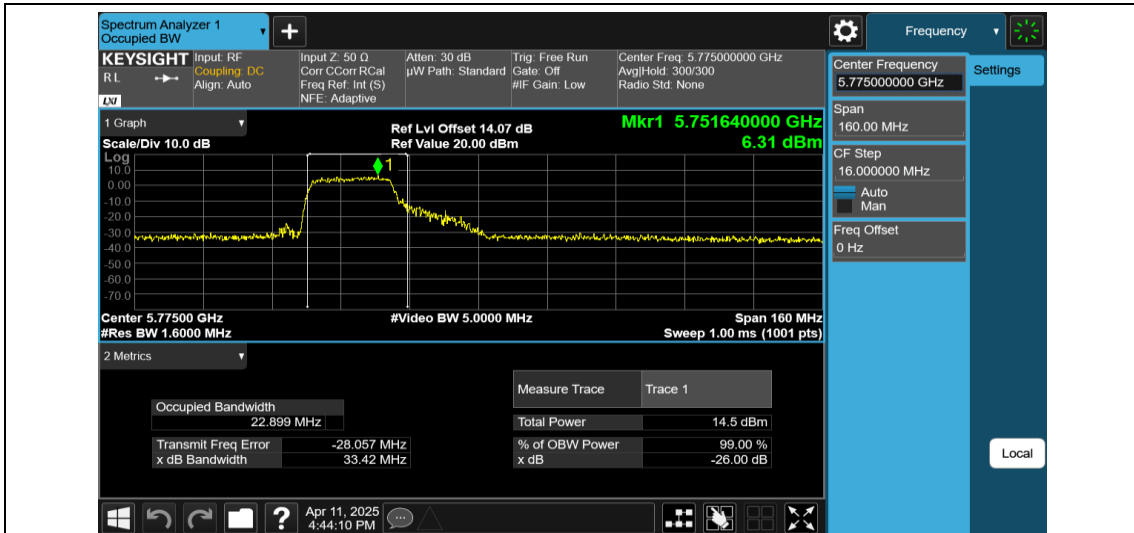
11AX80MIMO-Ant2-5775-242Tone-RU61
