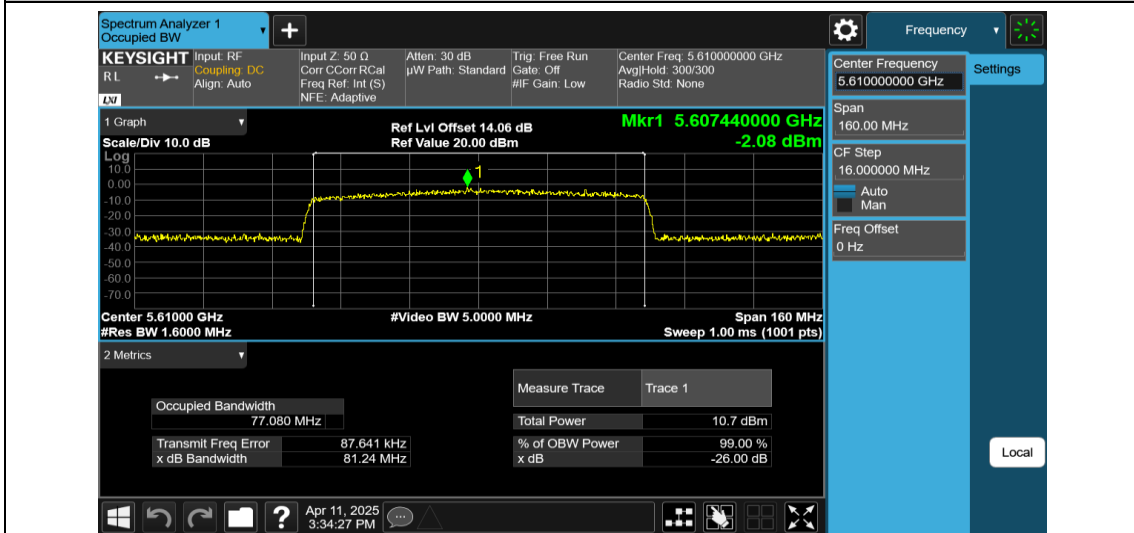
11AX80MIMO-Ant2-5610-996Tone-RU67
