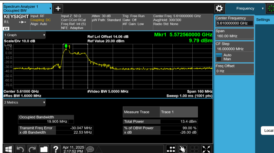
11AX80MIMO-Ant2-5610-52Tone-RU37
