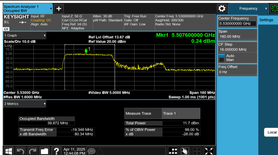
11AX80MIMO-Ant2-5530-484Tone-RU65
