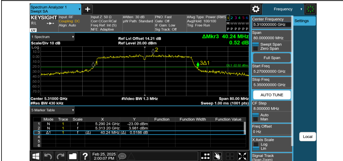
11N40MIMO-Ant2-5310
