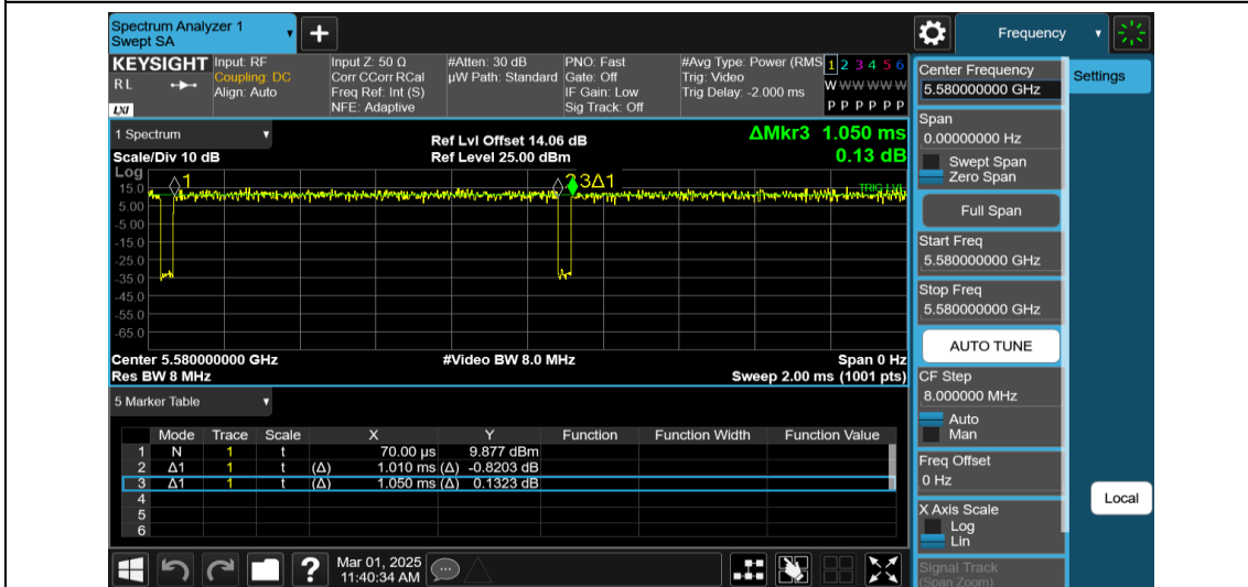
NTNV-11AX20MIMO-Ant2-5580
