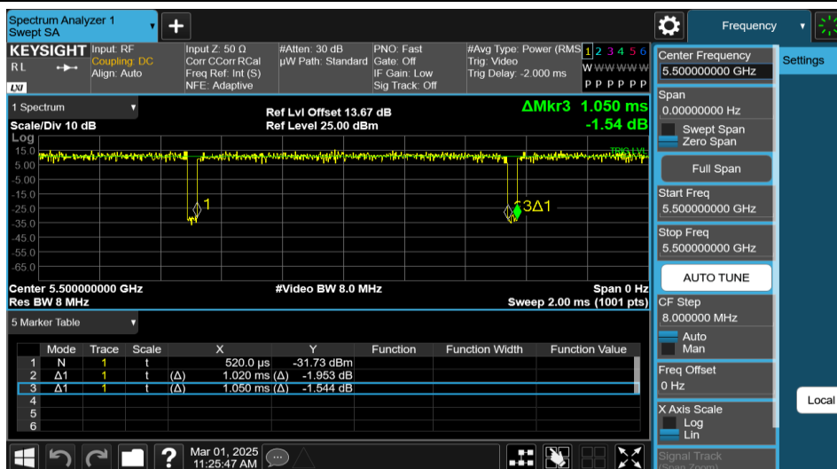
NTNV-11AX20MIMO-Ant2-5500
