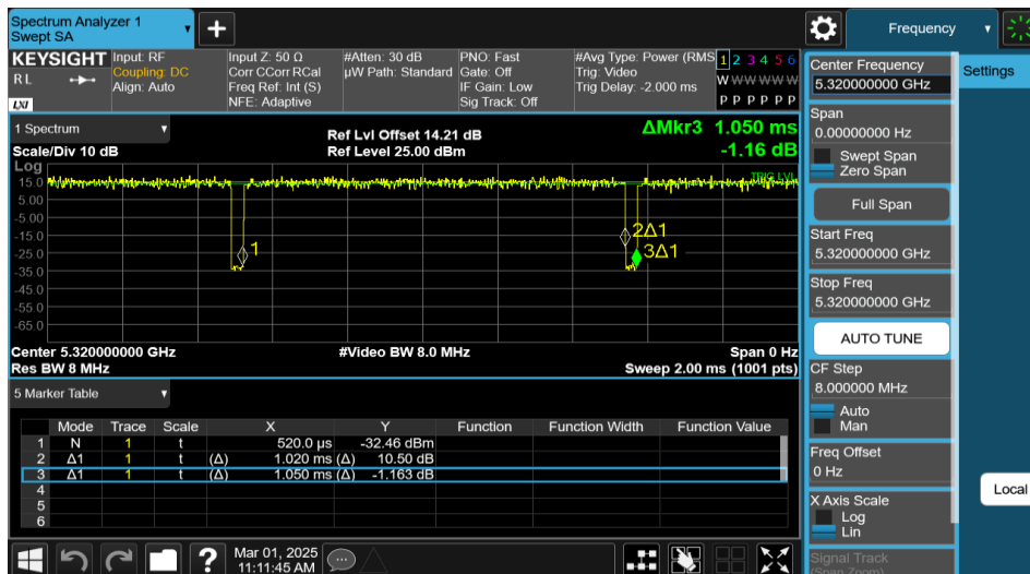
NTNV-11AX20MIMO-Ant2-5320
