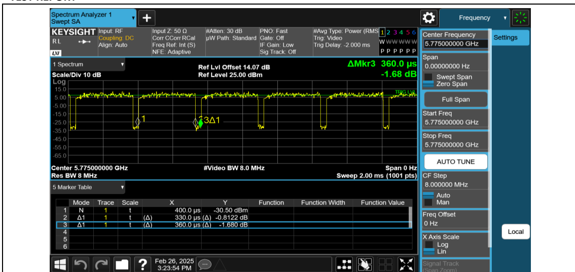
NTNV-11AC80MIMO-Ant2-5775
