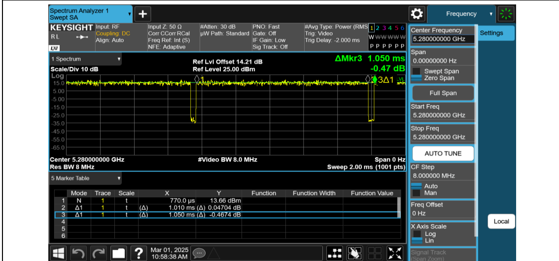
NTNV-11AX20MIMO-Ant2-5280
