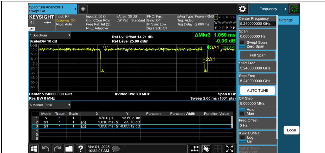
NTNV-11AX20MIMO-Ant2-5240
