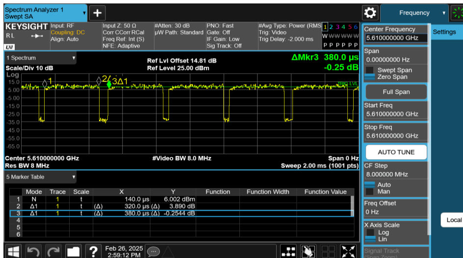
NTNV-11AC80MIMO-Ant1-5610
