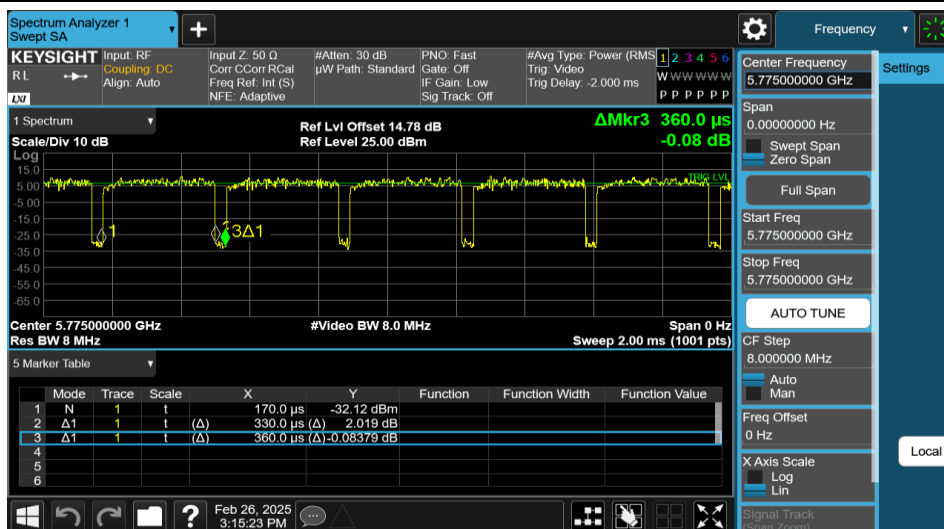
NTNV-11AC80MIMO-Ant1-5775
