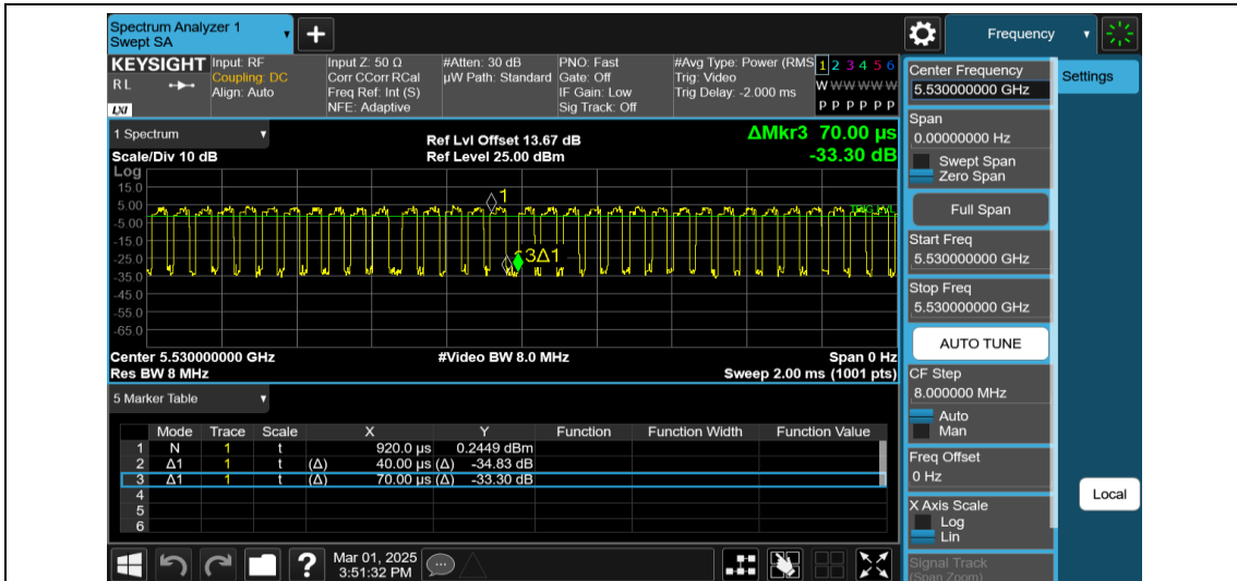
NTNV-11AX80MIMO-Ant2-5530
