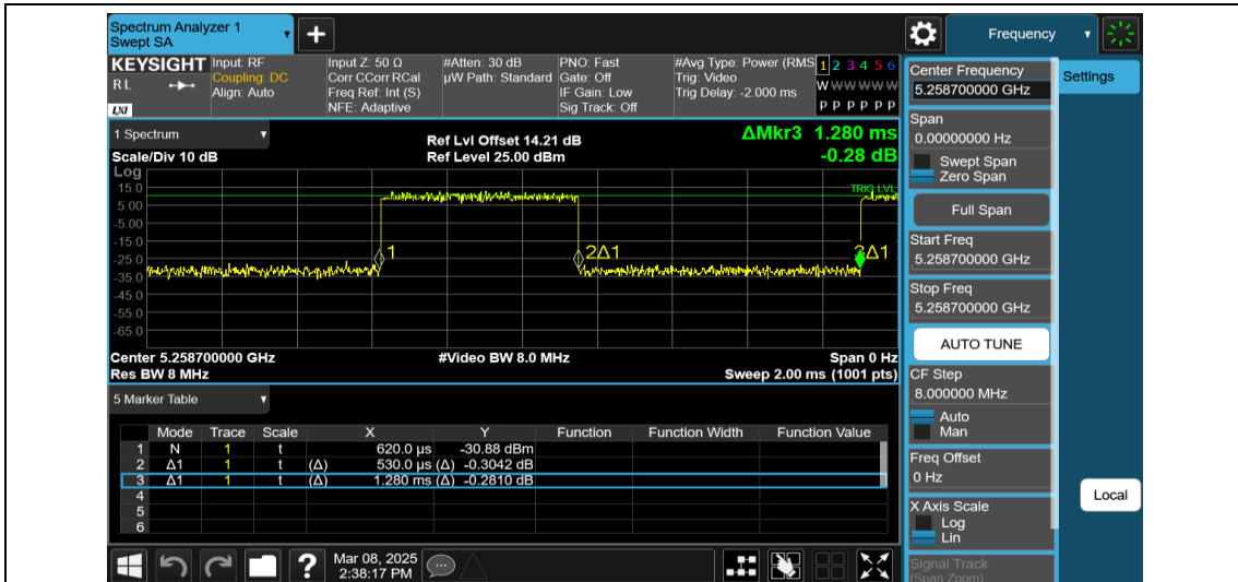
NTVN-11AX20MIMO-Ant2-5260-242Tone-RU61
