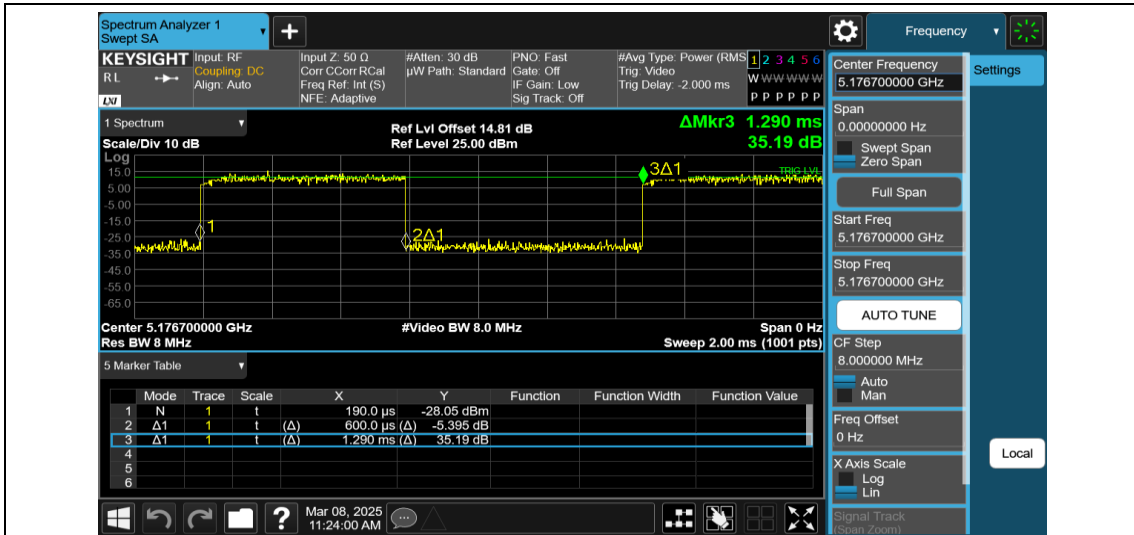
NTNV-11AX20MIMO-Ant1-5180-106Tone-RU53
