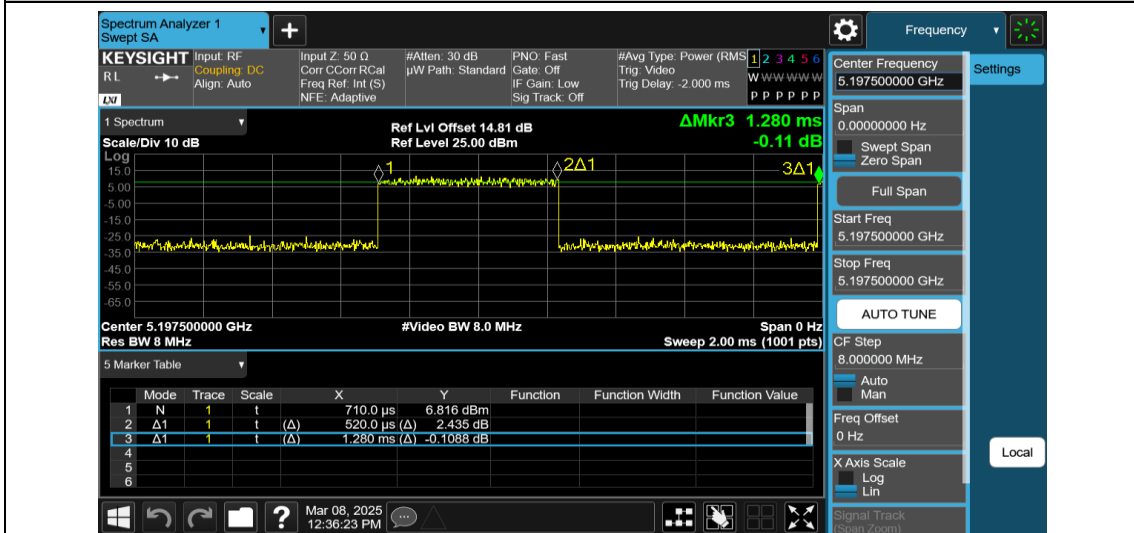
NTNV-11AX20MIMO-Ant1-5200-242Tone-RU61
