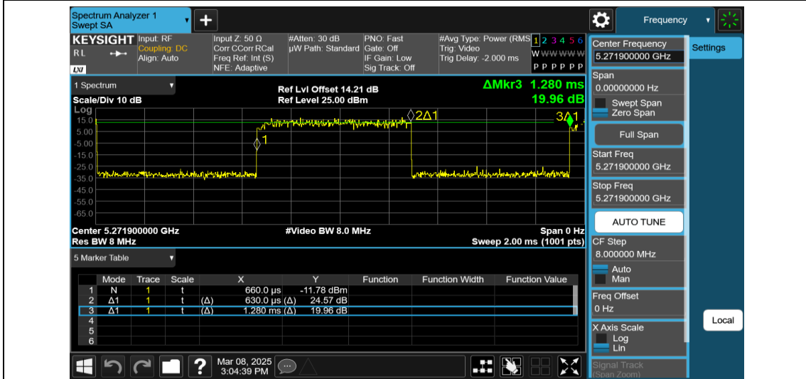
NTNV-11AX20MIMO-Ant2-5280-52Tone-RU37
