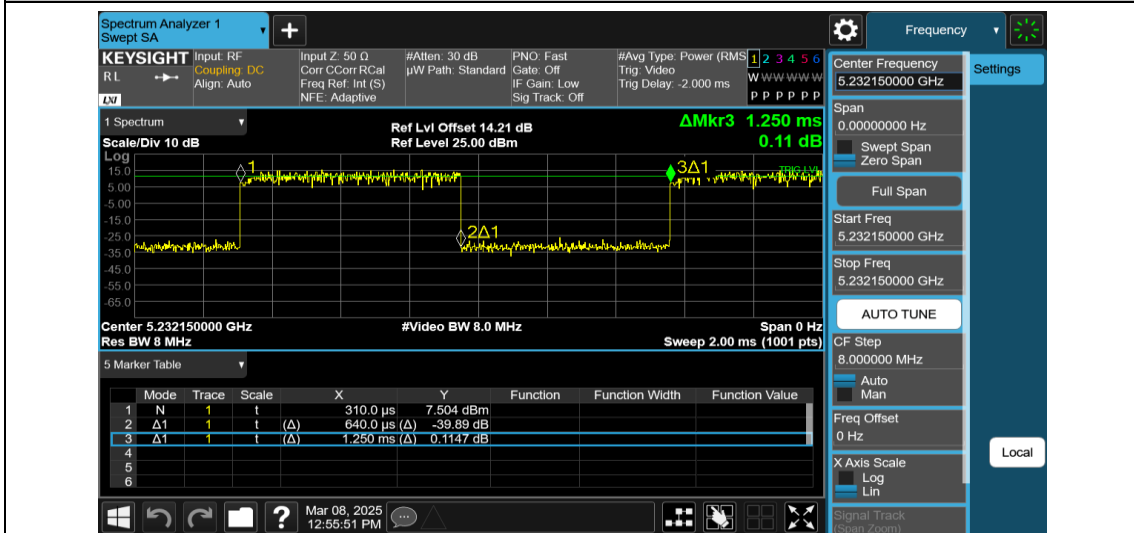
NTNV-11AX20MIMO-Ant2-5240-26Tone-RU0
