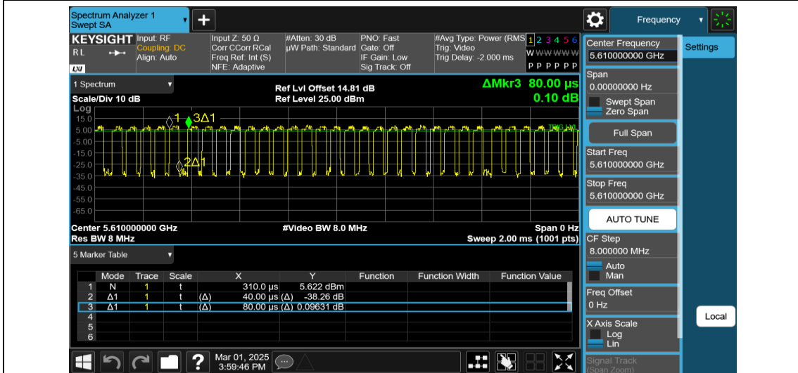
NTNV-11AX80MIMO-Ant1-5610
