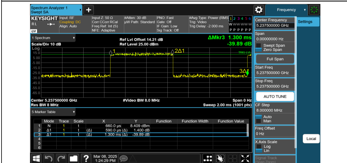
NTNV-11AX20MIMO-Ant2-5240-106Tone-RU53
