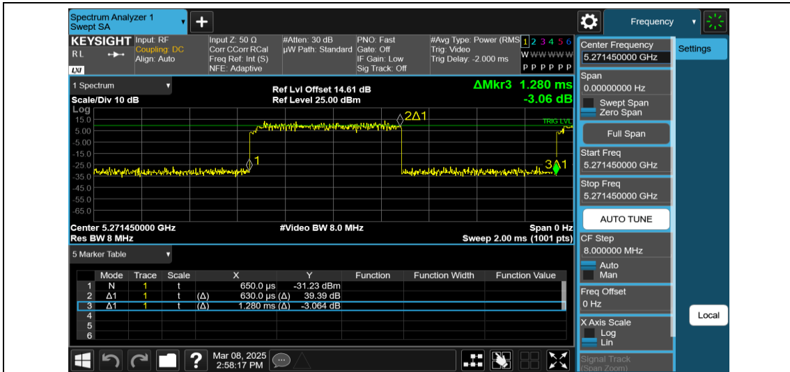
NTNV-11AX20MIMO-Ant1-5280-52Tone-RU37
