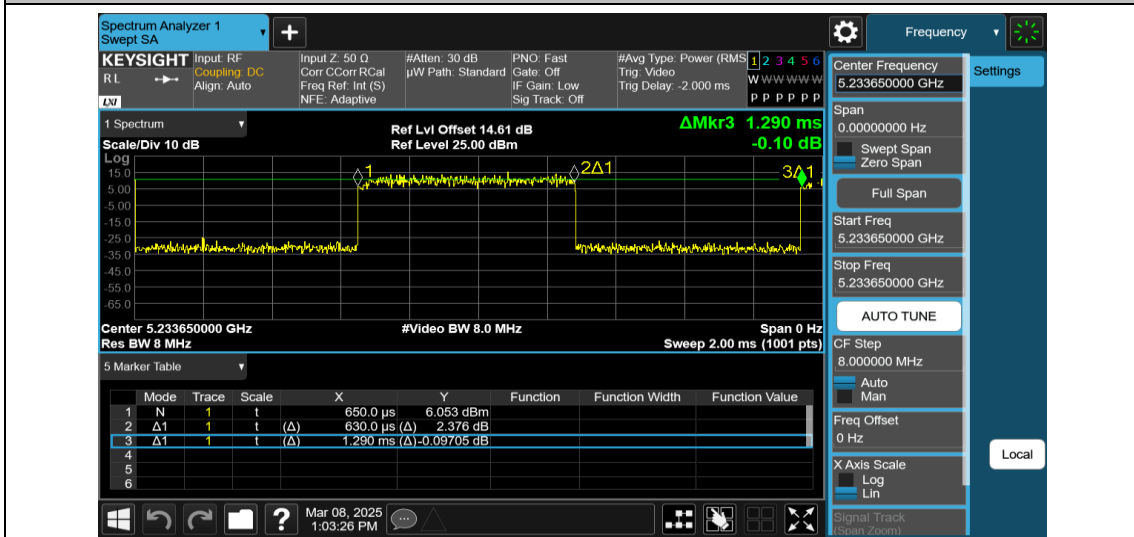
NTNV-11AX20MIMO-Ant1-5240-52Tone-RU37
