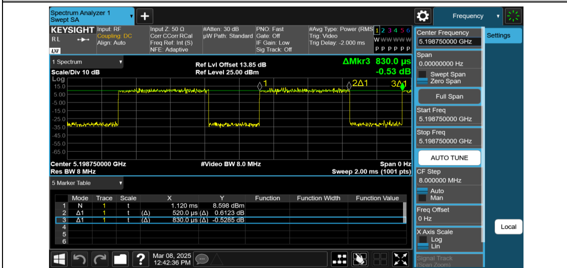
NTNV-11AX20MIMO-Ant2-5200-242Tone-RU61
