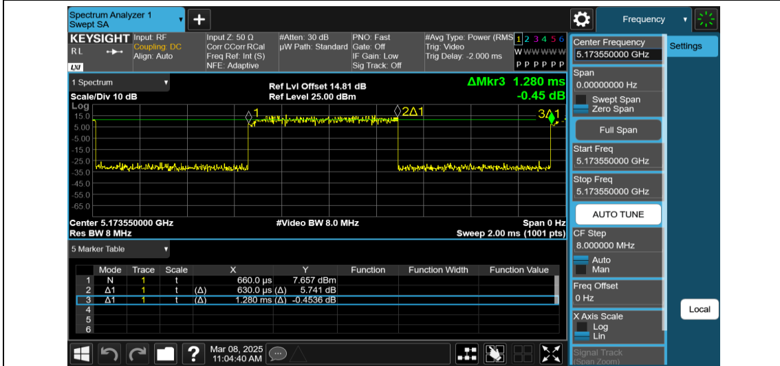
NTNV-11AX20MIMO-Ant1-5180-52Tone-RU37
