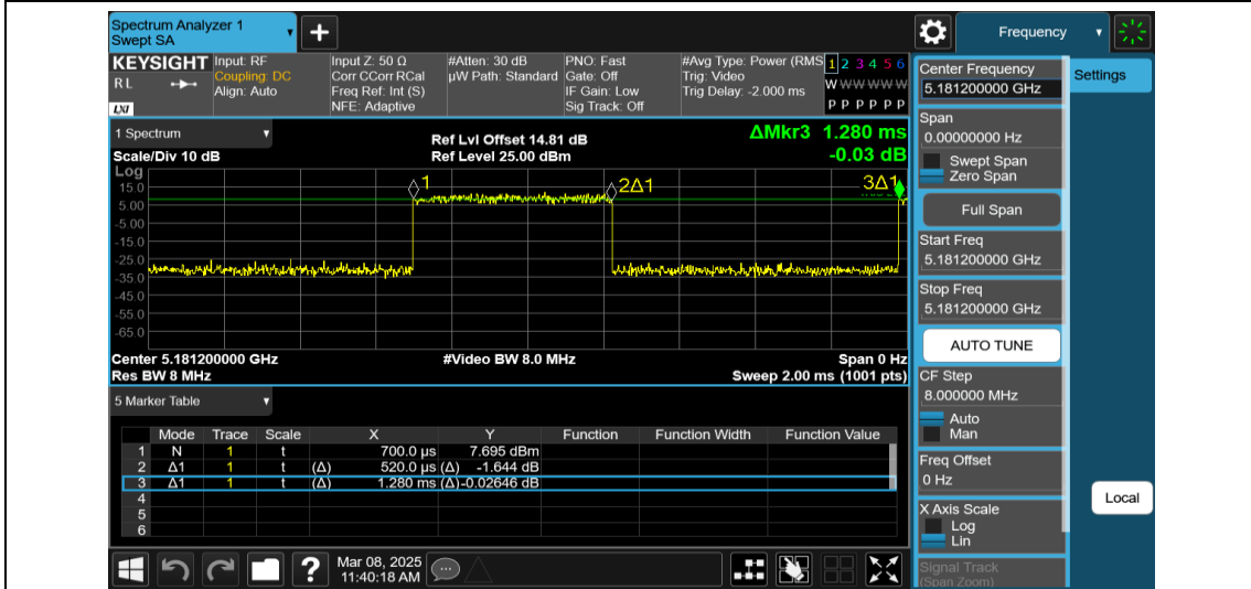
NTNV-11AX20MIMO-Ant1-5180-242Tone-RU61
