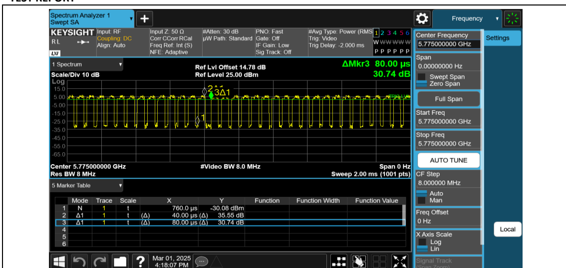
NTNV-11AX80MIMO-Ant1-5775
