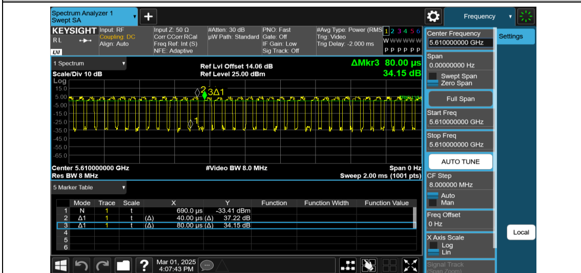
NTNV-11AX80MIMO-Ant2-5610
