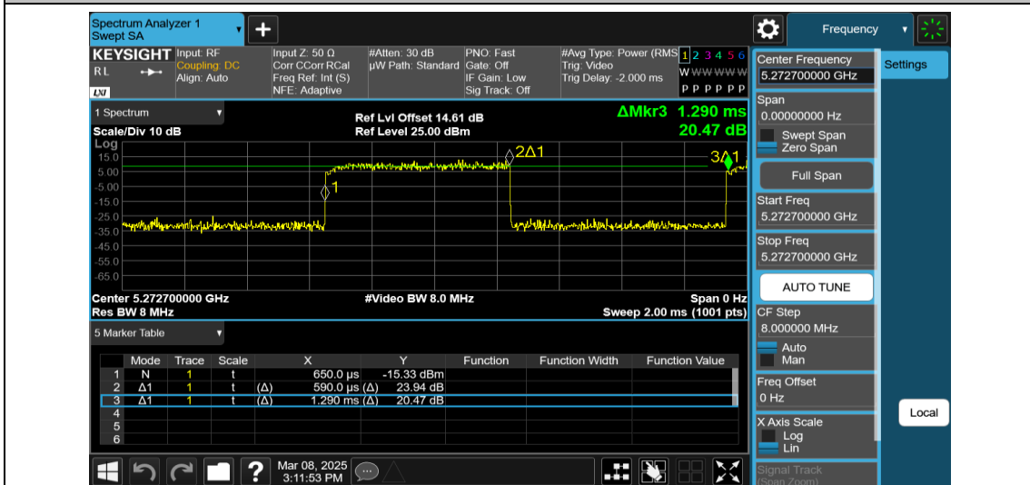
NTNV-11AX20MIMO-Ant1-5280-106Tone-RU53
