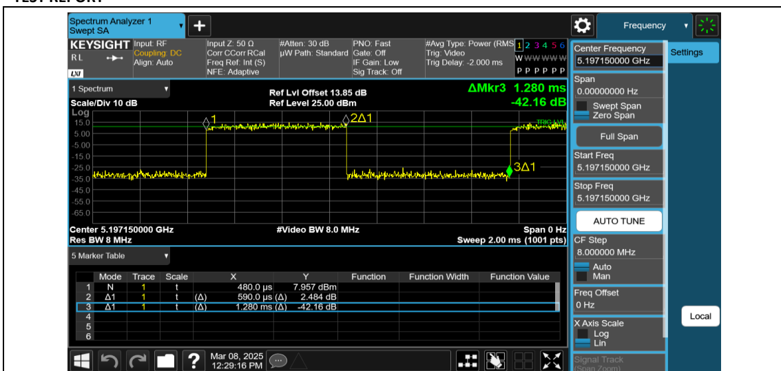
NTNV-11AX20MIMO-Ant2-5200-106Tone-RU53
