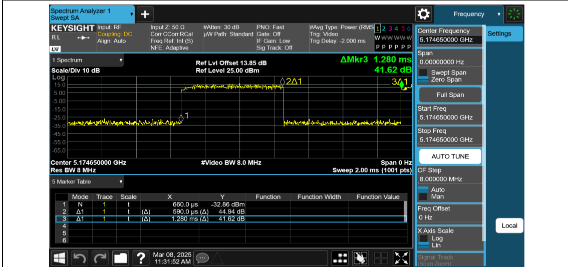
NTNV-11AX20MIMO-Ant2-5180-106Tone-RU53
