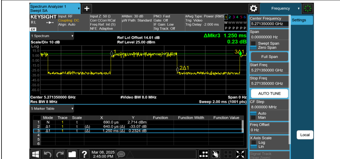
NTVN-11AX20MIMO-Ant1-5280-26Tone-RU0
