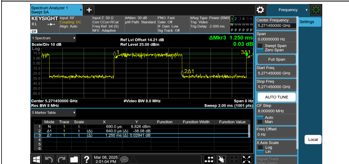
NTVN-11AX20MIMO-Ant2-5280-26Tone-RU0
