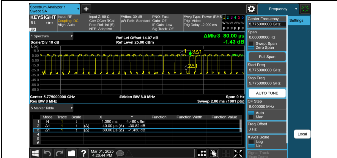
NTNV-11AX80MIMO-Ant2-5775
