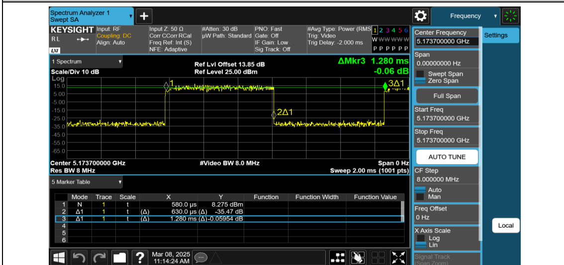
NTNV-11AX20MIMO-Ant2-5180-52Tone-RU37
