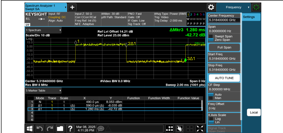
NTNV-11AX20MIMO-Ant2-5320-106Tone-RU53
