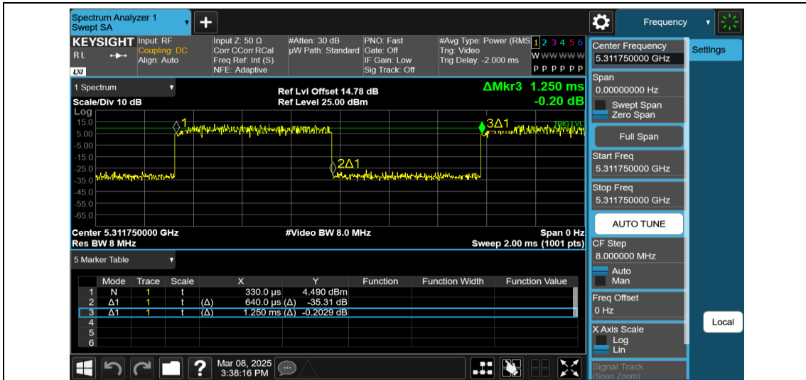
NTNV-11AX20MIMO-Ant1-5320-26Tone-RU0
