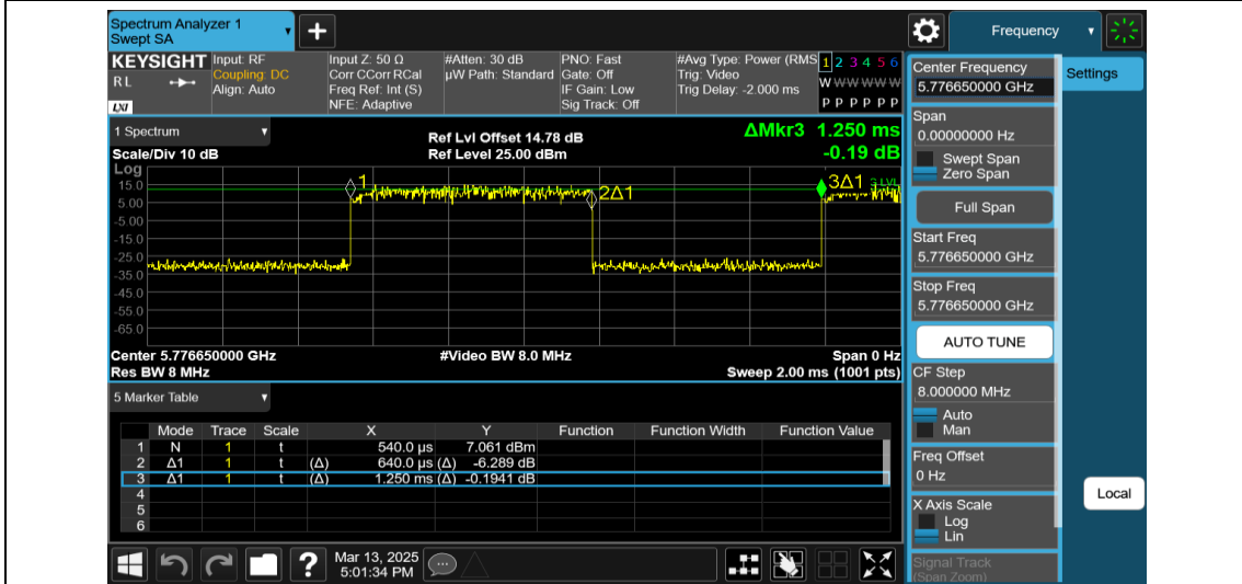
NTVN-11AX20MIMO-Ant1-5785-26Tone-RU0
