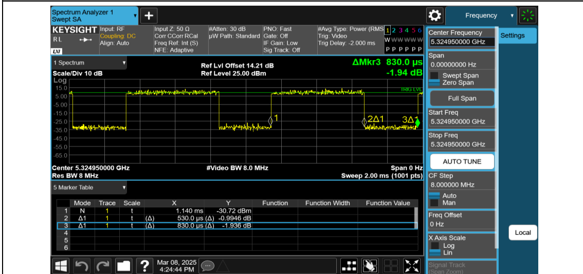
NTNV-11AX20MIMO-Ant2-5320-242Tone-RU61
