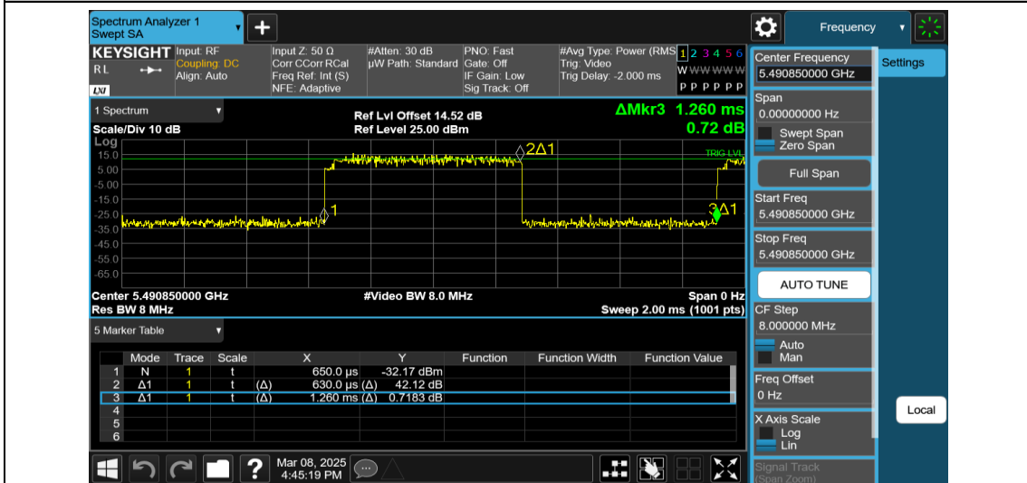
NTNV-11AX20MIMO-Ant1-5500-52Tone-RU37
