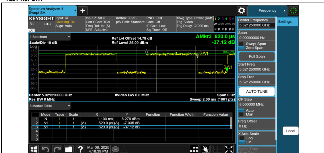
NTNV-11AX20MIMO-Ant1-5320-242Tone-RU61
