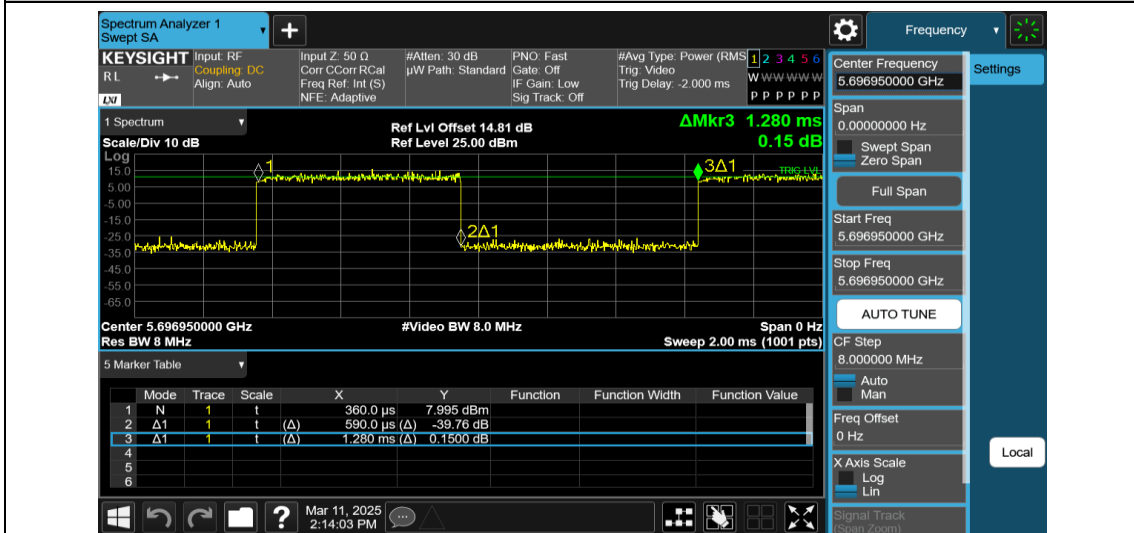
NTNV-11AX20MIMO-Ant1-5700-106Tone-RU53
