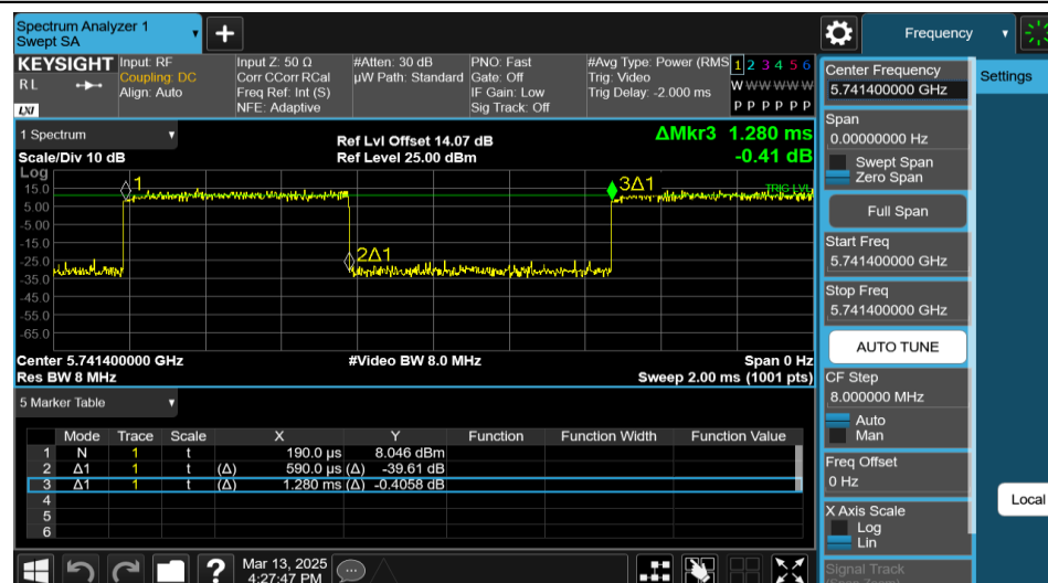
NTNV-11AX20MIMO-Ant2-5745-106Tone-RU53
