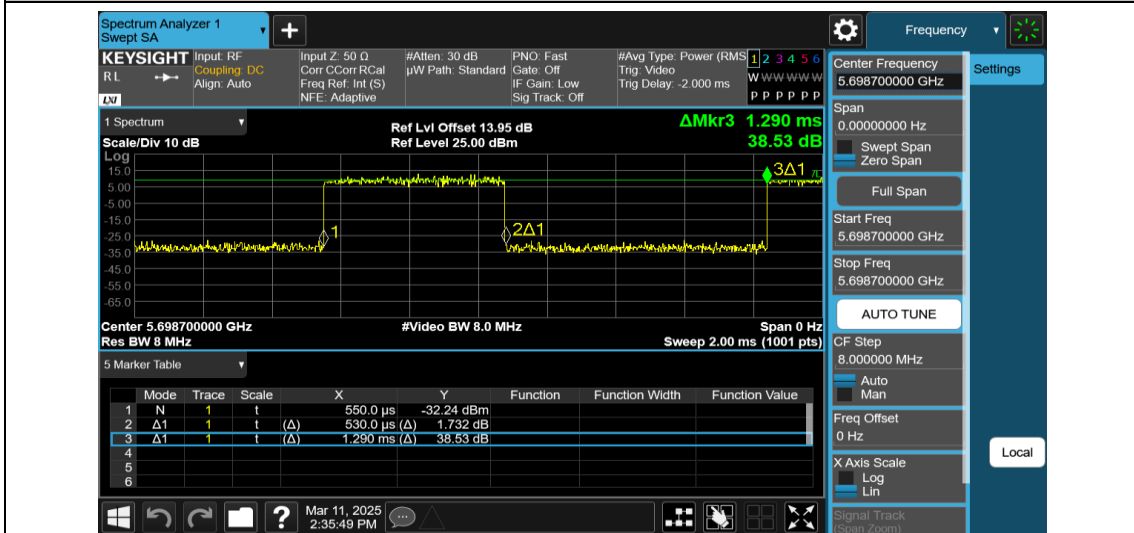
NTNV-11AX20MIMO-Ant2-5700-242Tone-RU61
