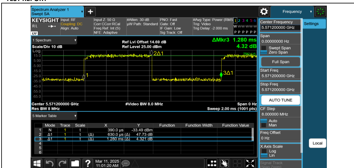
NTNV-11AX20MIMO-Ant1-5580-52Tone-RU37
