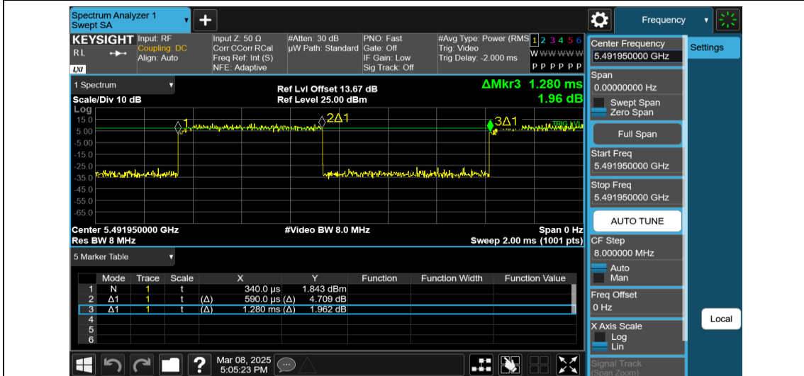
NTVN-11AX20MIMO-Ant2-5500-106Tone-RU53
