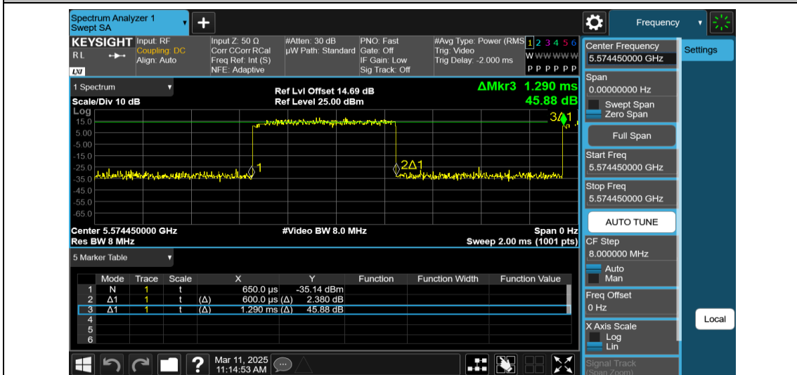
NTNV-11AX20MIMO-Ant1-5580-106Tone-RU53
