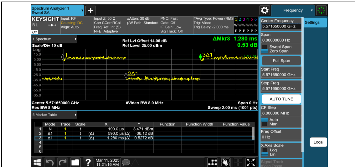
NTNV-11AX20MIMO-Ant2-5580-106Tone-RU53
