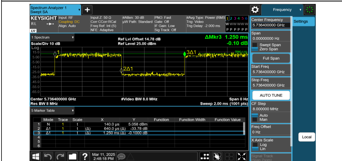
NTNV-11AX20MIMO-Ant1-5745-26Tone-RU0
