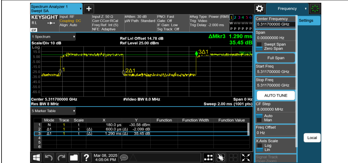
NTNV-11AX20MIMO-Ant1-5320-106Tone-RU53
