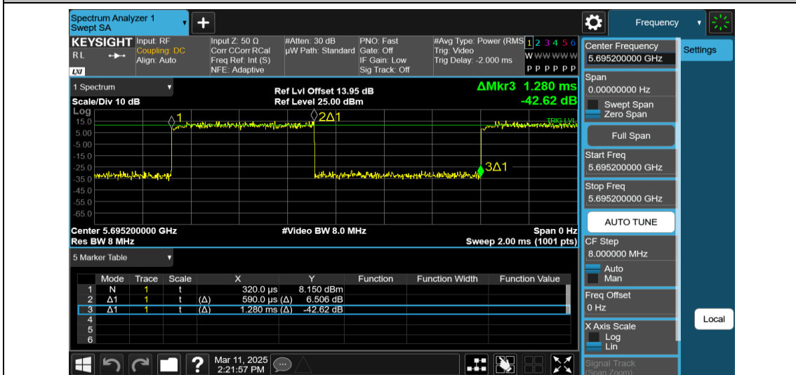
NTNV-11AX20MIMO-Ant2-5700-106Tone-RU53
