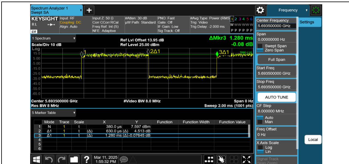
NTNV-11AX20MIMO-Ant2-5700-52Tone-RU37
