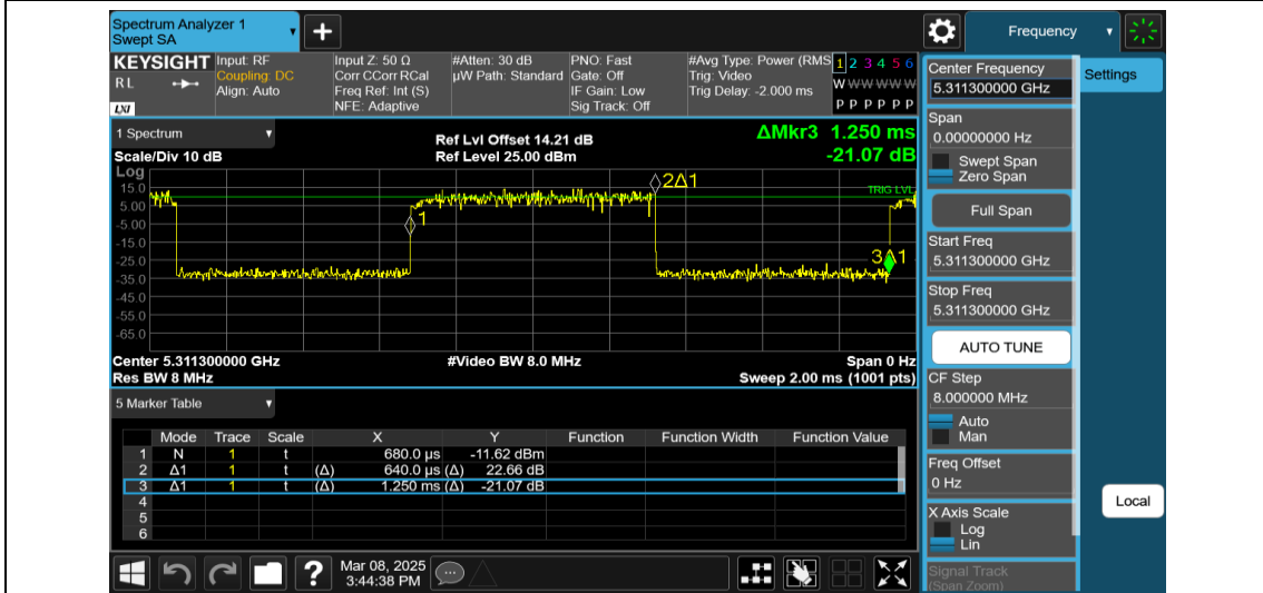
NTNV-11AX20MIMO-Ant2-5320-26Tone-RU0
