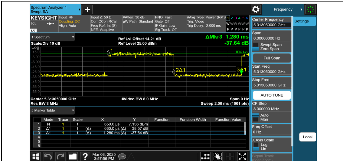
NTNV-11AX20MIMO-Ant2-5320-52Tone-RU37
