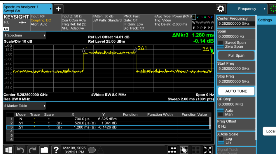
NTNV-11AX20MIMO-Ant1-5280-242Tone-RU61
