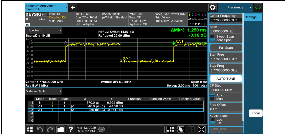
NTVN-11AX20MIMO-Ant2-5785-26Tone-RU0
