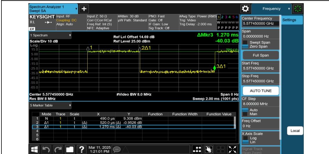
NTNV-11AX20MIMO-Ant1-5580-242Tone-RU61
