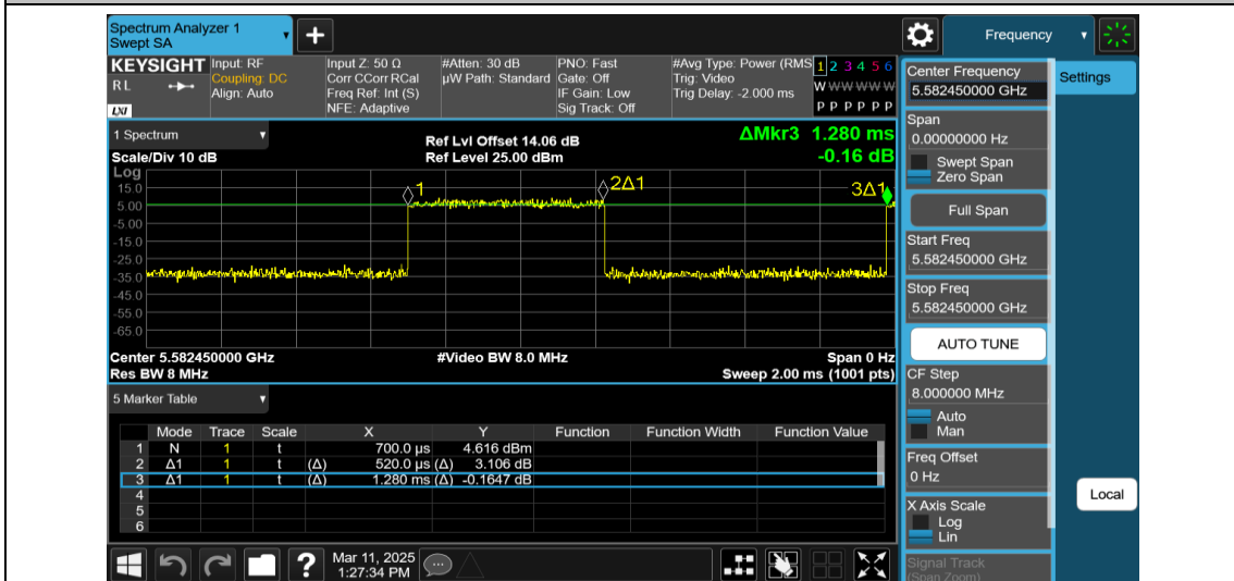
NTNV-11AX20MIMO-Ant2-5580-242Tone-RU61
