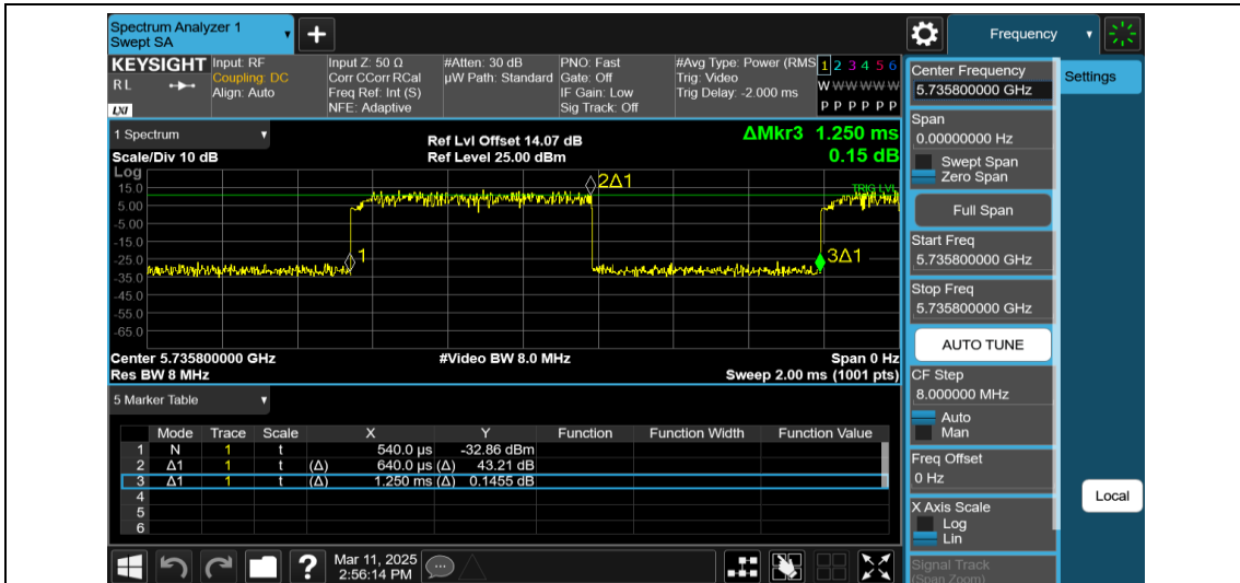
NTNV-11AX20MIMO-Ant2-5745-26Tone-RU0
