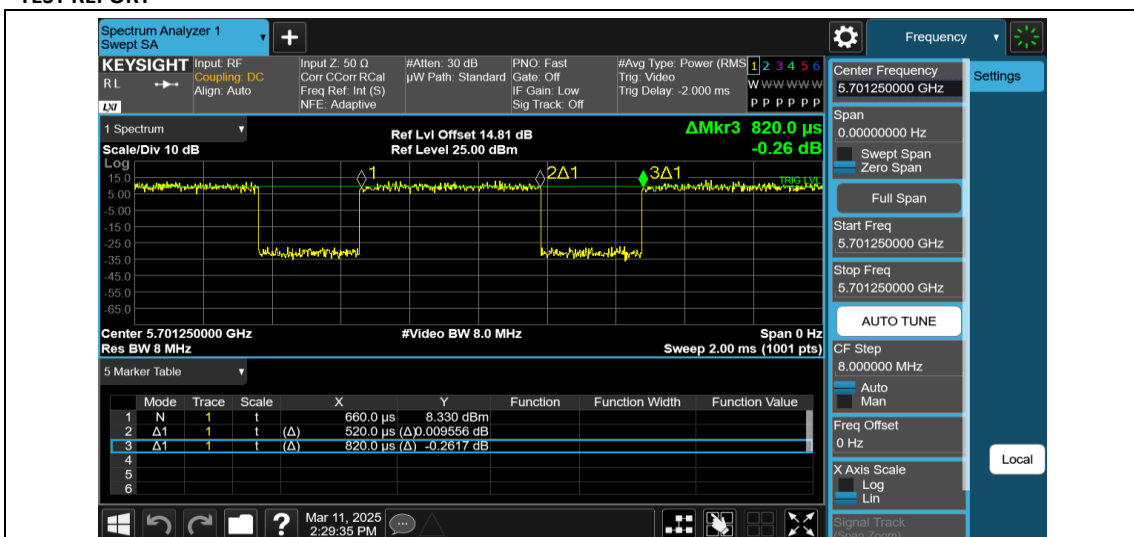
NTNV-11AX20MIMO-Ant1-5700-242Tone-RU61
