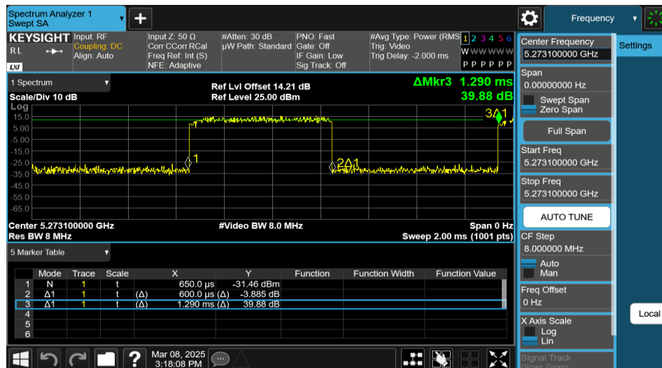
NTNV-11AX20MIMO-Ant2-5280-106Tone-RU53
