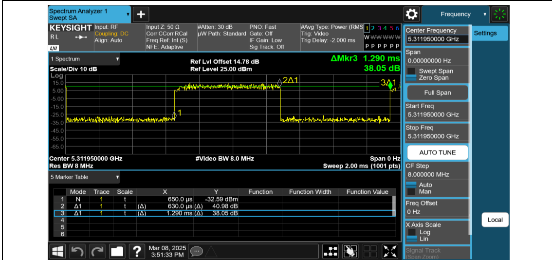
NTNV-11AX20MIMO-Ant1-5320-52Tone-RU37
