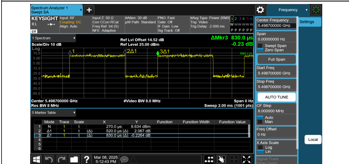
NTVN-11AX20MIMO-Ant1-5500-242Tone-RU61
