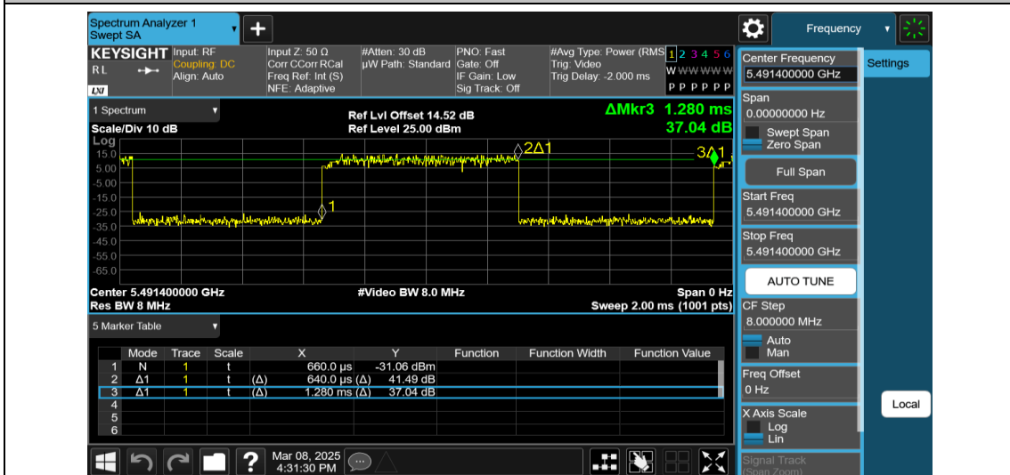
NTNV-11AX20MIMO-Ant1-5500-26Tone-RU0
