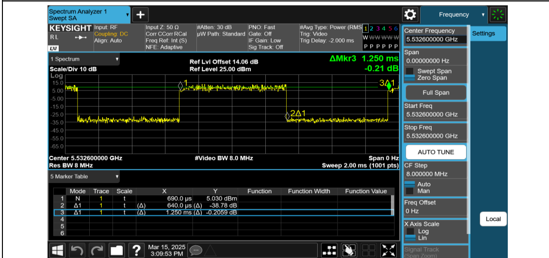
NTNV-11AX40MIMO-Ant2-5550-26Tone-RU0
