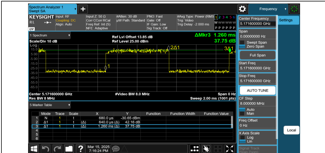
NTNV-11AX80MIMO-Ant2-5210-26Tone-RU0
