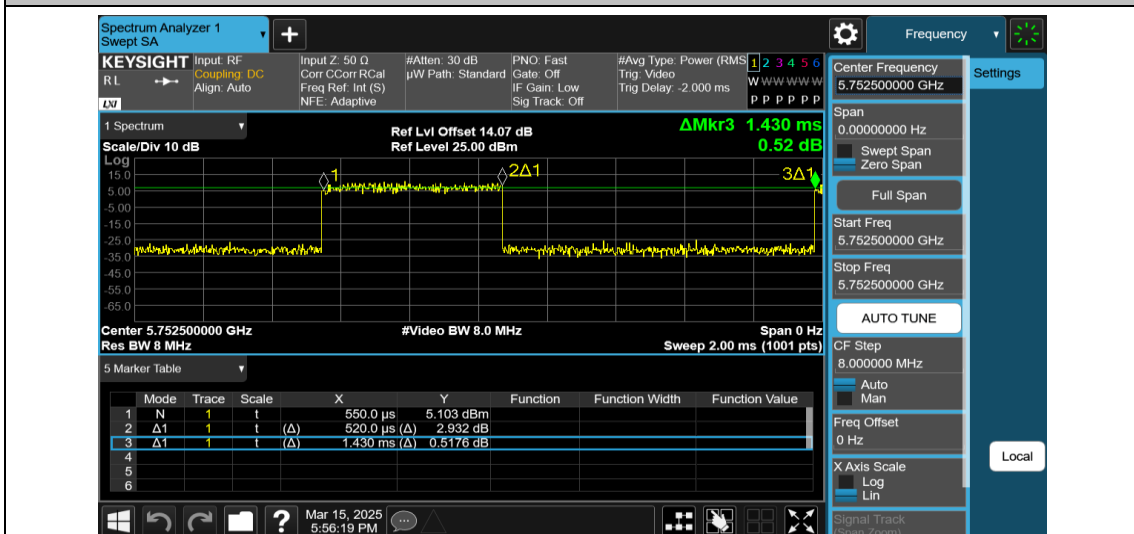
NTVN-11AX40MIMO-Ant2-5755-484Tone-RU65
