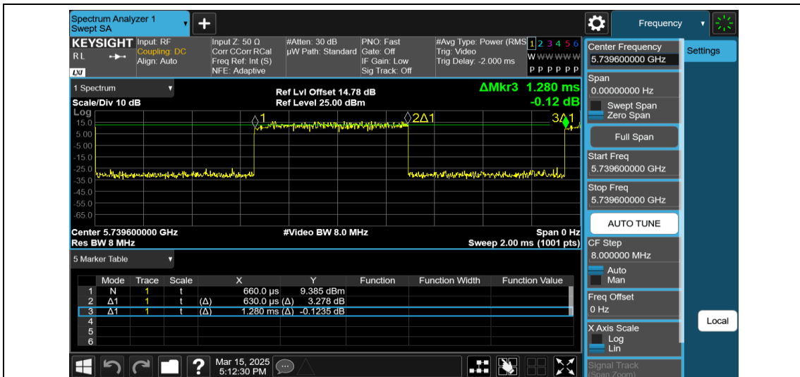
NTNV-11AX40MIMO-Ant1-5755-52Tone-RU37
