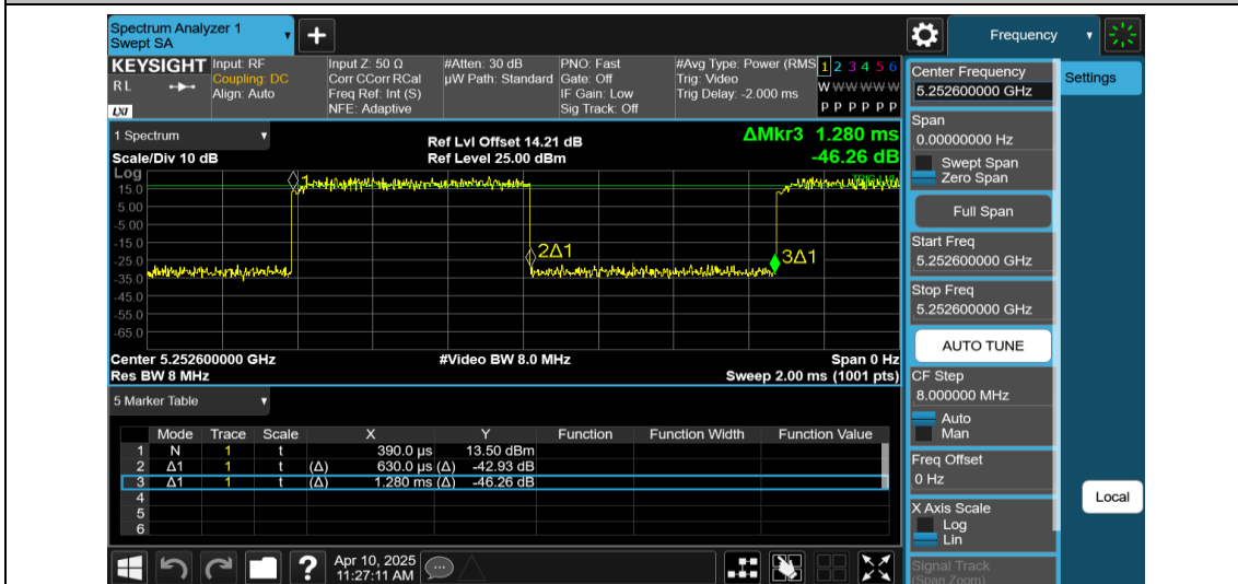
NTNV-11AX80MIMO-Ant2-5290-52Tone-RU37
