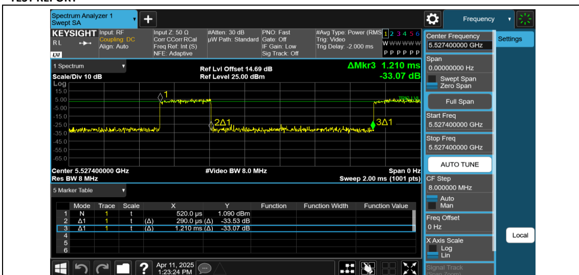
NTNV-11AX80MIMO-Ant1-5530-996Tone-RU67
