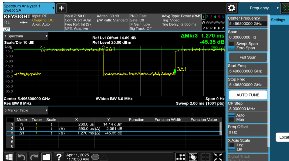
NTNV-11AX80MIMO-Ant1-5530-106Tone-RU53
