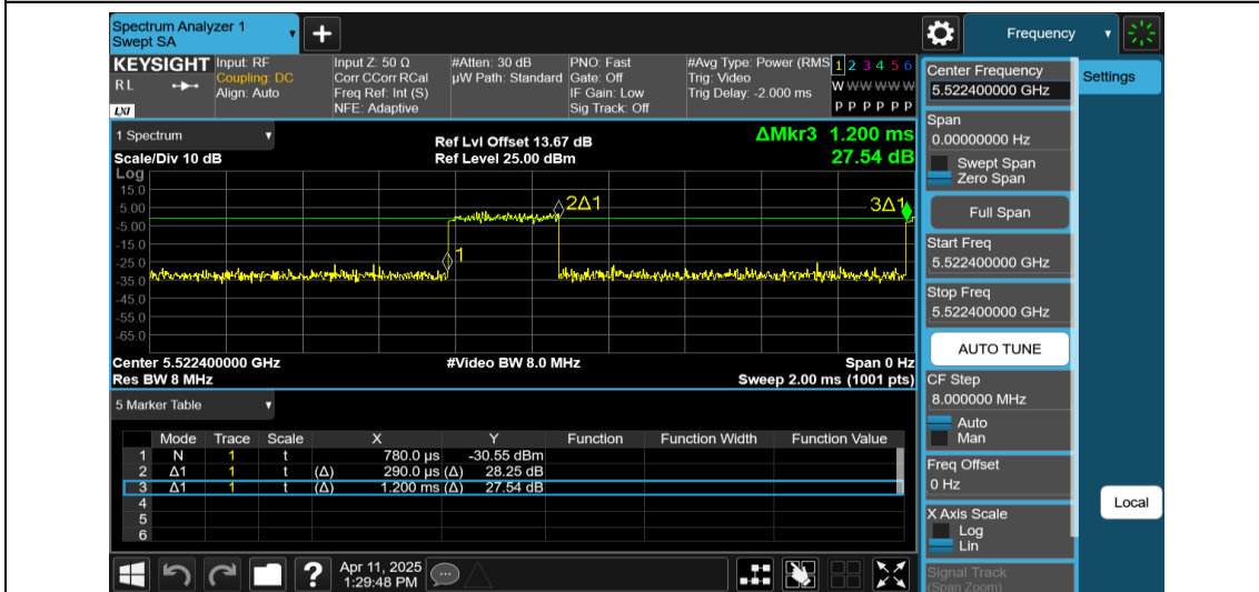
NTNV-11AX80MIMO-Ant2-5530-996Tone-RU67
