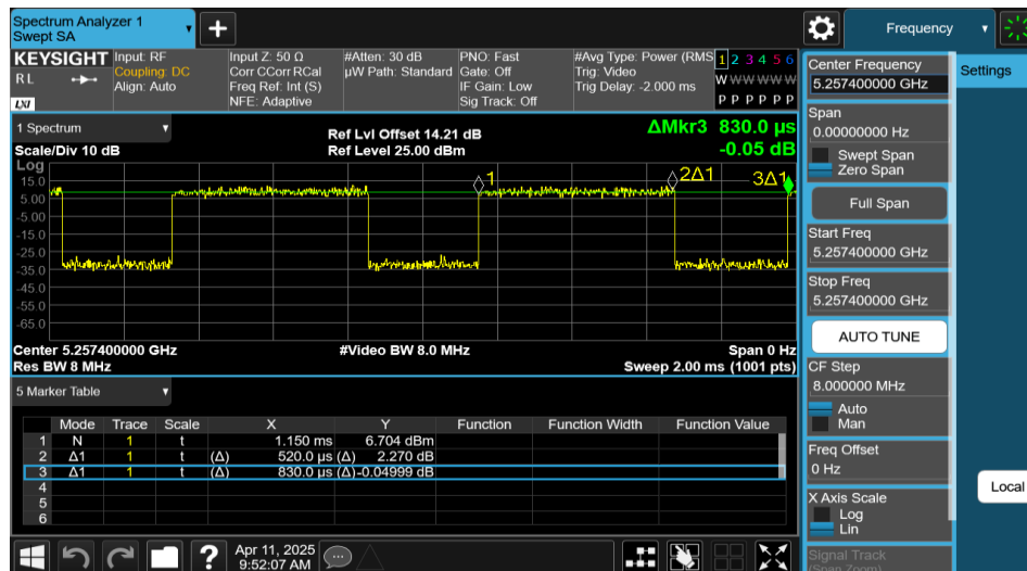
NTNV-11AX80MIMO-Ant2-5290-242Tone-RU61
