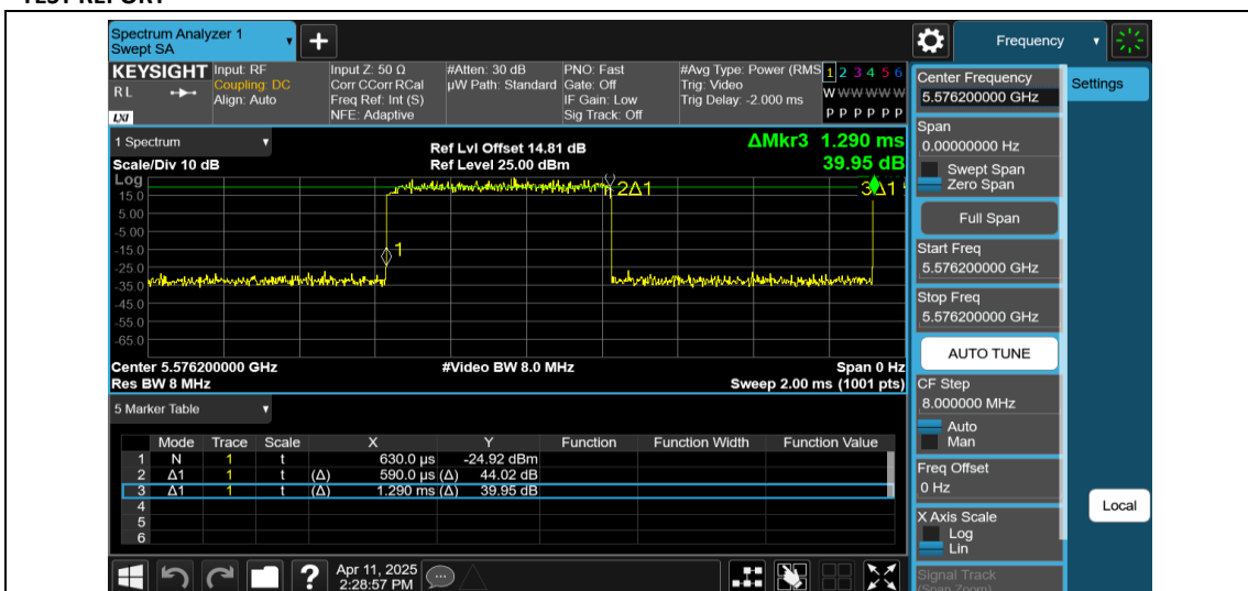
NTNV-11AX80MIMO-Ant1-5610-106Tone-RU53
