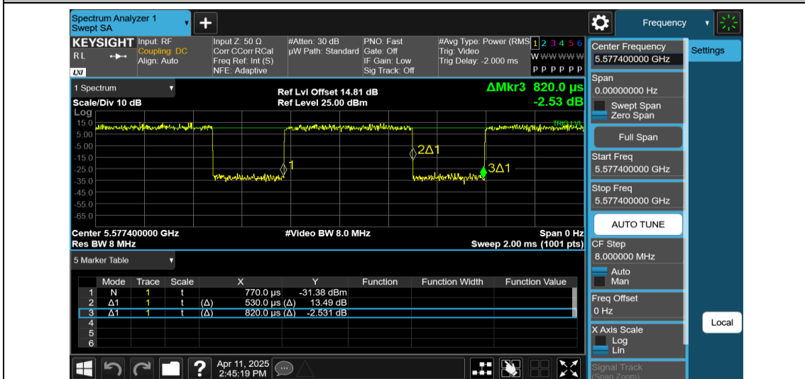
NTNV-11AX80MIMO-Ant1-5610-242Tone-RU61
