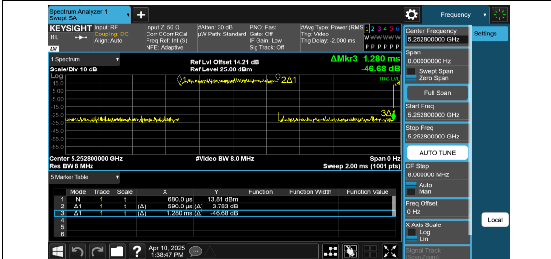
NTVN-11AX80MIMO-Ant2-5290-106Tone-RU53
