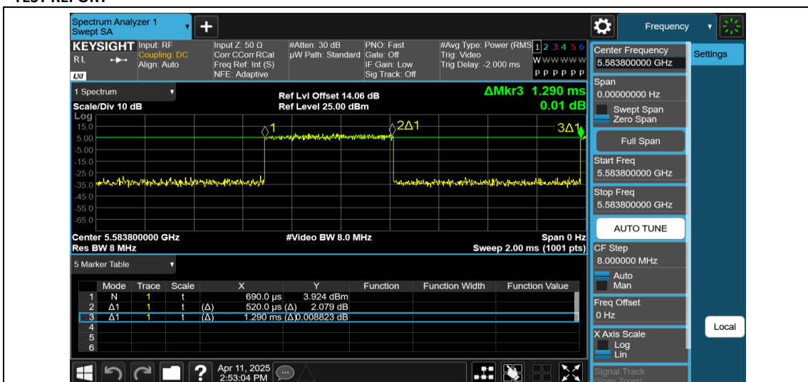
NTNV-11AX80MIMO-Ant2-5610-242Tone-RU61
