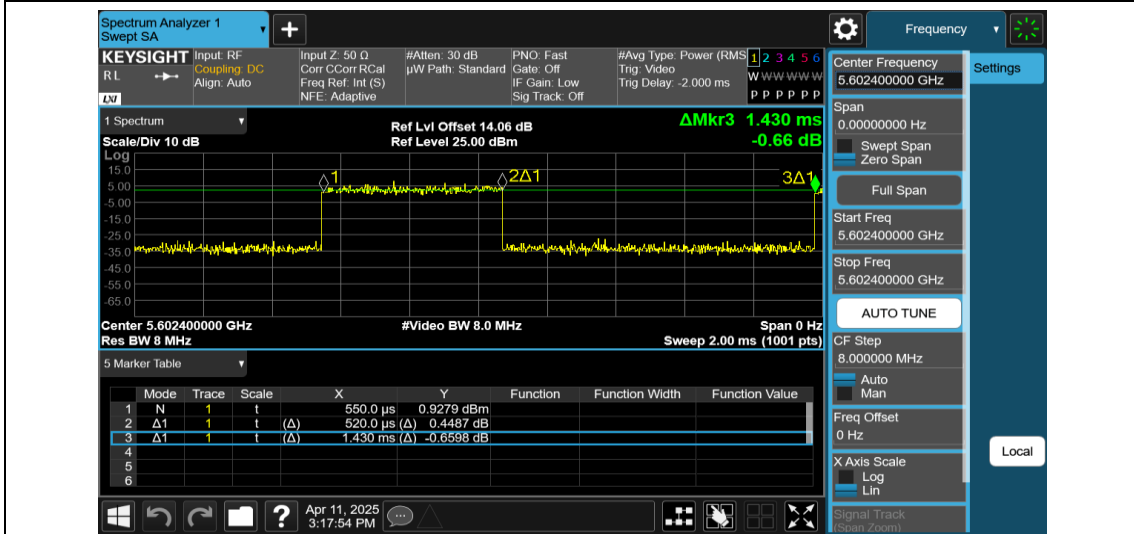
NTNV-11AX80MIMO-Ant2-5610-484Tone-RU65
