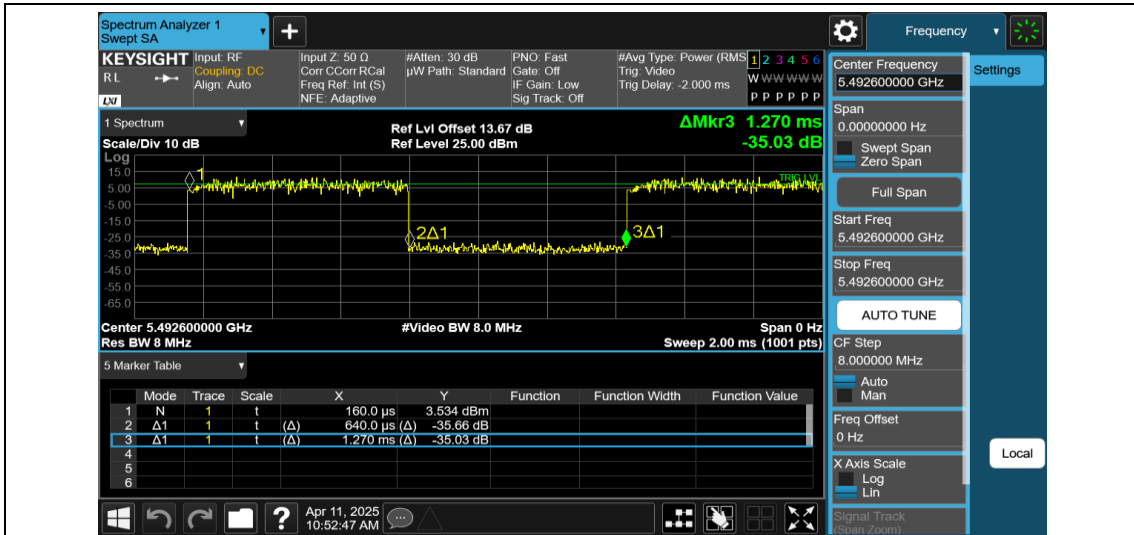
NTNV-11AX80MIMO-Ant2-5530-26Tone-RU0
