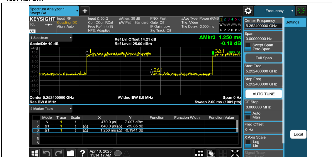
NTNV-11AX80MIMO-Ant2-5290-26Tone-RU0
