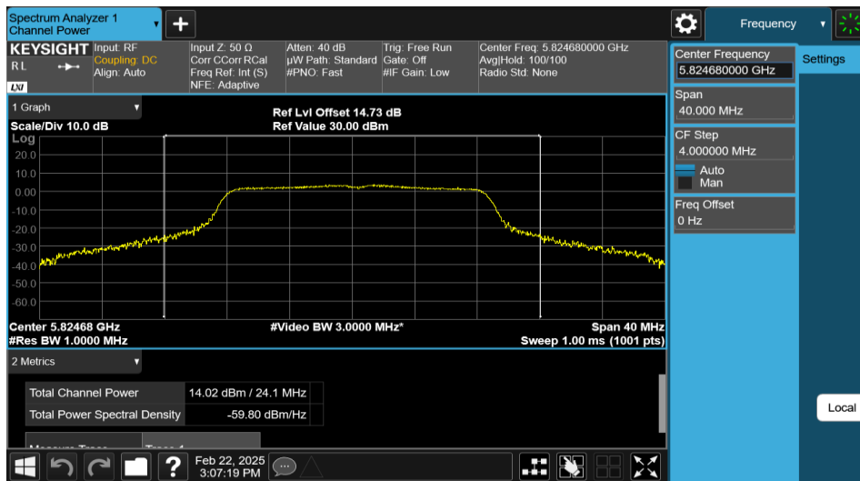
11A-Ant1-5825-PASS
