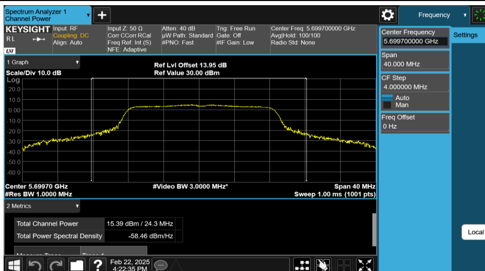
11A-Ant2-5700-PASS
