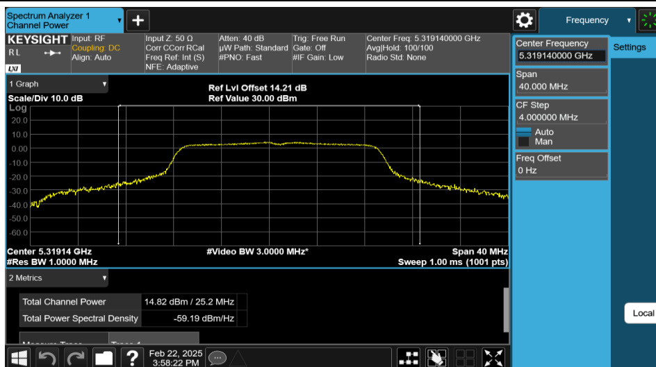
11A-Ant2-5320-PASS
