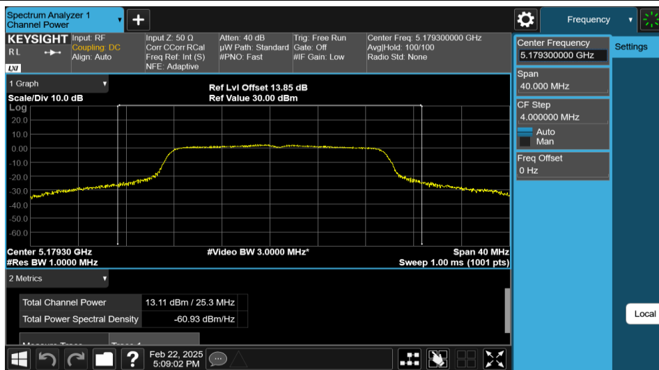
11N20MIMO-Ant2-5180-PASS
