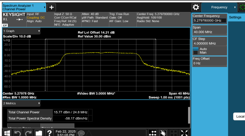
11A-Ant2-5280-PASS
