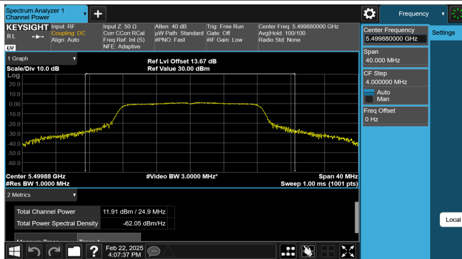
11A-Ant2-5500-PASS
