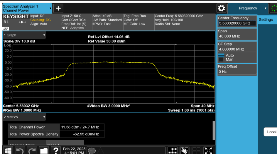
11A-Ant2-5580-PASS
