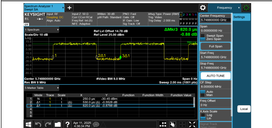
NTNV-11AX80MIMO-Ant1-5775-242Tone-RU61
