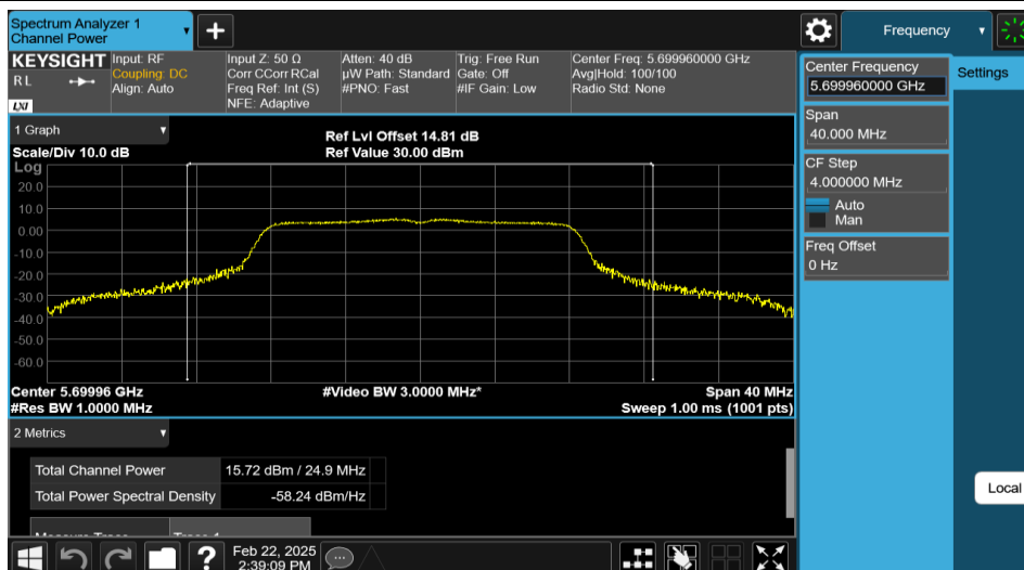
11A-Ant1-5700-PASS
