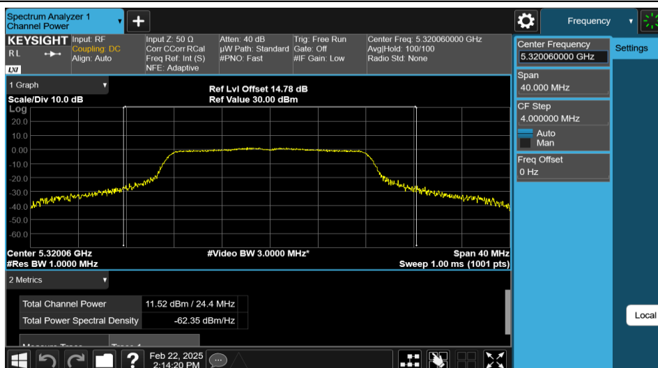
11A-Ant1-5320-PASS
