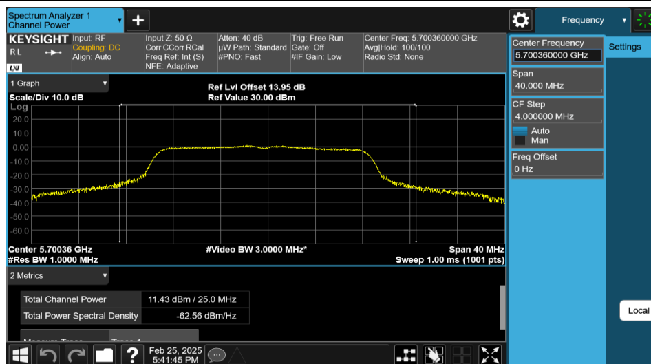
11AC20MIMO-Ant2-5700-PASS
