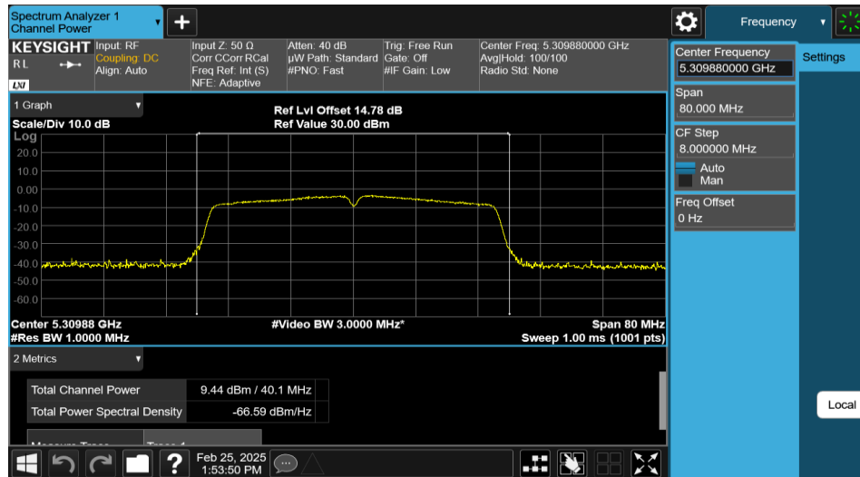
11N40MIMO-Ant1-5310-PASS
