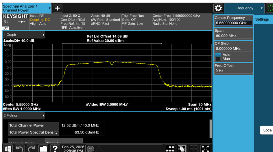
11N40MIMO-Ant1-5550-PASS
