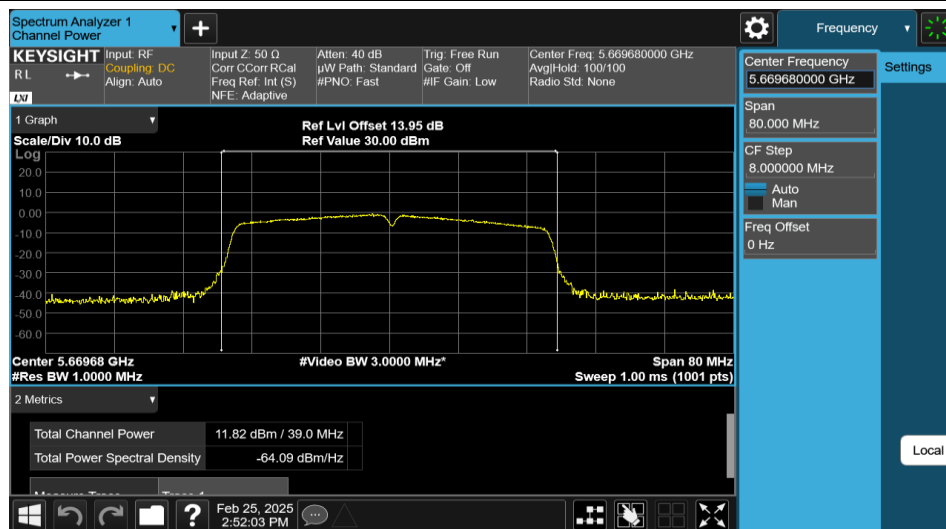
11N40MIMO-Ant2-5670-PASS
