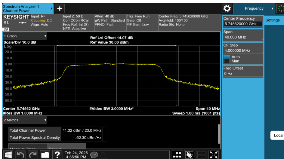
11N20MIMO-Ant2-5745-PASS
