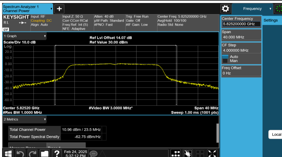
11N20MIMO-Ant2-5825-PASS
