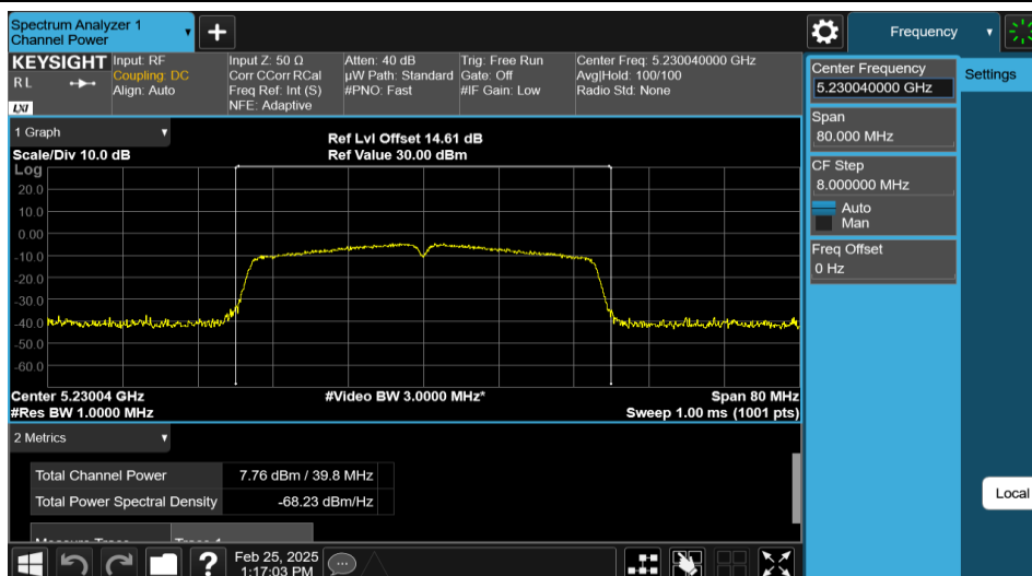
11N40MIMO-Ant1-5230-PASS
