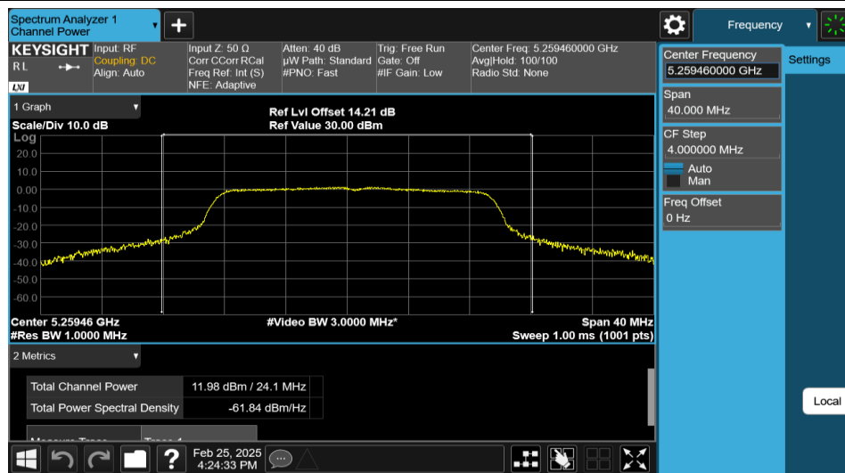
11AC20MIMO-Ant2-5260-PASS
