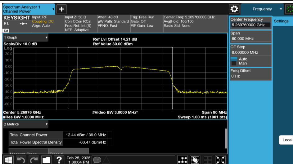
11N40MIMO-Ant2-5270-PASS
