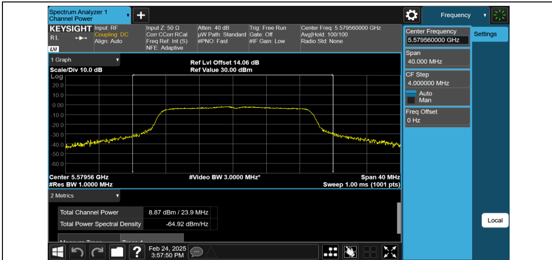
11N20MIMO-Ant2-5580-PASS
