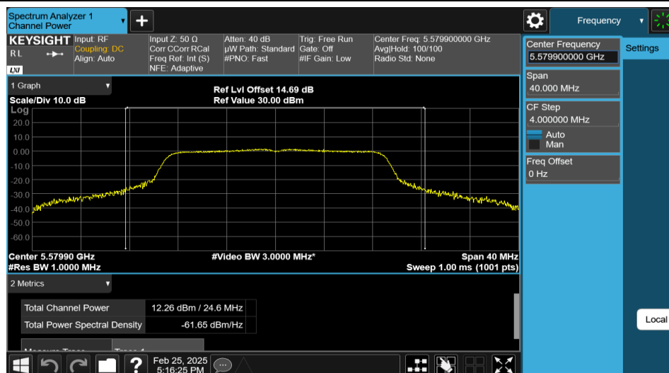
11AC20MIMO-Ant1-5580-PASS
