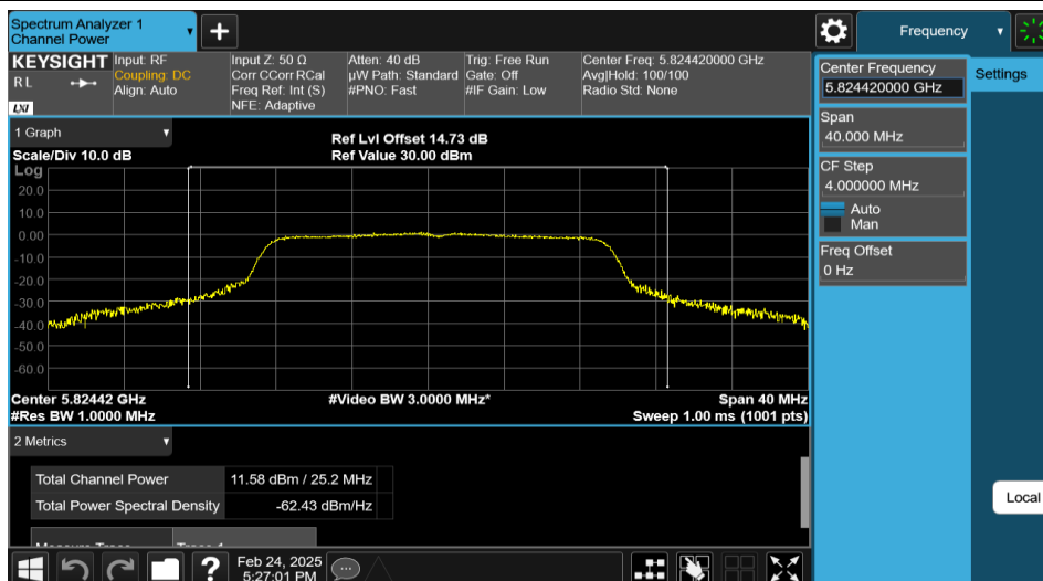
11N20MIMO-Ant1-5825-PASS
