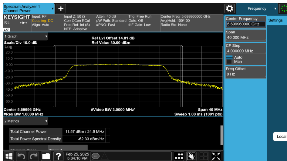
11AC20MIMO-Ant1-5700-PASS
