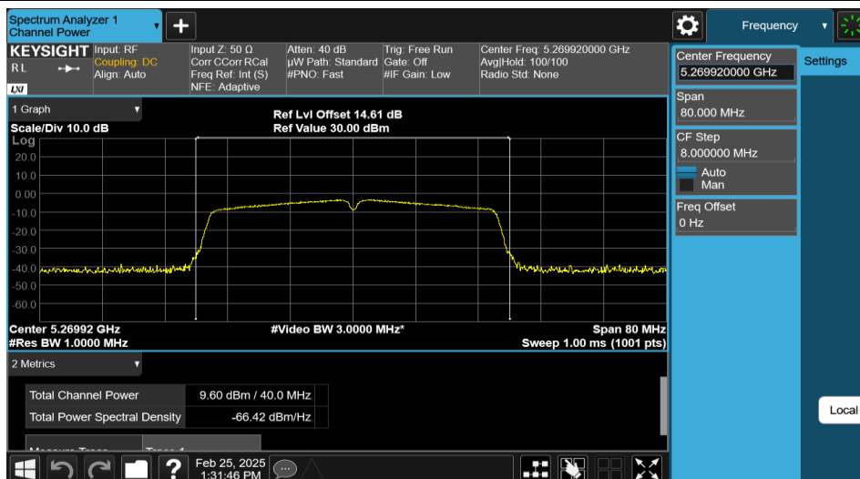
11N40MIMO-Ant1-5270-PASS
