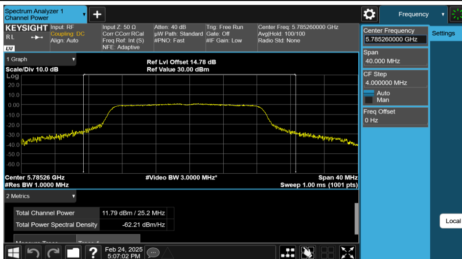
11N20MIMO-Ant1-5785-PASS
