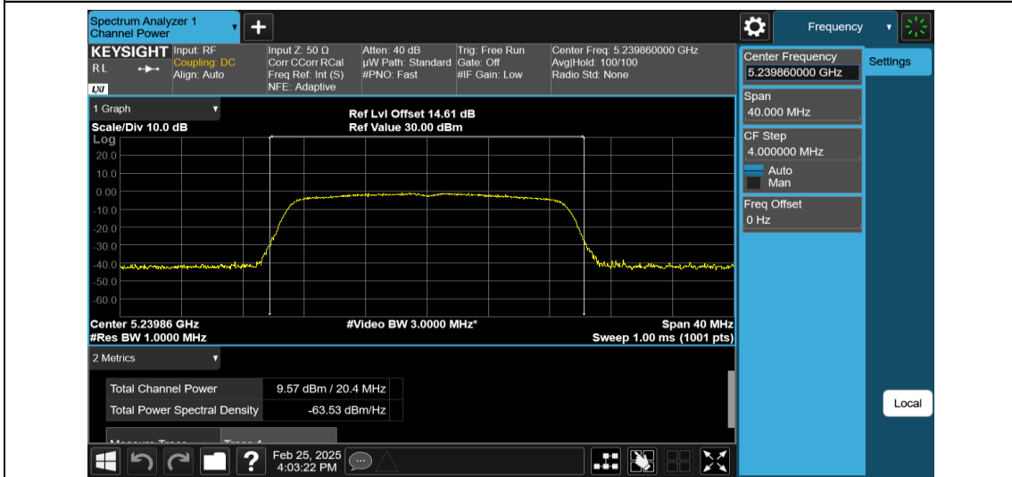
11AC20MIMO-Ant1-5240-PASS
