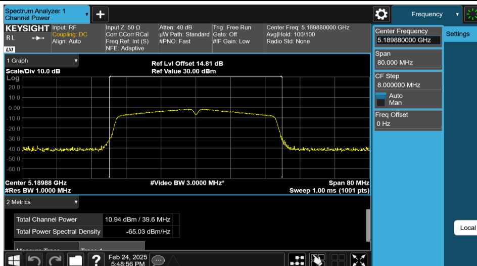
11N40MIMO-Ant1-5190-PASS
