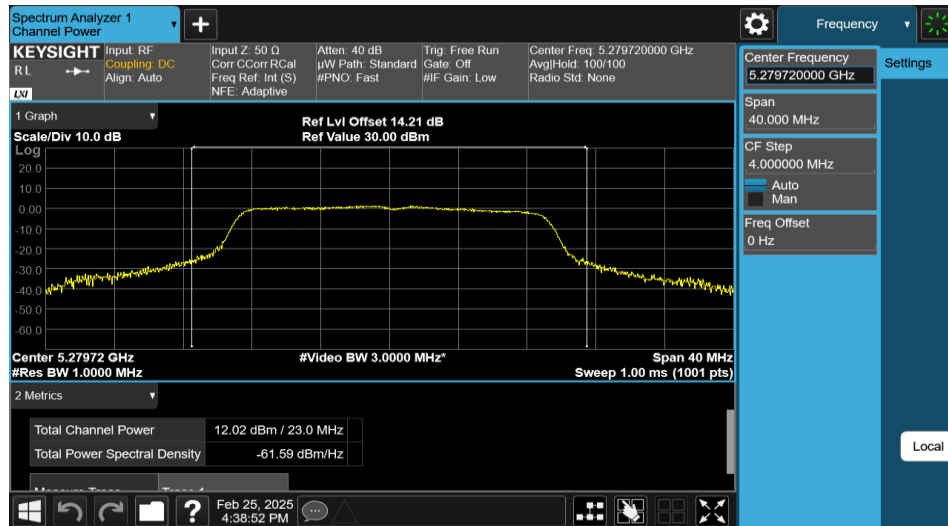
11AC20MIMO-Ant2-5280-PASS
