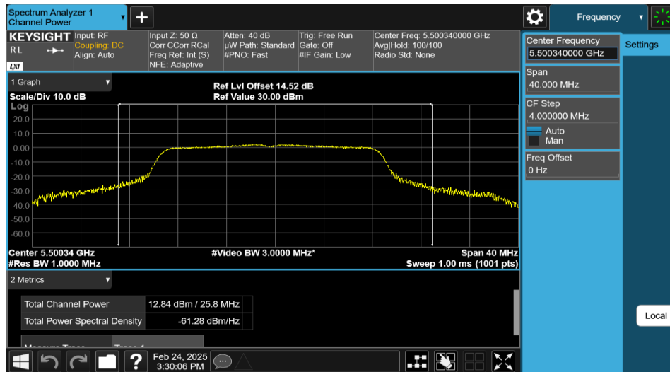
11N20MIMO-Ant1-5500-PASS
