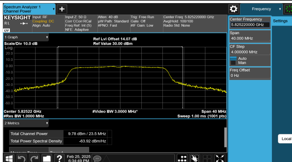
11AC20MIMO-Ant2-5825-PASS
