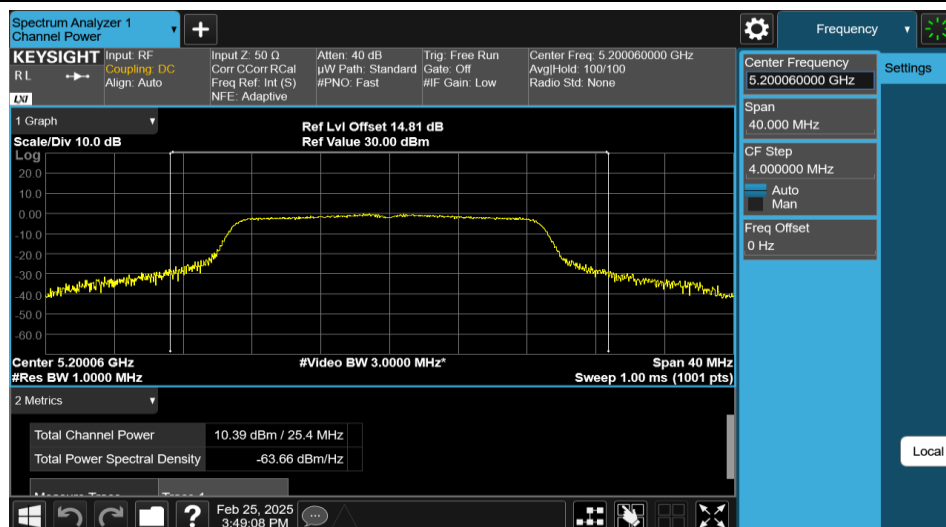
11AC20MIMO-Ant1-5200-PASS
