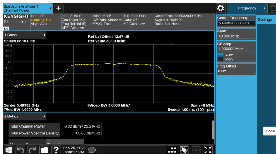
11AC20MIMO-Ant2-5500-PASS
