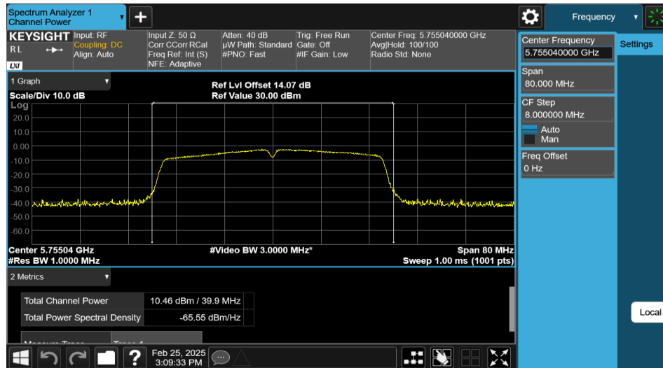
11N40MIMO-Ant2-5755-PASS
