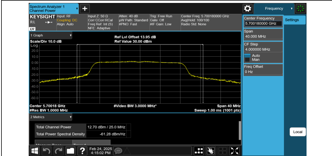
11N20MIMO-Ant2-5700-PASS
