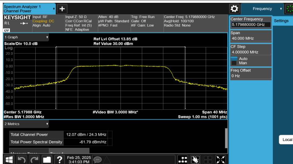
11AC20MIMO-Ant2-5180-PASS
