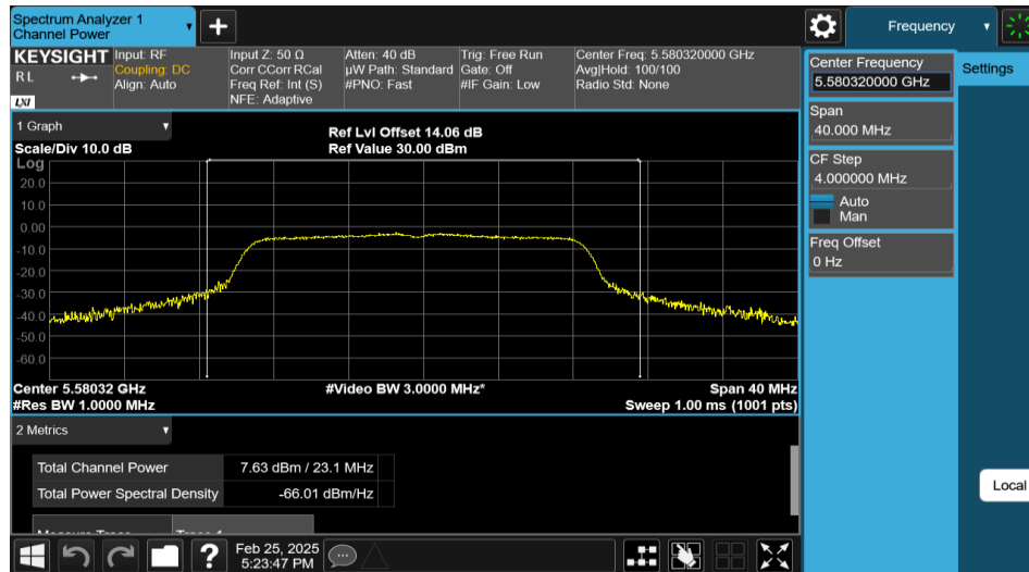
11AC20MIMO-Ant2-5580-PASS
