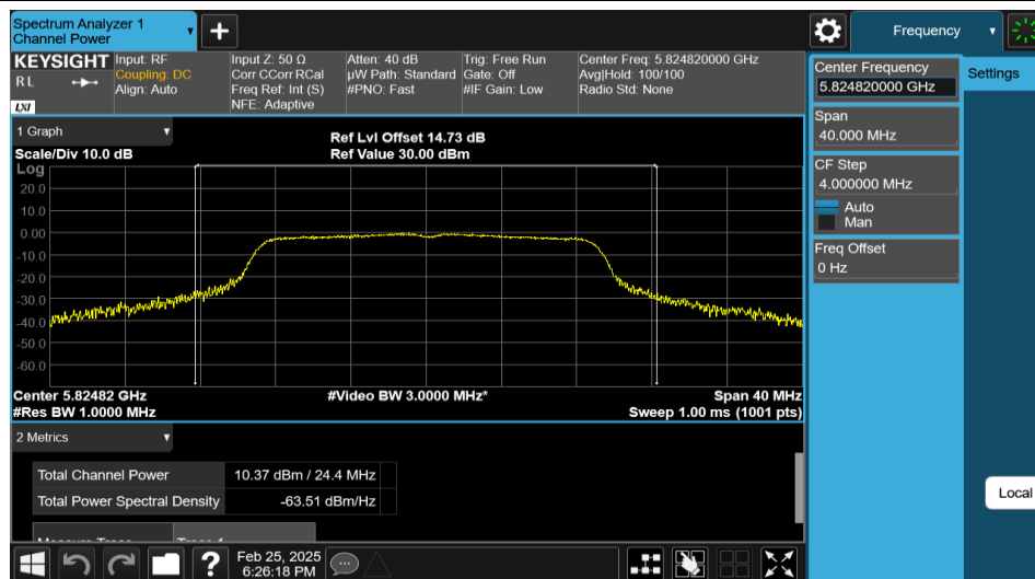
11AC20MIMO-Ant1-5825-PASS
