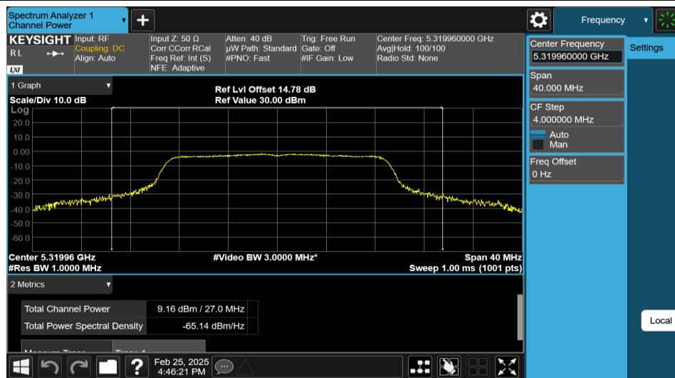
11AC20MIMO-Ant1-5320-PASS
