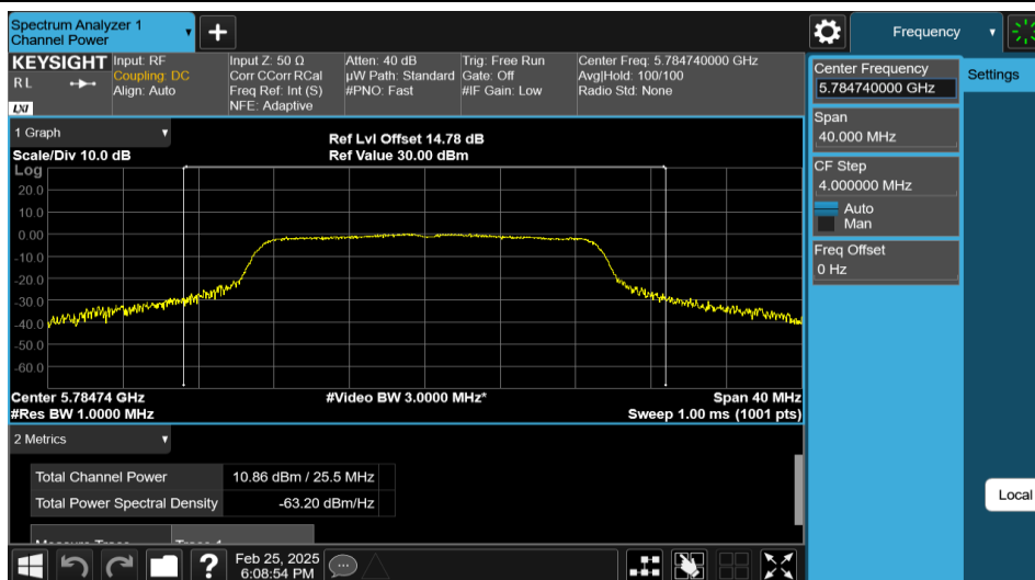
11AC20MIMO-Ant1-5785-PASS
