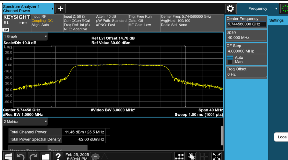
11AC20MIMO-Ant1-5745-PASS
