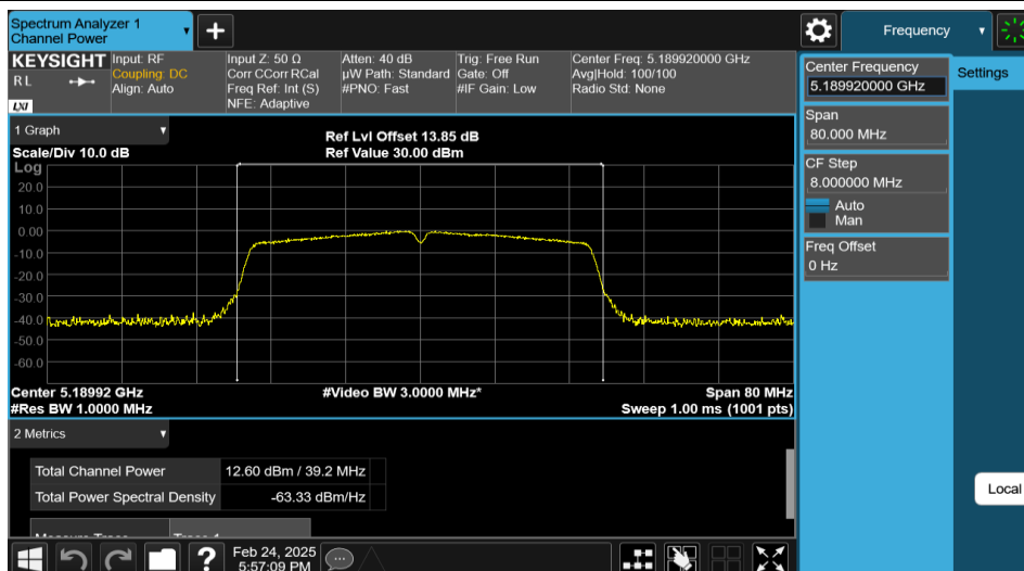
11N40MIMO-Ant2-5190-PASS
