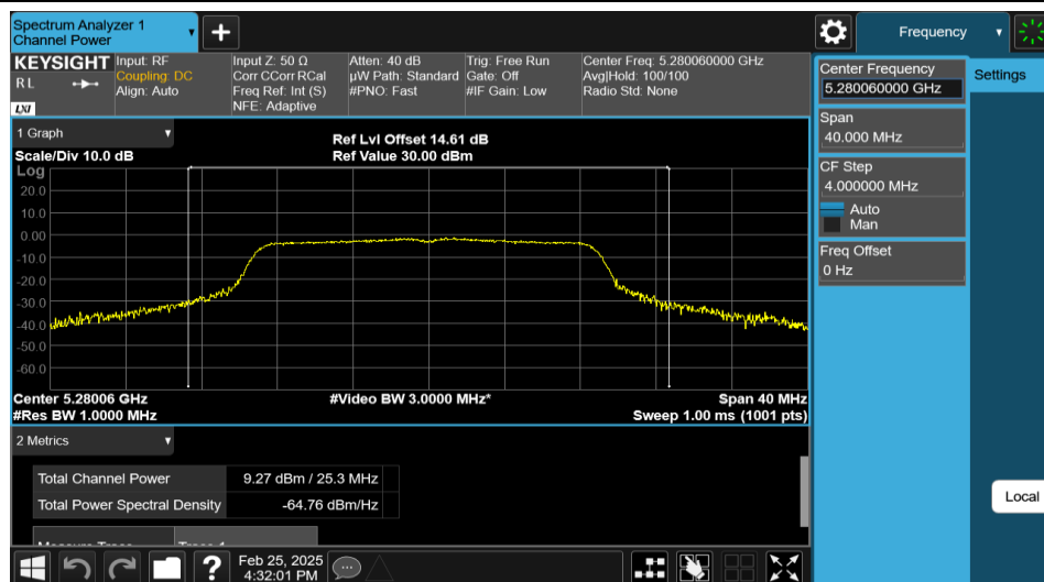
11AC20MIMO-Ant1-5280-PASS
