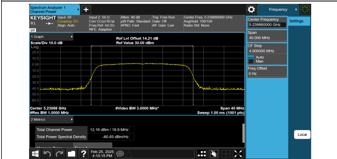
11AC20MIMO-Ant2-5240-PASS
