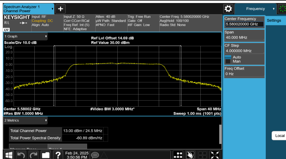
11N20MIMO-Ant1-5580-PASS
