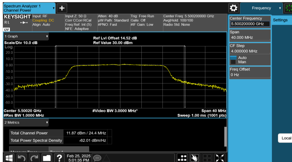
11AC20MIMO-Ant1-5500-PASS
