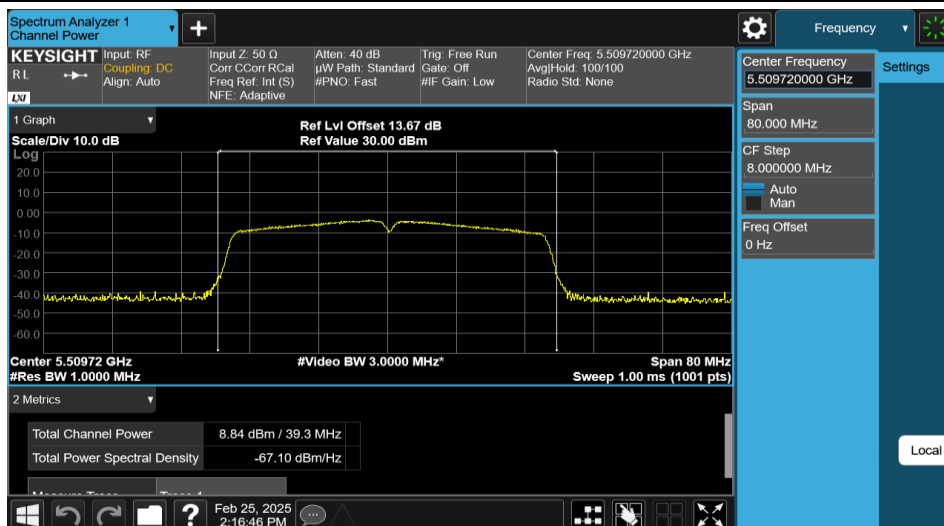
11N40MIMO-Ant2-5510-PASS
