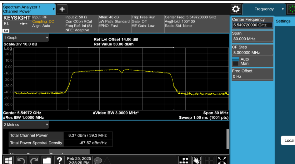
11N40MIMO-Ant2-5550-PASS
