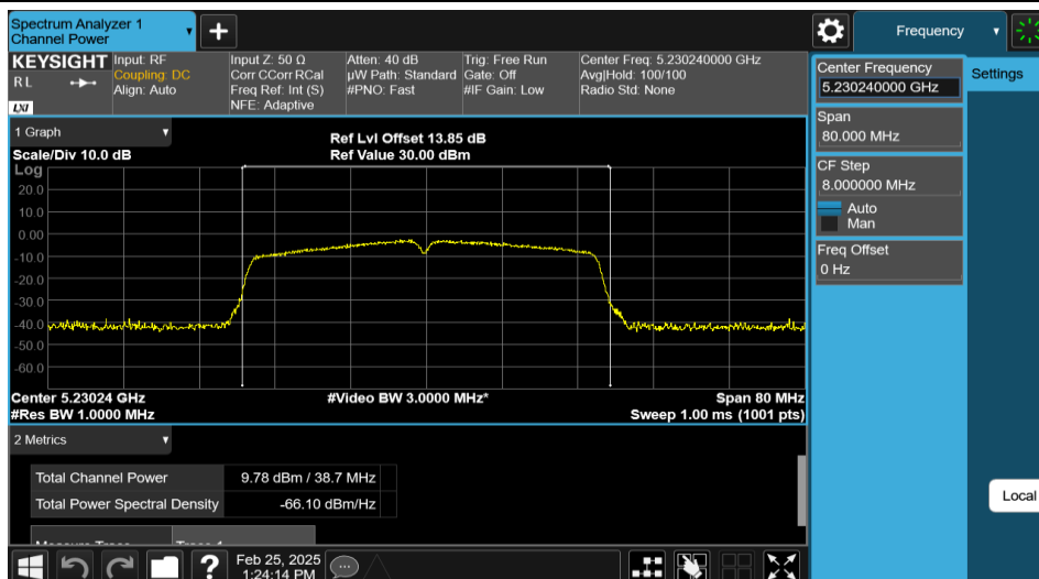
11N40MIMO-Ant2-5230-PASS
