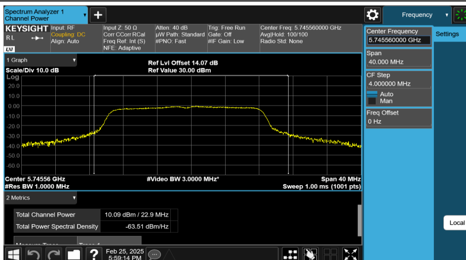
11AC20MIMO-Ant2-5745-PASS
