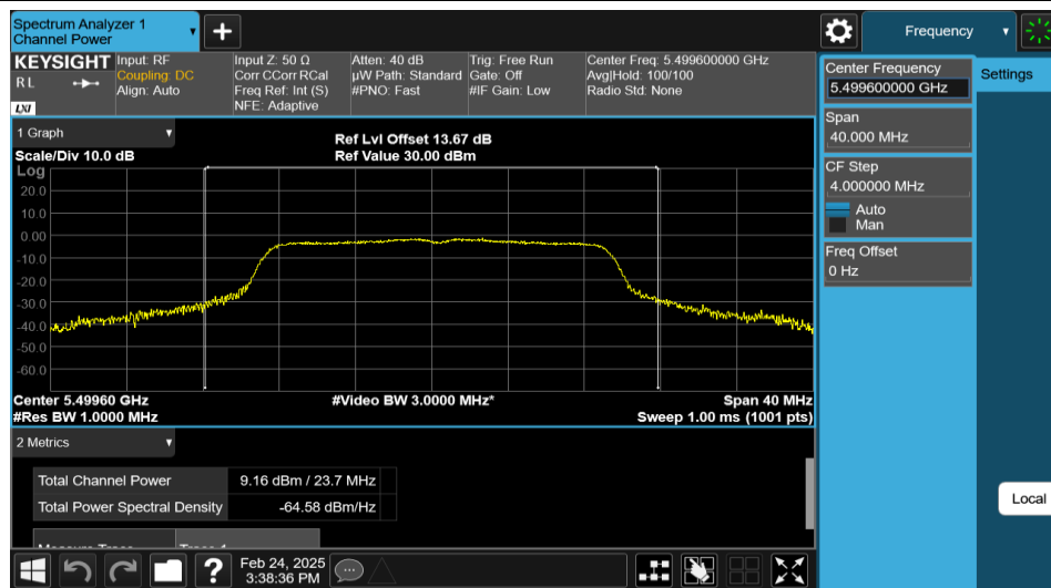
11N20MIMO-Ant2-5500-PASS
