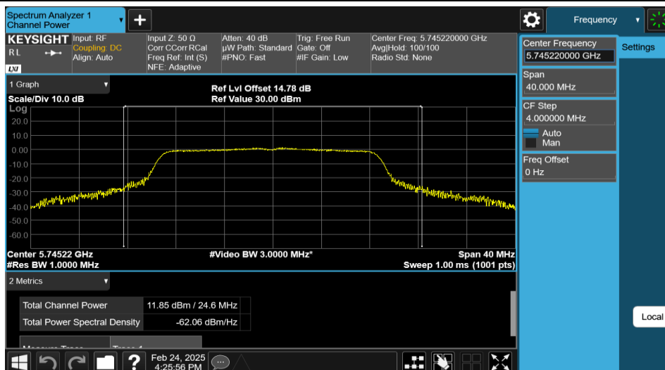
11N20MIMO-Ant1-5745-PASS
