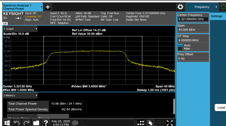
11AC20MIMO-Ant2-5320-PASS
