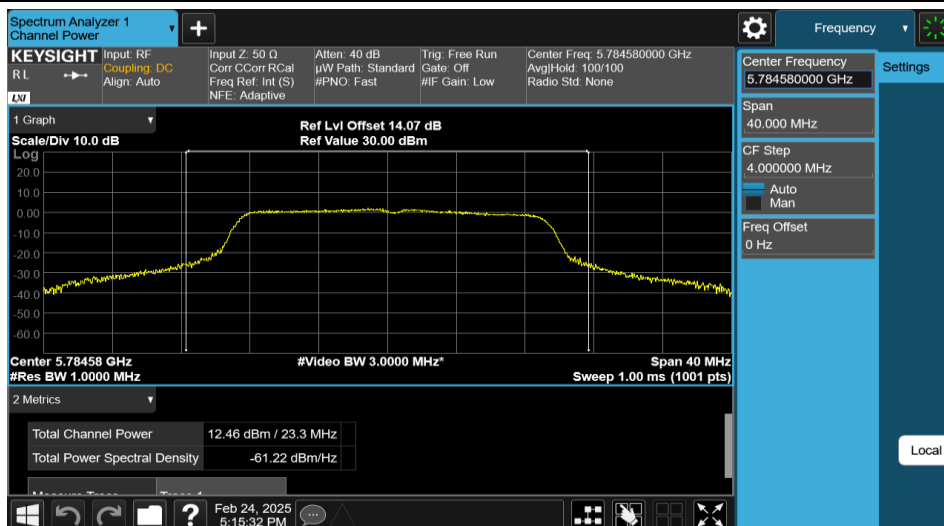
11N20MIMO-Ant2-5785-PASS
