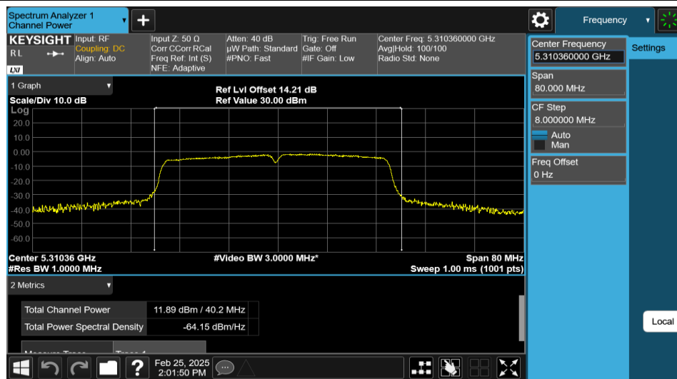
11N40MIMO-Ant2-5310-PASS
