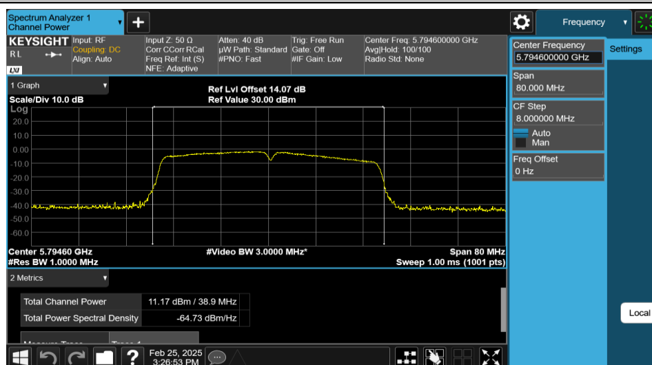
11N40MIMO-Ant2-5795-PASS
