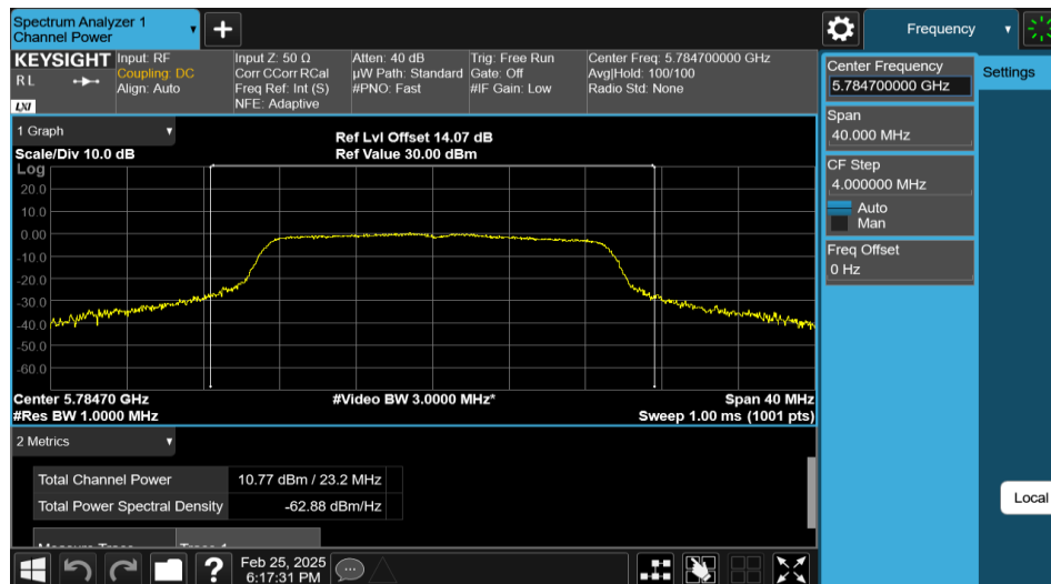
11AC20MIMO-Ant2-5785-PASS
