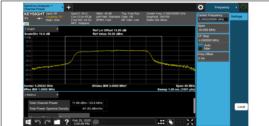
11AC20MIMO-Ant2-5200-PASS
