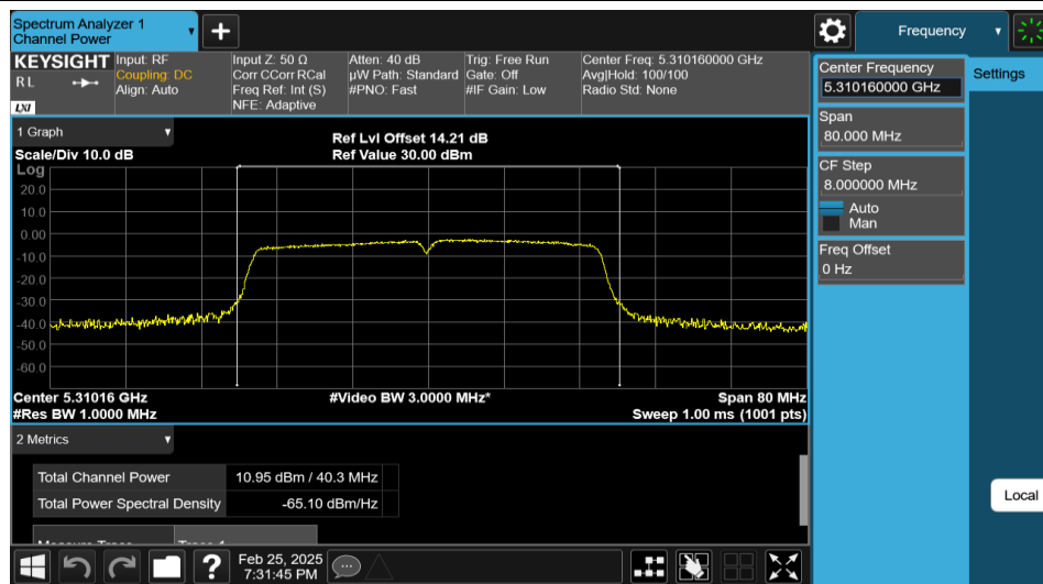
11AC40MIMO-Ant2-5310-PASS
