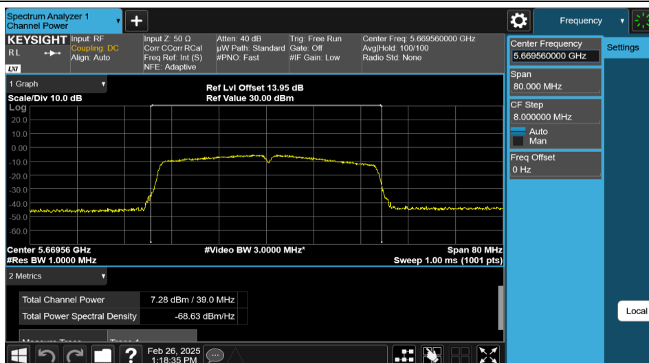
11AC40MIMO-Ant2-5670-PASS
