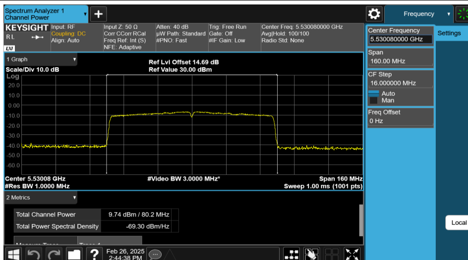
11AC80MIMO-Ant1-5530-PASS
