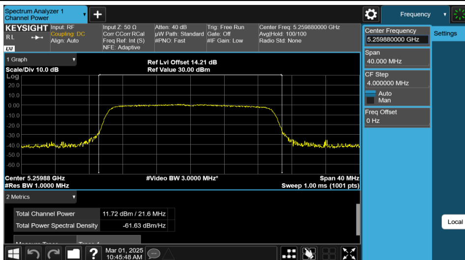
11AX20MIMO-Ant2-5260-PASS
