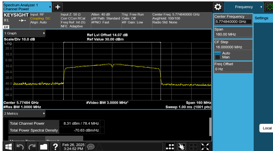
11AC80MIMO-Ant2-5775-PASS
