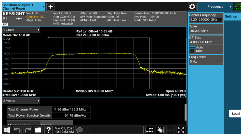
11AX20MIMO-Ant2-5200-PASS
