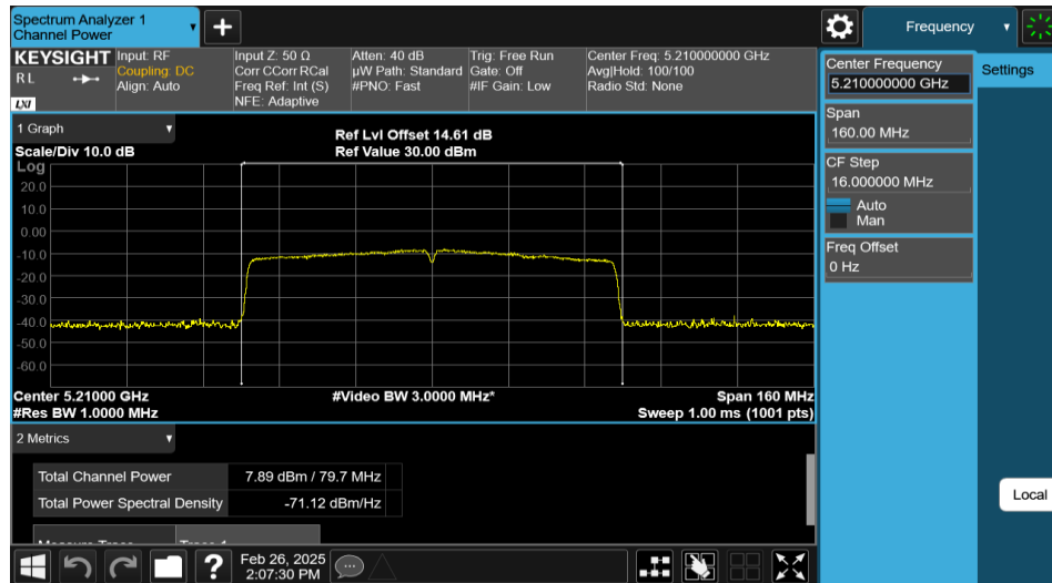
11AC80MIMO-Ant1-5210-PASS
