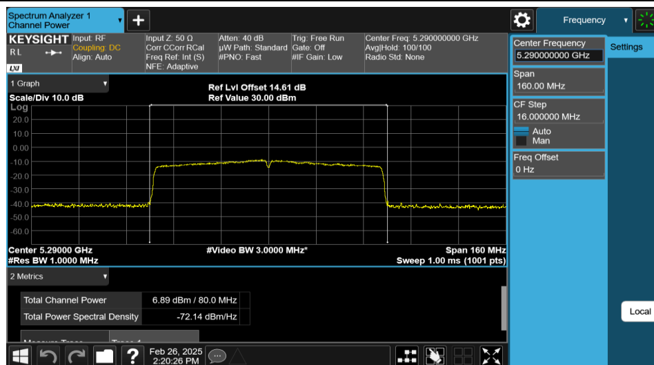
11AC80MIMO-Ant1-5290-PASS
