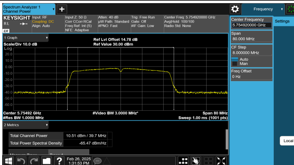
11AC40MIMO-Ant1-5755-PASS
