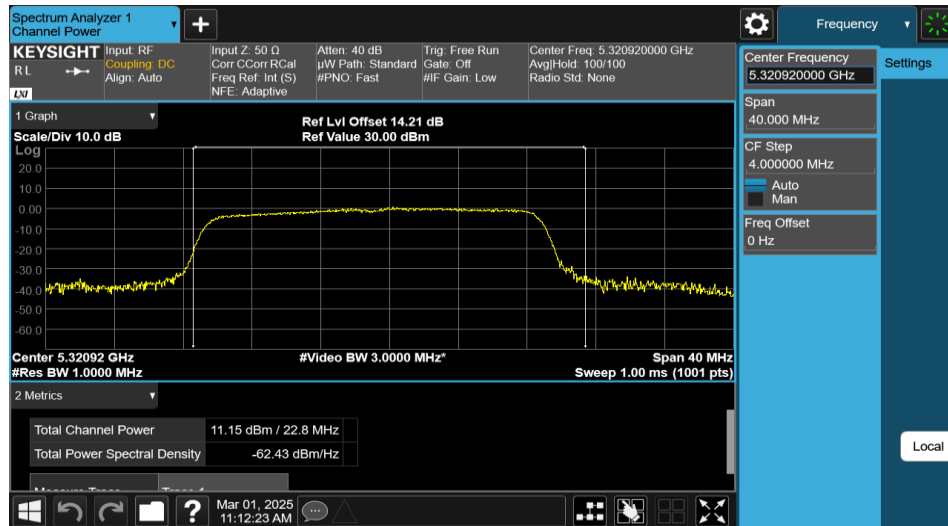
11AX20MIMO-Ant2-5320-PASS
