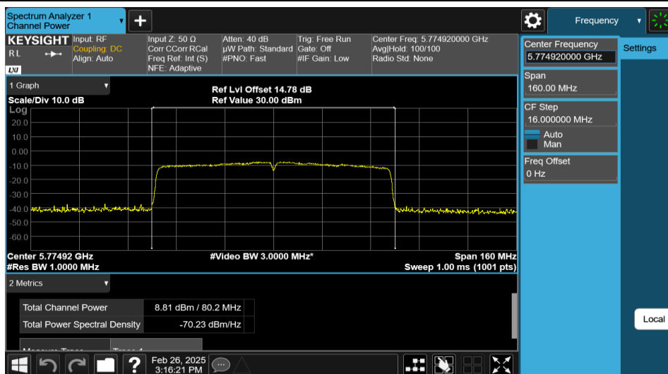
11AC80MIMO-Ant1-5775-PASS
