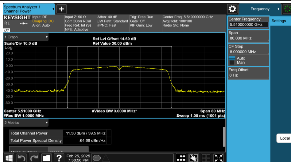
11AC40MIMO-Ant1-5510-PASS
