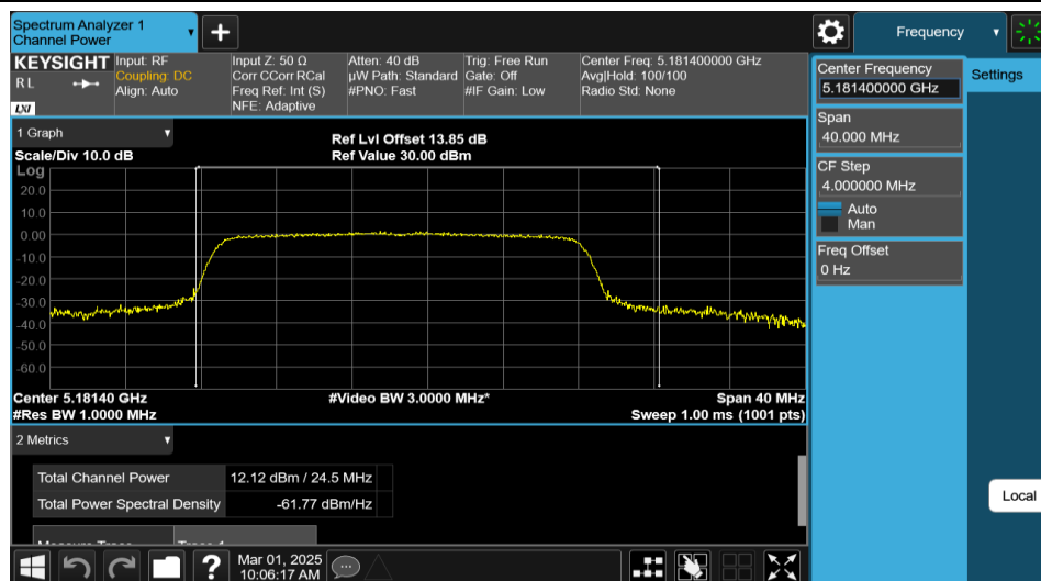
11AX20MIMO-Ant2-5180-PASS
