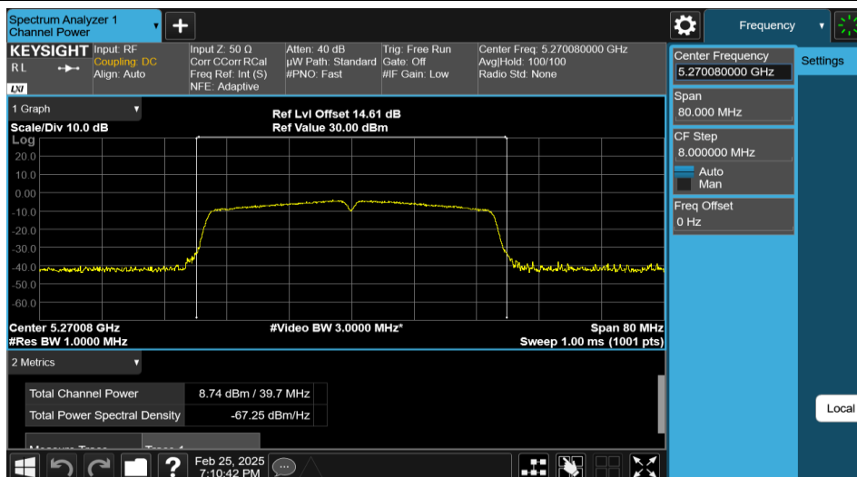
11AC40MIMO-Ant1-5270-PASS
