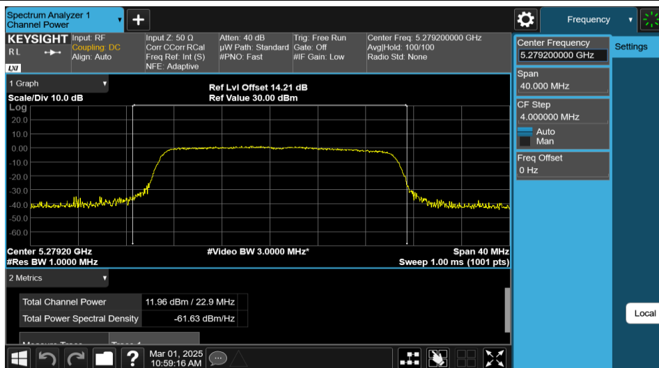
11AX20MIMO-Ant2-5280-PASS
