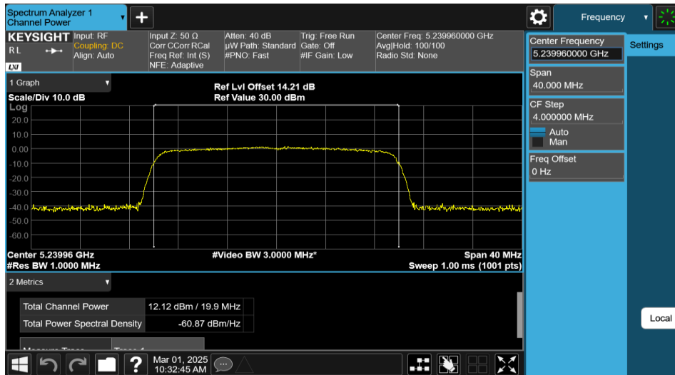
11AX20MIMO-Ant2-5240-PASS
