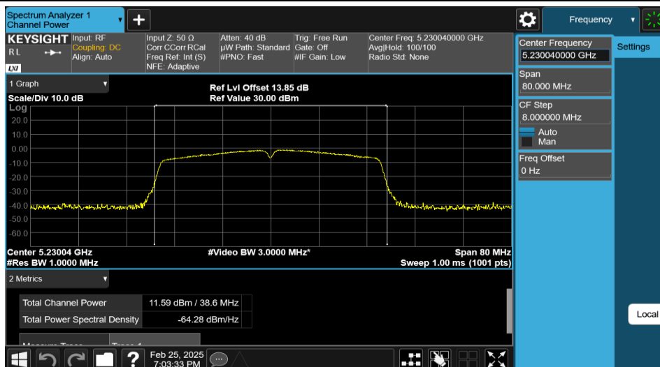
11AC40MIMO-Ant2-5230-PASS
