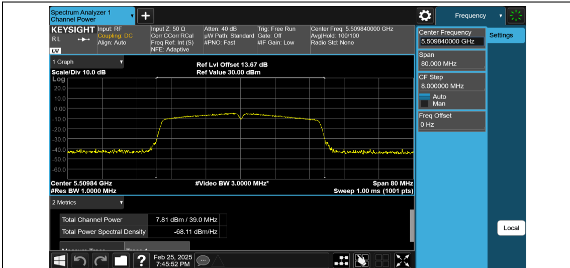
11AC40MIMO-Ant2-5510-PASS
