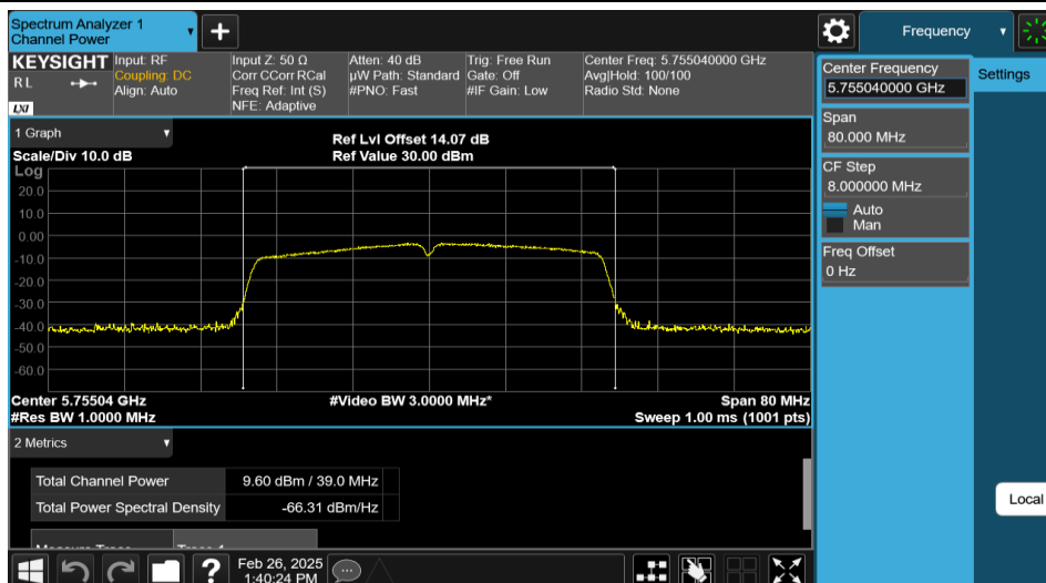
11AC40MIMO-Ant2-5755-PASS
