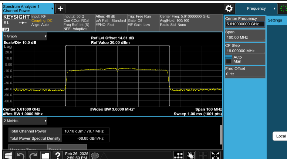
11AC80MIMO-Ant1-5610-PASS
