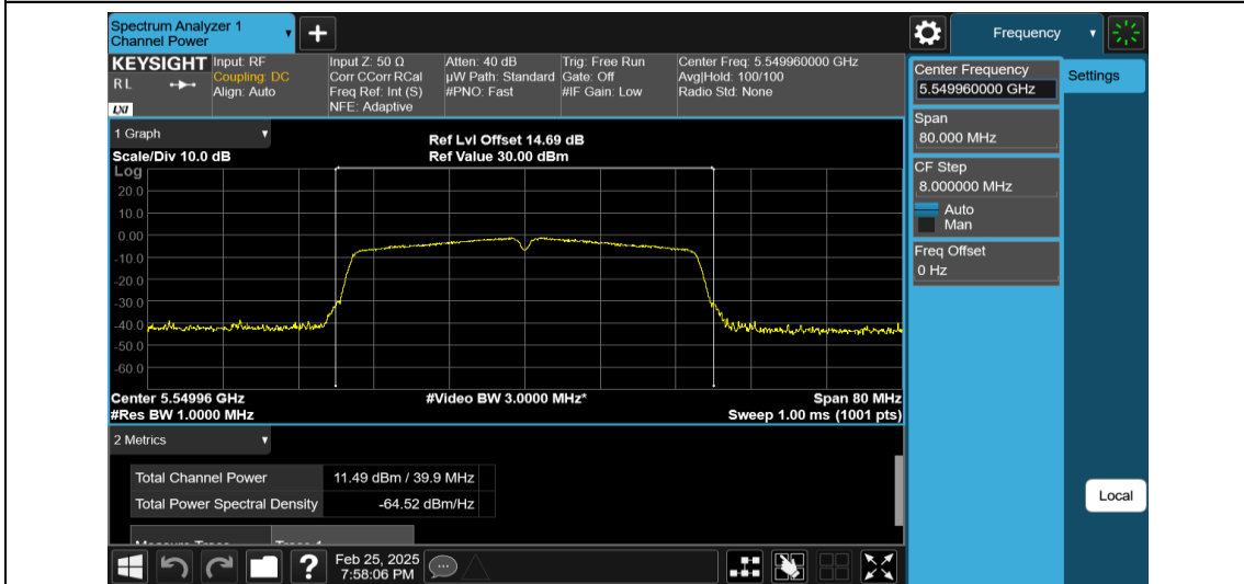
11AC40MIMO-Ant1-5550-PASS
