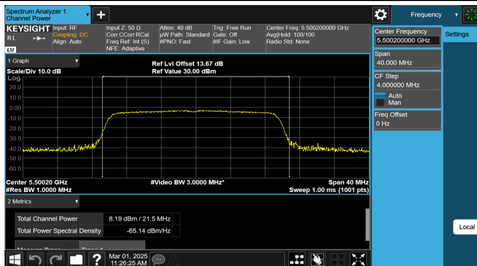
11AX20MIMO-Ant2-5500-PASS
