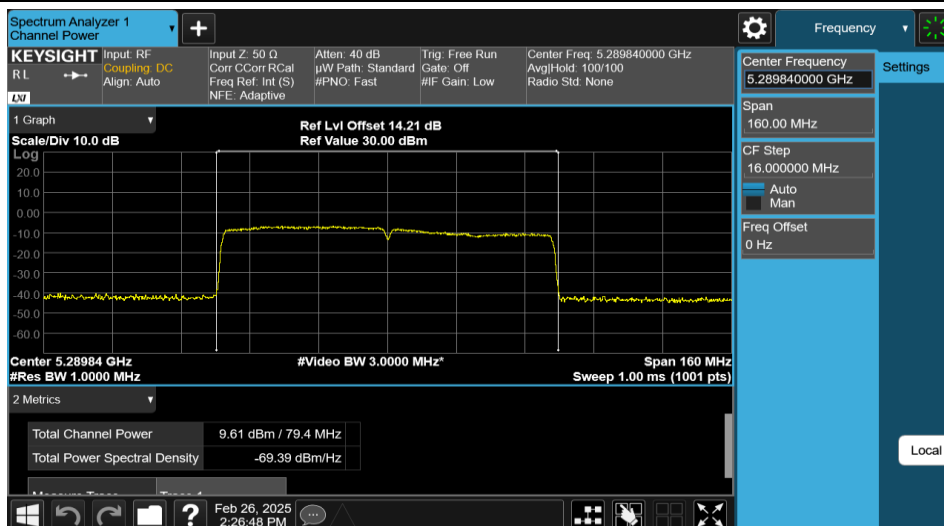
11AC80MIMO-Ant2-5290-PASS
