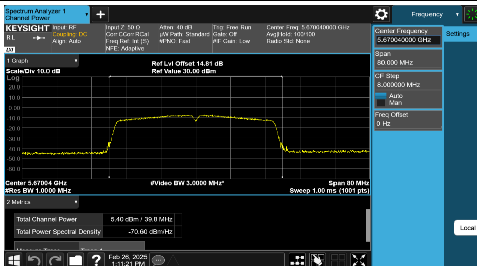
11AC40MIMO-Ant1-5670-PASS
