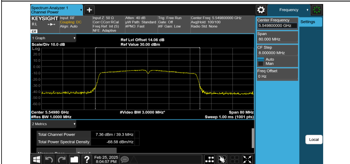
11AC40MIMO-Ant2-5550-PASS
