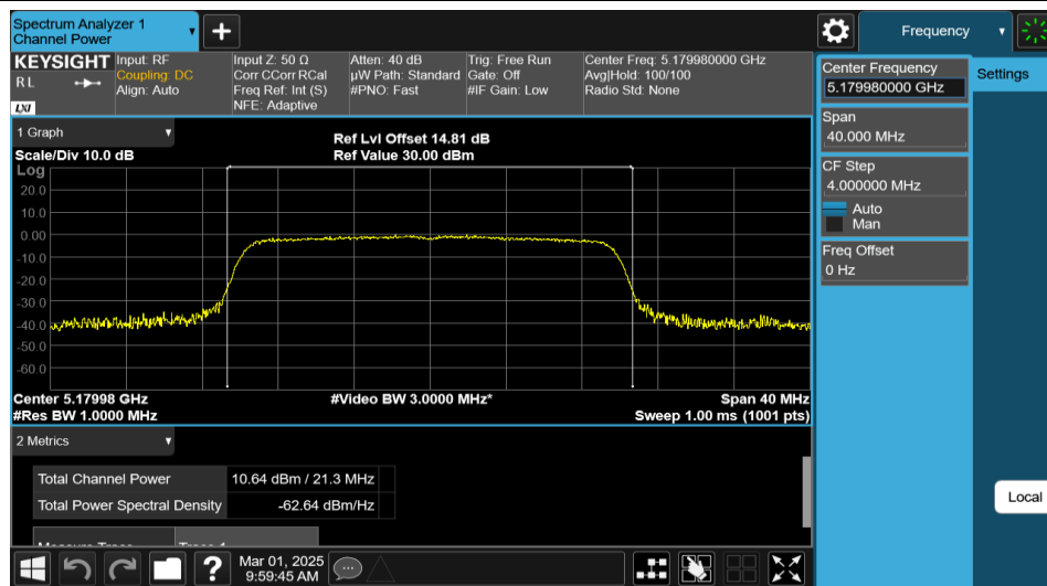
11AX20MIMO-Ant1-5180-PASS
