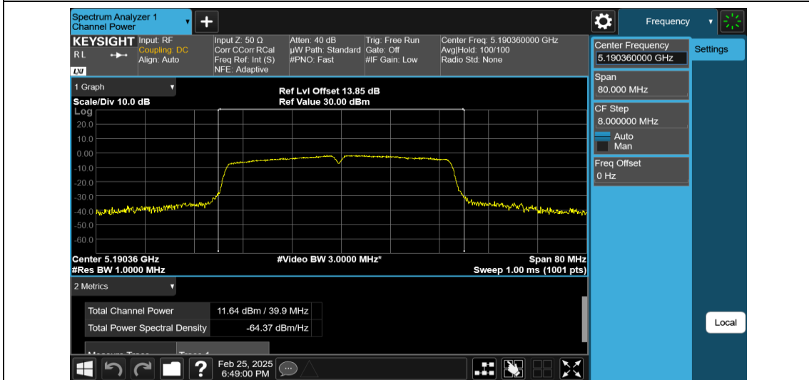
11AC40MIMO-Ant2-5190-PASS
