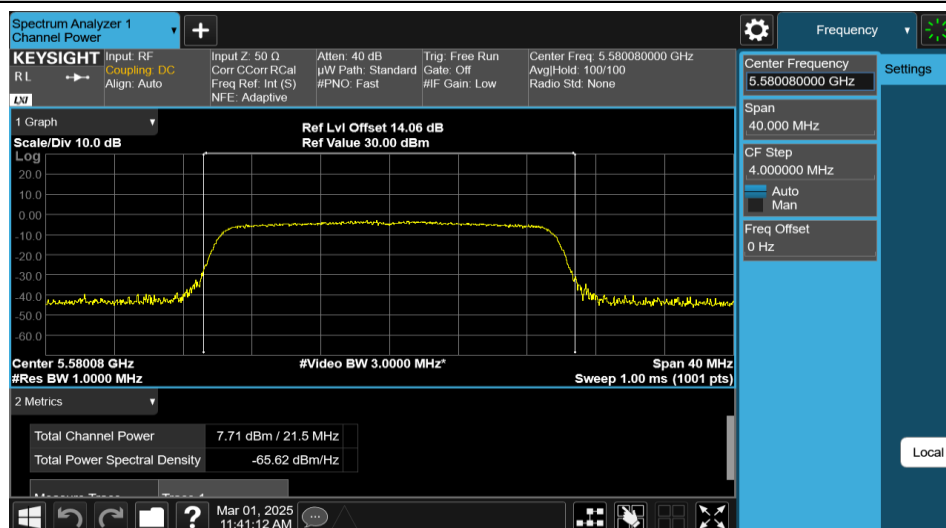
11AX20MIMO-Ant2-5580-PASS
