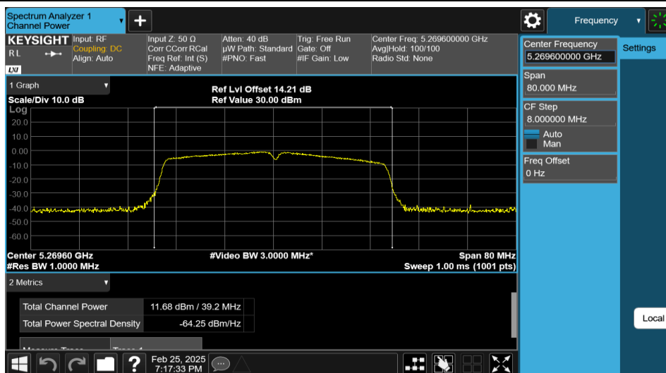
11AC40MIMO-Ant2-5270-PASS
