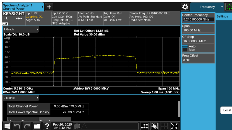
11AC80MIMO-Ant2-5210-PASS
