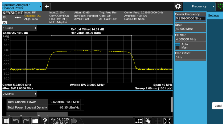
11AX20MIMO-Ant1-5240-PASS
