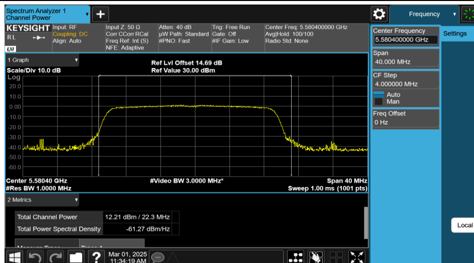
11AX20MIMO-Ant1-5580-PASS
