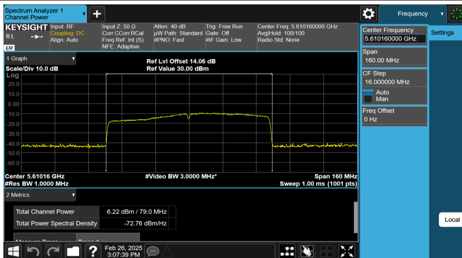
11AC80MIMO-Ant2-5610-PASS
