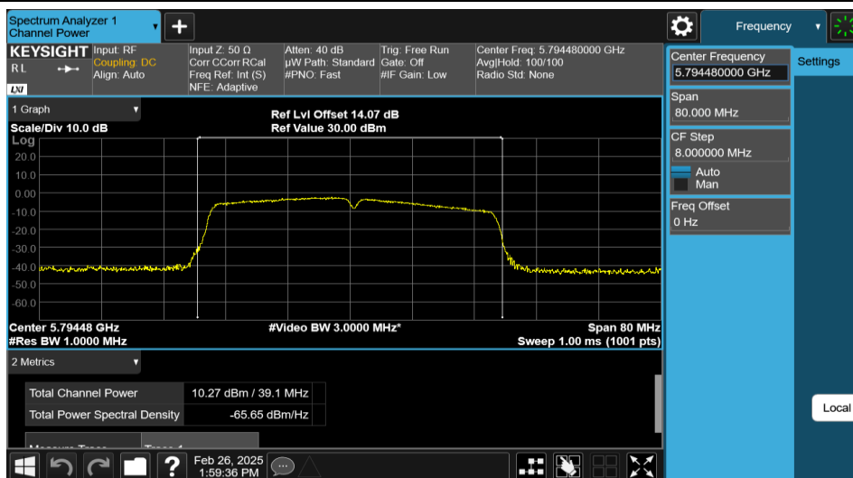
11AC40MIMO-Ant2-5795-PASS
