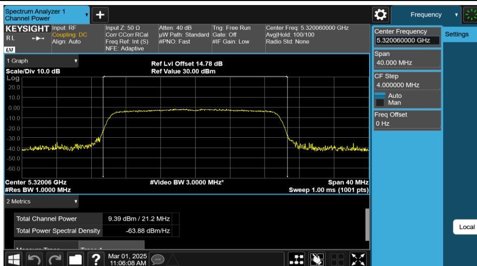
11AX20MIMO-Ant1-5320-PASS
