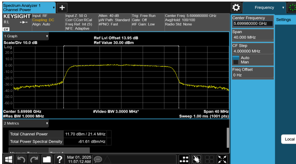
11AX20MIMO-Ant2-5700-PASS
