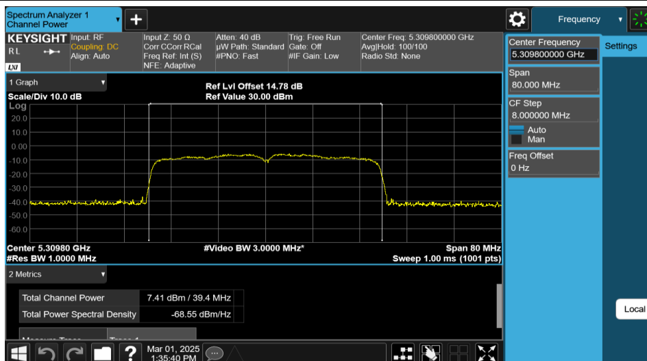
11AX40MIMO-Ant1-5310-PASS
