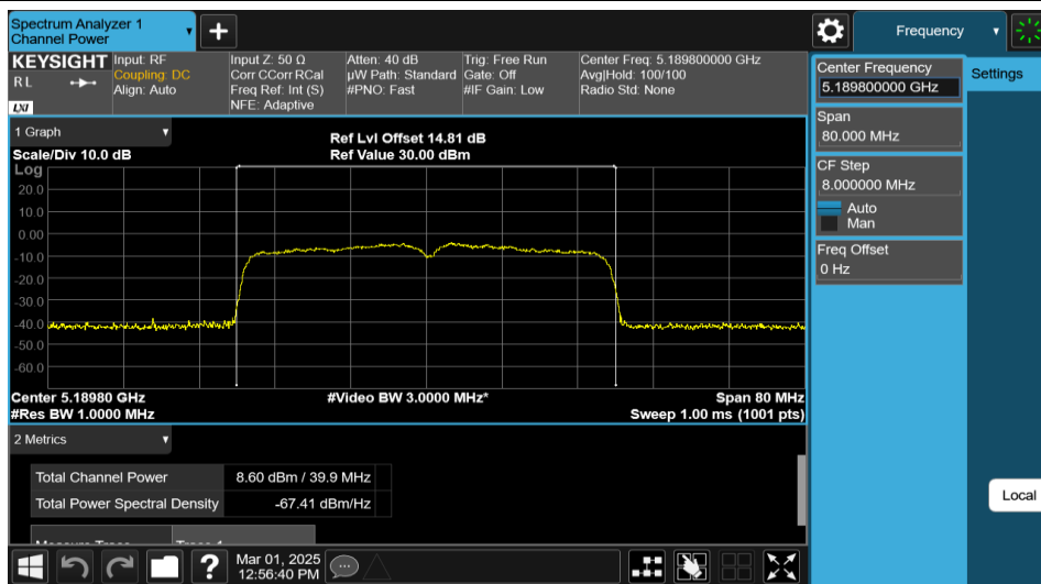
11AX40MIMO-Ant1-5190-PASS
