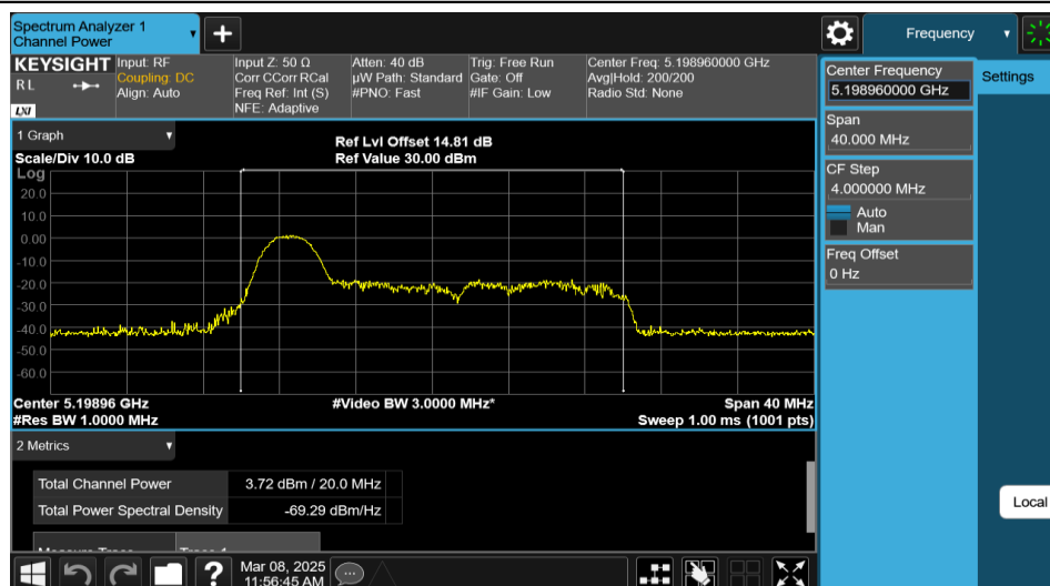
11AX20MIMO-Ant1-5200-26Tone-RU0-PASS
