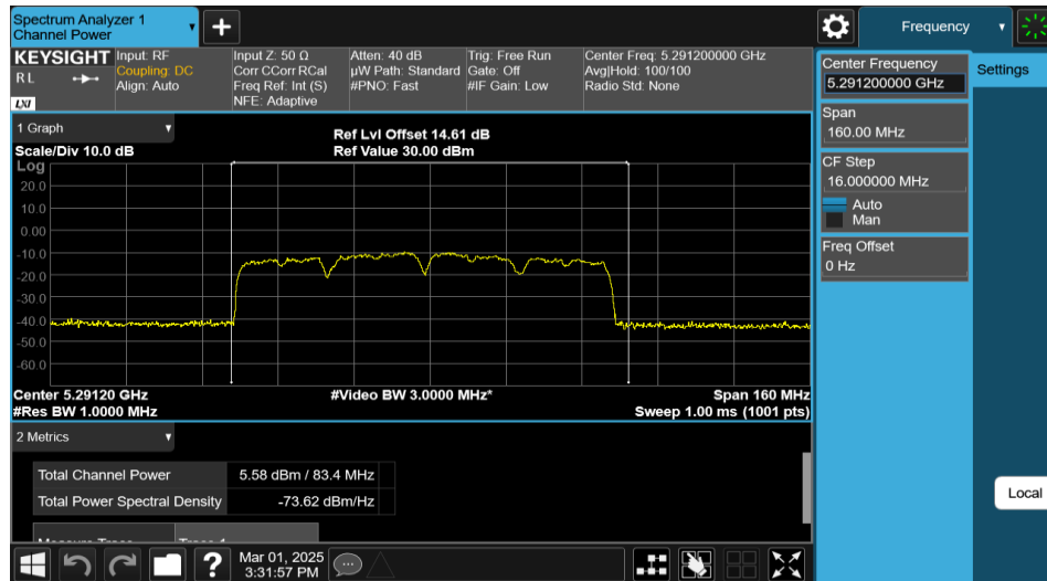
11AX80MIMO-Ant1-5290-PASS
