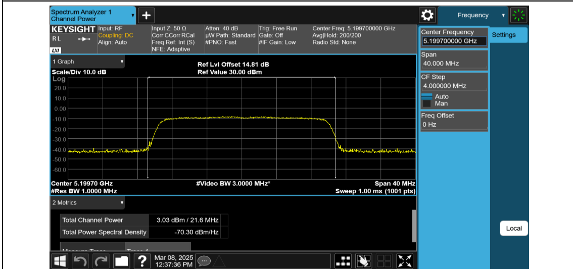
11AX20MIMO-Ant1-5200-242Tone-RU61-PASS
