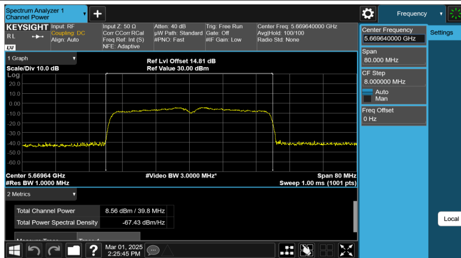
11AX40MIMO-Ant1-5670-PASS
