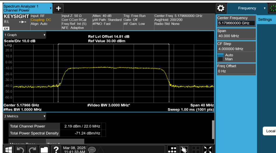
11AX20MIMO-Ant1-5180-242Tone-RU61-PASS
