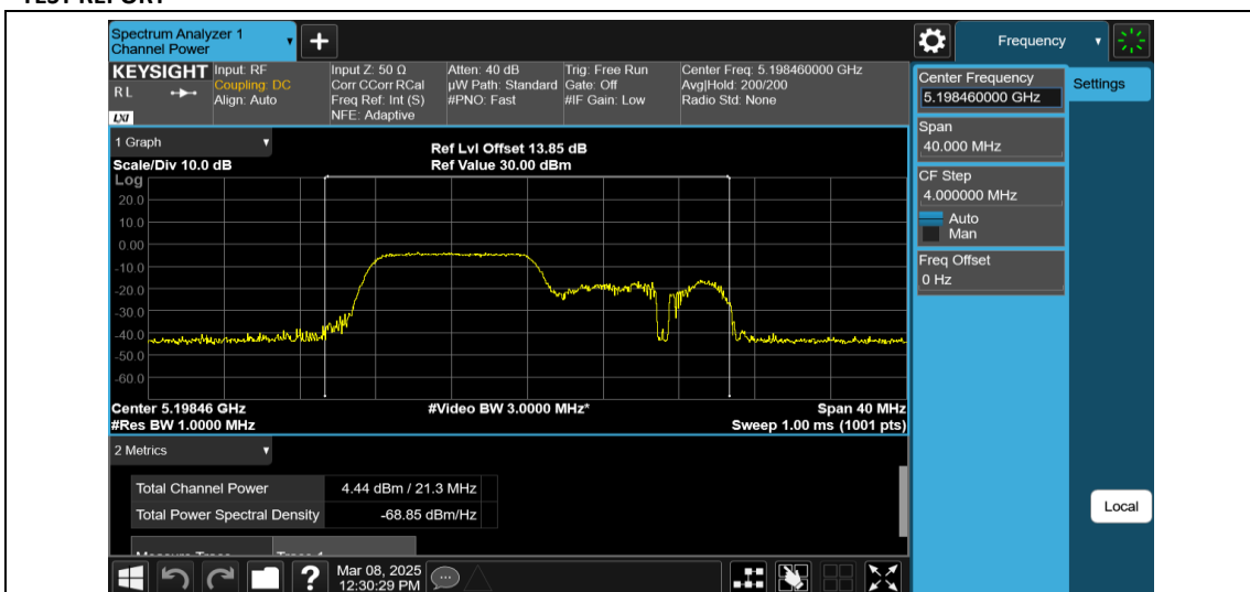
11AX20MIMO-Ant2-5200-106Tone-RU53-PASS
