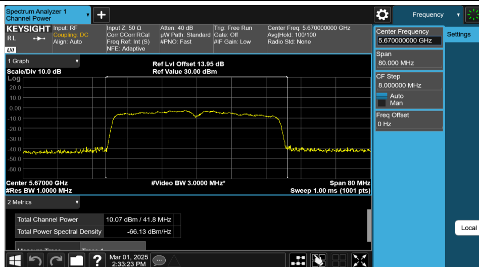
11AX40MIMO-Ant2-5670-PASS
