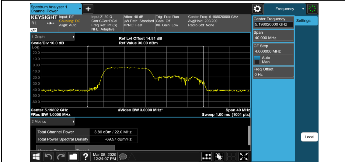
11AX20MIMO-Ant1-5200-106Tone-RU53-PASS
