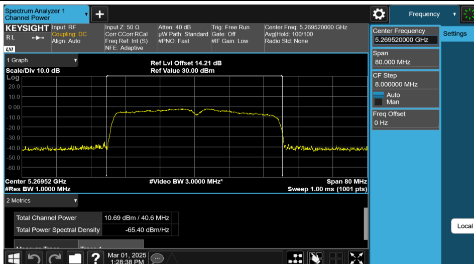
11AX40MIMO-Ant2-5270-PASS
