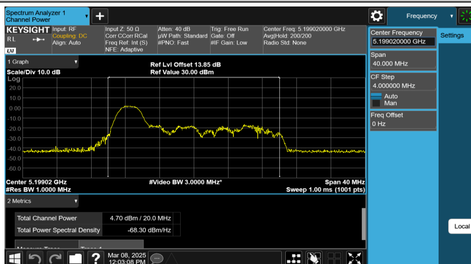
11AX20MIMO-Ant2-5200-26Tone-RU0-PASS
