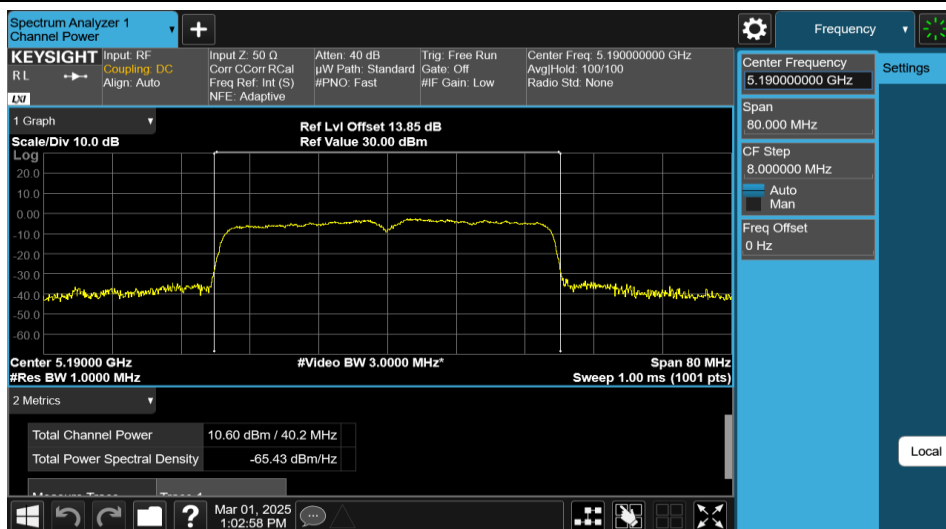
11AX40MIMO-Ant2-5190-PASS
