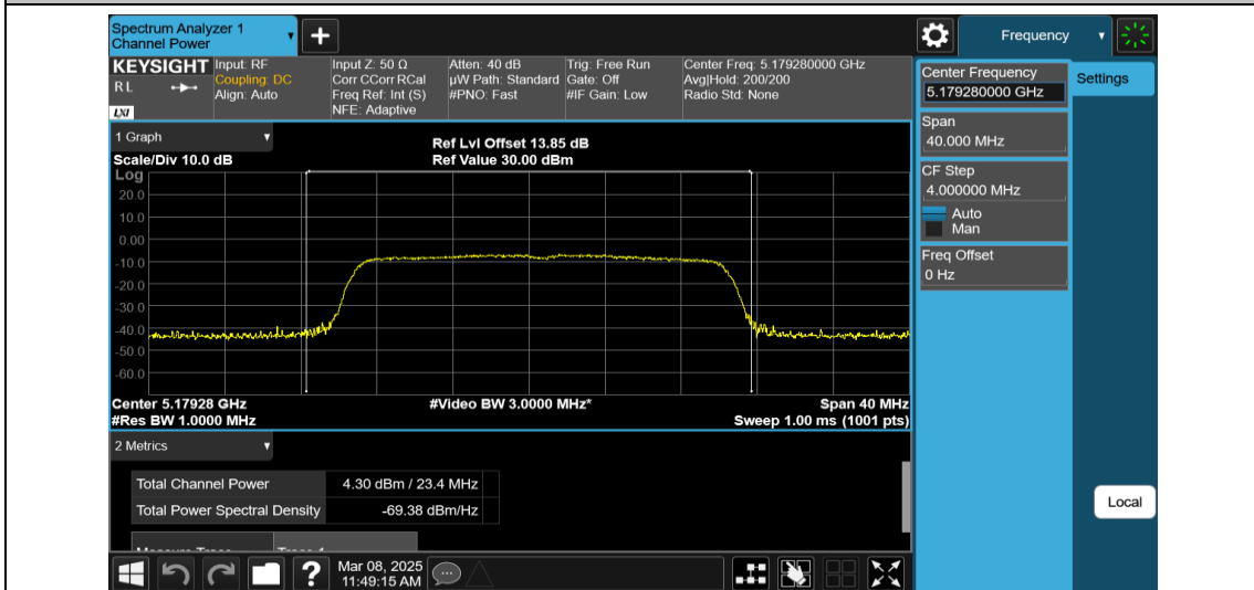
11AX20MIMO-Ant2-5180-242Tone-RU61-PASS
