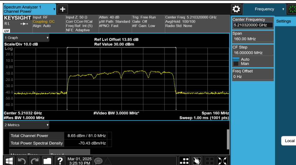
11AX80MIMO-Ant2-5210-PASS
