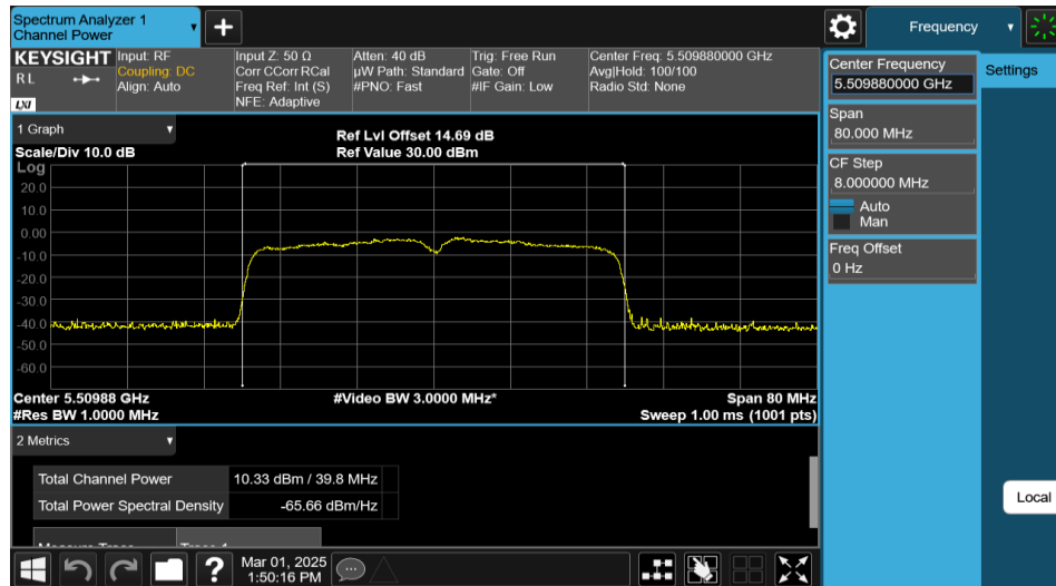
11AX40MIMO-Ant1-5510-PASS
