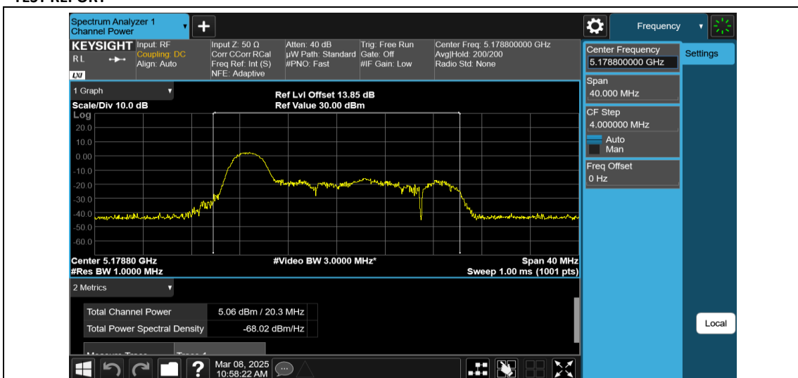
11AX20MIMO-Ant2-5180-26Tone-RU0-PASS
