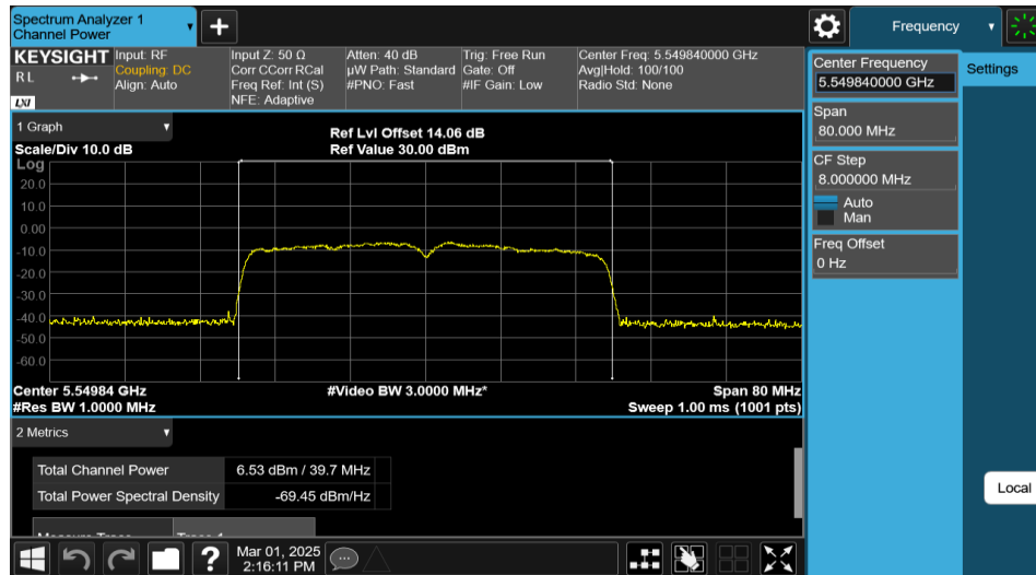
11AX40MIMO-Ant2-5550-PASS
