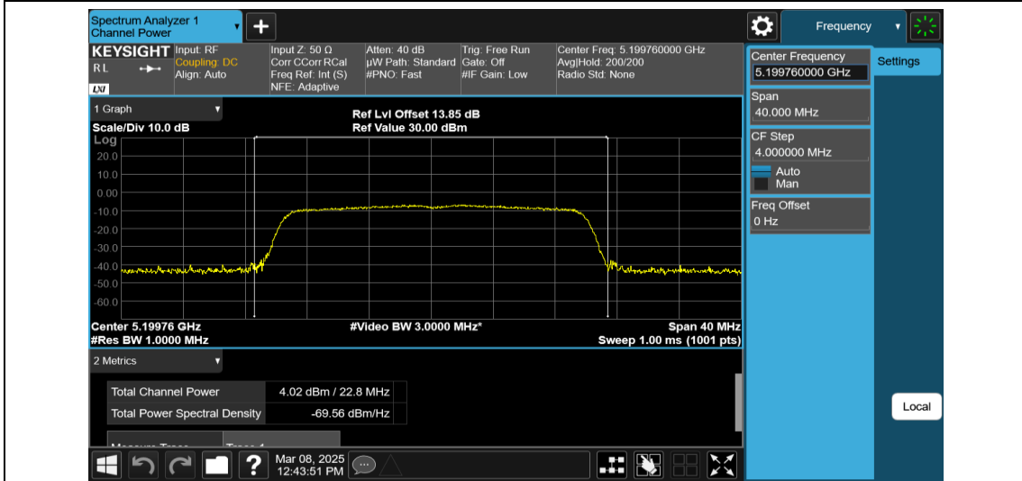
11AX20MIMO-Ant2-5200-242Tone-RU61-PASS
