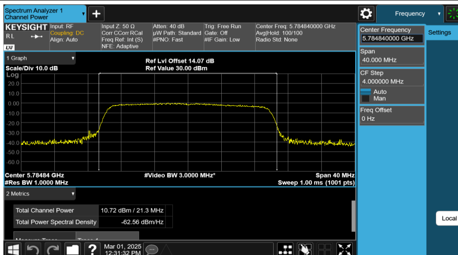
11AX20MIMO-Ant2-5785-PASS
