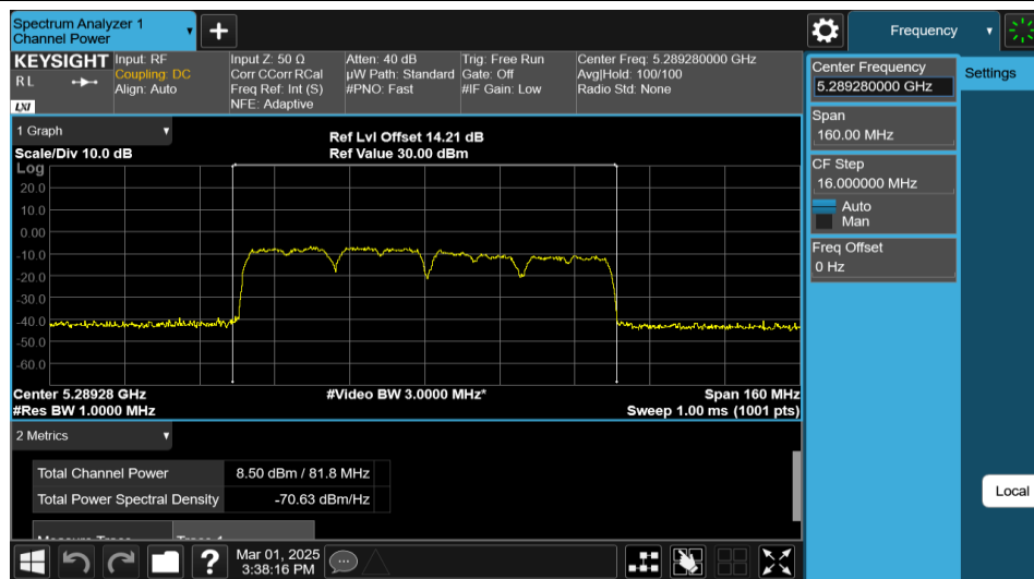
11AX80MIMO-Ant2-5290-PASS
