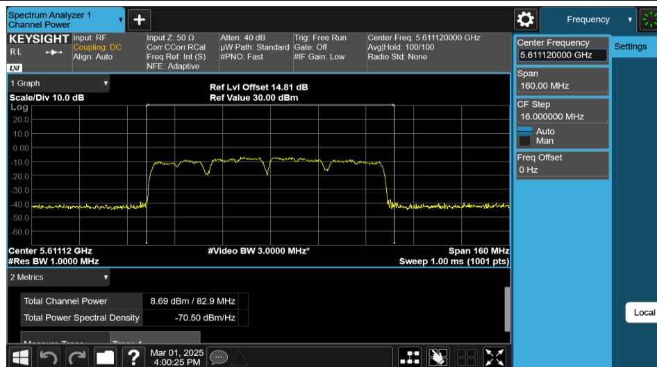
11AX80MIMO-Ant1-5610-PASS
