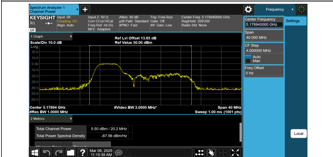
11AX20MIMO-Ant2-5180-52Tone-RU37-PASS
