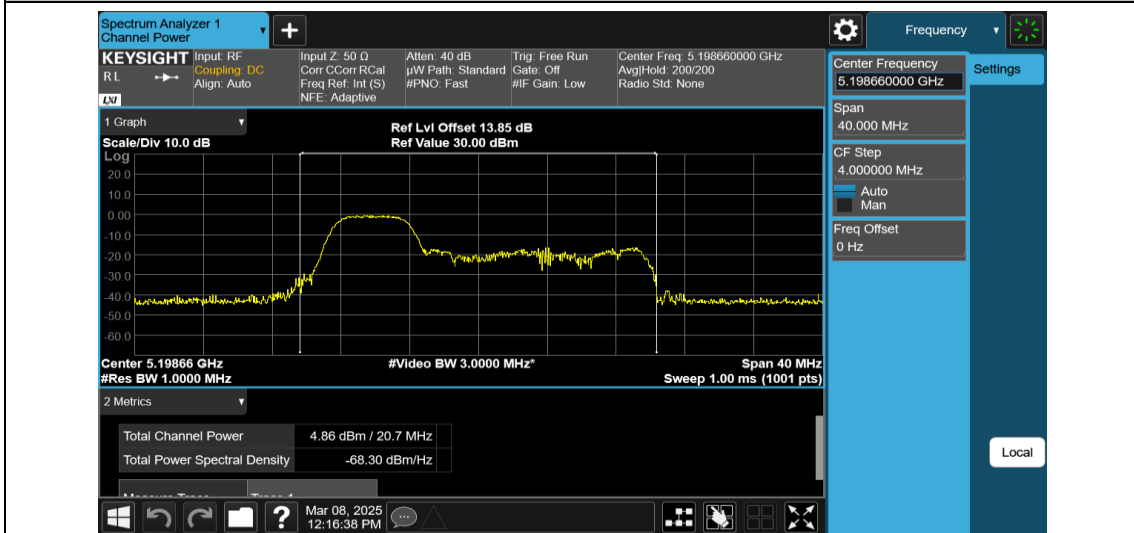
11AX20MIMO-Ant2-5200-52Tone-RU37-PASS
