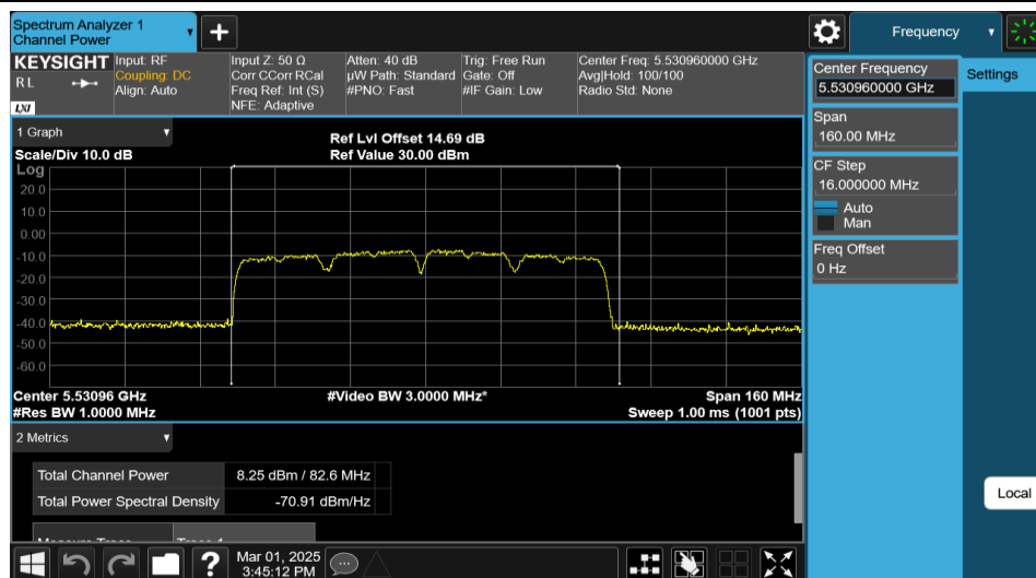
11AX80MIMO-Ant1-5530-PASS
