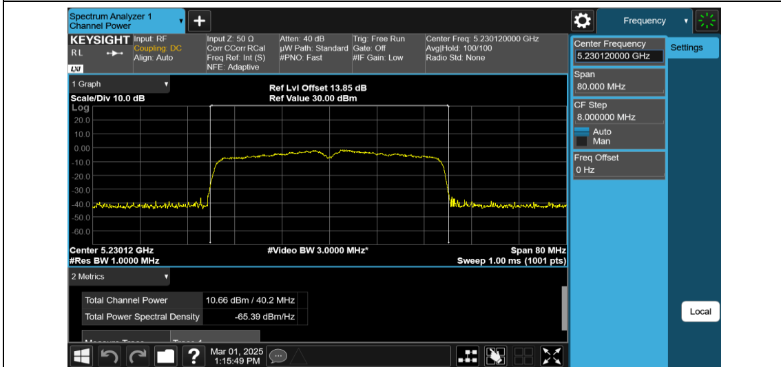
11AX40MIMO-Ant2-5230-PASS
