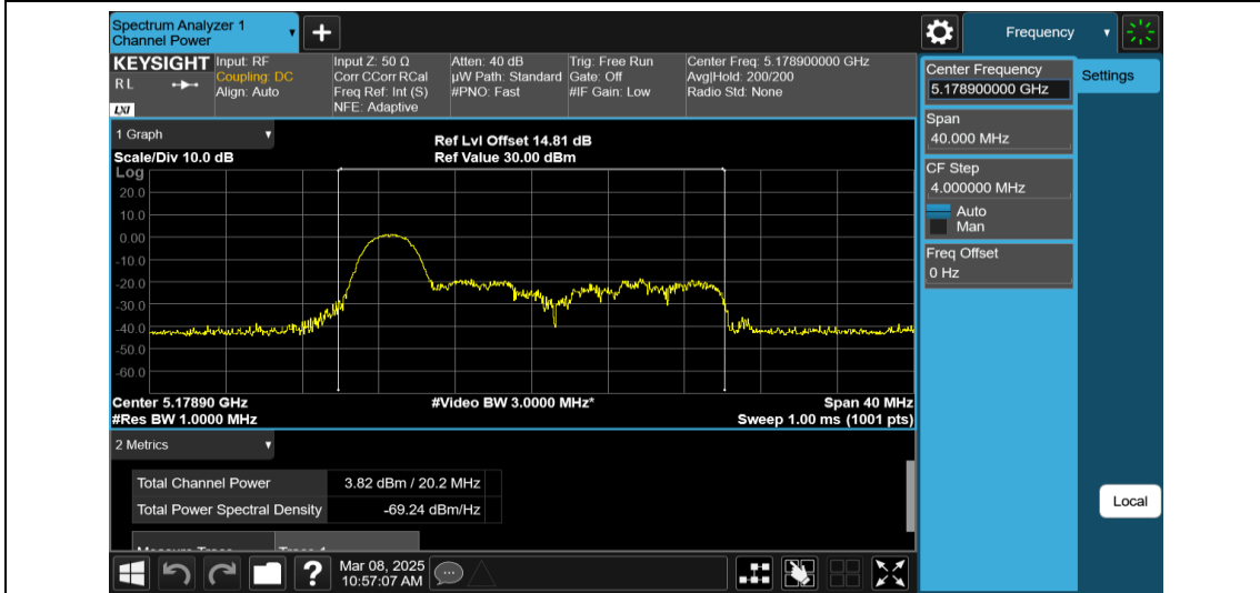
11AX20MIMO-Ant1-5180-26Tone-RU0-PASS
