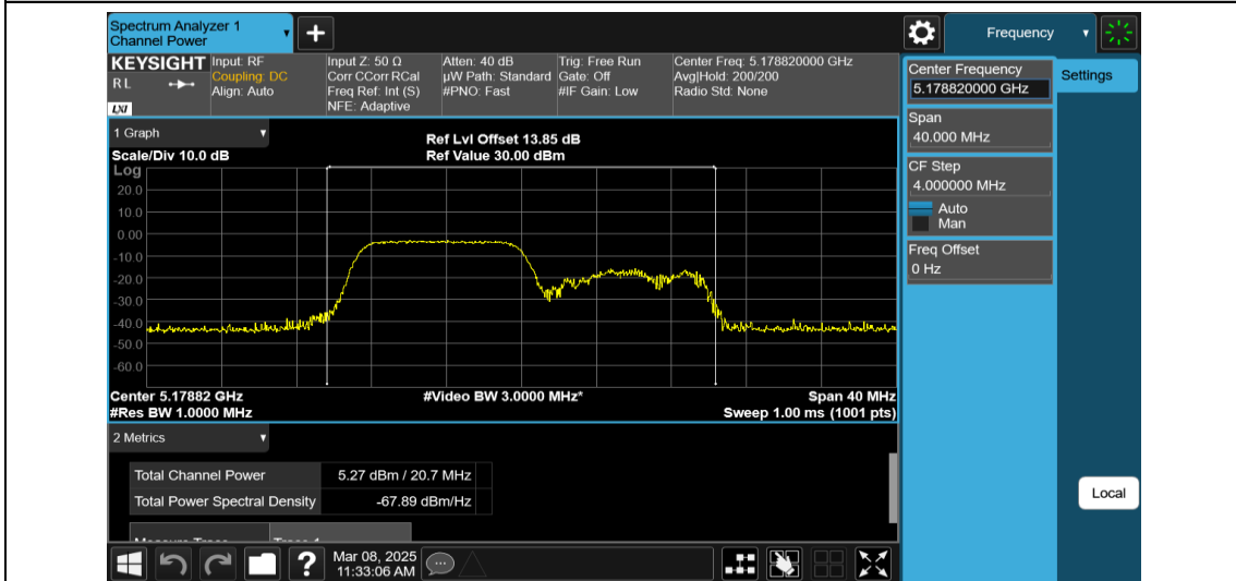
11AX20MIMO-Ant2-5180-106Tone-RU53-PASS
