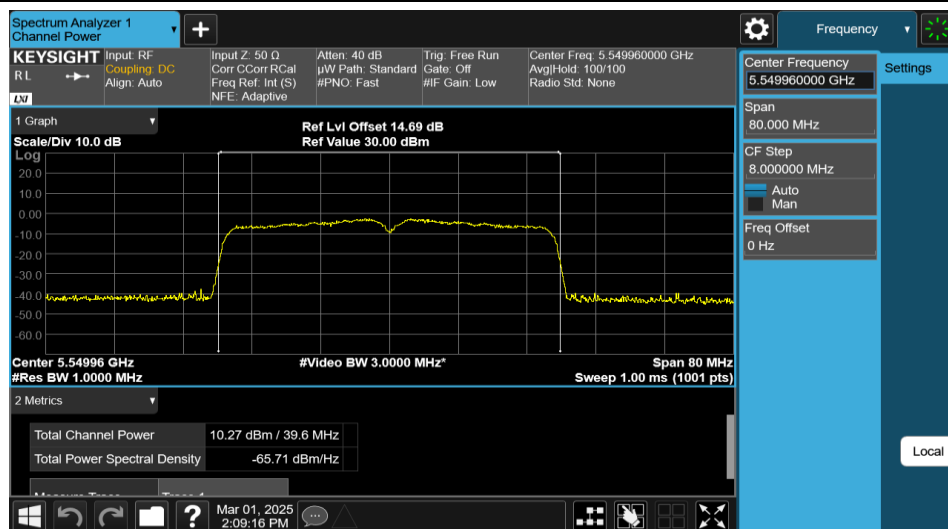
11AX40MIMO-Ant1-5550-PASS
