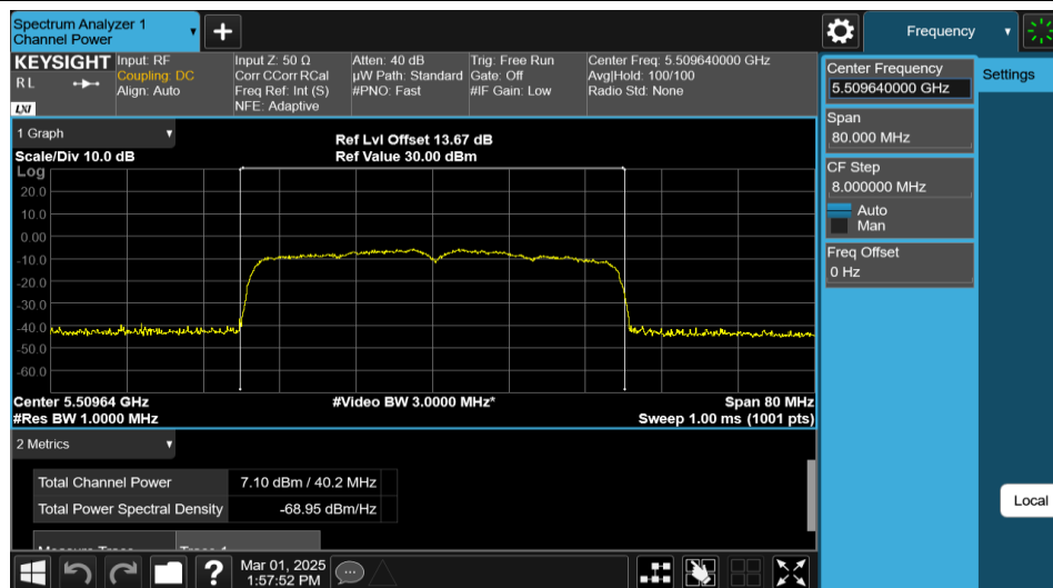
11AX40MIMO-Ant2-5510-PASS
