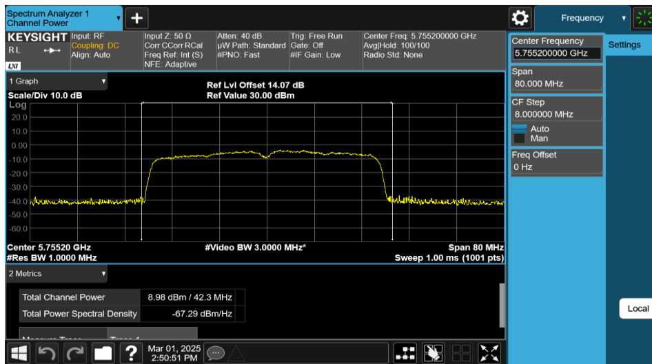
11AX40MIMO-Ant2-5755-PASS
