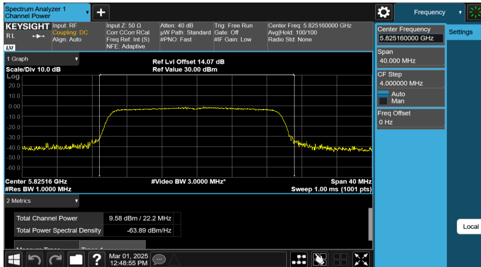
11AX20MIMO-Ant2-5825-PASS
