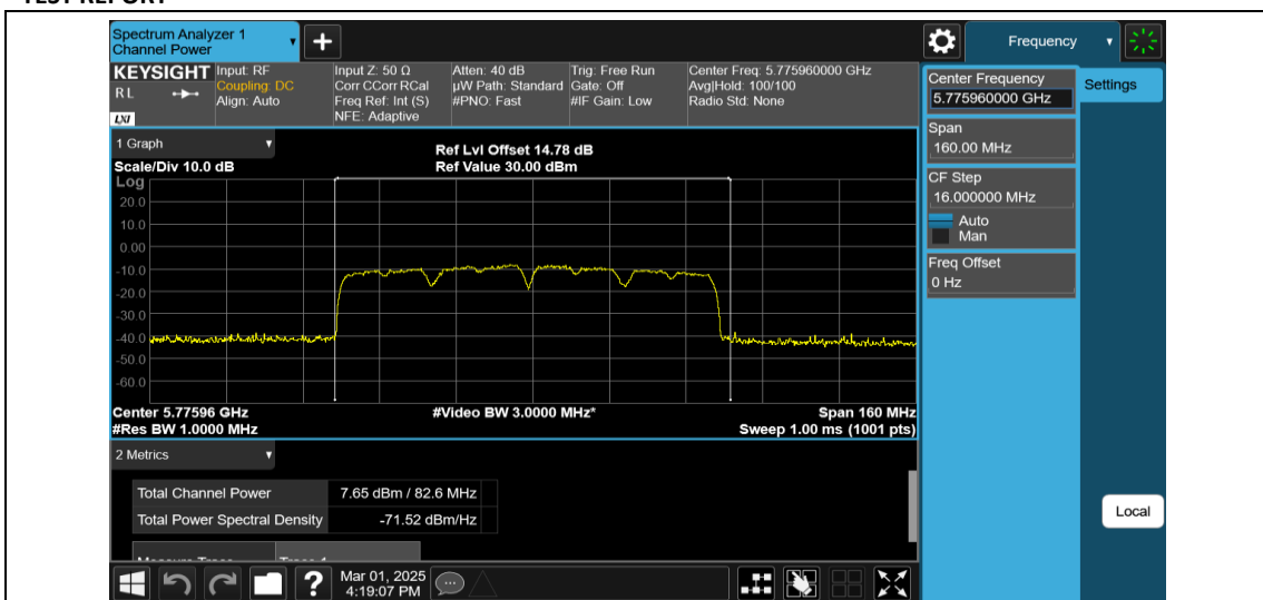
11AX80MIMO-Ant1-5775-PASS
