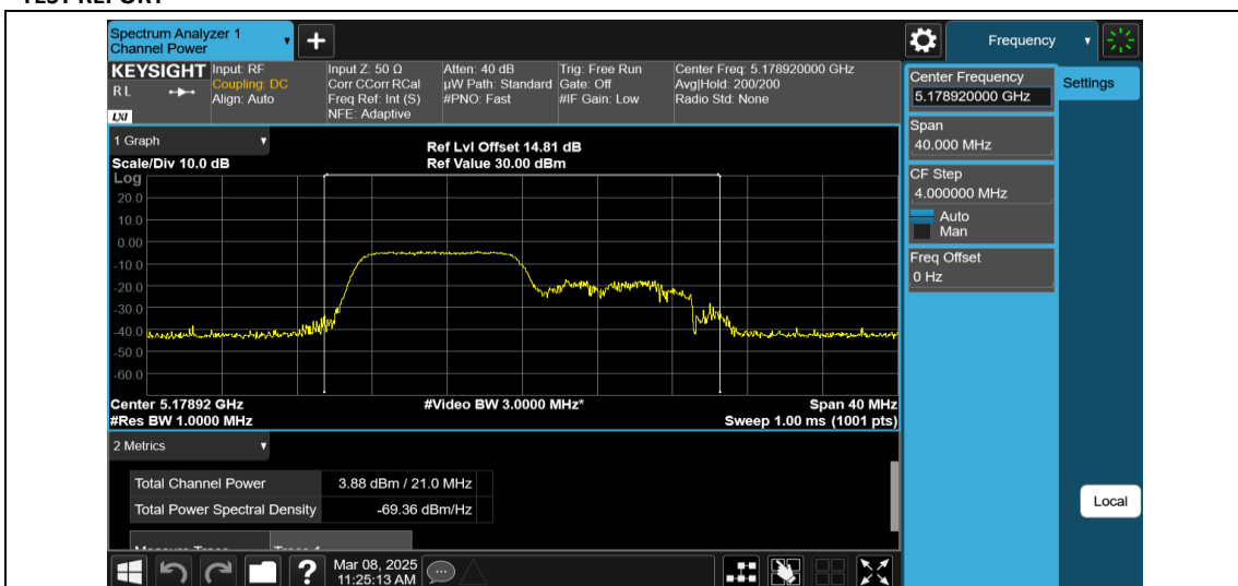
11AX20MIMO-Ant1-5180-106Tone-RU53-PASS
