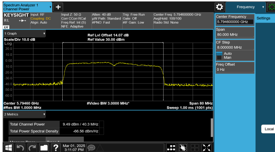
11AX40MIMO-Ant2-5795-PASS
