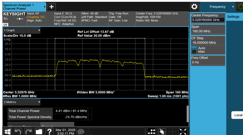
11AX80MIMO-Ant2-5530-PASS
