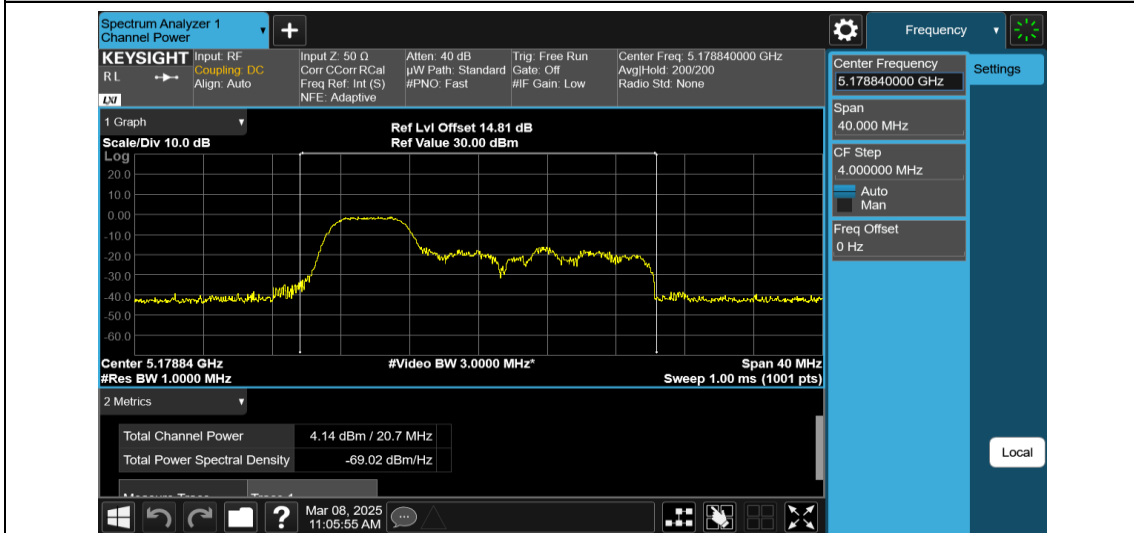
11AX20MIMO-Ant1-5180-52Tone-RU37-PASS
