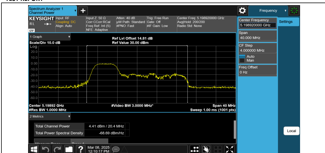
11AX20MIMO-Ant1-5200-52Tone-RU37-PASS
