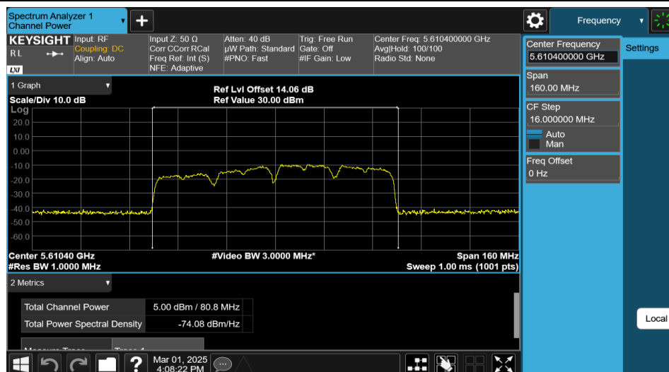
11AX80MIMO-Ant2-5610-PASS
