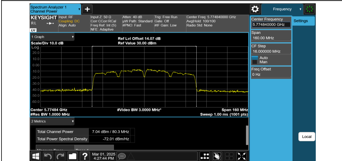
11AX80MIMO-Ant2-5775-PASS
