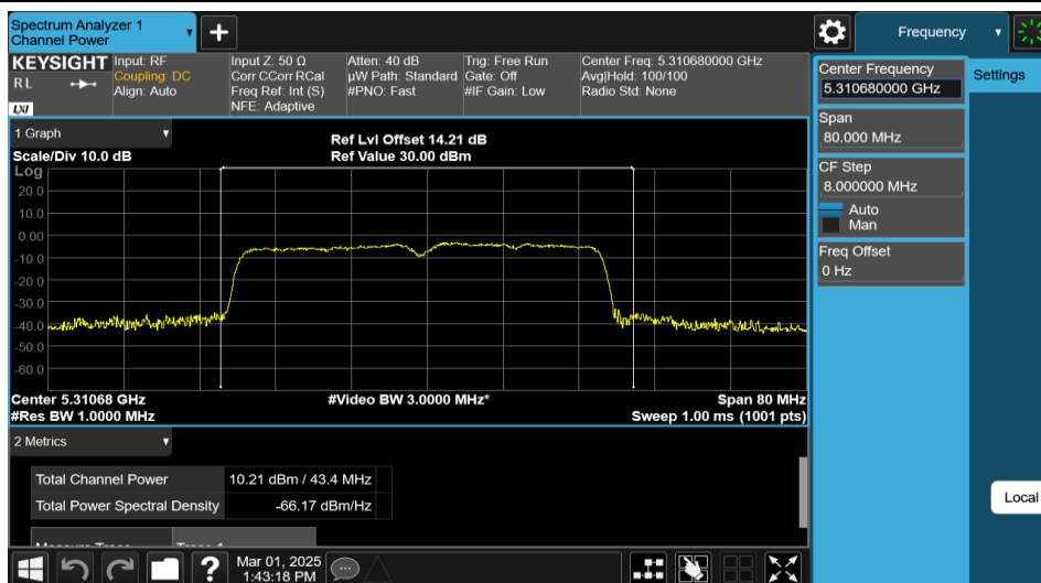
11AX40MIMO-Ant2-5310-PASS
