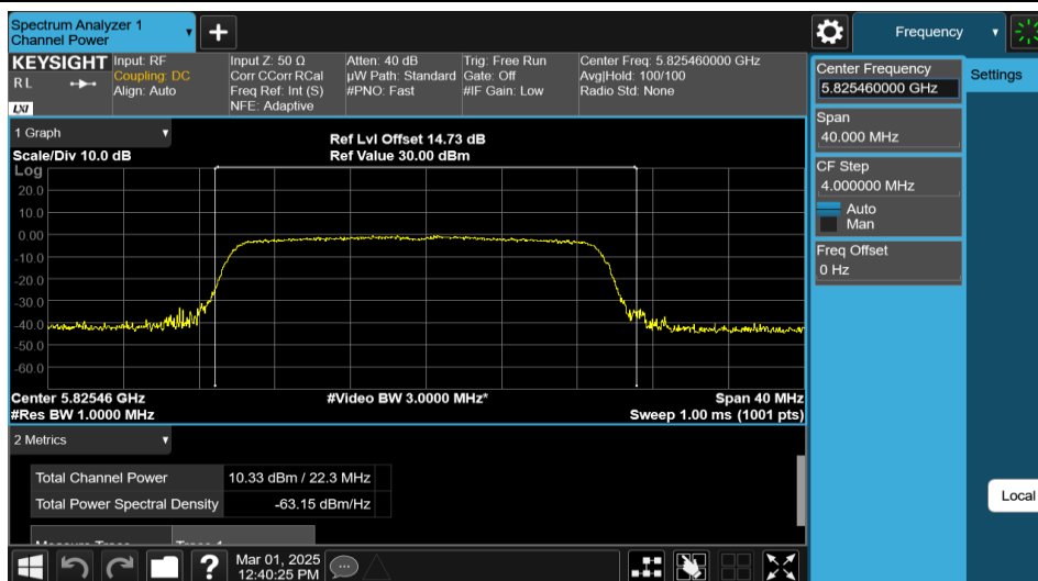
11AX20MIMO-Ant1-5825-PASS
