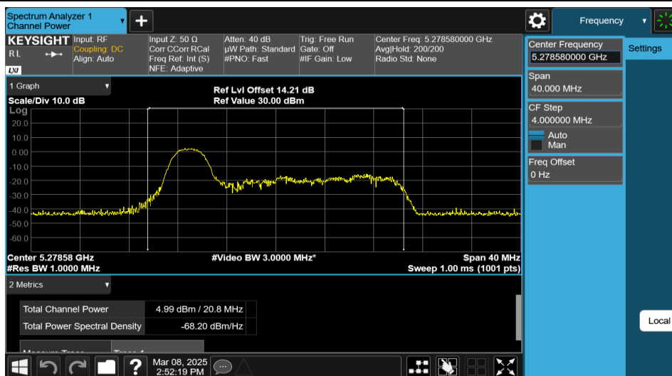
11AX20MIMO-Ant2-5280-26Tone-RU0-PASS
