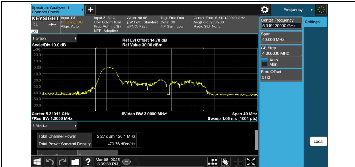
11AX20MIMO-Ant1-5320-26Tone-RU0-PASS
