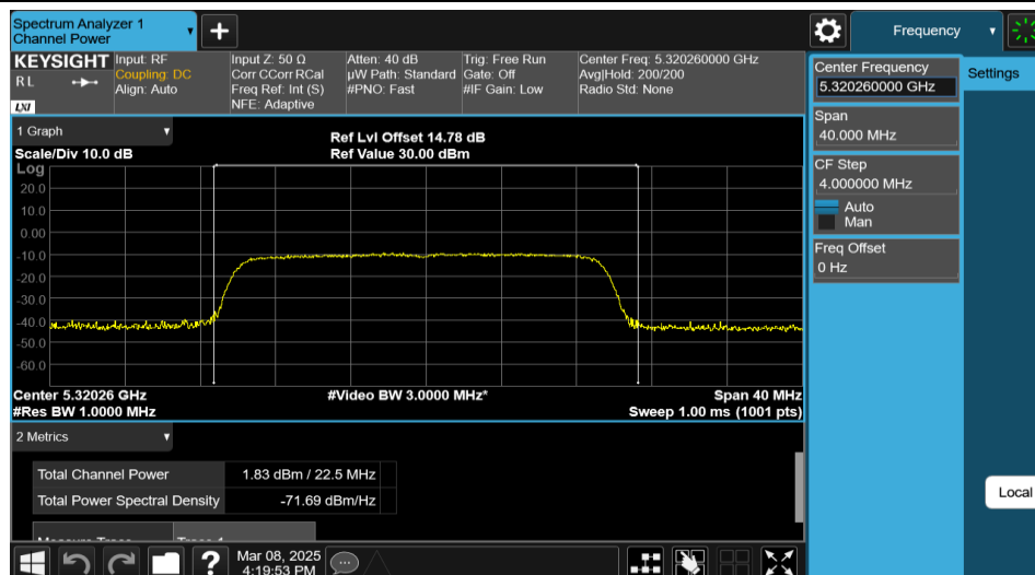
11AX20MIMO-Ant1-5320-242Tone-RU61-PASS
