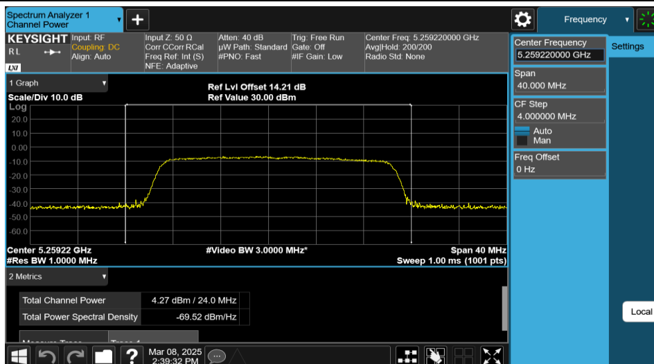
11AX20MIMO-Ant2-5260-242Tone-RU61-PASS
