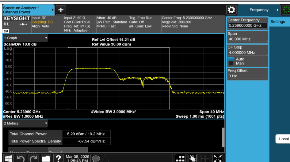
11AX20MIMO-Ant2-5240-106Tone-RU53-PASS
