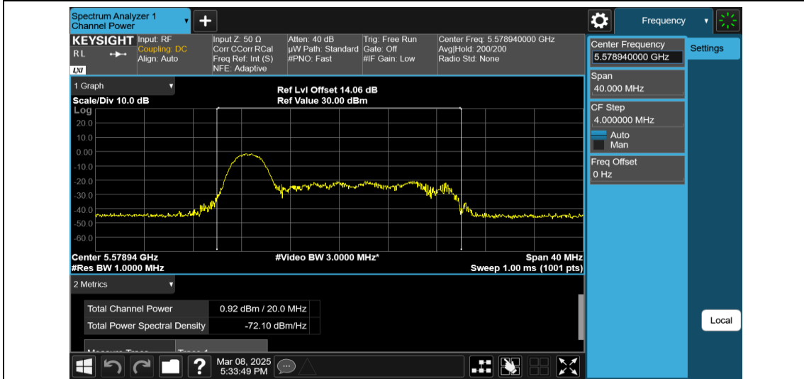
11AX20MIMO-Ant2-5580-26Tone-RU0-PASS
