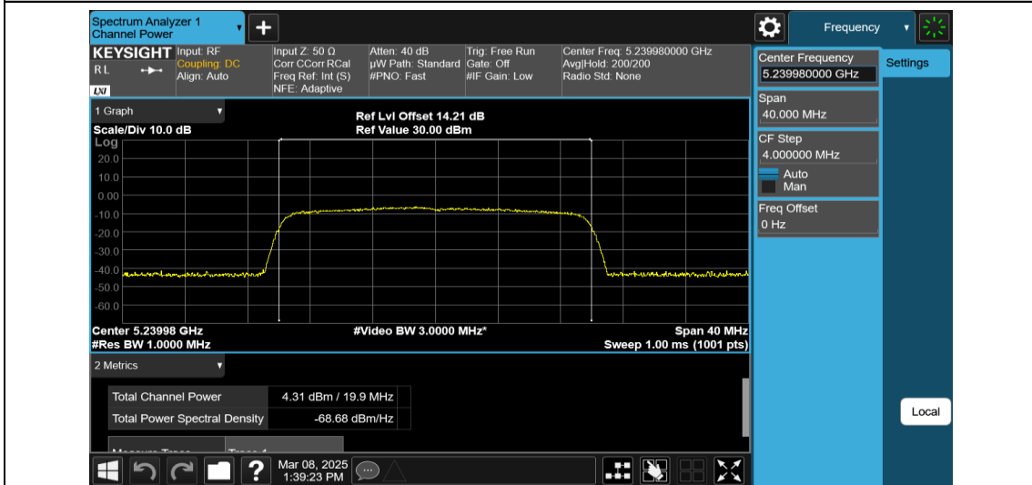
11AX20MIMO-Ant2-5240-242Tone-RU61-PASS
