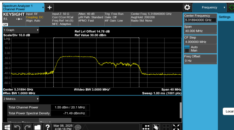
11AX20MIMO-Ant1-5320-106Tone-RU53-PASS
