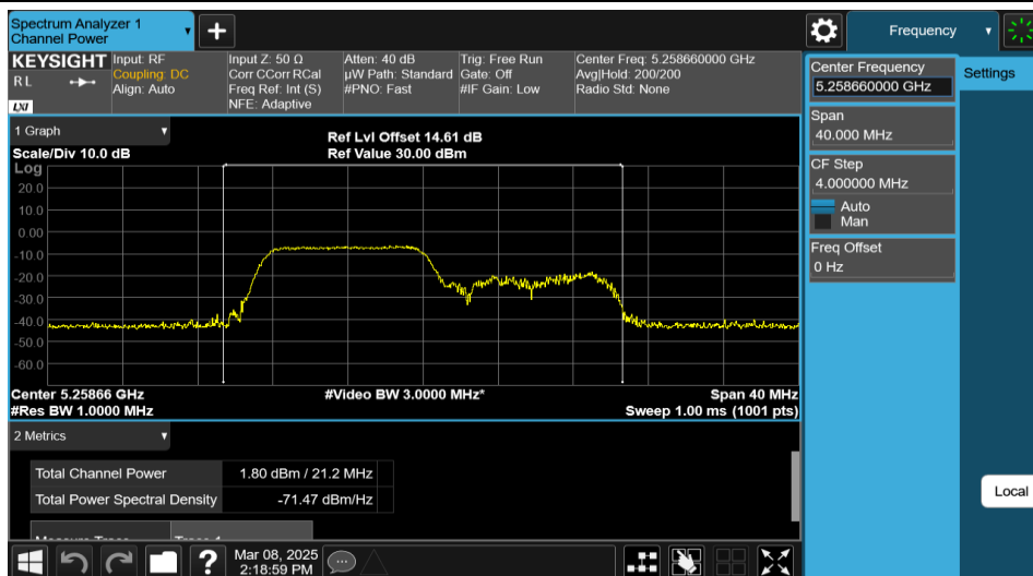
11AX20MIMO-Ant1-5260-106Tone-RU53-PASS
