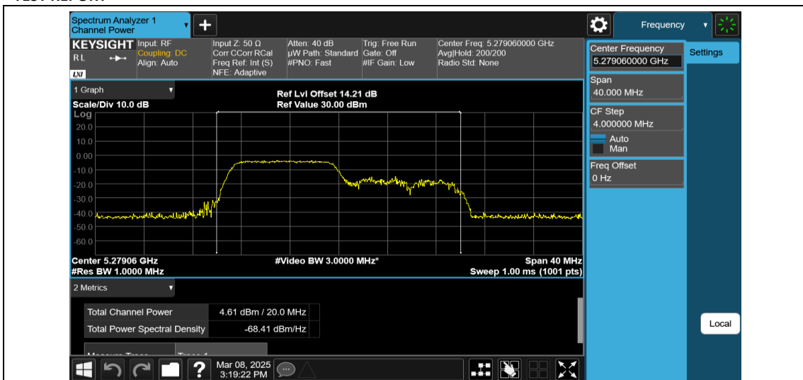
11AX20MIMO-Ant2-5280-106Tone-RU53-PASS
