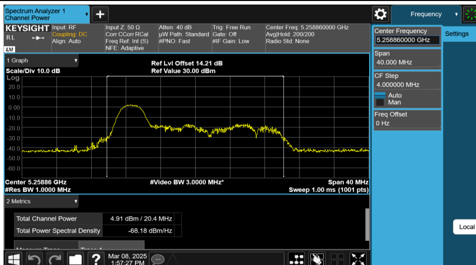
11AX20MIMO-Ant2-5260-26Tone-RU0-PASS
