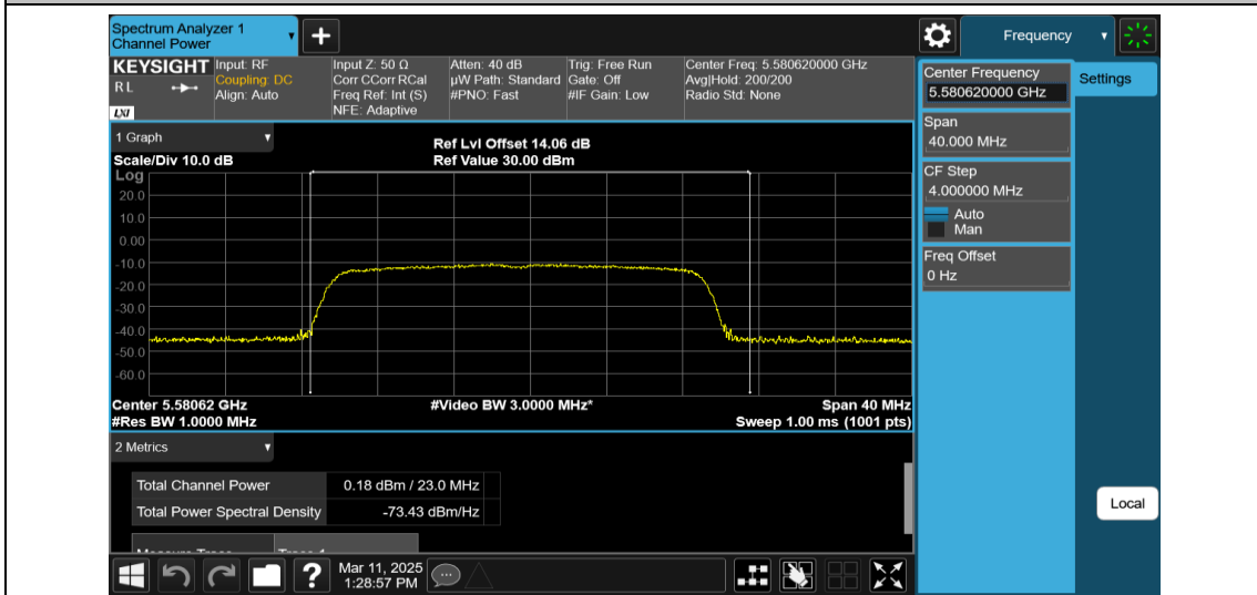
11AX20MIMO-Ant2-5580-242Tone-RU61-PASS
