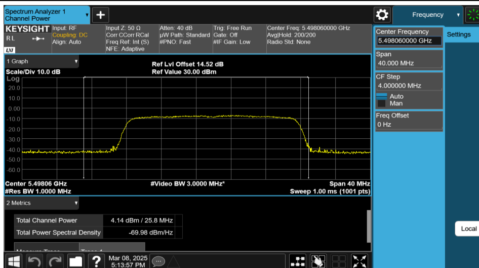
11AX20MIMO-Ant1-5500-242Tone-RU61-PASS
