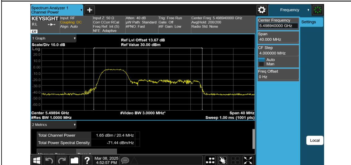
11AX20MIMO-Ant2-5500-52Tone-RU37-PASS
