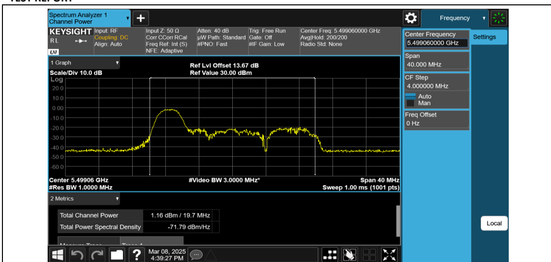
11AX20MIMO-Ant2-5500-26Tone-RU0-PASS
