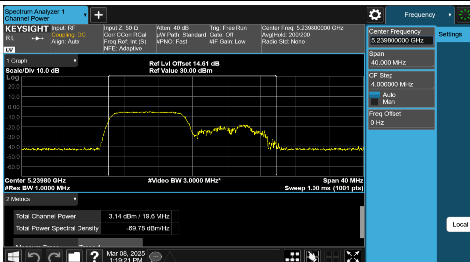
11AX20MIMO-Ant1-5240-106Tone-RU53-PASS
