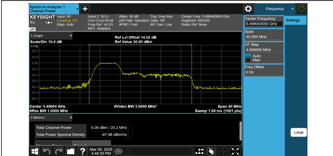
11AX20MIMO-Ant1-5500-52Tone-RU37-PASS
