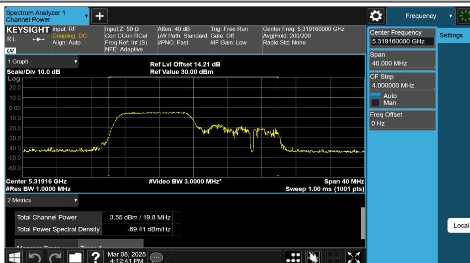
11AX20MIMO-Ant2-5320-106Tone-RU53-PASS
