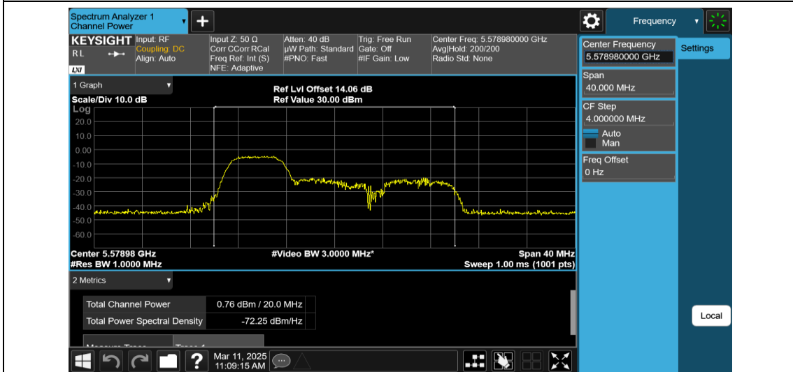
11AX20MIMO-Ant2-5580-52Tone-RU37-PASS
