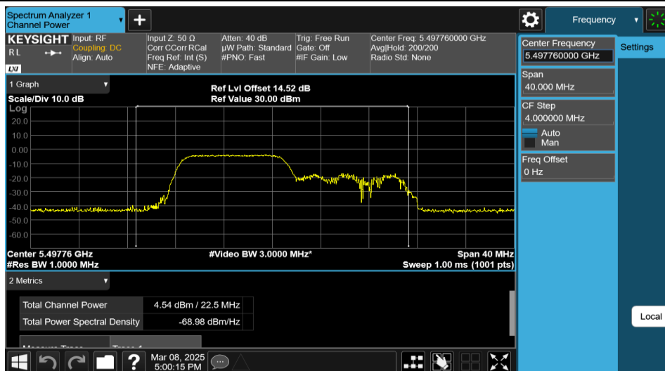
11AX20MIMO-Ant1-5500-106Tone-RU53-PASS
