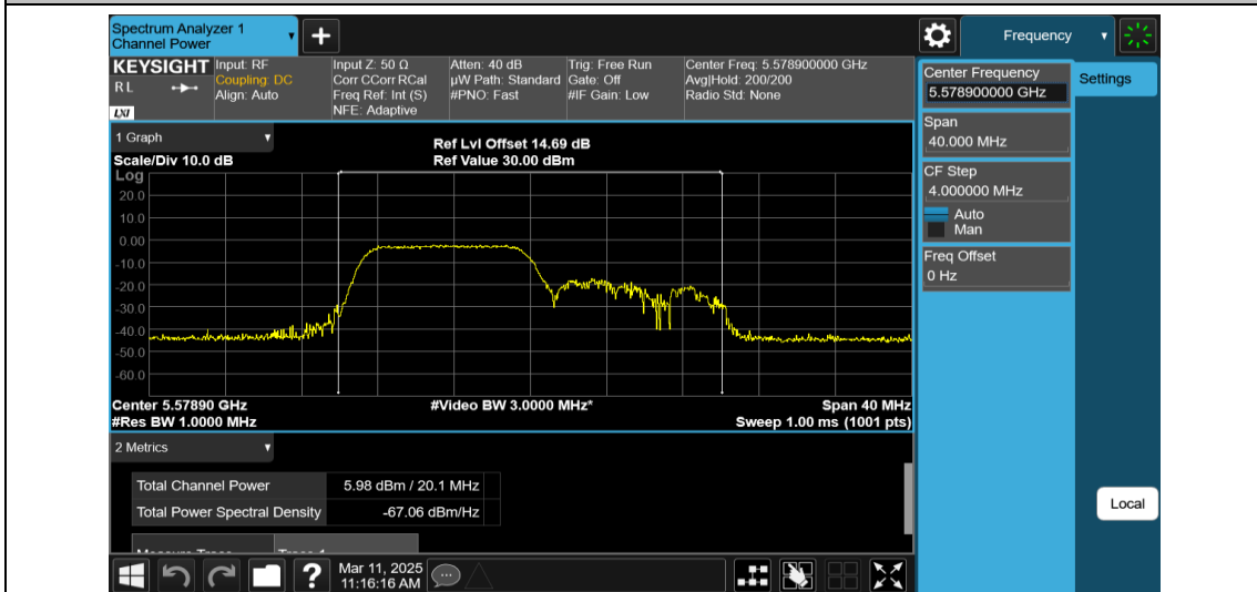
11AX20MIMO-Ant1-5580-106Tone-RU53-PASS
