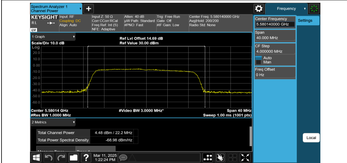
11AX20MIMO-Ant1-5580-242Tone-RU61-PASS
