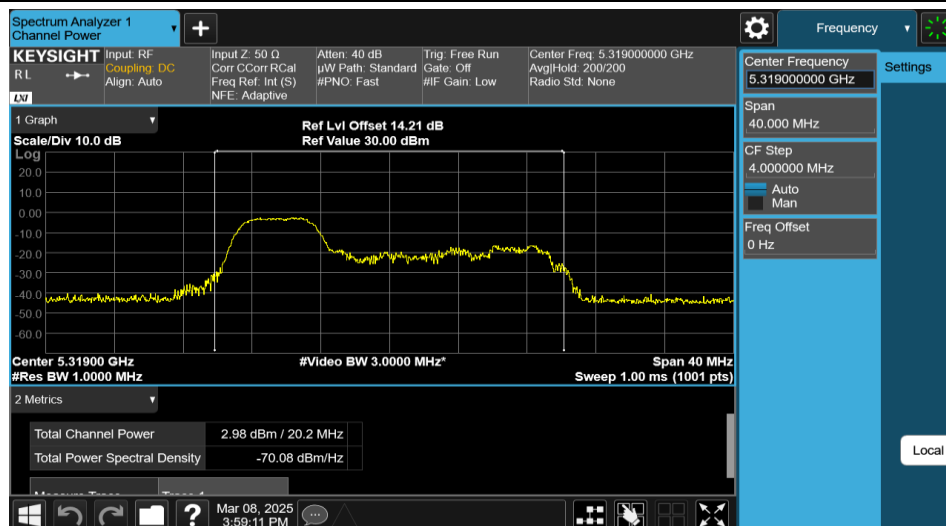
11AX20MIMO-Ant2-5320-52Tone-RU37-PASS
