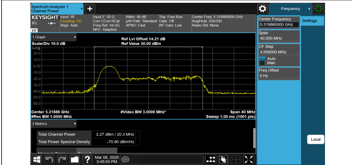
11AX20MIMO-Ant2-5320-26Tone-RU0-PASS
