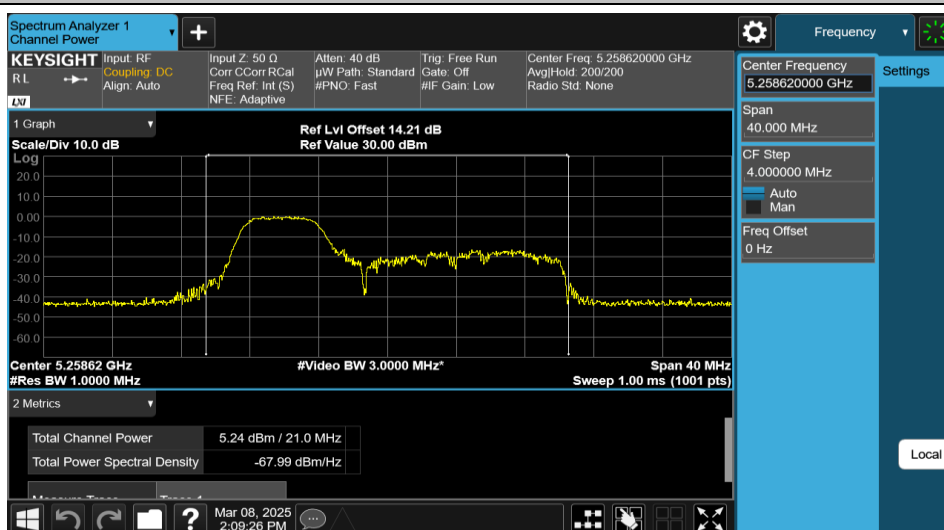
11AX20MIMO-Ant2-5260-52Tone-RU37-PASS
