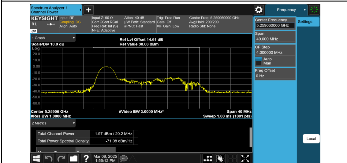
11AX20MIMO-Ant1-5260-26Tone-RU0-PASS
