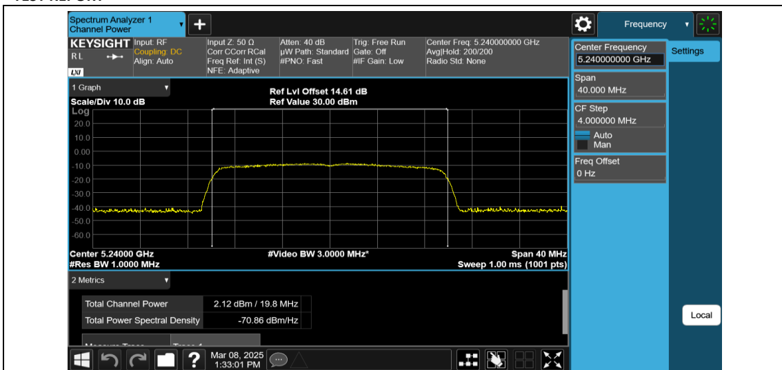
11AX20MIMO-Ant1-5240-242Tone-RU61-PASS
