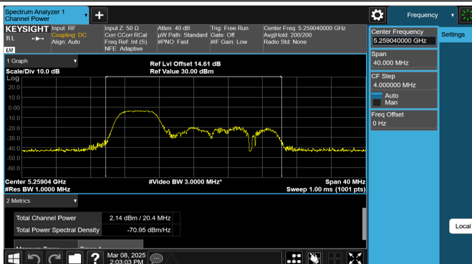
11AX20MIMO-Ant1-5260-52Tone-RU37-PASS
