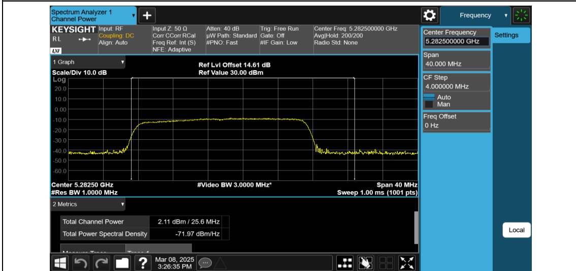
11AX20MIMO-Ant1-5280-242Tone-RU61-PASS
