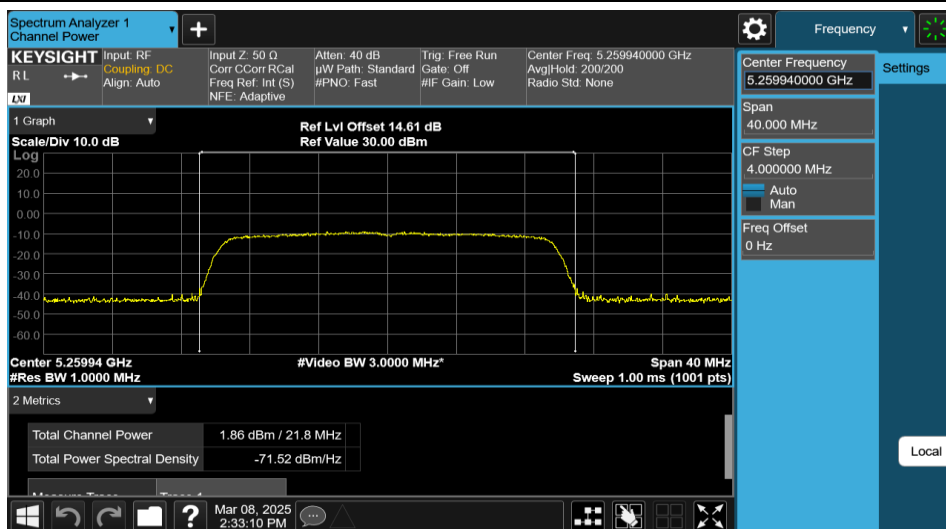
11AX20MIMO-Ant1-5260-242Tone-RU61-PASS
