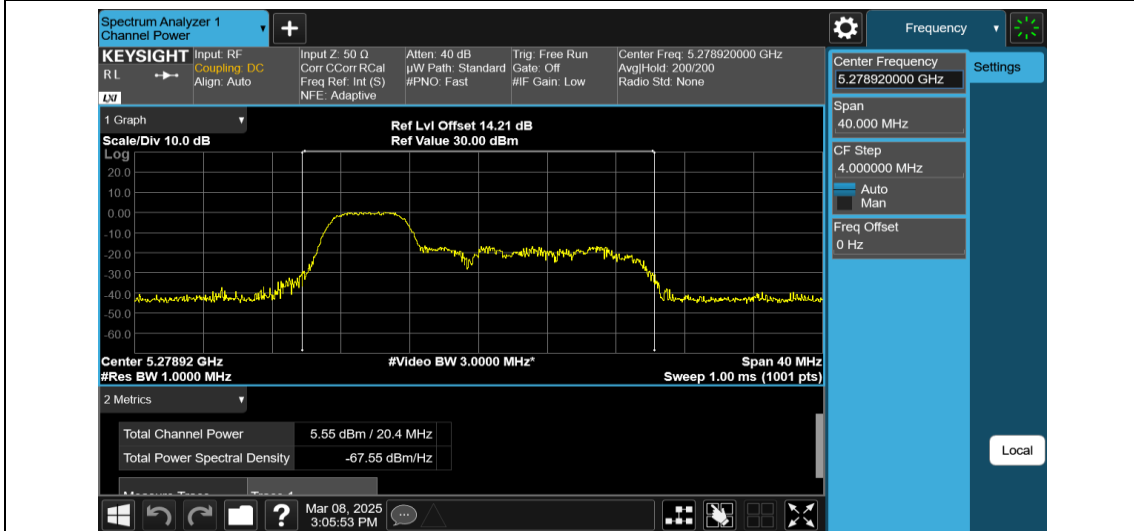
11AX20MIMO-Ant2-5280-52Tone-RU37-PASS
