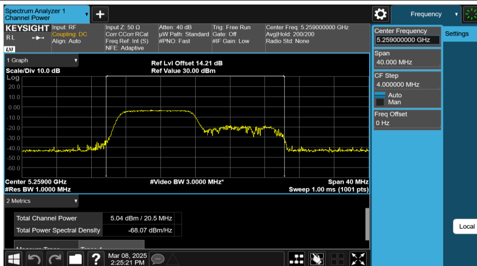
11AX20MIMO-Ant2-5260-106Tone-RU53-PASS
