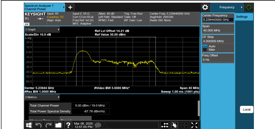
11AX20MIMO-Ant2-5240-26Tone-RU0-PASS
