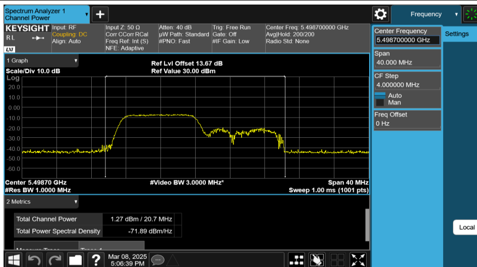
11AX20MIMO-Ant2-5500-106Tone-RU53-PASS
