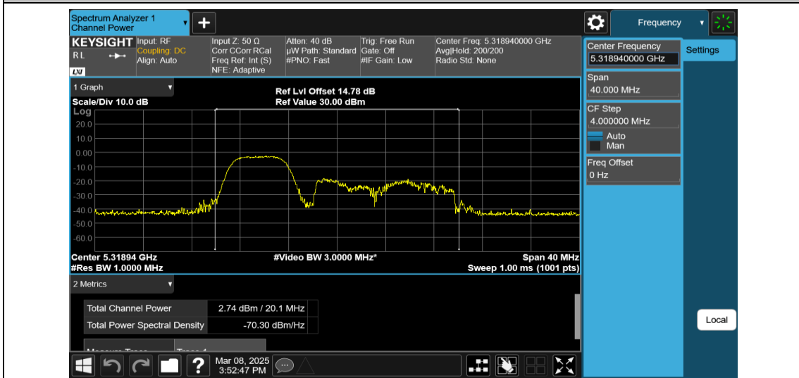
11AX20MIMO-Ant1-5320-52Tone-RU37-PASS
