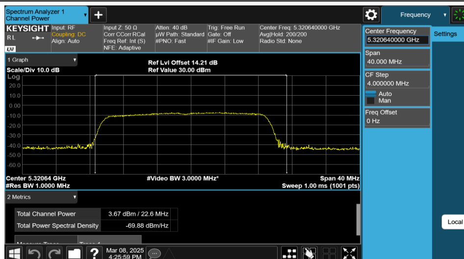
11AX20MIMO-Ant2-5320-242Tone-RU61-PASS
