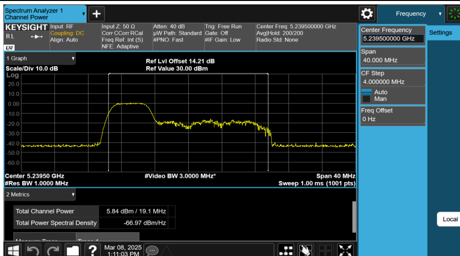
11AX20MIMO-Ant2-5240-52Tone-RU37-PASS
