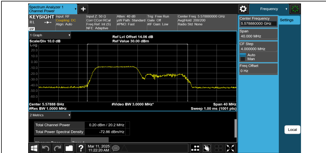
11AX20MIMO-Ant2-5580-106Tone-RU53-PASS
