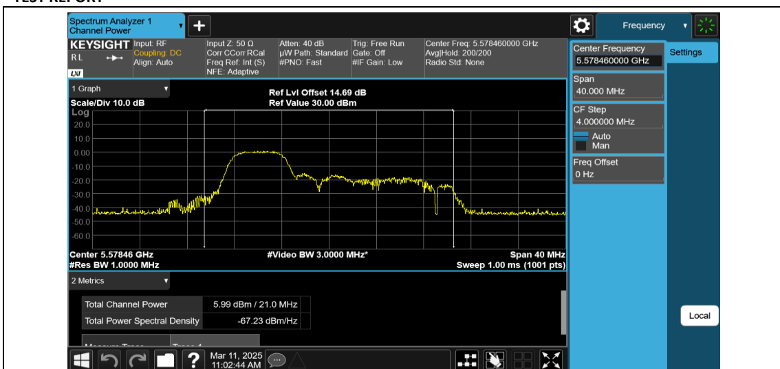
11AX20MIMO-Ant1-5580-52Tone-RU37-PASS
