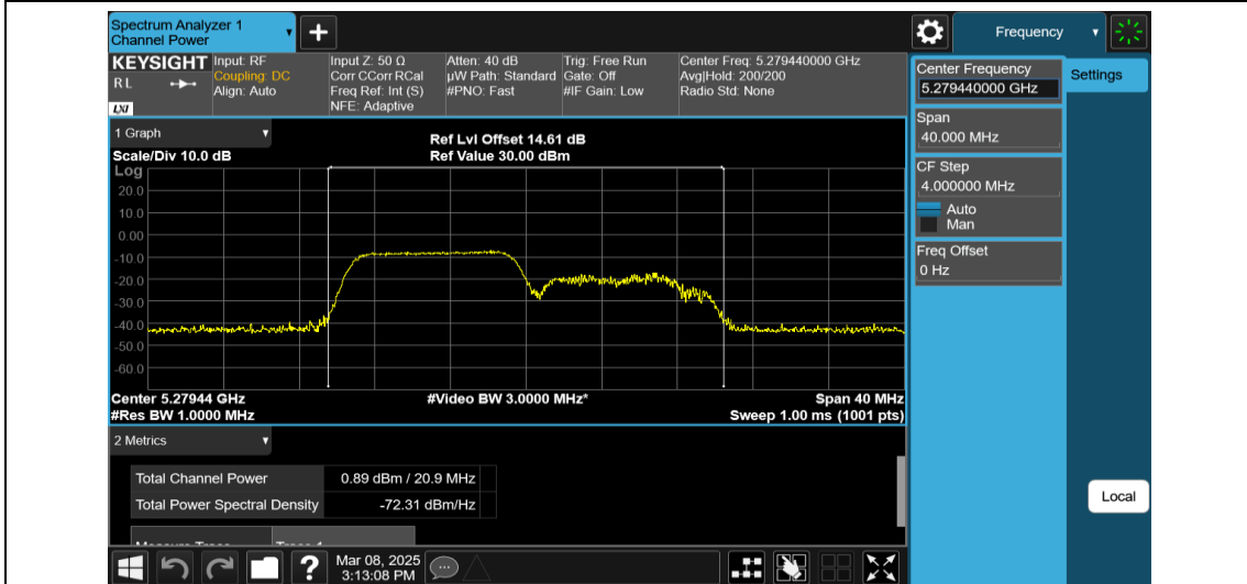
11AX20MIMO-Ant1-5280-106Tone-RU53-PASS
