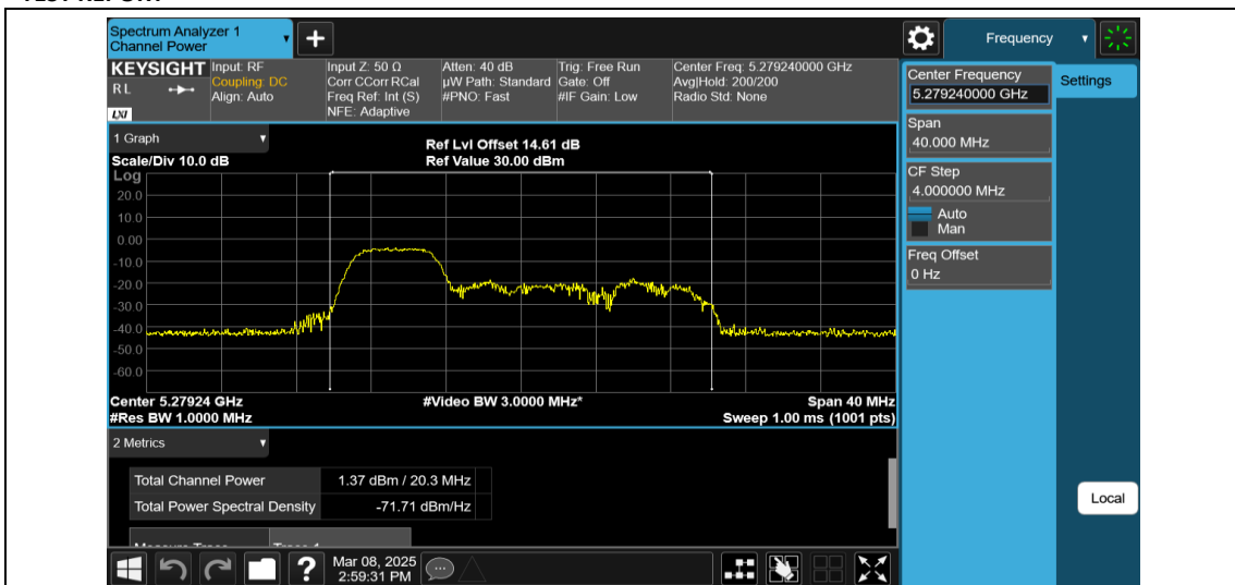
11AX20MIMO-Ant1-5280-52Tone-RU37-PASS
