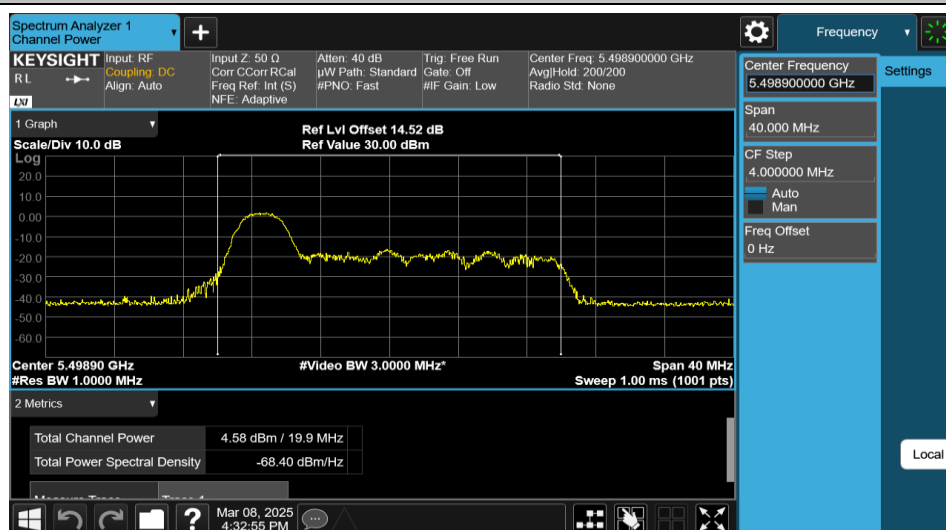
11AX20MIMO-Ant1-5500-26Tone-RU0-PASS
