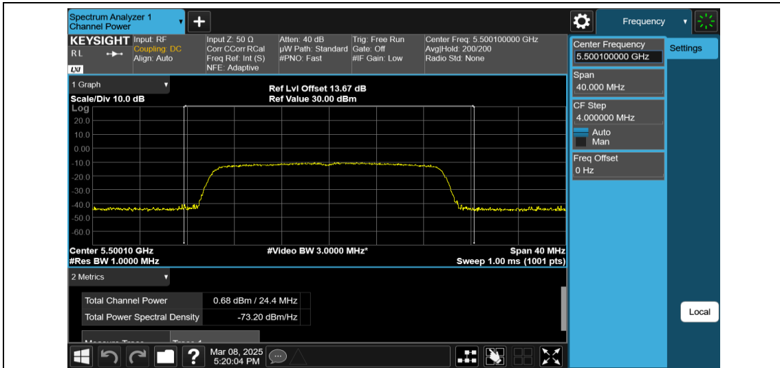
11AX20MIMO-Ant2-5500-242Tone-RU61-PASS
