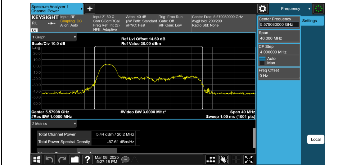
11AX20MIMO-Ant1-5580-26Tone-RU0-PASS
