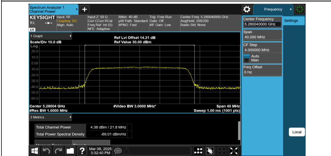
11AX20MIMO-Ant2-5280-242Tone-RU61-PASS
