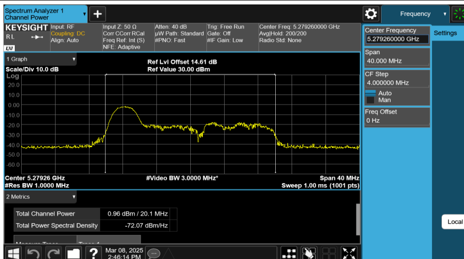
11AX20MIMO-Ant1-5280-26Tone-RU0-PASS
