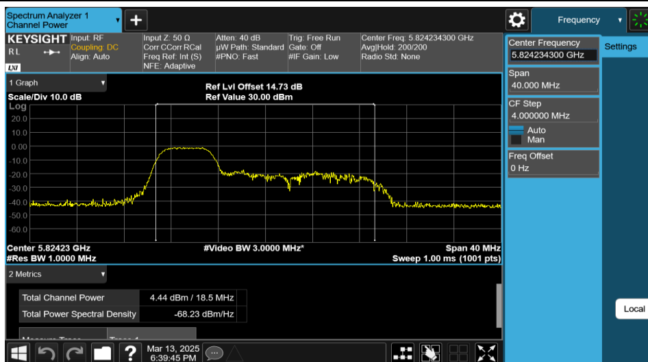
11AX20MIMO-Ant1-5825-52Tone-RU37-PASS
