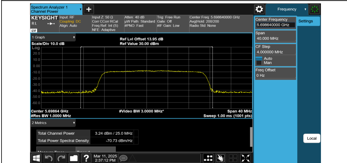
11AX20MIMO-Ant2-5700-242Tone-RU61-PASS
