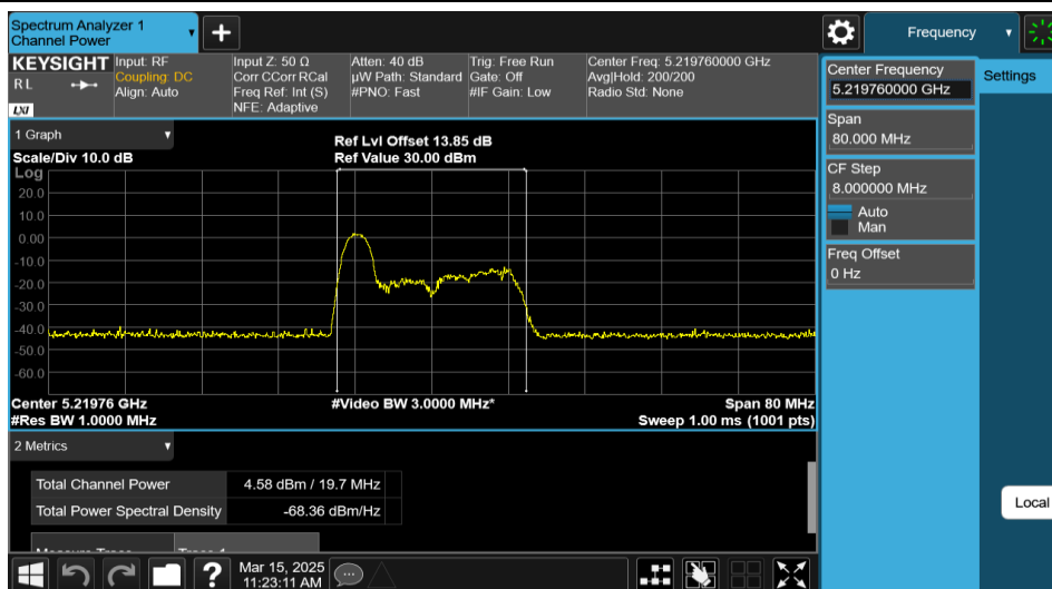
11AX40MIMO-Ant2-5230-26Tone-RU0-PASS
