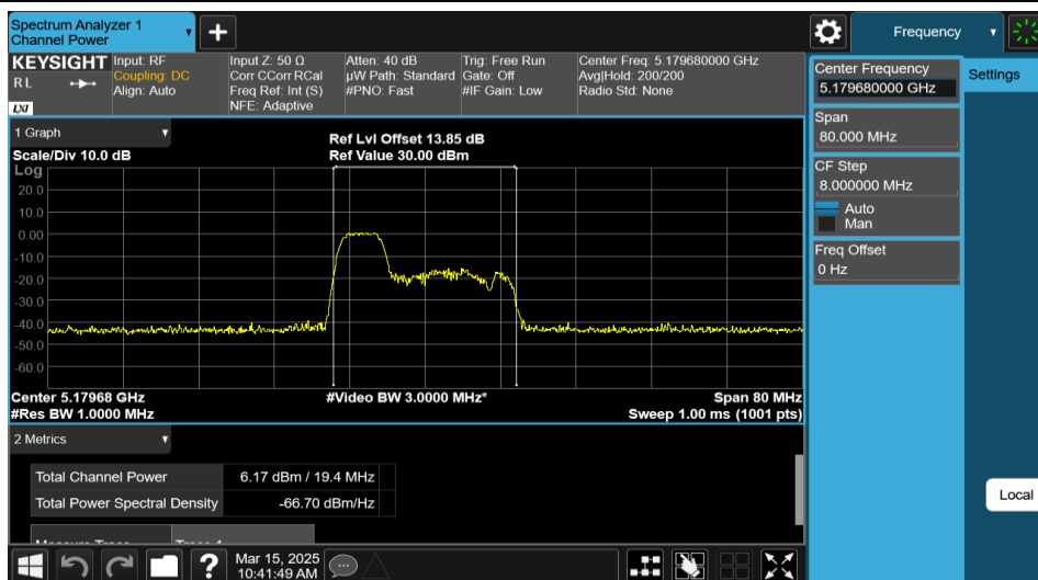
11AX40MIMO-Ant2-5190-52Tone-RU37-PASS
