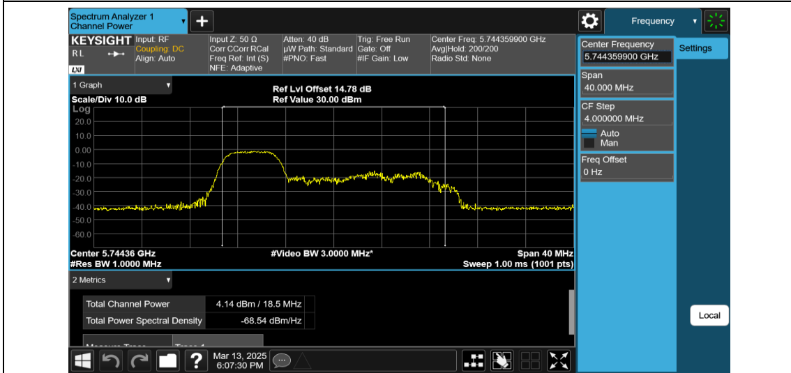
11AX20MIMO-Ant1-5745-52Tone-RU37-PASS
