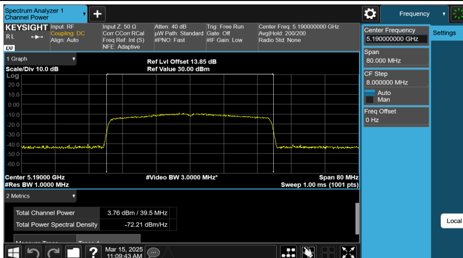
11AX40MIMO-Ant2-5190-484Tone-RU65-PASS
