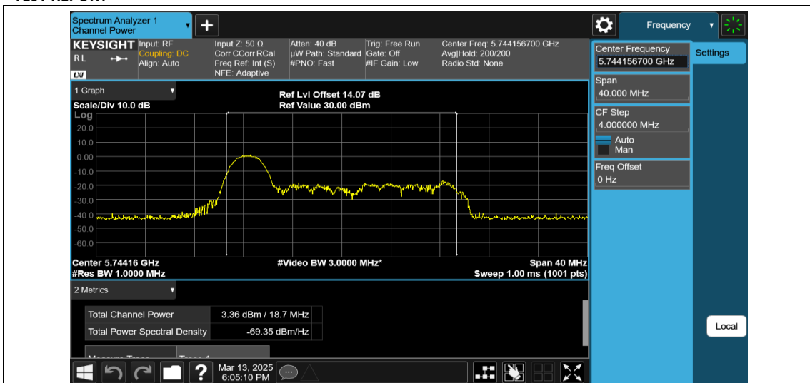
11AX20MIMO-Ant2-5745-26Tone-RU0-PASS
