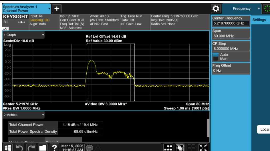
11AX40MIMO-Ant1-5230-26Tone-RU0-PASS
