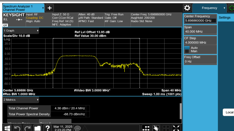
11AX20MIMO-Ant2-5700-106Tone-RU53-PASS
