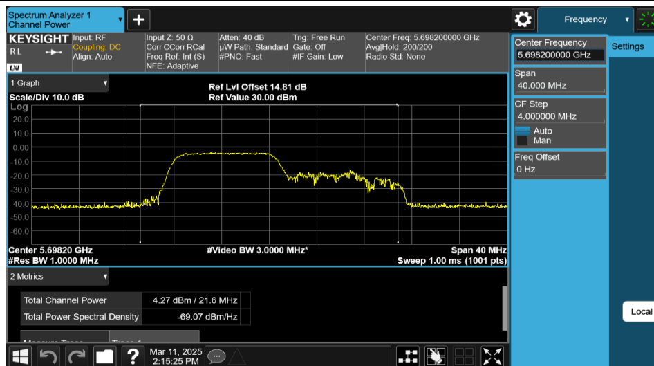
11AX20MIMO-Ant1-5700-106Tone-RU53-PASS
