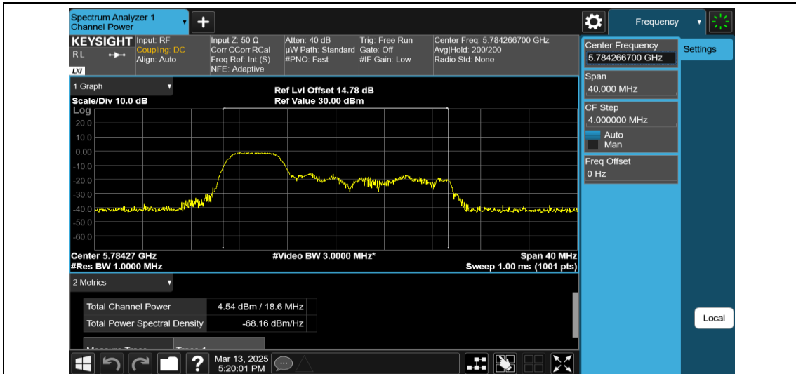
11AX20MIMO-Ant1-5785-52Tone-RU37-PASS
