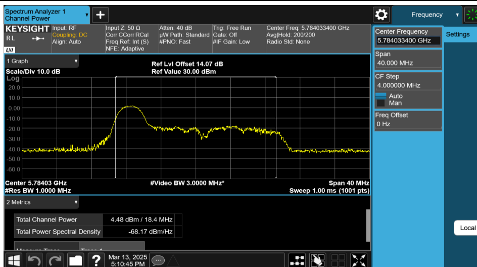
11AX20MIMO-Ant2-5785-26Tone-RU0-PASS
