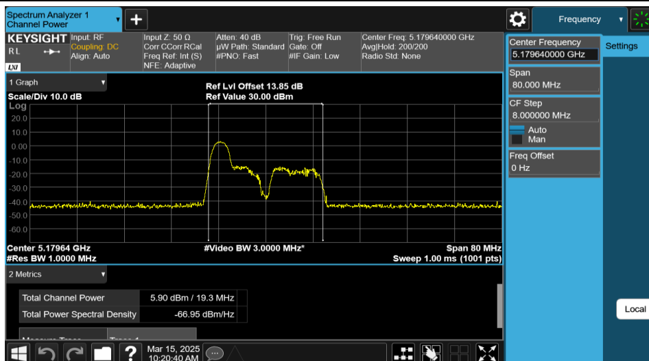
11AX40MIMO-Ant2-5190-26Tone-RU0-PASS
