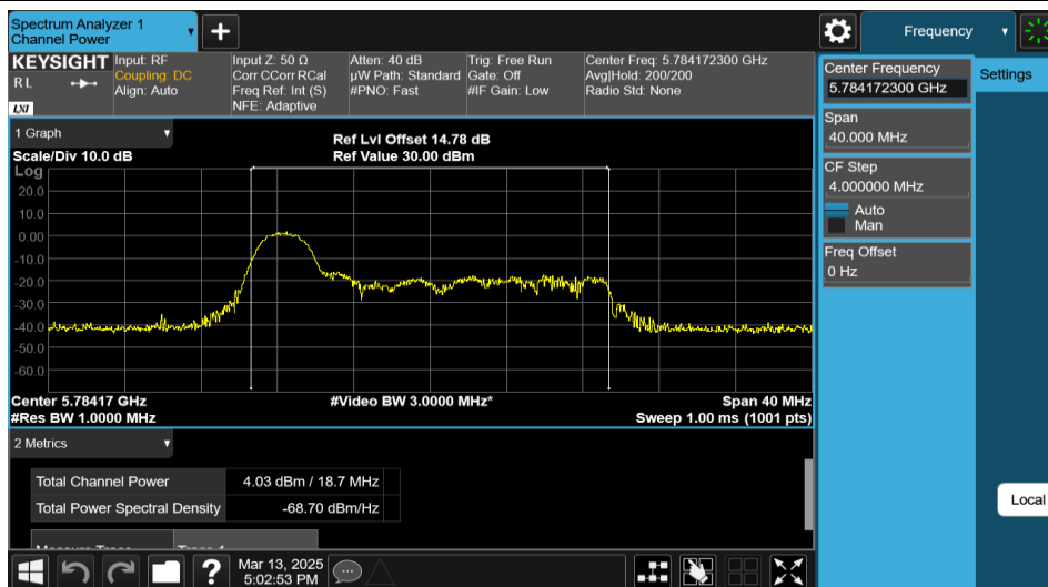
11AX20MIMO-Ant1-5785-26Tone-RU0-PASS
