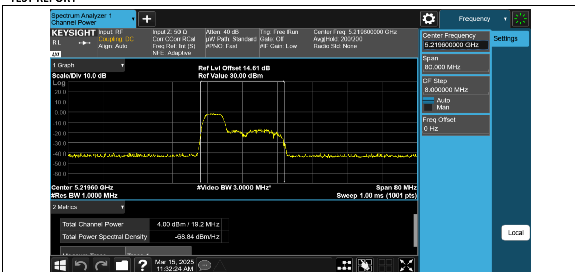
11AX40MIMO-Ant1-5230-52Tone-RU37-PASS
