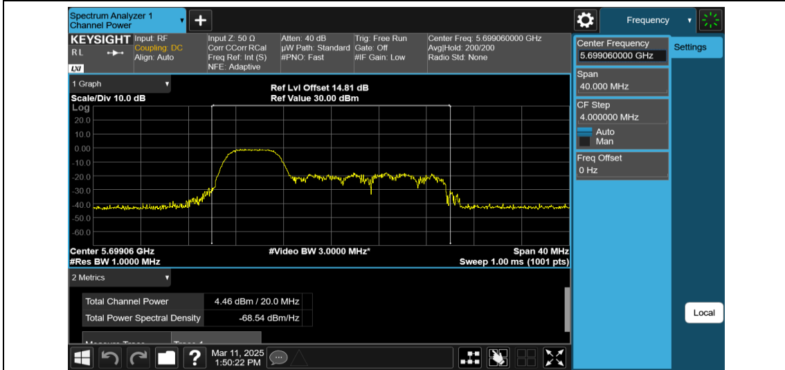
11AX20MIMO-Ant1-5700-52Tone-RU37-PASS
