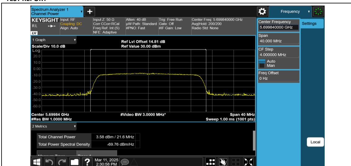
11AX20MIMO-Ant1-5700-242Tone-RU61-PASS
