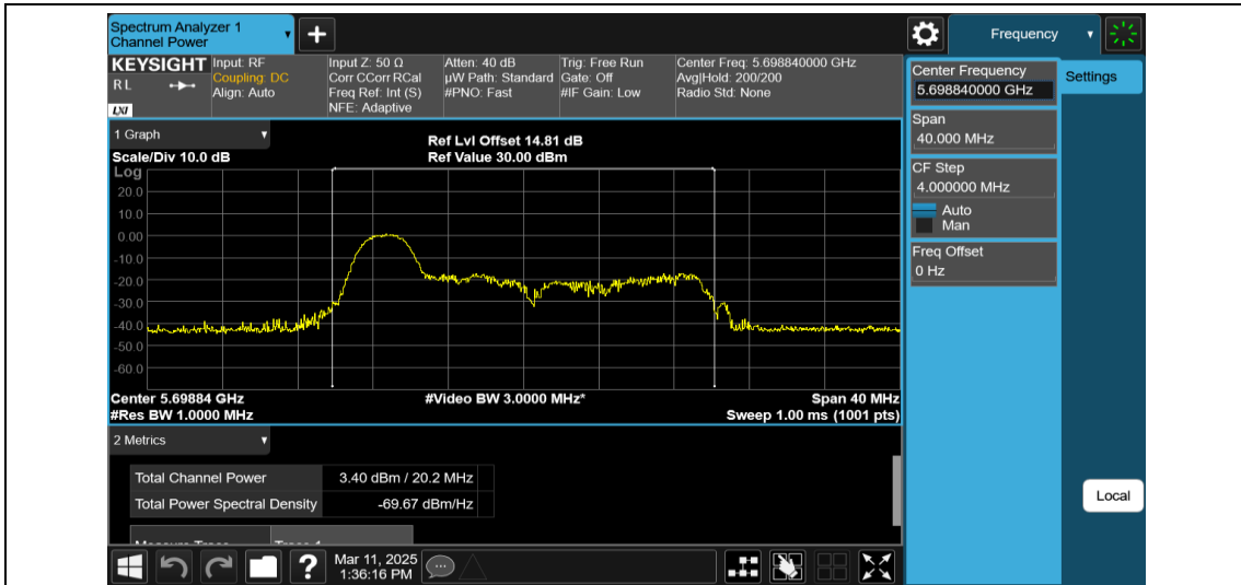
11AX20MIMO-Ant1-5700-26Tone-RU0-PASS
