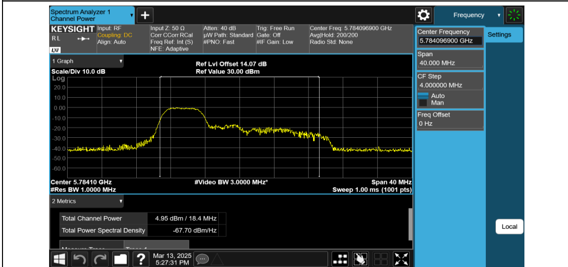
11AX20MIMO-Ant2-5785-52Tone-RU37-PASS
