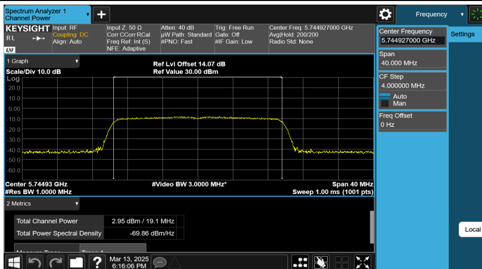
11AX20MIMO-Ant2-5745-242Tone-RU61-PASS
