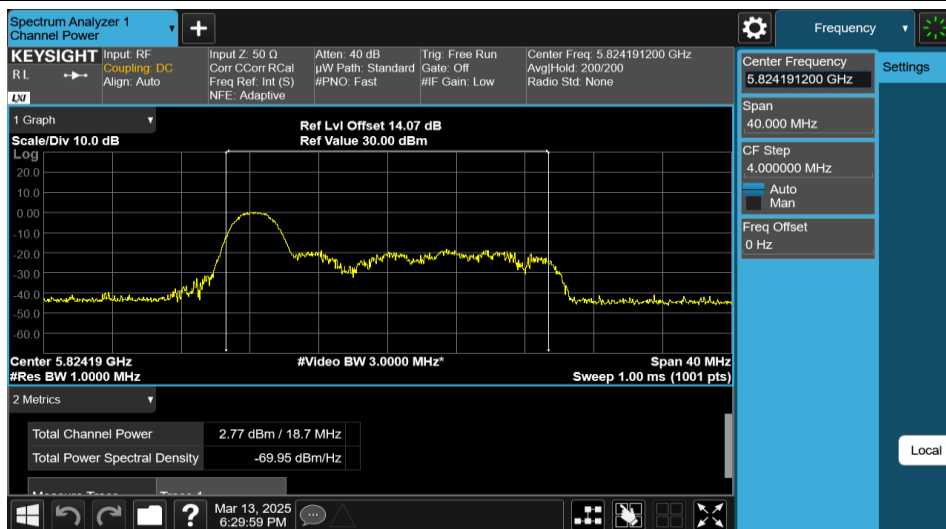
11AX20MIMO-Ant2-5825-26Tone-RU0-PASS
