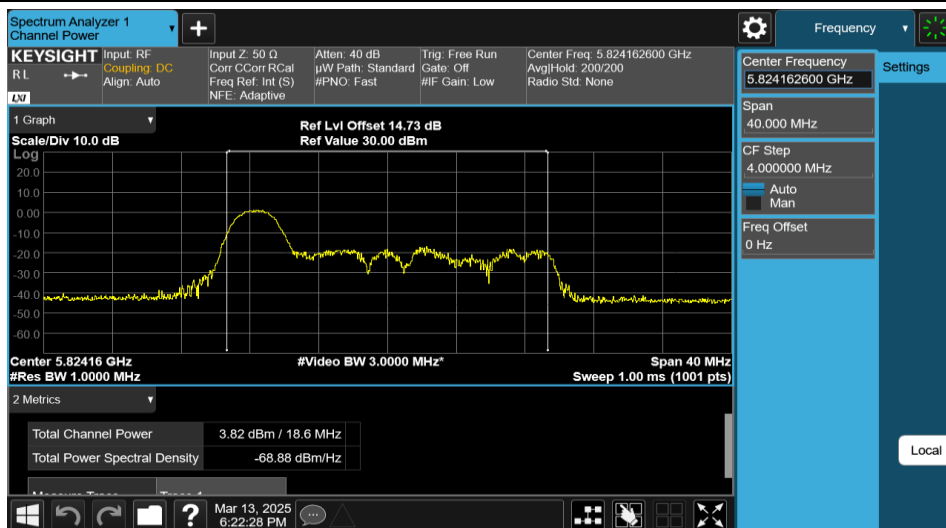
11AX20MIMO-Ant1-5825-26Tone-RU0-PASS
