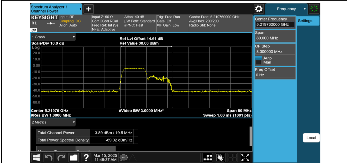
11AX40MIMO-Ant1-5230-106Tone-RU53-PASS
