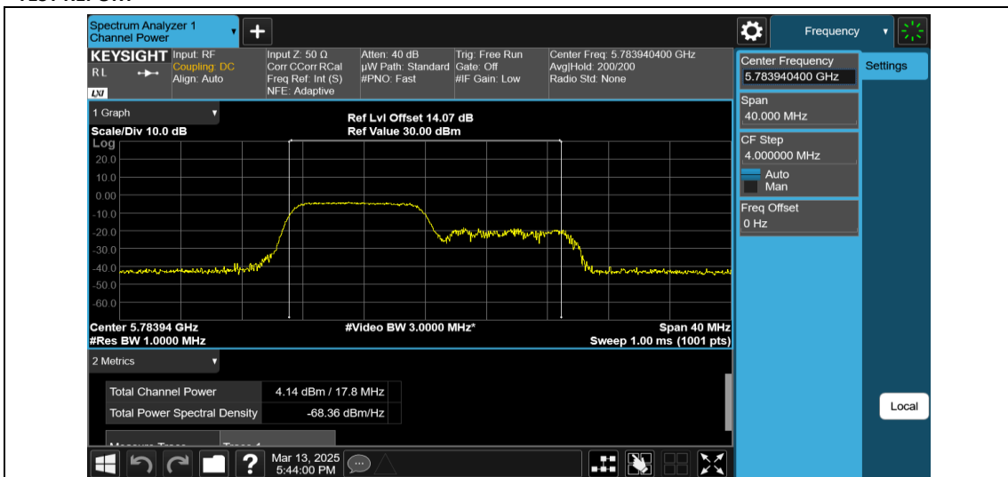
11AX20MIMO-Ant2-5785-106Tone-RU53-PASS
