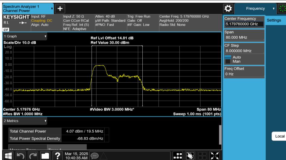
11AX40MIMO-Ant1-5190-52Tone-RU37-PASS
