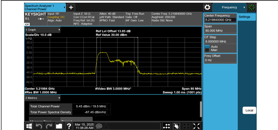
11AX40MIMO-Ant2-5230-52Tone-RU37-PASS
