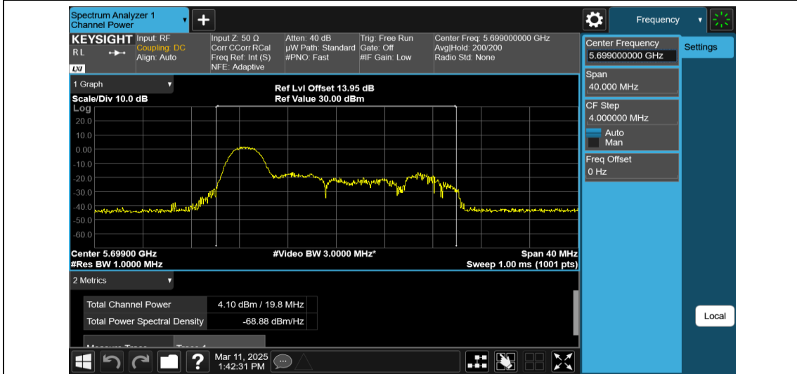
11AX20MIMO-Ant2-5700-26Tone-RU0-PASS
