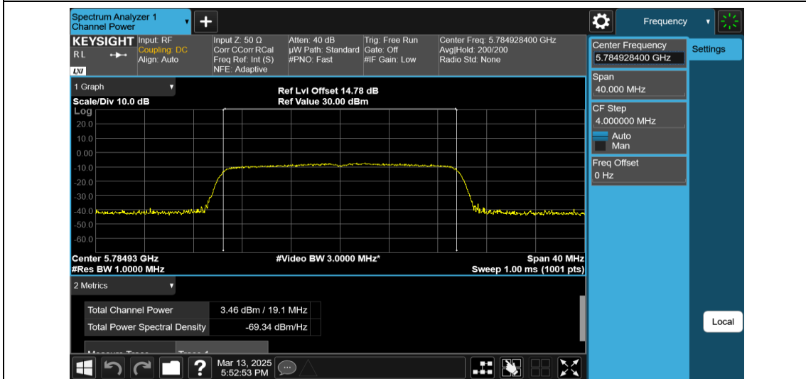
11AX20MIMO-Ant1-5785-242Tone-RU61-PASS
