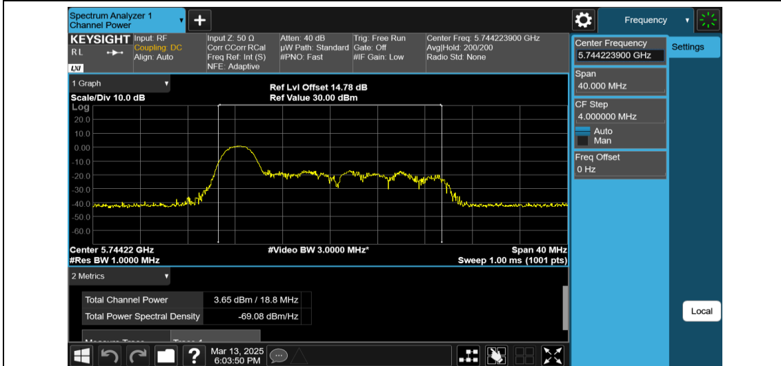
11AX20MIMO-Ant1-5745-26Tone-RU0-PASS
