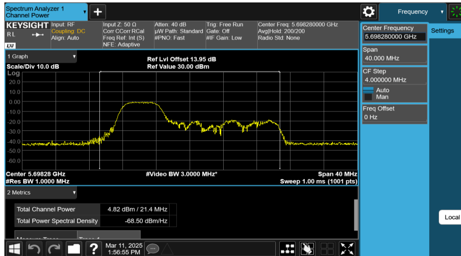
11AX20MIMO-Ant2-5700-52Tone-RU37-PASS
