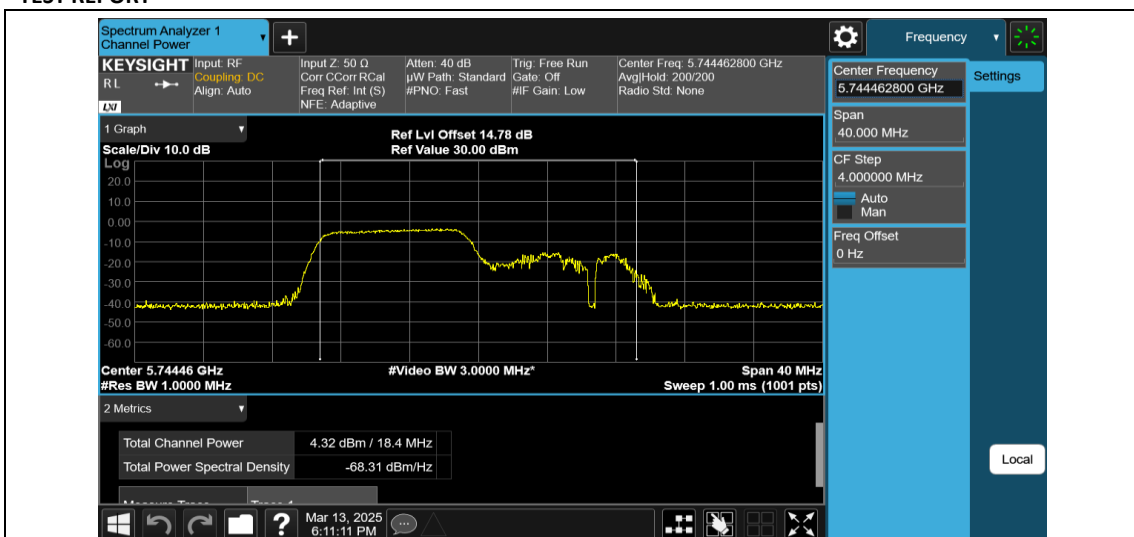
11AX20MIMO-Ant1-5745-106Tone-RU53-PASS
