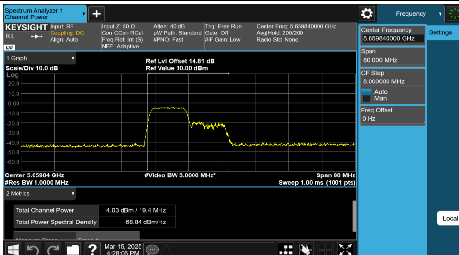
11AX40MIMO-Ant1-5670-106Tone-RU53-PASS
