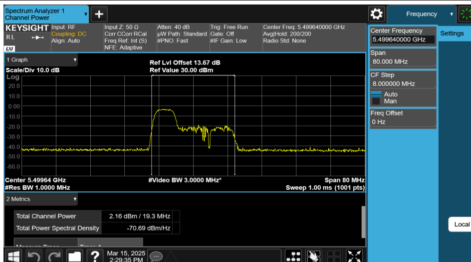
11AX40MIMO-Ant2-5510-52Tone-RU37-PASS
