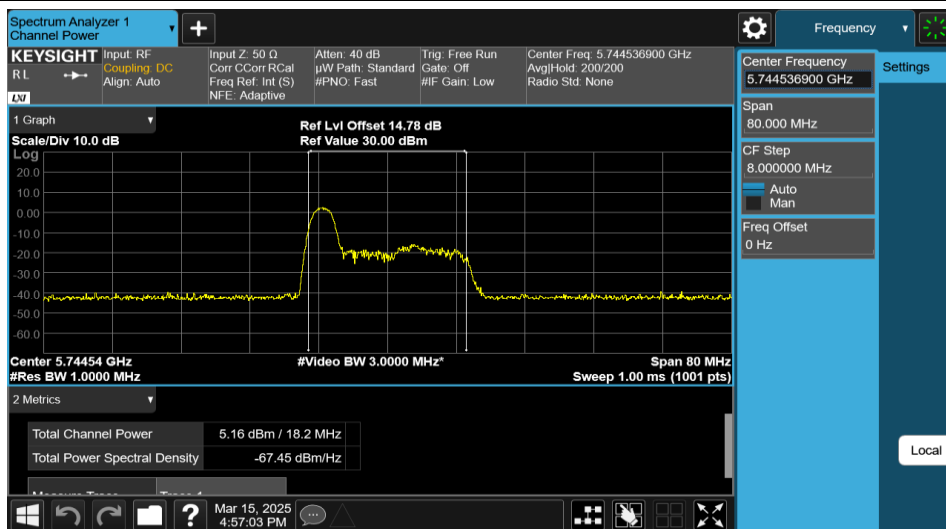
11AX40MIMO-Ant1-5755-26Tone-RU0-PASS
