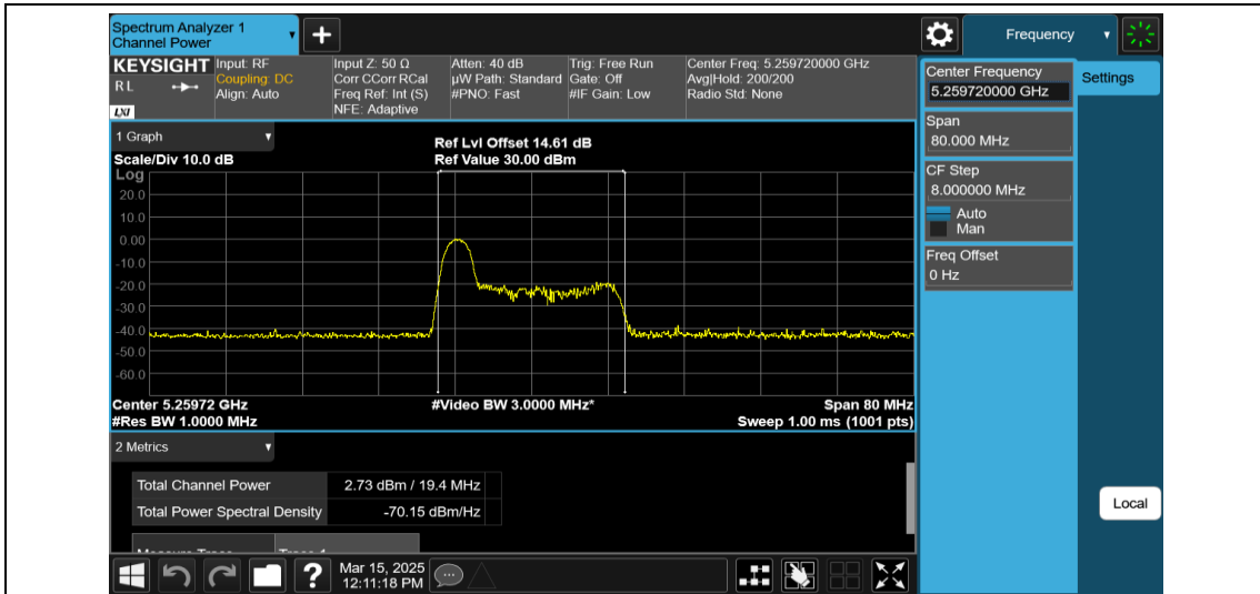
11AX40MIMO-Ant1-5270-26Tone-RU0-PASS
