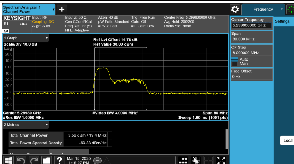
11AX40MIMO-Ant1-5310-52Tone-RU37-PASS
