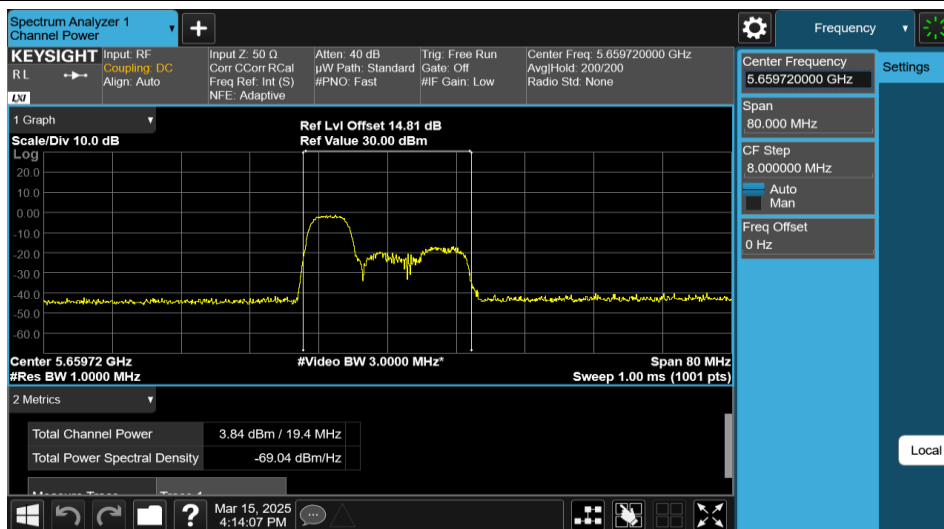
11AX40MIMO-Ant1-5670-52Tone-RU37-PASS
