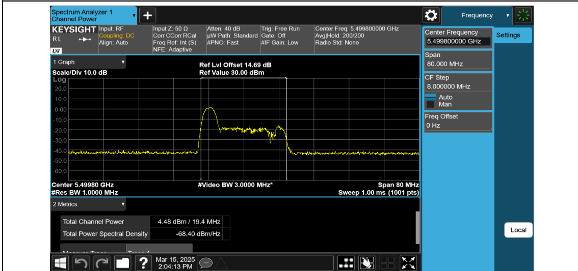
11AX40MIMO-Ant1-5510-26Tone-RU0-PASS
