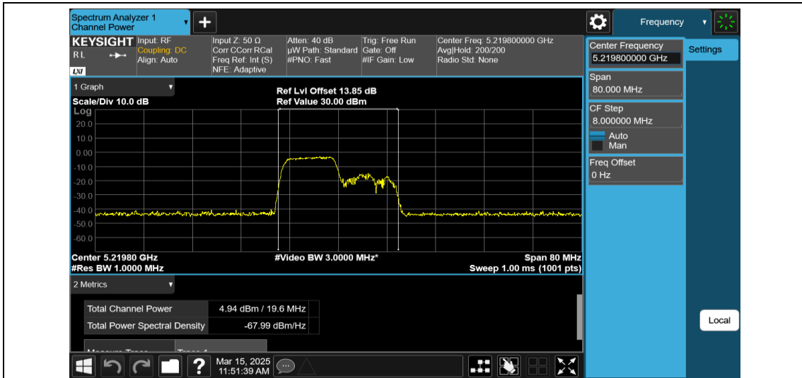
11AX40MIMO-Ant2-5230-106Tone-RU53-PASS
