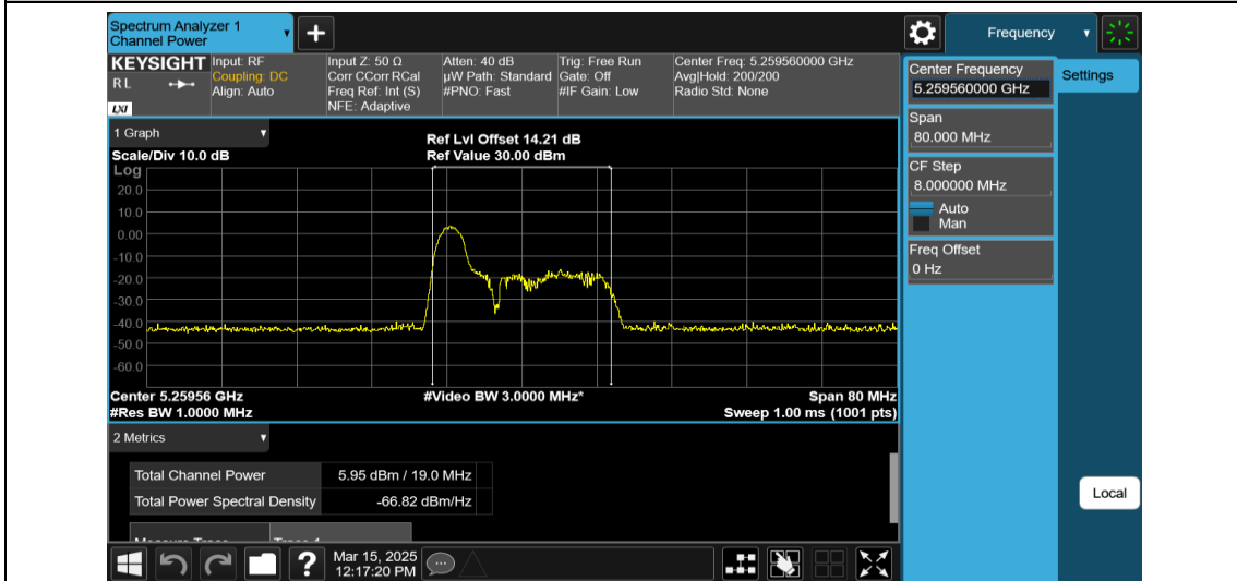
11AX40MIMO-Ant2-5270-26Tone-RU0-PASS
