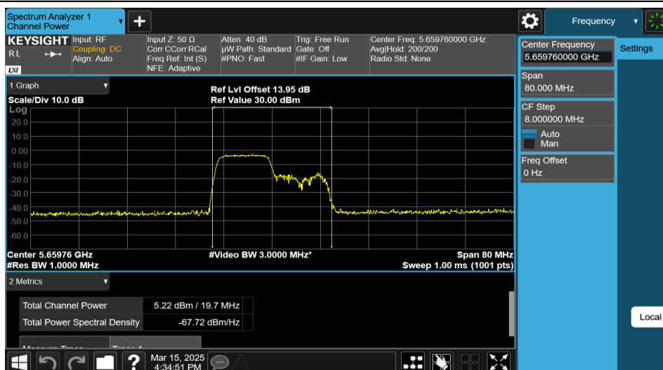
11AX40MIMO-Ant2-5670-106Tone-RU53-PASS
