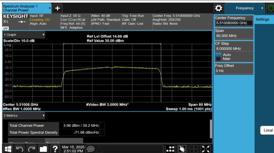
11AX40MIMO-Ant1-5510-484Tone-RU65-PASS
