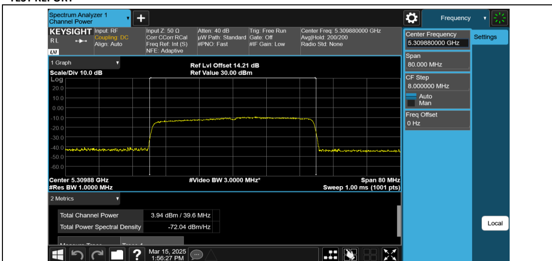
11AX40MIMO-Ant2-5310-484Tone-RU65-PASS
