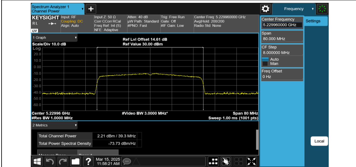
11AX40MIMO-Ant1-5230-484Tone-RU65-PASS
