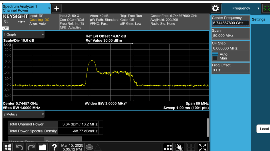
11AX40MIMO-Ant2-5755-26Tone-RU0-PASS
