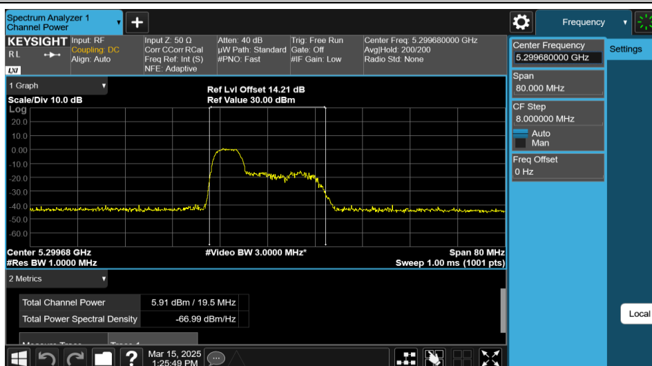
11AX40MIMO-Ant2-5310-52Tone-RU37-PASS
