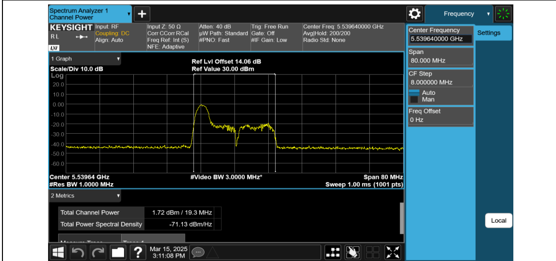
11AX40MIMO-Ant2-5550-26Tone-RU0-PASS
