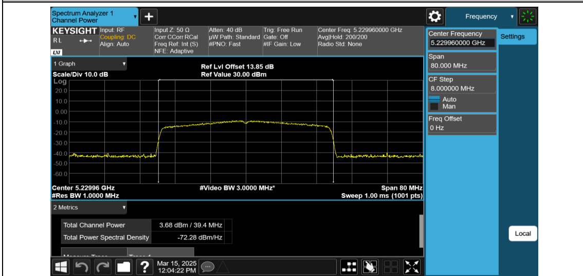
11AX40MIMO-Ant2-5230-484Tone-RU65-PASS
