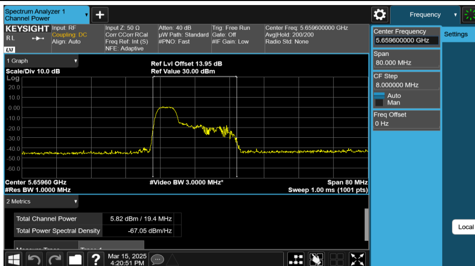
11AX40MIMO-Ant2-5670-52Tone-RU37-PASS
