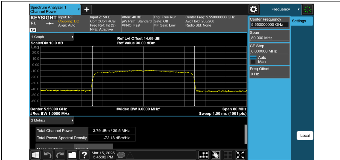
11AX40MIMO-Ant1-5550-484Tone-RU65-PASS
