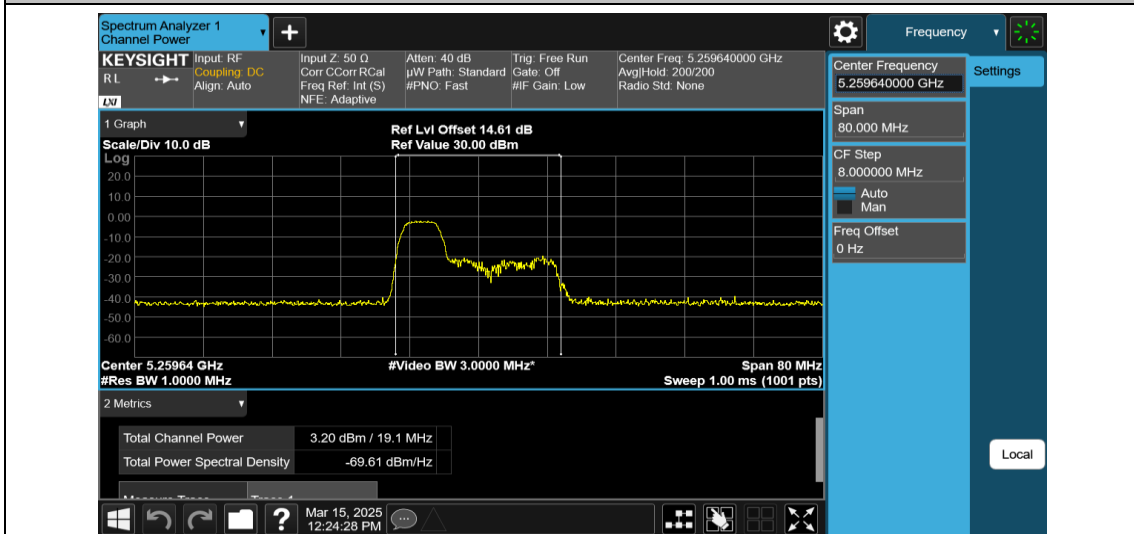
11AX40MIMO-Ant1-5270-52Tone-RU37-PASS
