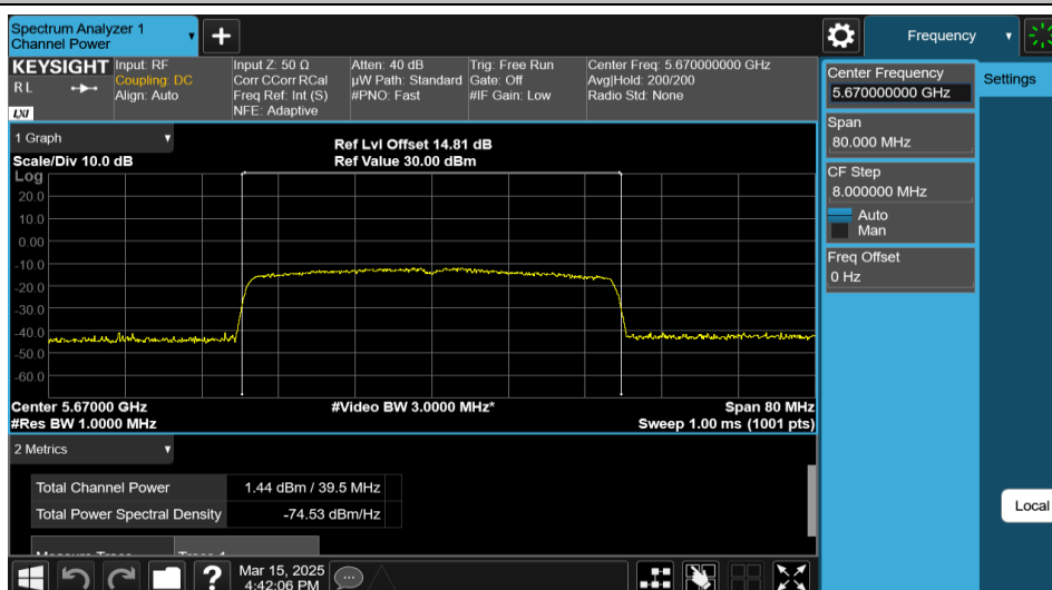
11AX40MIMO-Ant1-5670-484Tone-RU65-PASS
