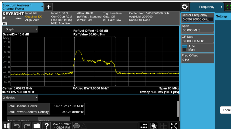
11AX40MIMO-Ant2-5670-26Tone-RU0-PASS
