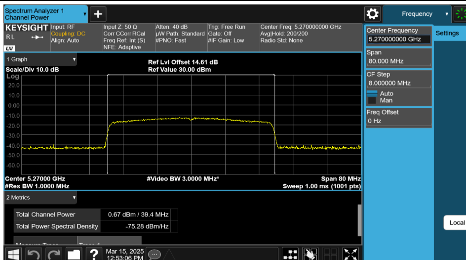
11AX40MIMO-Ant1-5270-484Tone-RU65-PASS
