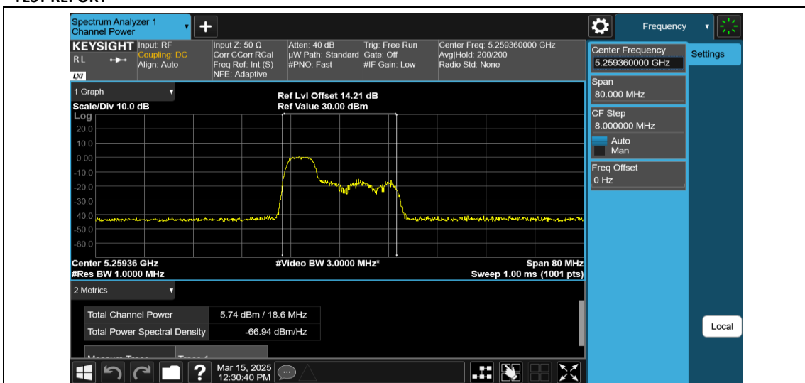
11AX40MIMO-Ant2-5270-52Tone-RU37-PASS
