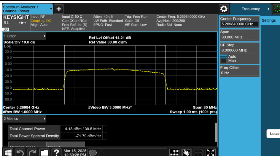
11AX40MIMO-Ant2-5270-484Tone-RU65-PASS
