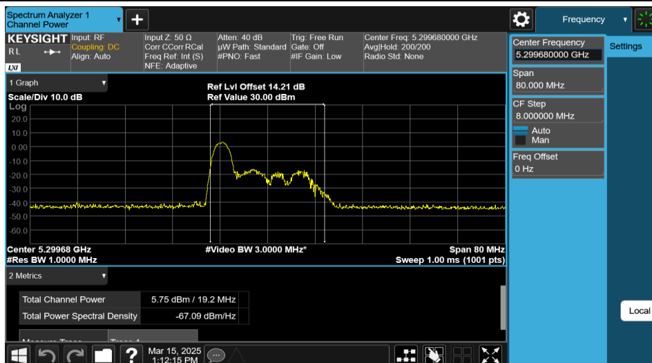
11AX40MIMO-Ant2-5310-26Tone-RU0-PASS
