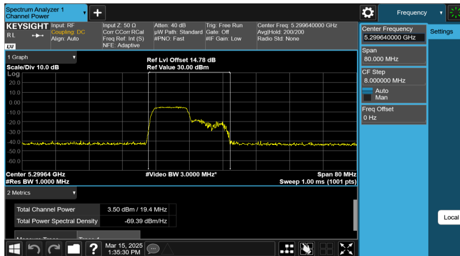
11AX40MIMO-Ant1-5310-106Tone-RU53-PASS
