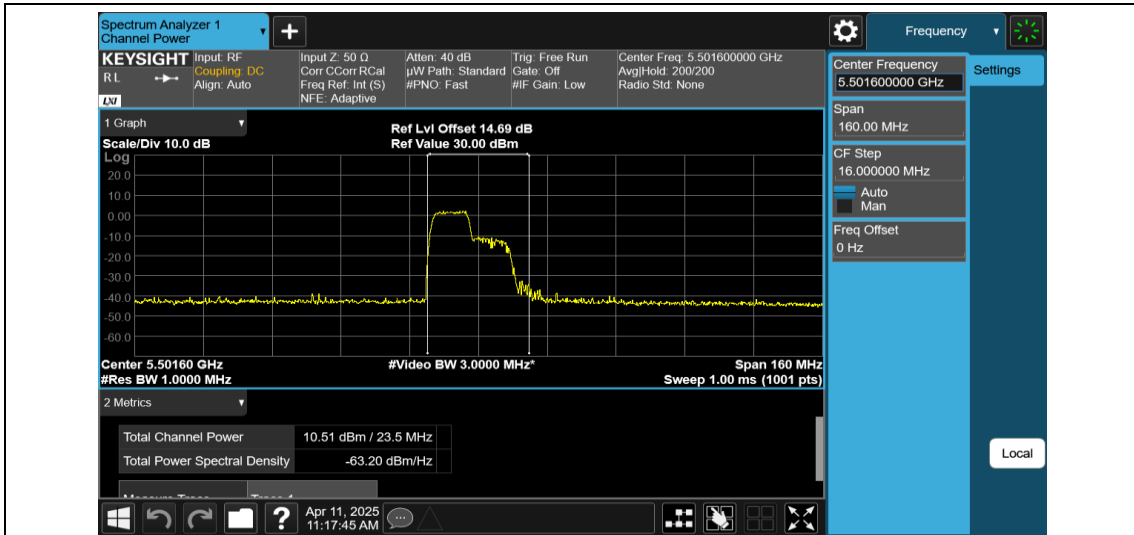
11AX80MIMO-Ant1-5530-106Tone-RU53-PASS
