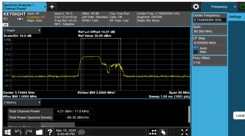
11AX40MIMO-Ant2-5755-106Tone-RU53-PASS
