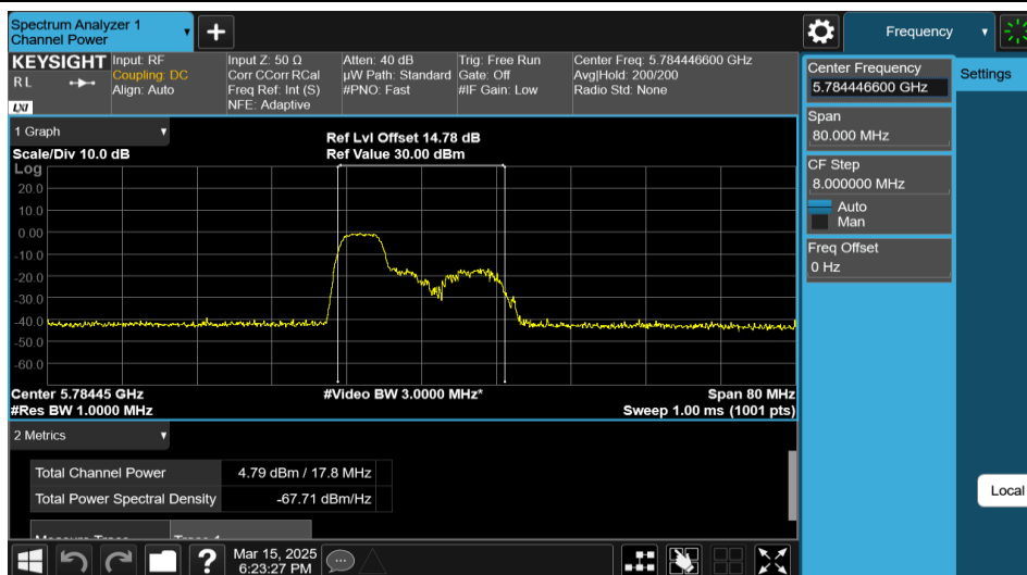
11AX40MIMO-Ant1-5795-52Tone-RU37-PASS
