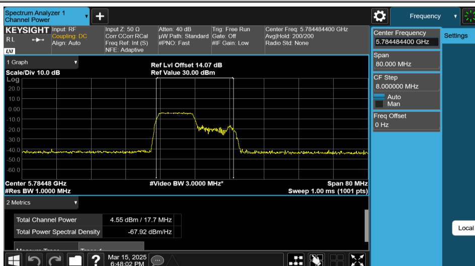
11AX40MIMO-Ant2-5795-106Tone-RU53-PASS
