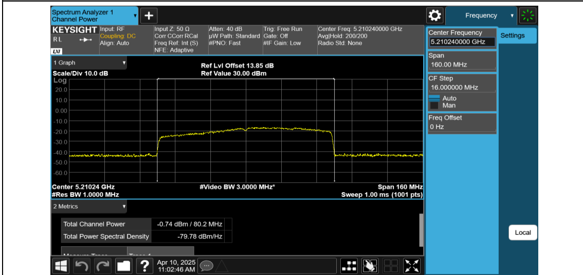
11AX80MIMO-Ant2-5210-996Tone-RU67-PASS
