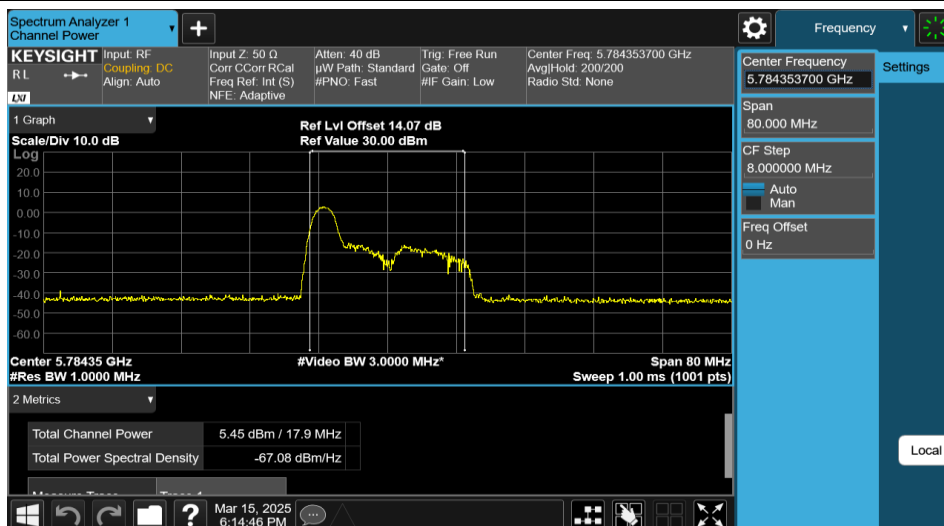
11AX40MIMO-Ant2-5795-26Tone-RU0-PASS
