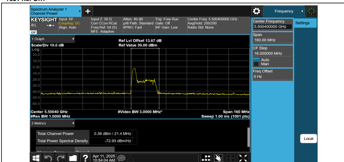
11AX80MIMO-Ant2-5530-26Tone-RU0-PASS
