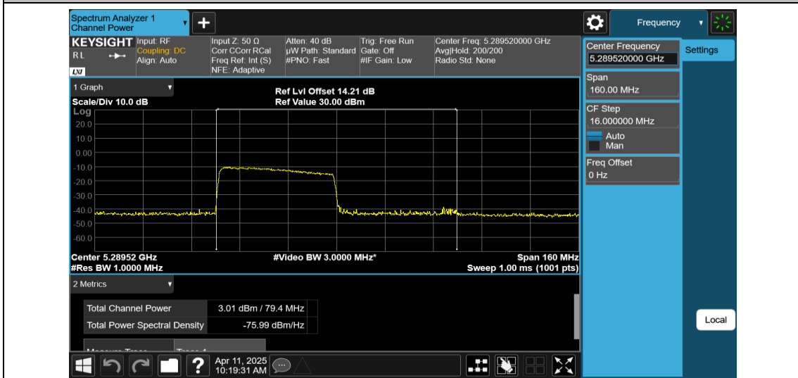
11AX80MIMO-Ant2-5290-484Tone-RU65-PASS
