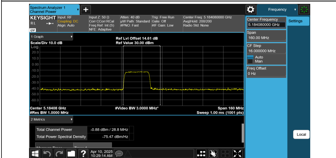
11AX80MIMO-Ant1-5210-242Tone-RU61-PASS
