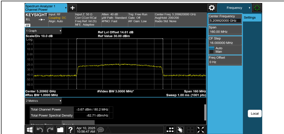
11AX80MIMO-Ant1-5210-996Tone-RU67-PASS
