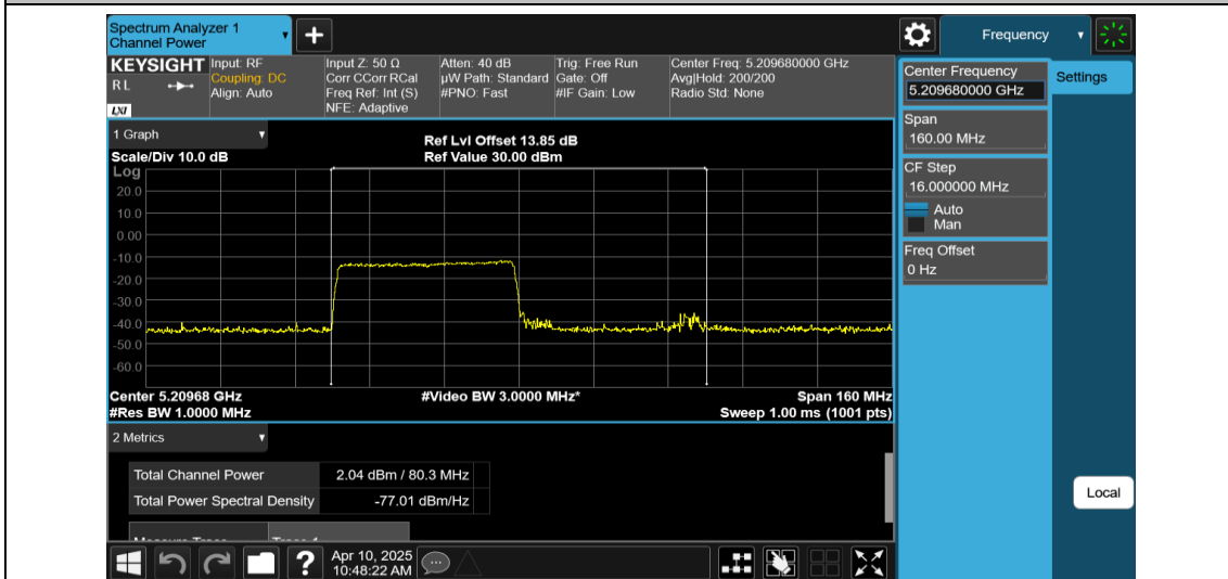
11AX80MIMO-Ant2-5210-484Tone-RU65-PASS
