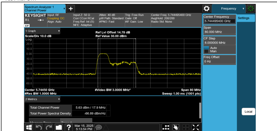
11AX40MIMO-Ant1-5755-52Tone-RU37-PASS
