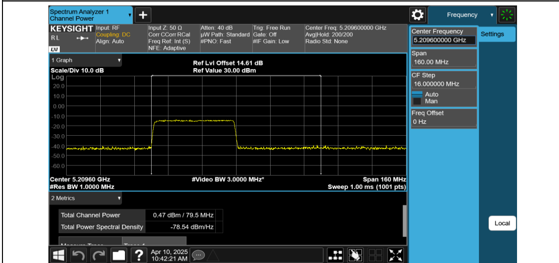
11AX80MIMO-Ant1-5210-484Tone-RU65-PASS
