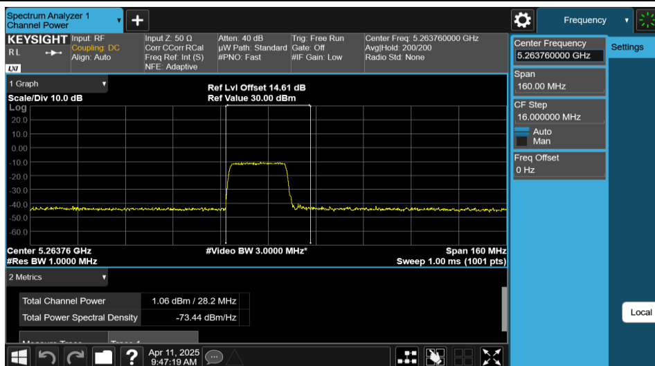
11AX80MIMO-Ant1-5290-242Tone-RU61-PASS
