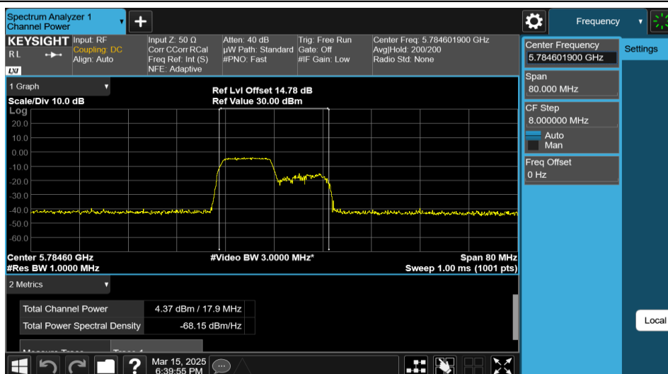
11AX40MIMO-Ant1-5795-106Tone-RU53-PASS
