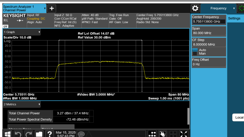
11AX40MIMO-Ant2-5755-484Tone-RU65-PASS
