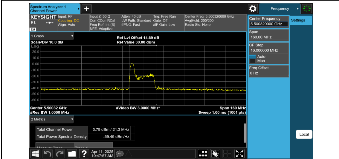
11AX80MIMO-Ant1-5530-26Tone-RU0-PASS
