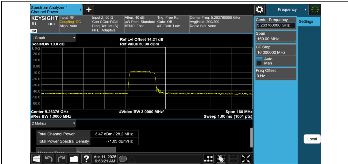
11AX80MIMO-Ant2-5290-242Tone-RU61-PASS
