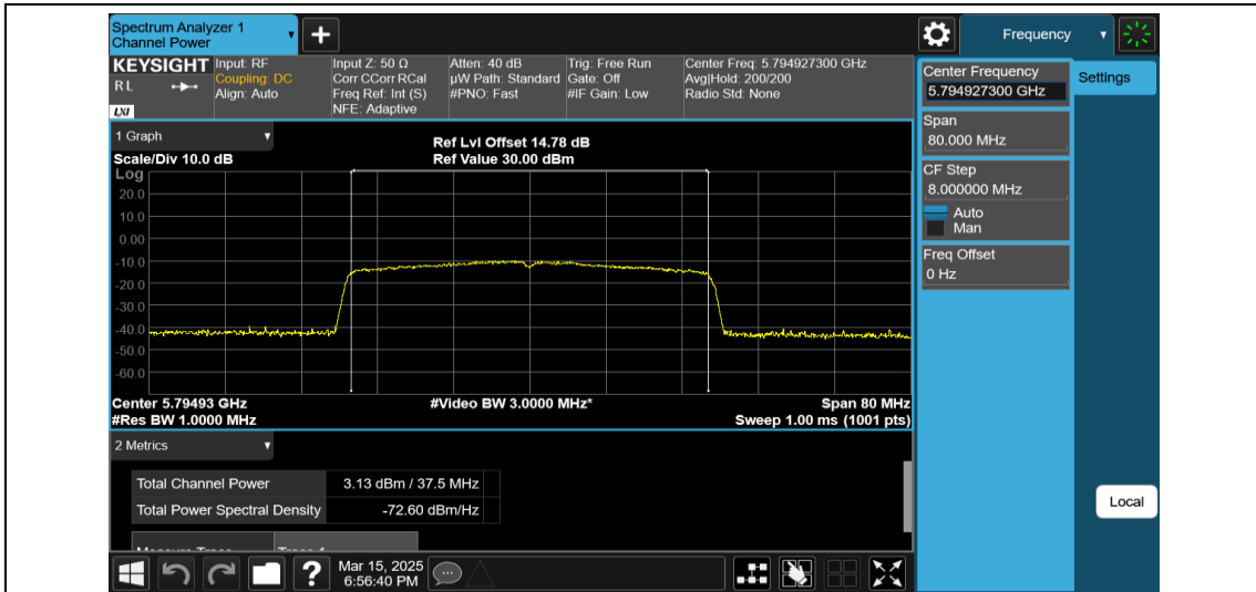
11AX40MIMO-Ant1-5795-484Tone-RU65-PASS
