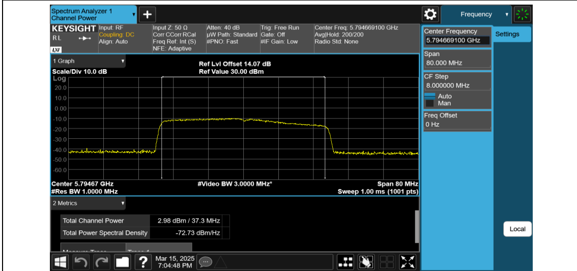
11AX40MIMO-Ant2-5795-484Tone-RU65-PASS
