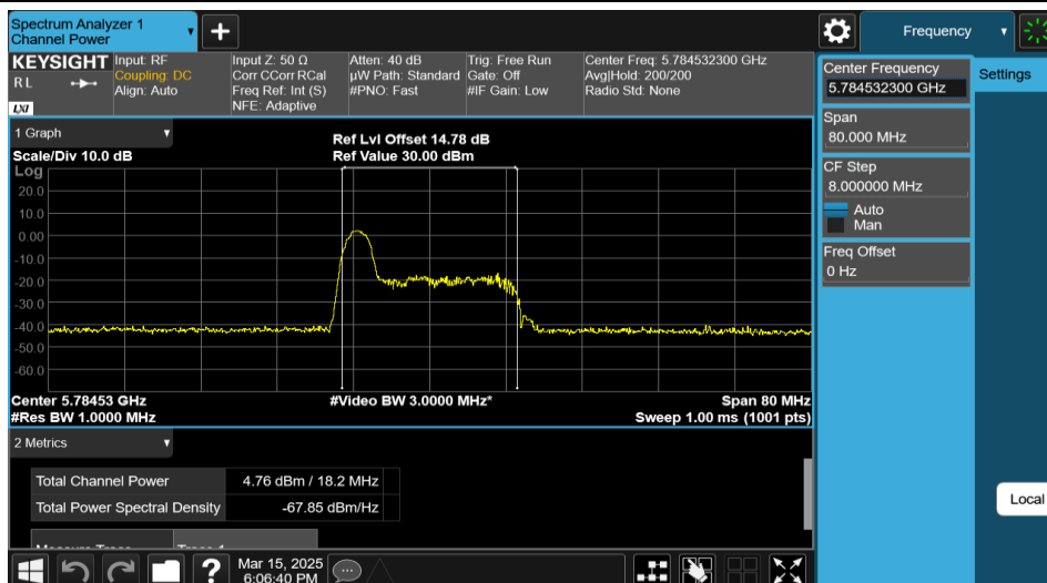
11AX40MIMO-Ant1-5795-26Tone-RU0-PASS
