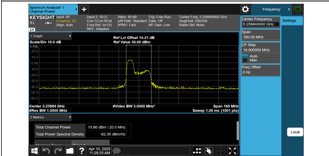
11AX80MIMO-Ant2-5290-52Tone-RU37-PASS
