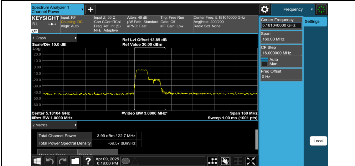
11AX80MIMO-Ant2-5210-106Tone-RU53-PASS
