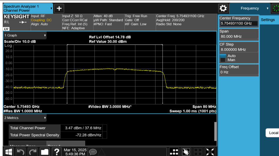
11AX40MIMO-Ant1-5755-484Tone-RU65-PASS
