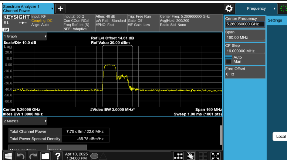
11AX80MIMO-Ant1-5290-106Tone-RU53-PASS
