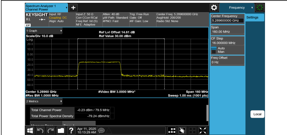
11AX80MIMO-Ant1-5290-484Tone-RU65-PASS
