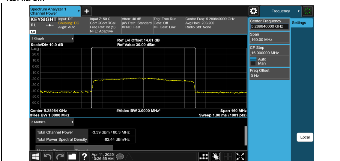
11AX80MIMO-Ant1-5290-996Tone-RU67-PASS
