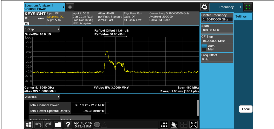
11AX80MIMO-Ant1-5210-26Tone-RU0-PASS
