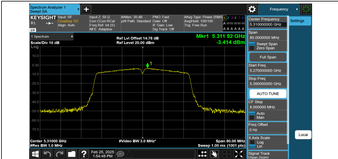
11N40MIMO-Ant1-5310-PASS
