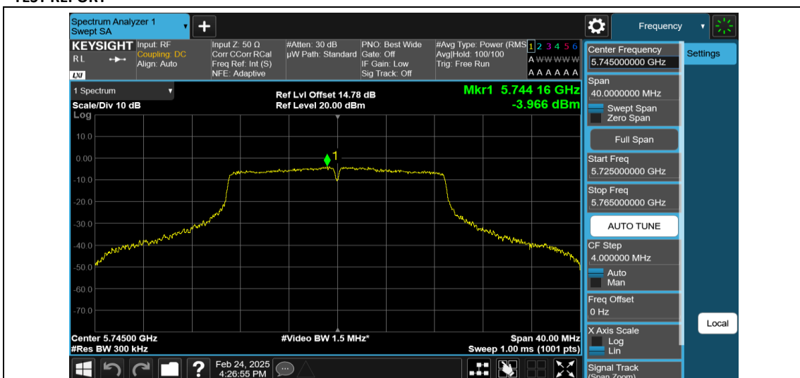
11N20MIMO-Ant1-5745-PASS
