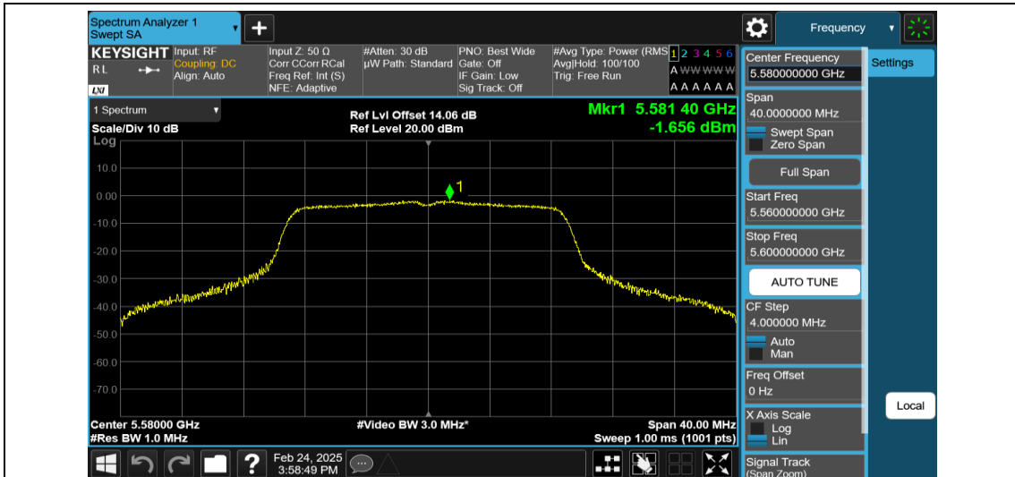
11N20MIMO-Ant2-5580-PASS
