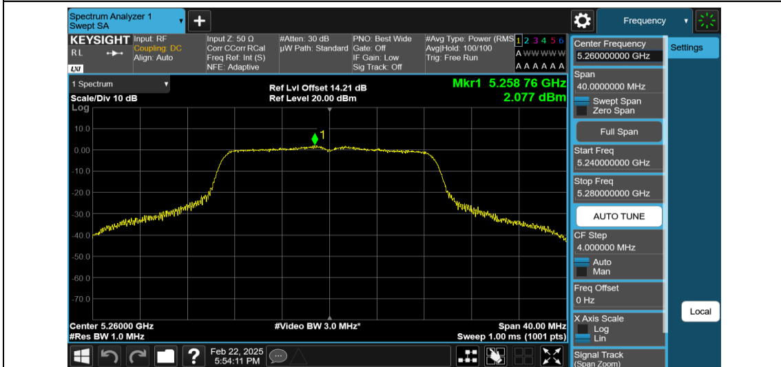
11N20MIMO-Ant2-5260-PASS
