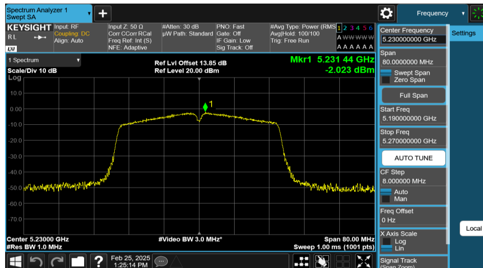
11N40MIMO-Ant2-5230-PASS
