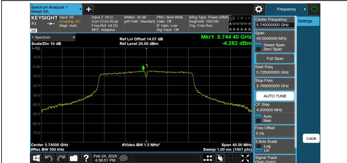
11N20MIMO-Ant2-5745-PASS
