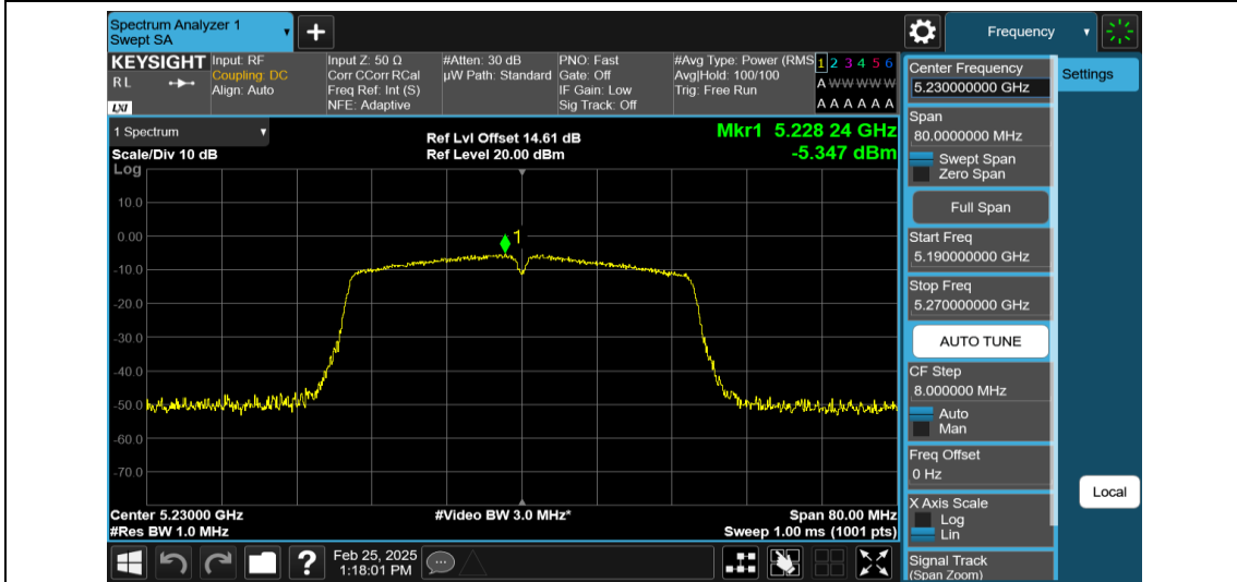
11N40MIMO-Ant1-5230-PASS
