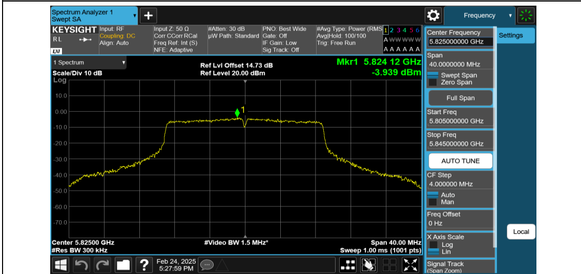
11N20MIMO-Ant1-5825-PASS
