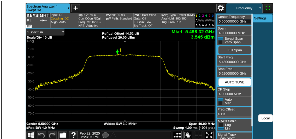
11A-Ant1-5500-PASS
