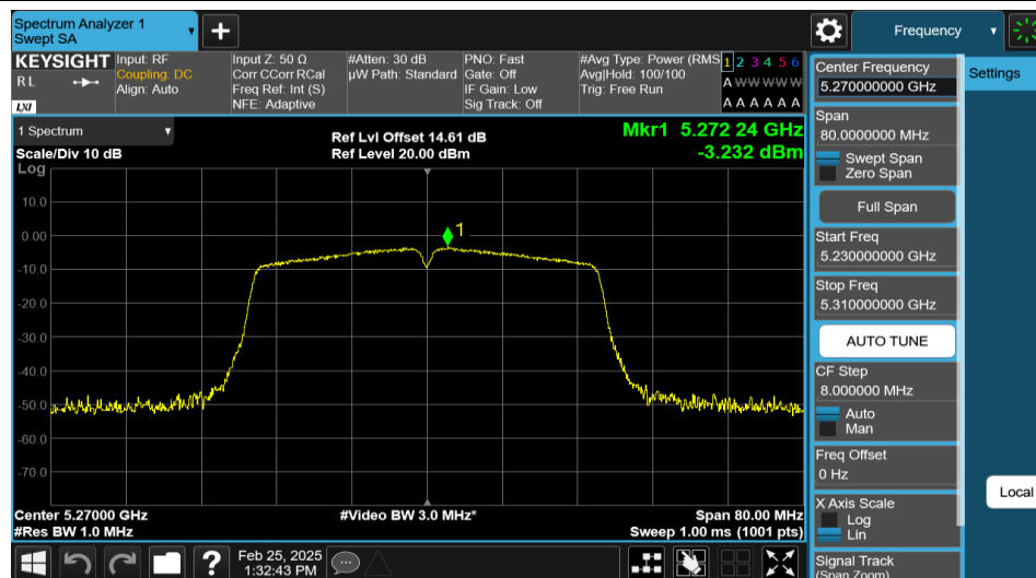
11N40MIMO-Ant1-5270-PASS
