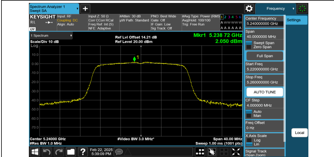
11N20MIMO-Ant2-5240-PASS
