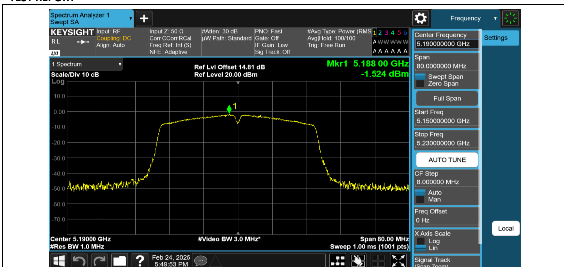
11N40MIMO-Ant1-5190-PASS
