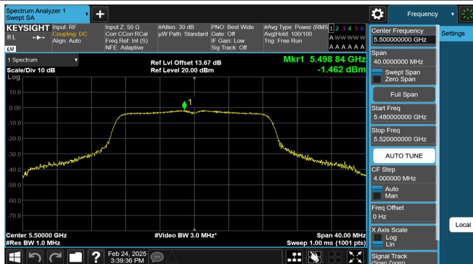
11N20MIMO-Ant2-5500-PASS
