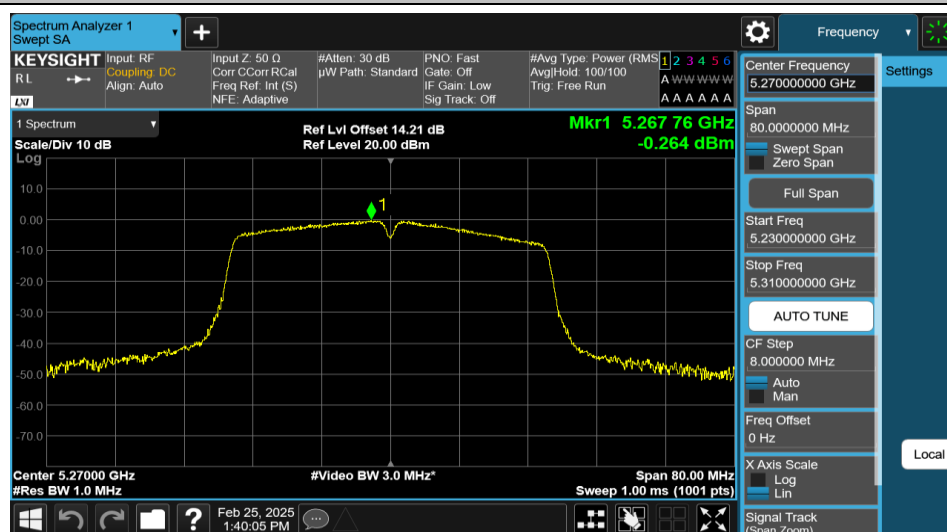
11N40MIMO-Ant2-5270-PASS
