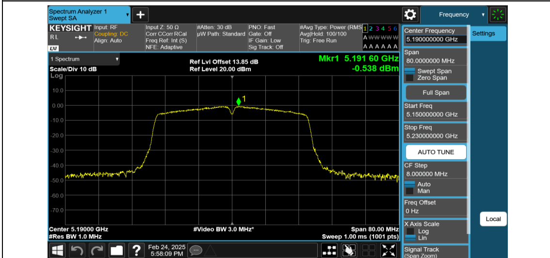
11N40MIMO-Ant2-5190-PASS
