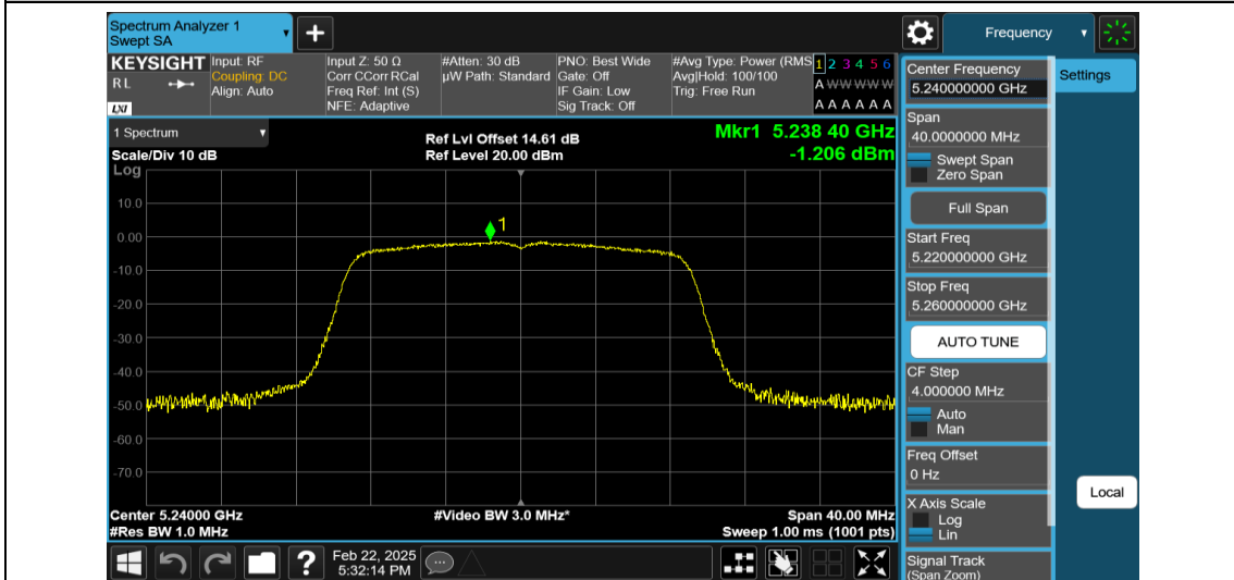
11N20MIMO-Ant1-5240-PASS
