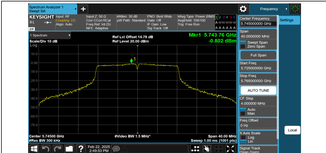
11A-Ant1-5745-PASS
