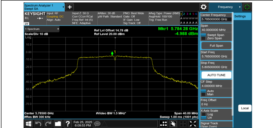
11AC20MIMO-Ant1-5785-PASS
