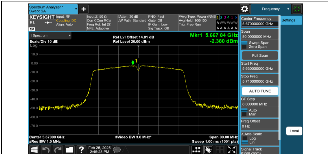
11N40MIMO-Ant1-5670-PASS
