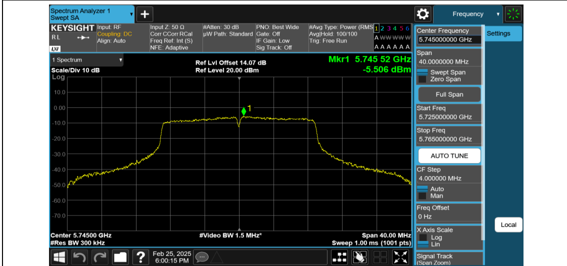
11AC20MIMO-Ant2-5745-PASS
