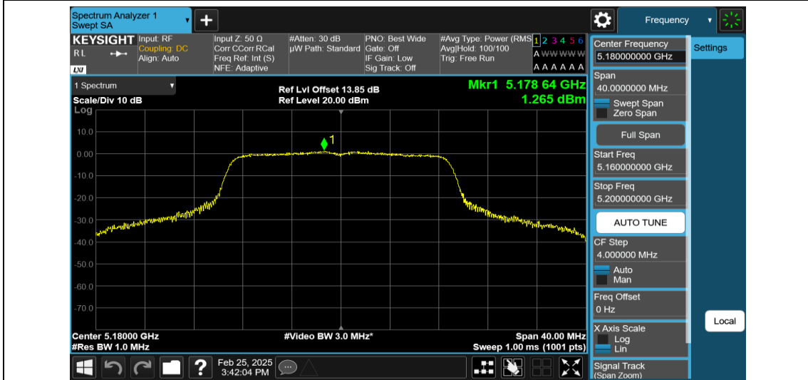
11AC20MIMO-Ant2-5180-PASS
