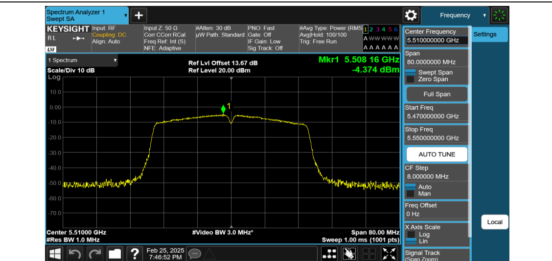
11AC40MIMO-Ant2-5510-PASS
