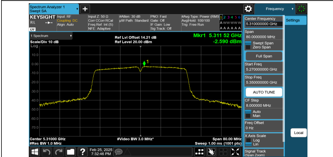
11AC40MIMO-Ant2-5310-PASS
