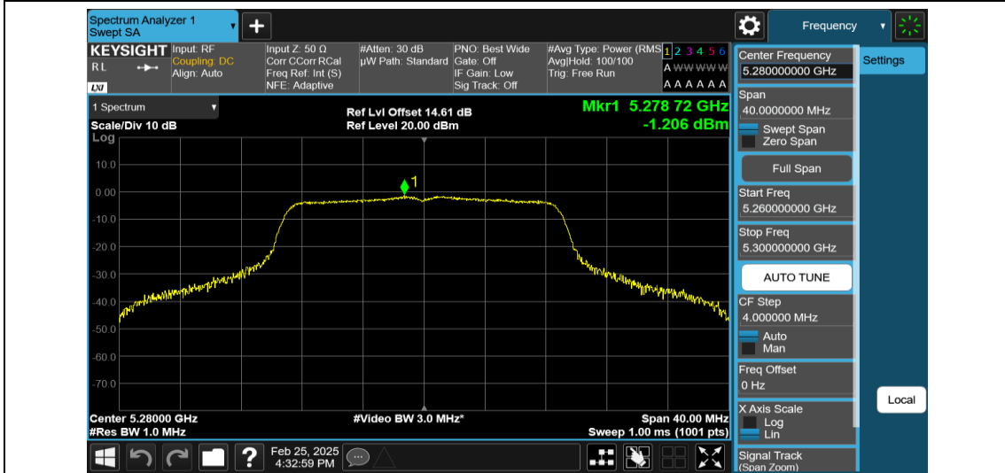
11AC20MIMO-Ant1-5280-PASS
