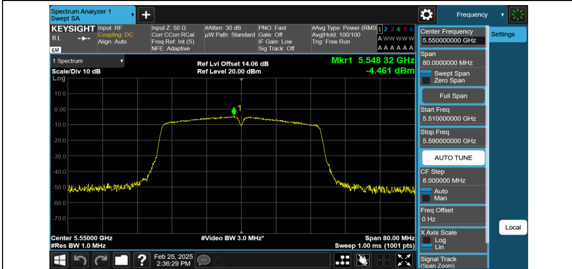
11N40MIMO-Ant2-5550-PASS
