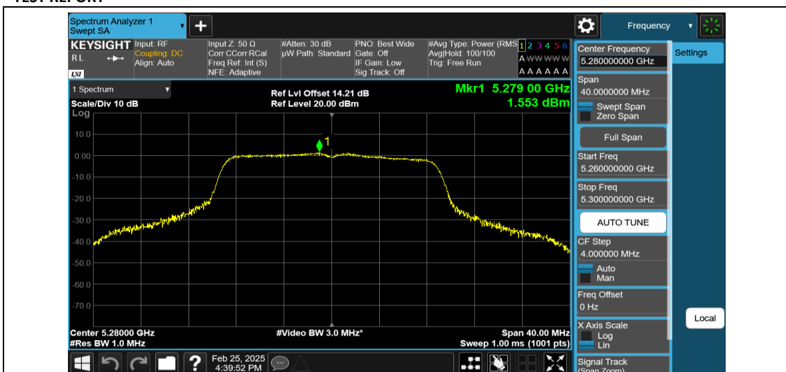
11AC20MIMO-Ant2-5280-PASS
