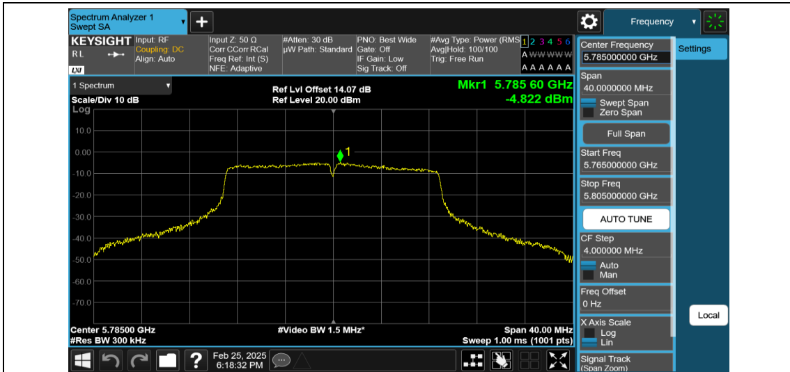
11AC20MIMO-Ant2-5785-PASS
