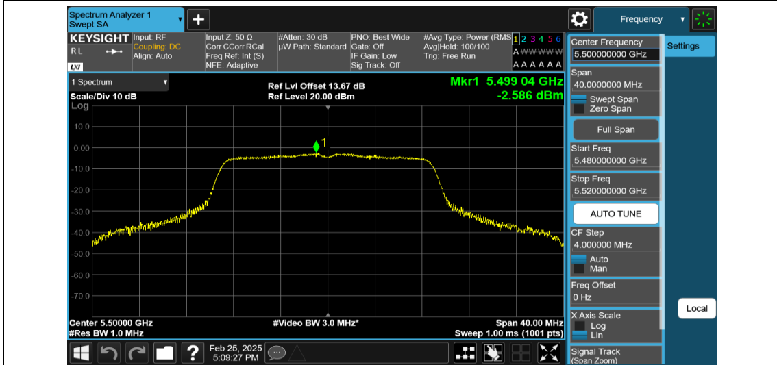
11AC20MIMO-Ant2-5500-PASS
