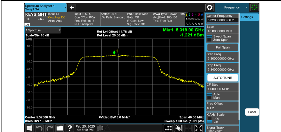
11AC20MIMO-Ant1-5320-PASS
