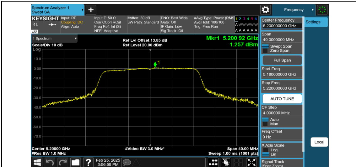
11AC20MIMO-Ant2-5200-PASS
