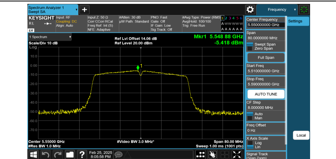
11AC40MIMO-Ant2-5550-PASS
