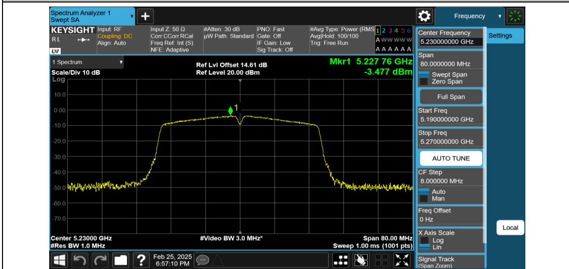
11AC40MIMO-Ant1-5230-PASS
