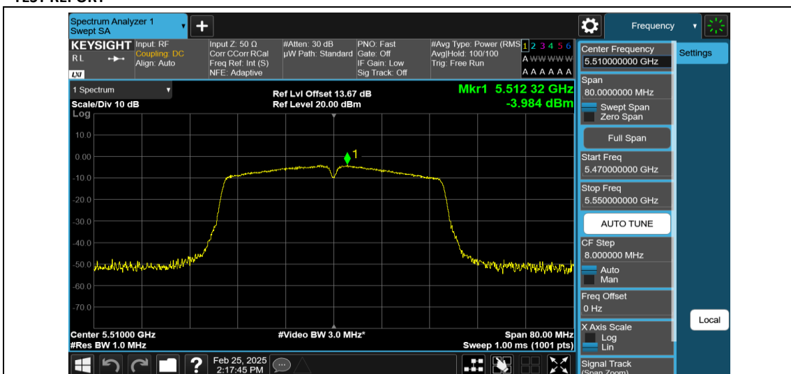
11N40MIMO-Ant2-5510-PASS
