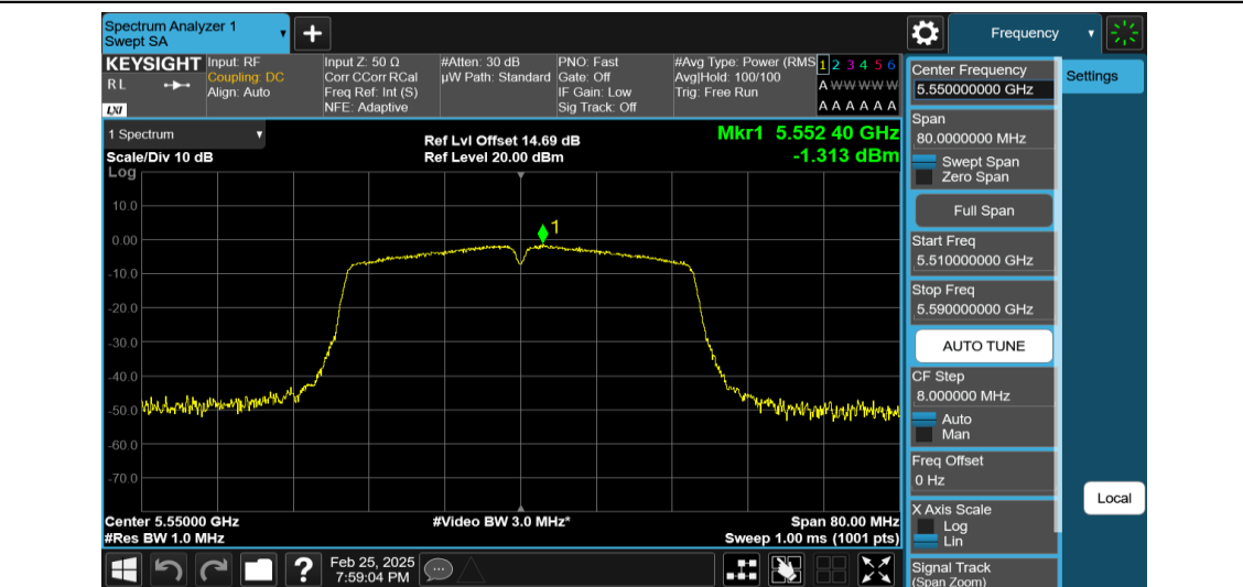
11AC40MIMO-Ant1-5550-PASS
