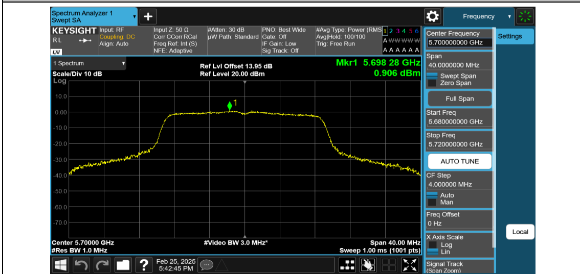
11AC20MIMO-Ant2-5700-PASS
