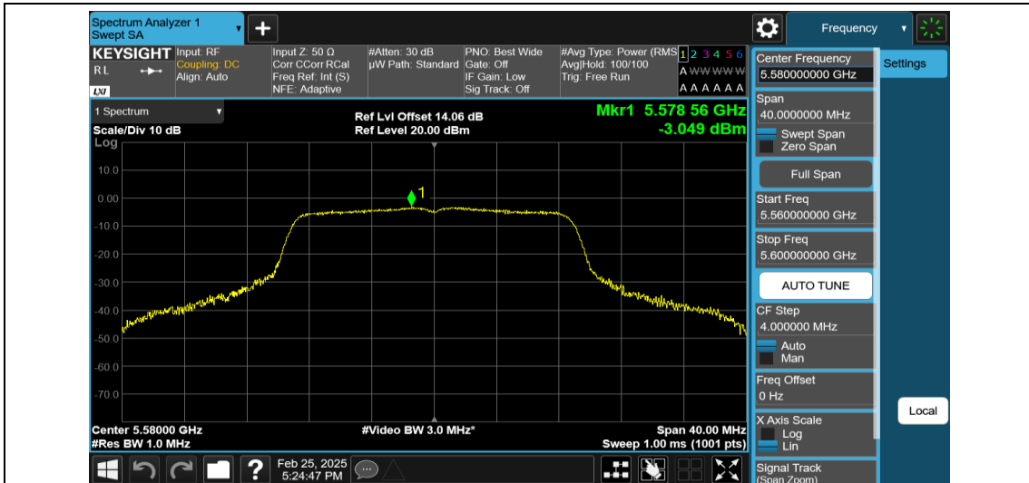
11AC20MIMO-Ant2-5580-PASS
