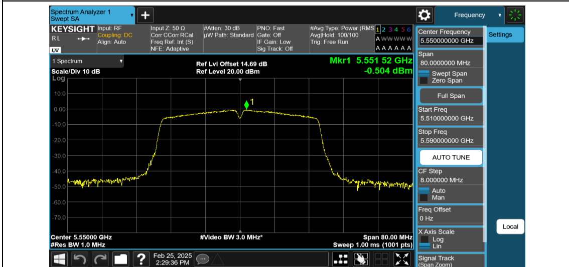
11N40MIMO-Ant1-5550-PASS
