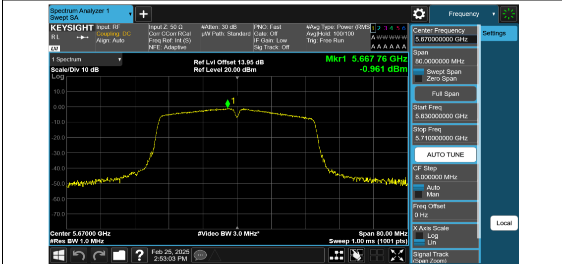
11N40MIMO-Ant2-5670-PASS
