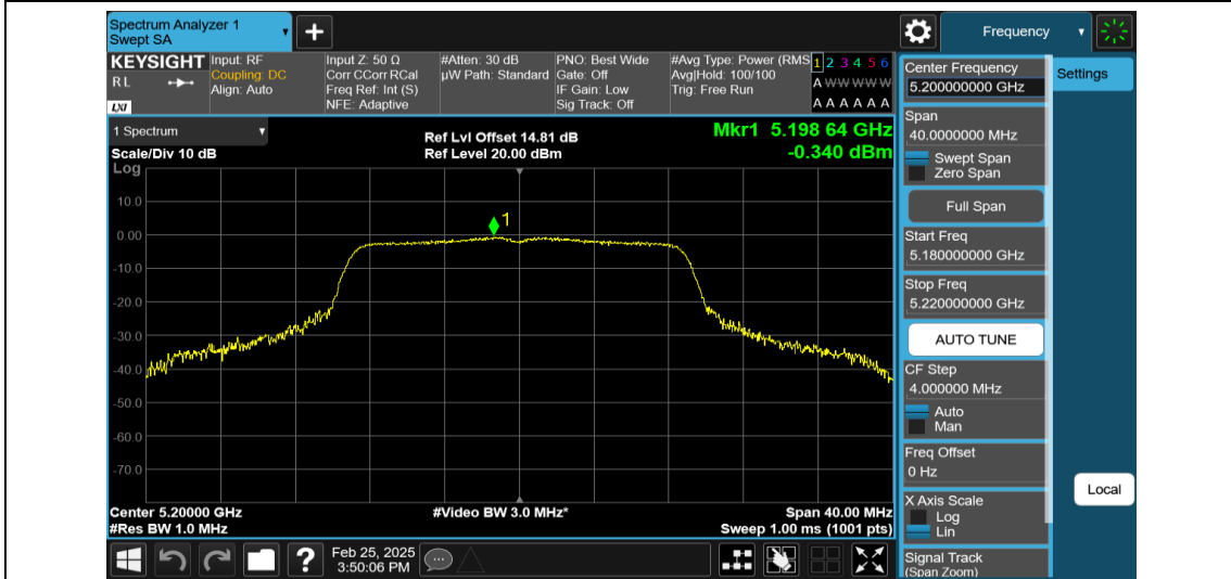
11AC20MIMO-Ant1-5200-PASS
