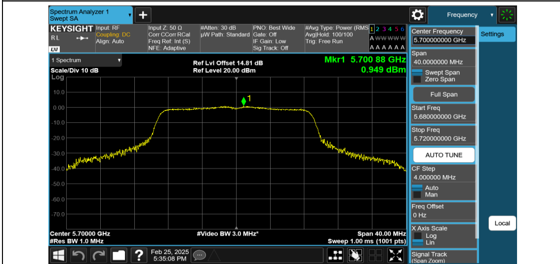
11AC20MIMO-Ant1-5700-PASS
