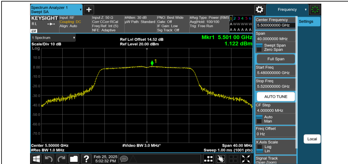
11AC20MIMO-Ant1-5500-PASS
