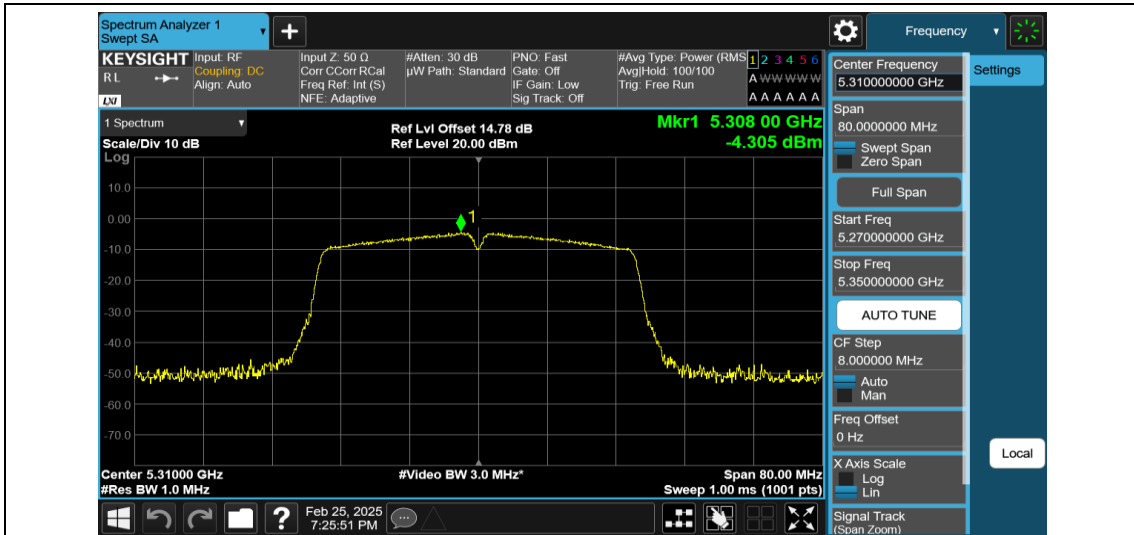
11AC40MIMO-Ant1-5310-PASS
