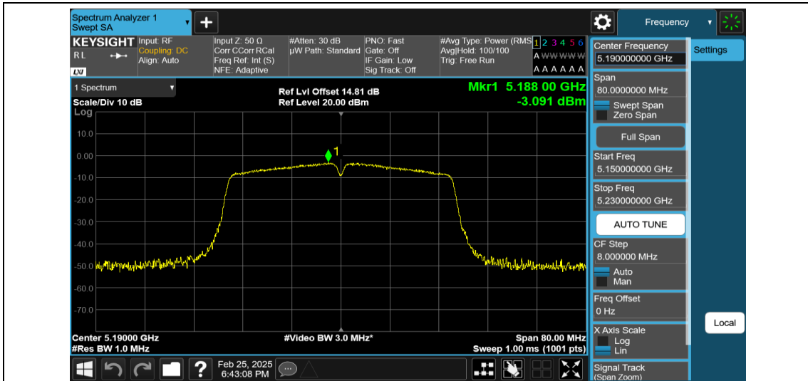
11AC40MIMO-Ant1-5190-PASS
