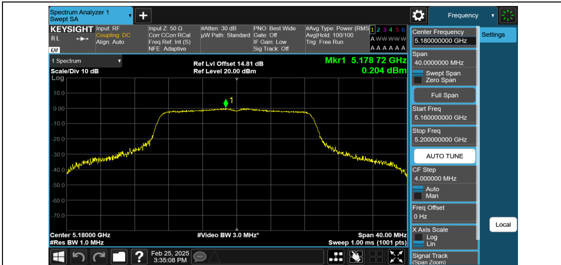
11AC20MIMO-Ant1-5180-PASS
