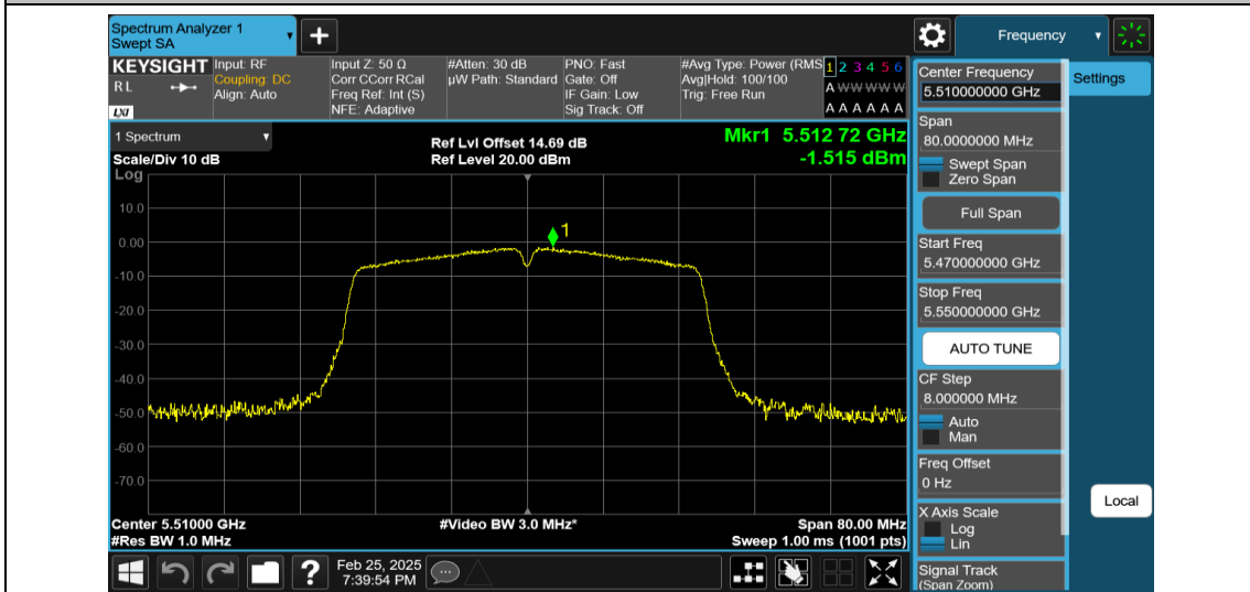
11AC40MIMO-Ant1-5510-PASS
