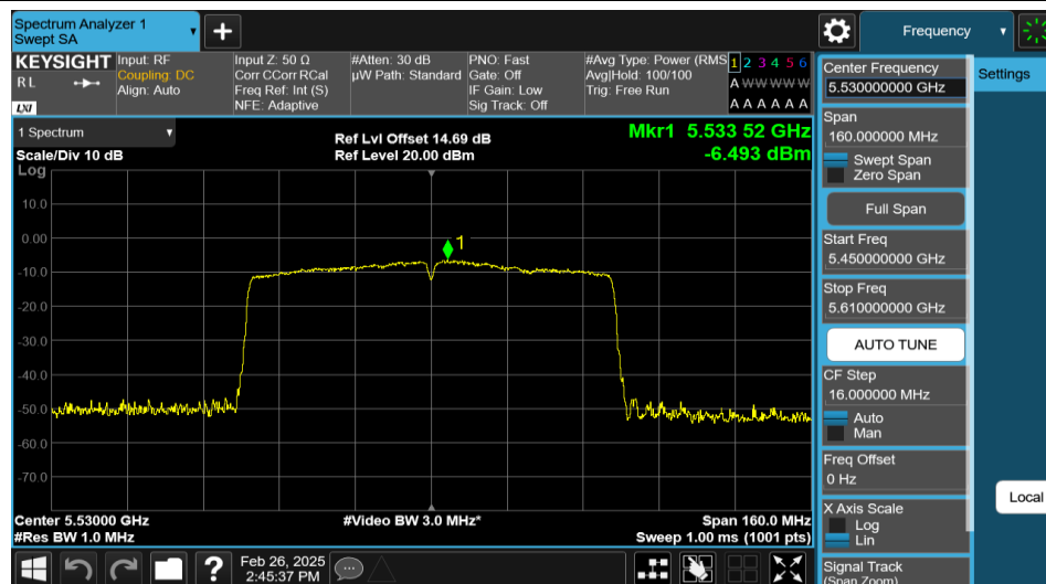
11AC80MIMO-Ant1-5530-PASS
