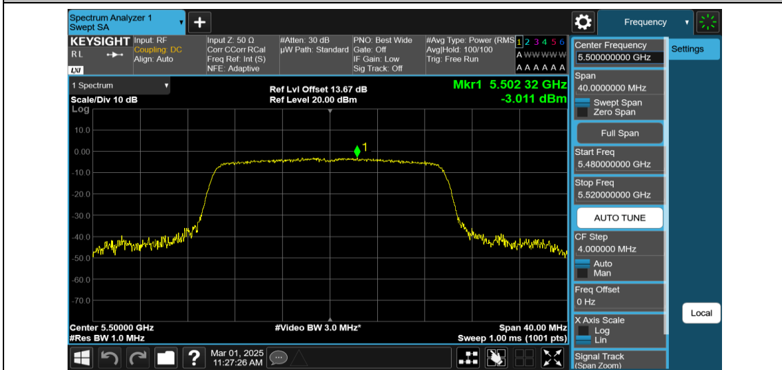
11AX20MIMO-Ant2-5500-PASS
