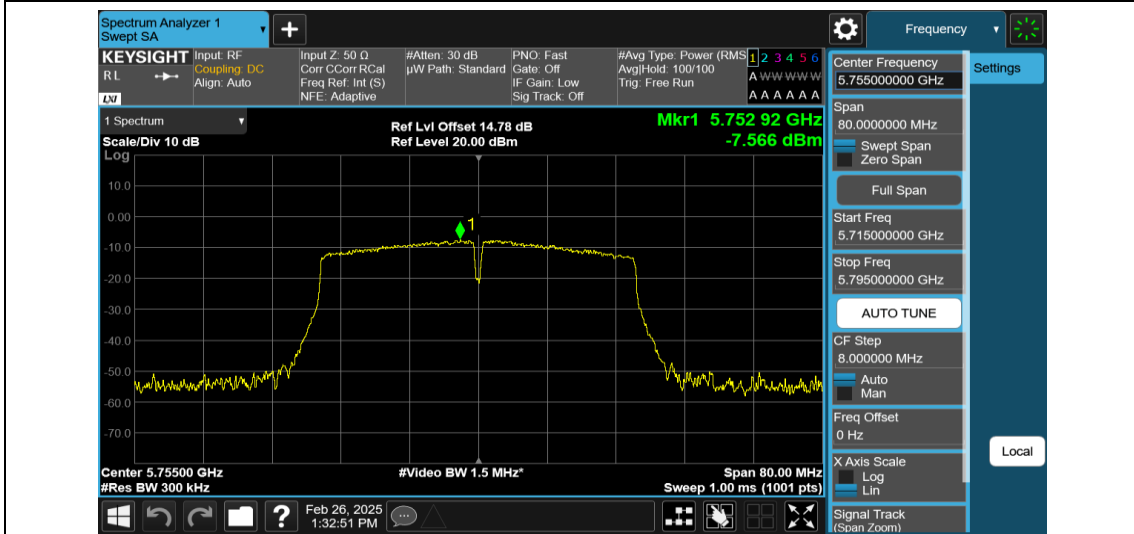
11AC40MIMO-Ant1-5755-PASS
