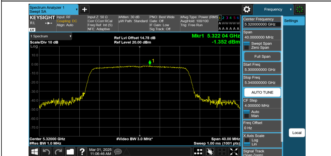
11AX20MIMO-Ant1-5320-PASS
