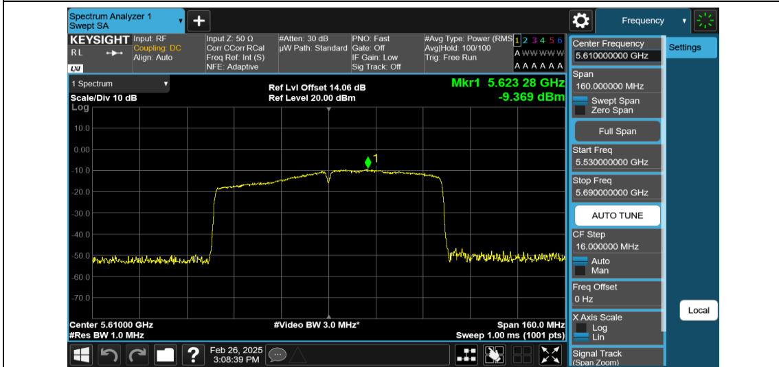
11AC80MIMO-Ant2-5610-PASS
