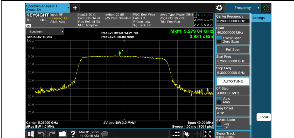
11AX20MIMO-Ant2-5280-PASS
