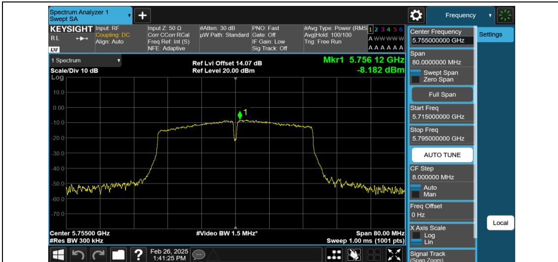
11AC40MIMO-Ant2-5755-PASS
