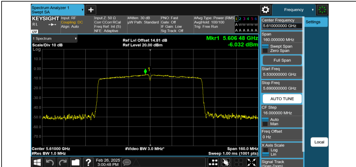
11AC80MIMO-Ant1-5610-PASS
