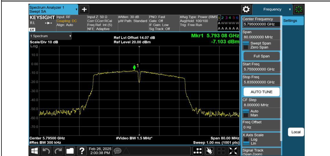
11AC40MIMO-Ant2-5795-PASS
