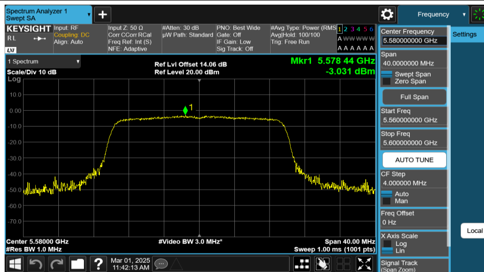
11AX20MIMO-Ant2-5580-PASS
