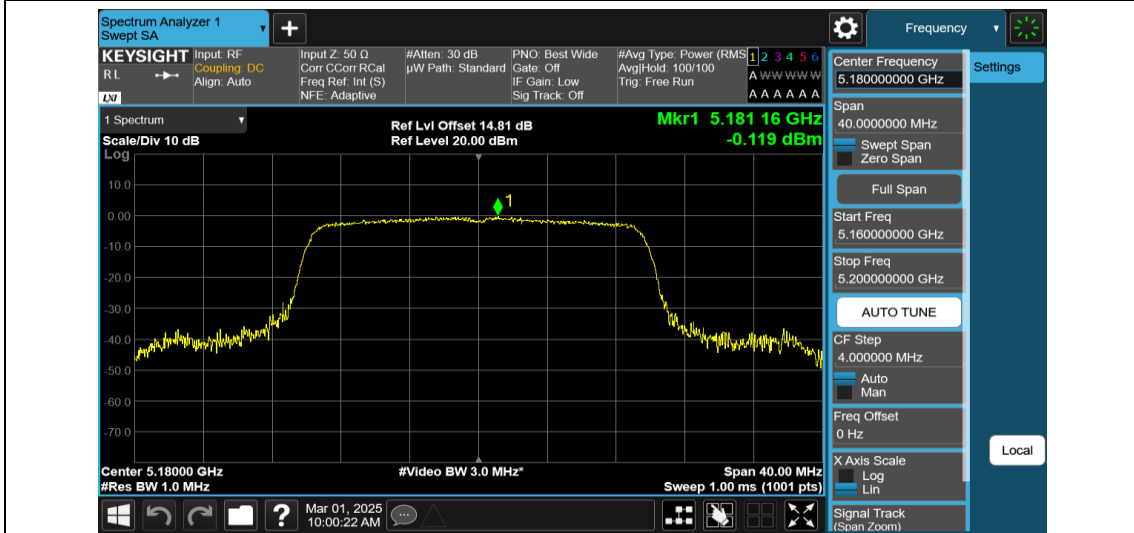
11AX20MIMO-Ant1-5180-PASS
