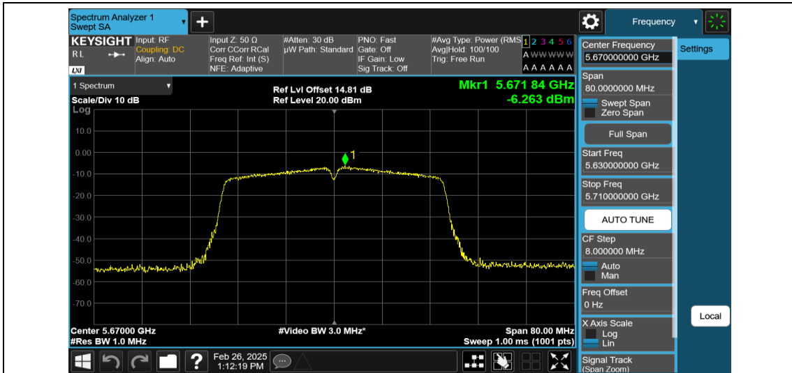
11AC40MIMO-Ant1-5670-PASS
