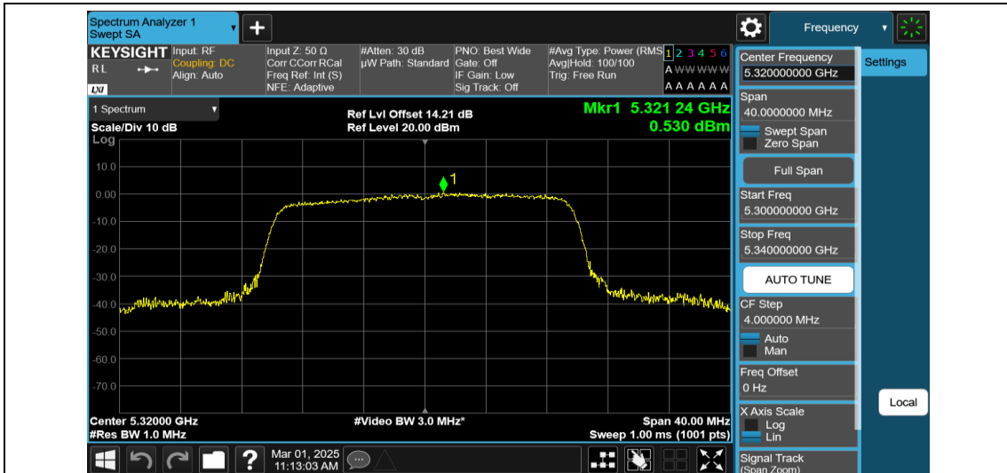
11AX20MIMO-Ant2-5320-PASS
