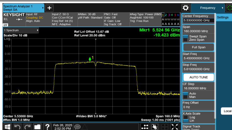
11AC80MIMO-Ant2-5530-PASS
