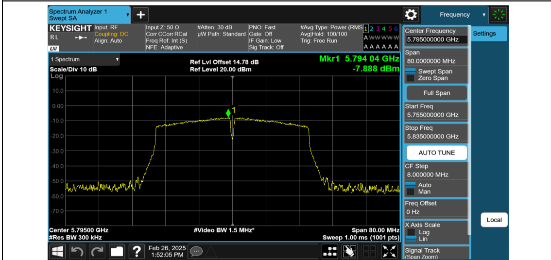
11AC40MIMO-Ant1-5795-PASS
