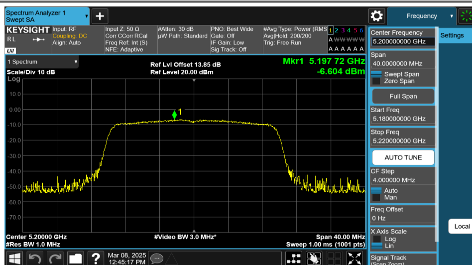
11AX20MIMO-Ant2-5200-242Tone-RU61-PASS
