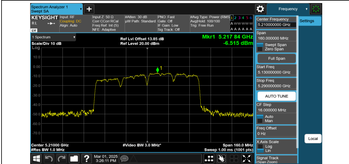
11AX80MIMO-Ant2-5210-PASS
