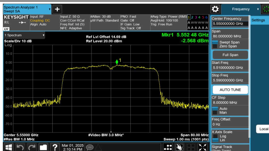
11AX40MIMO-Ant1-5550-PASS
