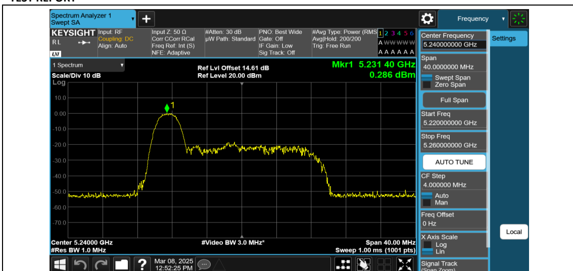
11AX20MIMO-Ant1-5240-26Tone-RU0-PASS
