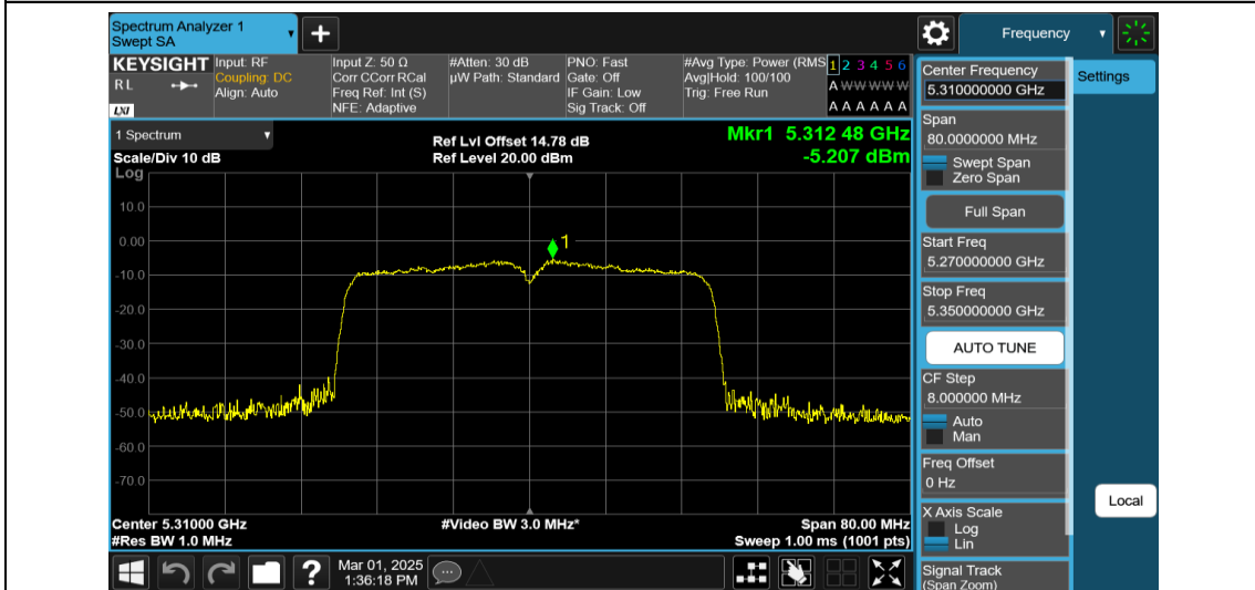
11AX40MIMO-Ant1-5310-PASS
