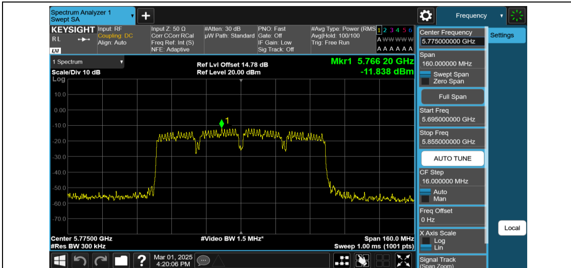
11AX80MIMO-Ant1-5775-PASS
