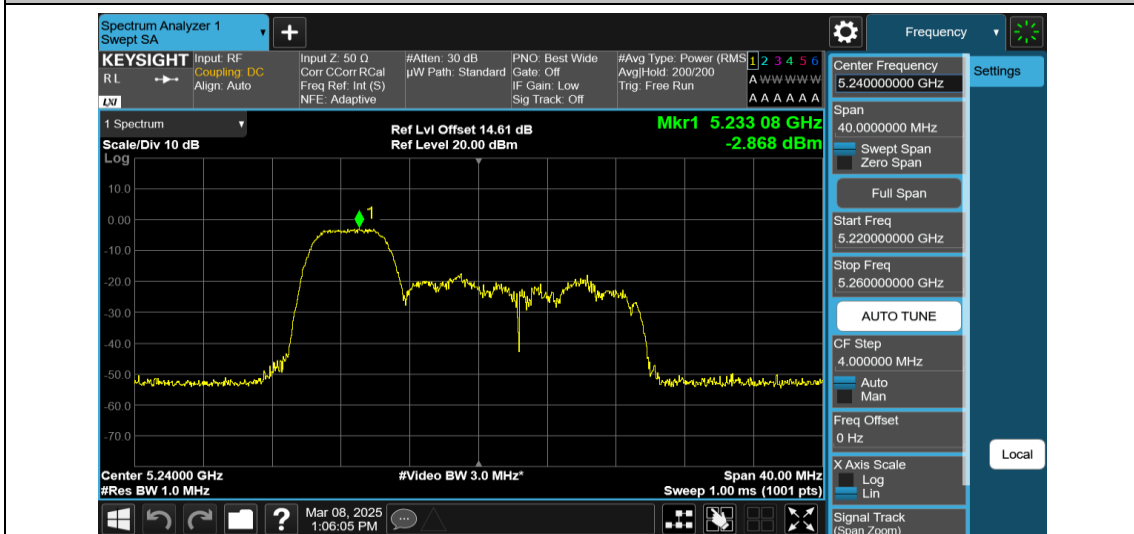
11AX20MIMO-Ant1-5240-52Tone-RU37-PASS
