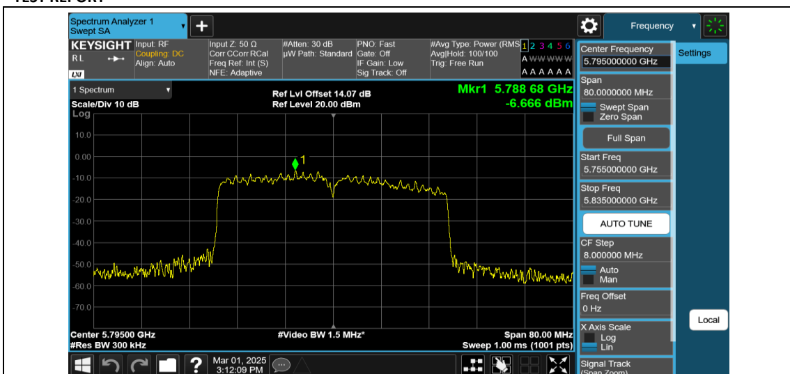
11AX40MIMO-Ant2-5795-PASS
