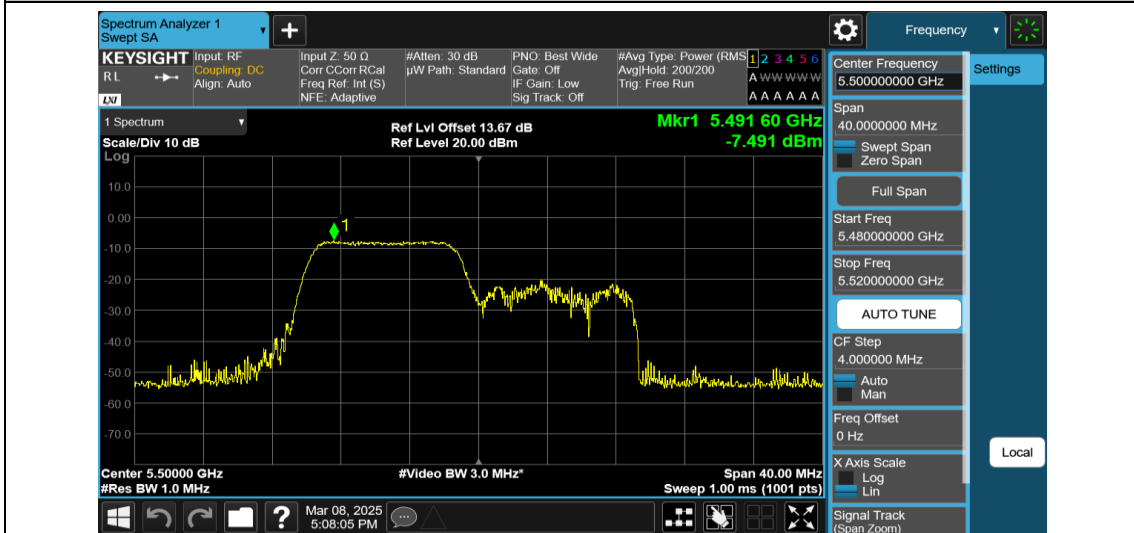
11AX20MIMO-Ant2-5500-106Tone-RU53-PASS
