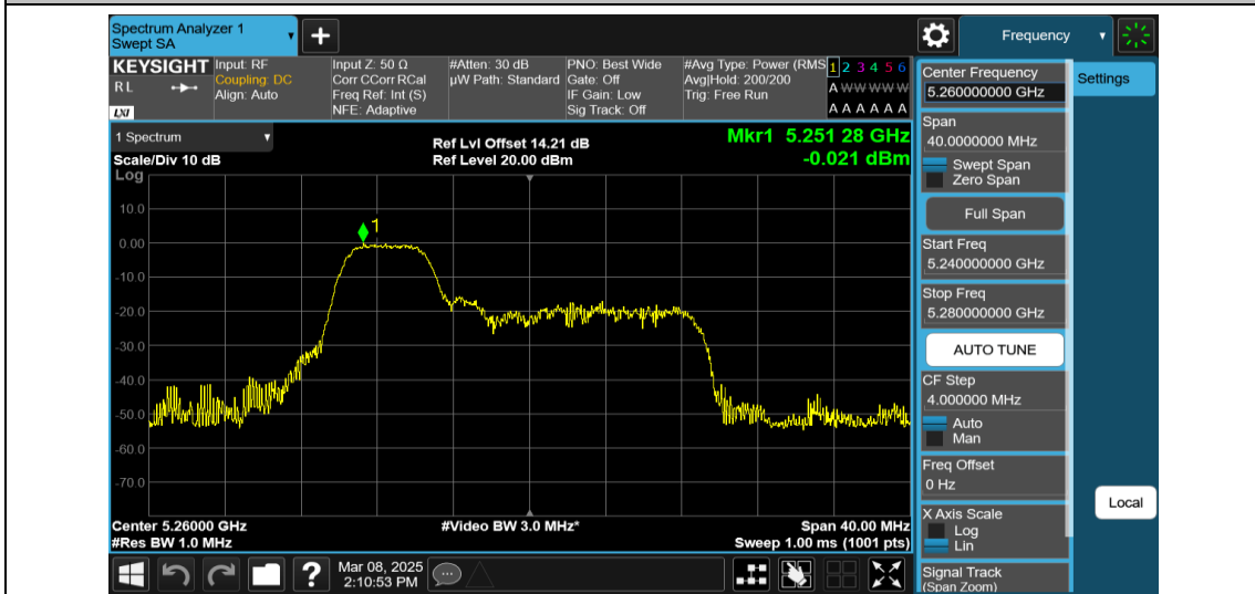
11AX20MIMO-Ant2-5260-52Tone-RU37-PASS
