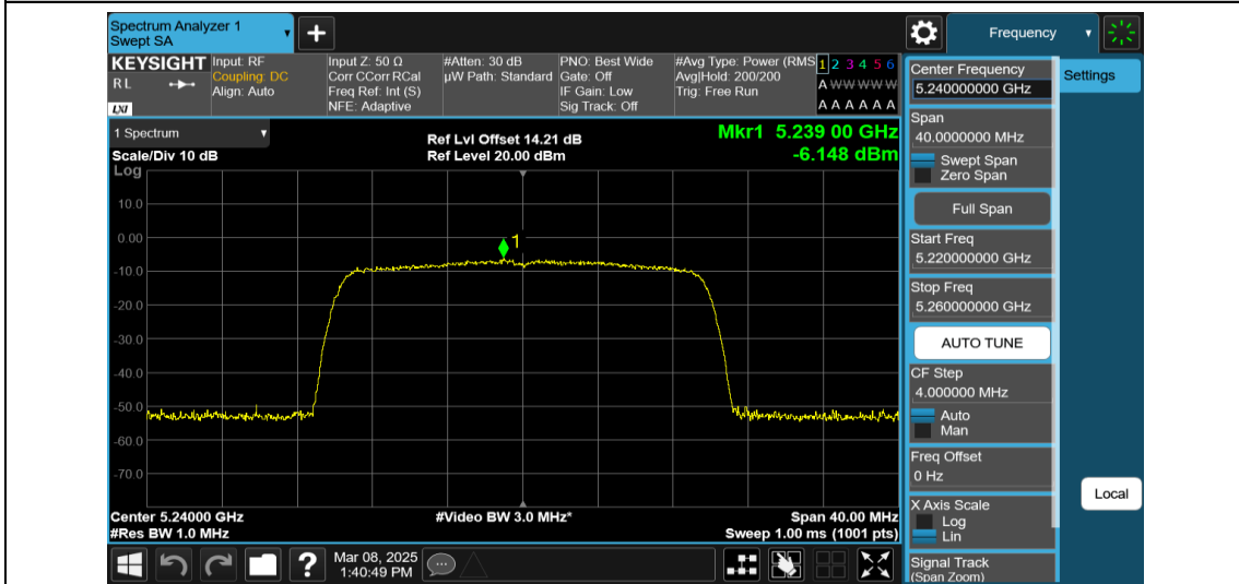
11AX20MIMO-Ant2-5240-242Tone-RU61-PASS
