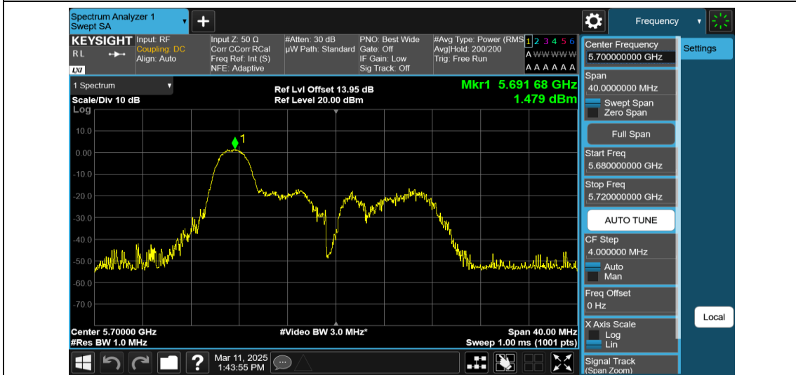
11AX20MIMO-Ant2-5700-26Tone-RU0-PASS
