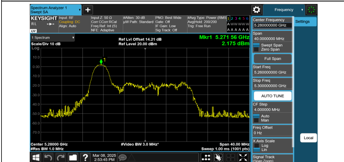
11AX20MIMO-Ant2-5280-26Tone-RU0-PASS
