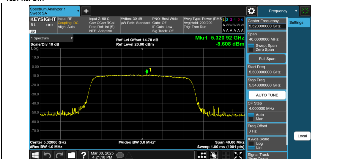
11AX20MIMO-Ant1-5320-242Tone-RU61-PASS
