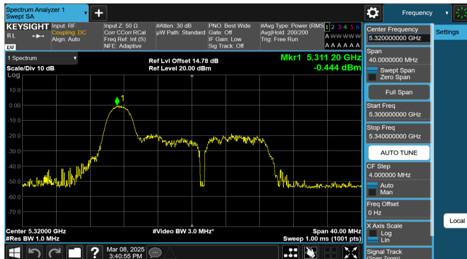
11AX20MIMO-Ant1-5320-26Tone-RU0-PASS
