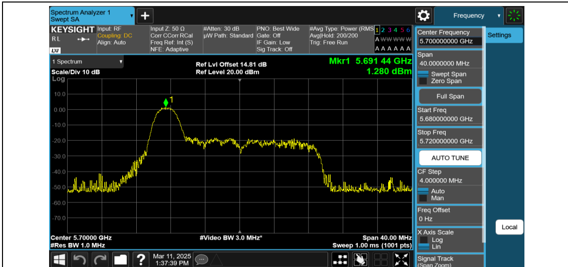
11AX20MIMO-Ant1-5700-26Tone-RU0-PASS
