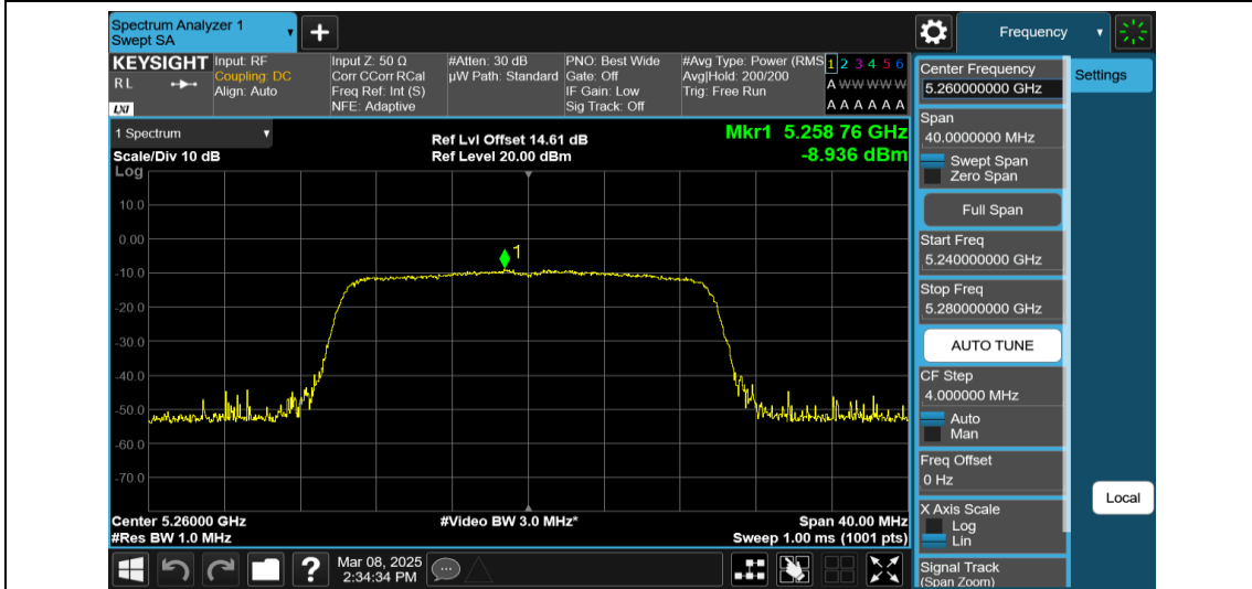
11AX20MIMO-Ant1-5260-242Tone-RU61-PASS
