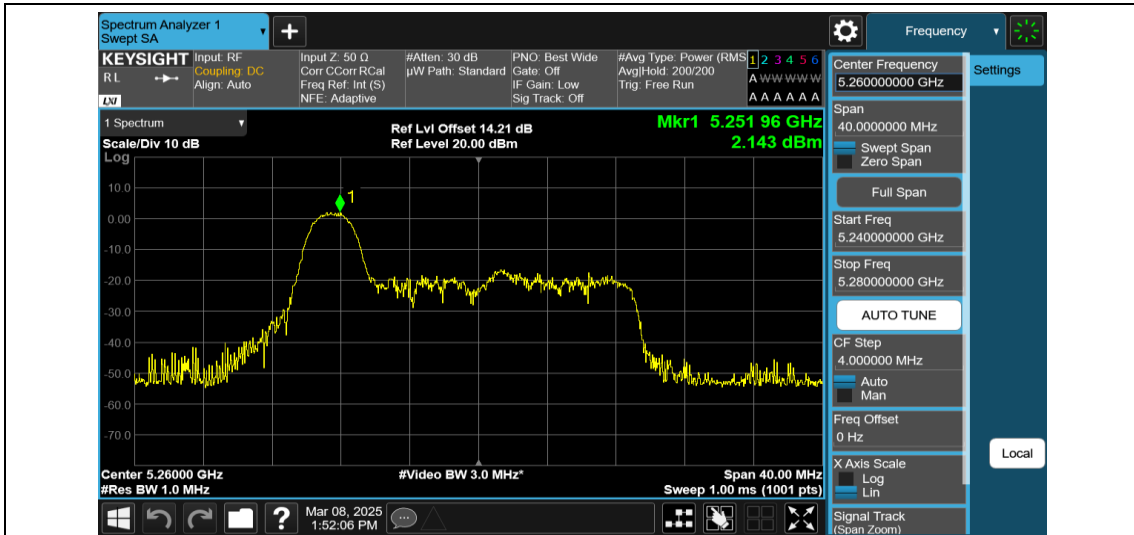
11AX20MIMO-Ant2-5260-26Tone-RU0-PASS
