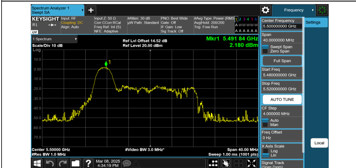
11AX20MIMO-Ant1-5500-26Tone-RU0-PASS
