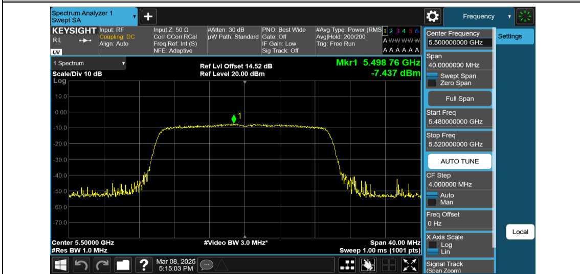
11AX20MIMO-Ant1-5500-242Tone-RU61-PASS
