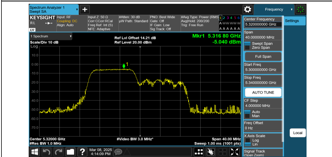
11AX20MIMO-Ant2-5320-106Tone-RU53-PASS
