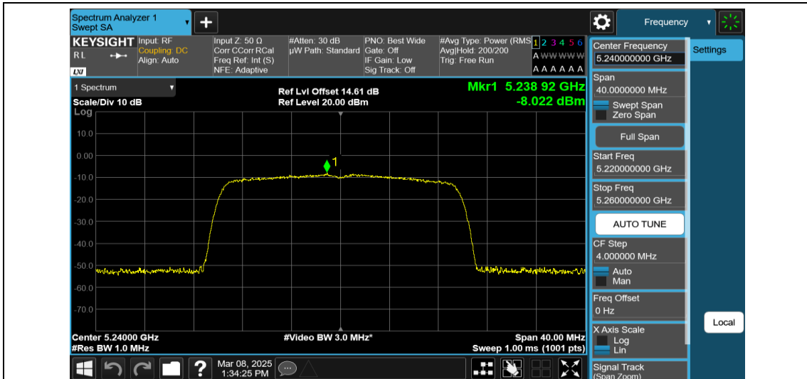
11AX20MIMO-Ant1-5240-242Tone-RU61-PASS
