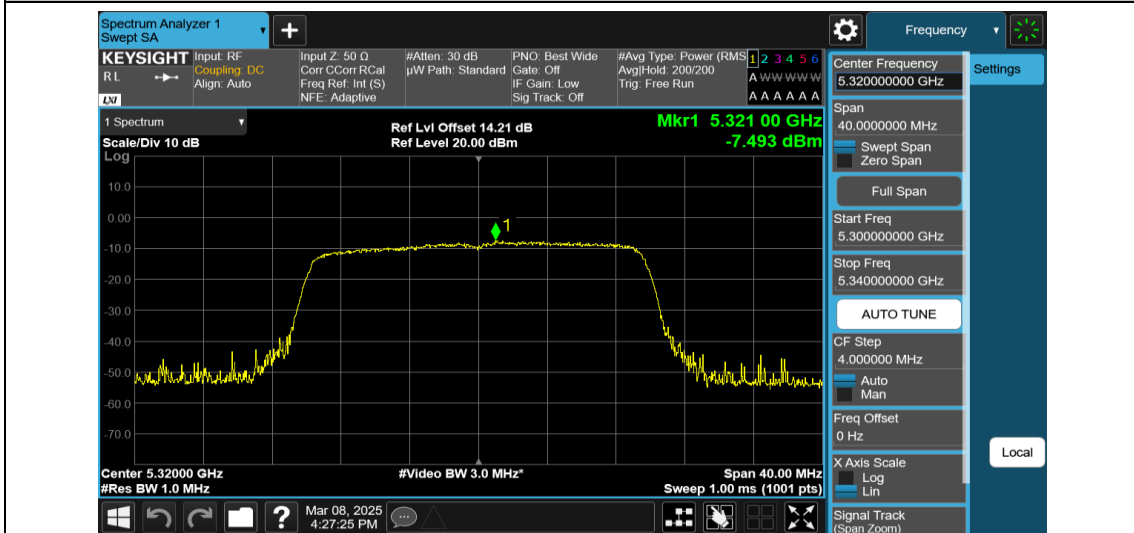
11AX20MIMO-Ant2-5320-242Tone-RU61-PASS
