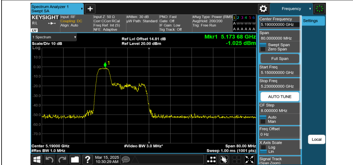
11AX40MIMO-Ant1-5190-52Tone-RU37-PASS
