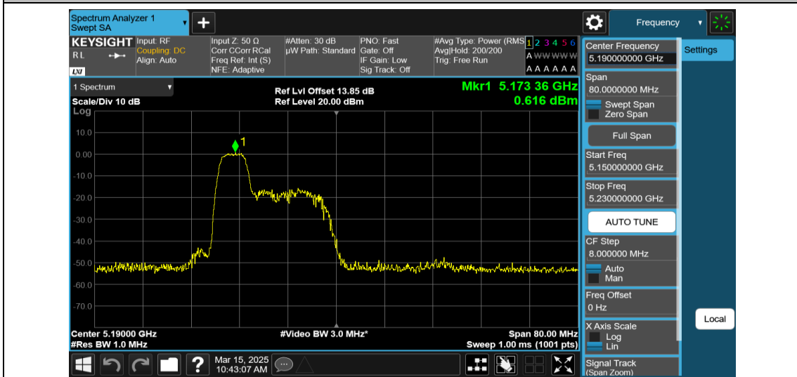
11AX40MIMO-Ant2-5190-52Tone-RU37-PASS
