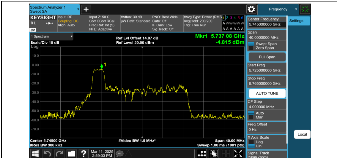
11AX20MIMO-Ant2-5745-26Tone-RU0-PASS
