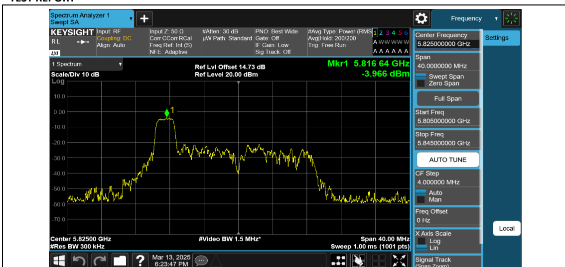
11AX20MIMO-Ant1-5825-26Tone-RU0-PASS
