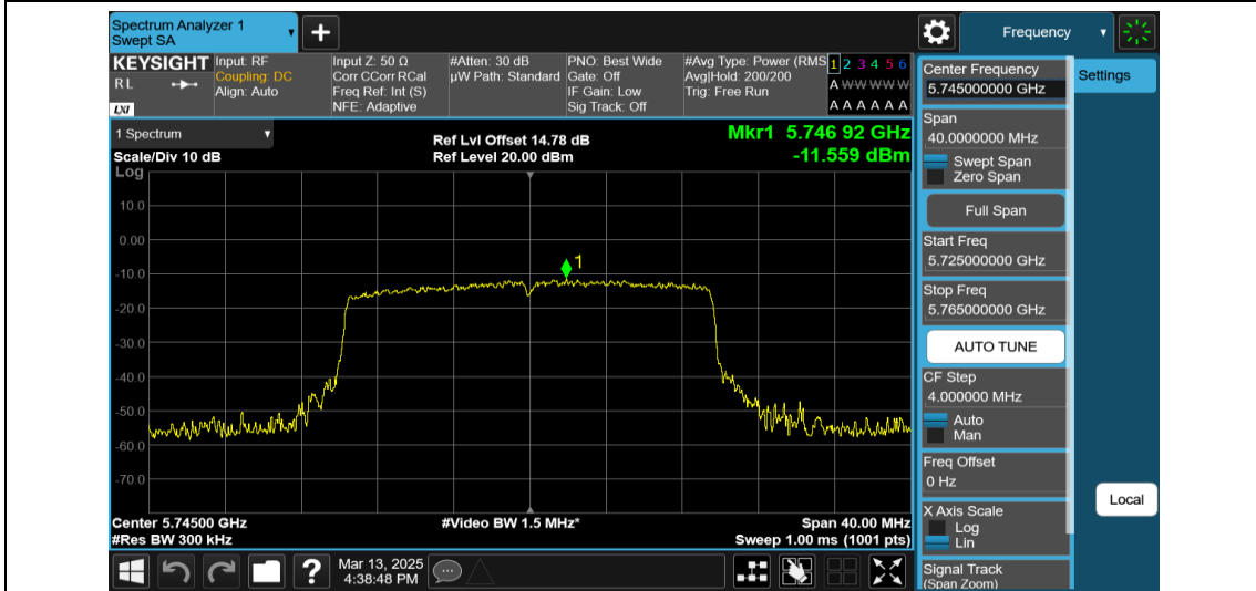
11AX20MIMO-Ant1-5745-242Tone-RU61-PASS
