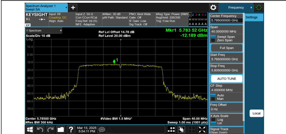
11AX20MIMO-Ant1-5785-242Tone-RU61-PASS
