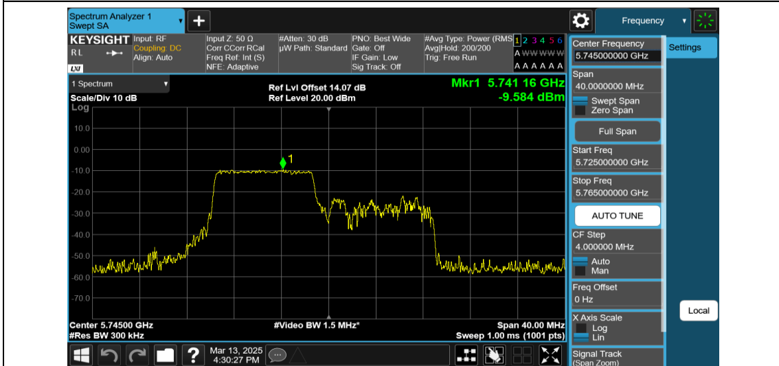
11AX20MIMO-Ant2-5745-106Tone-RU53-PASS
