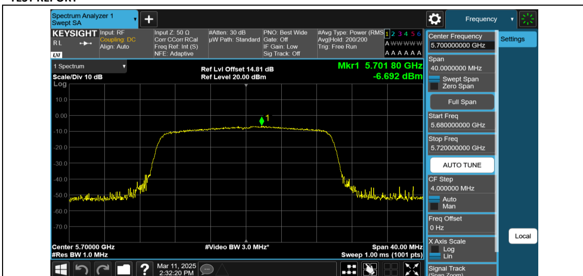
11AX20MIMO-Ant1-5700-242Tone-RU61-PASS
