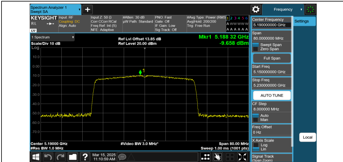
11AX40MIMO-Ant2-5190-484Tone-RU65-PASS
