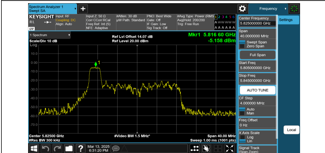
11AX20MIMO-Ant2-5825-26Tone-RU0-PASS
