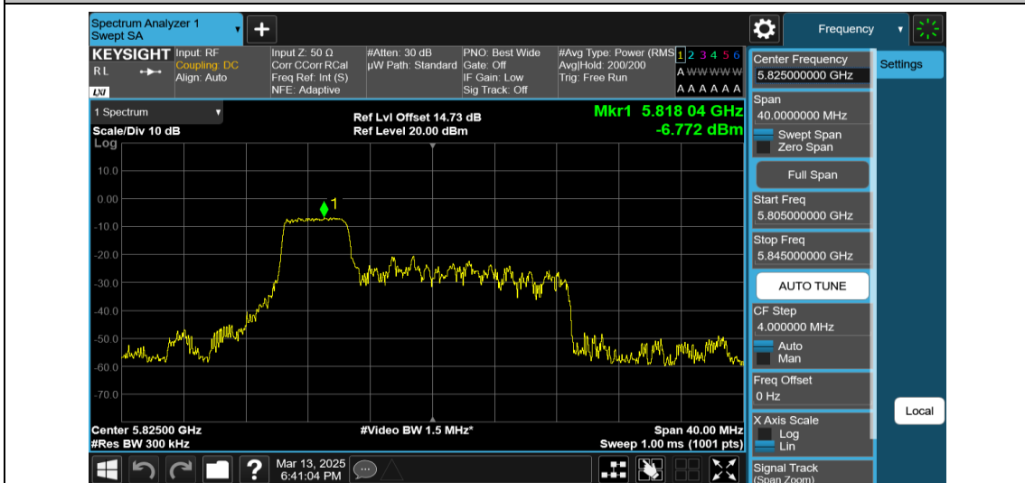
11AX20MIMO-Ant1-5825-52Tone-RU37-PASS
