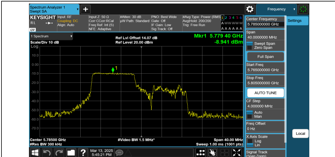
11AX20MIMO-Ant2-5785-106Tone-RU53-PASS
