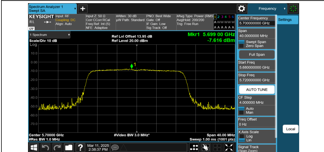
11AX20MIMO-Ant2-5700-242Tone-RU61-PASS
