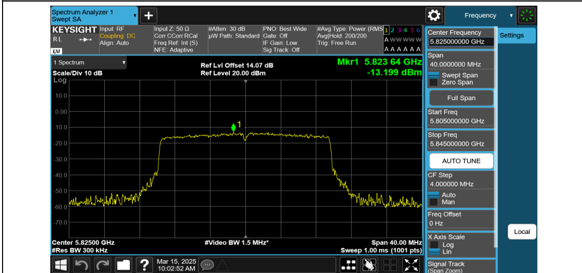
11AX20MIMO-Ant2-5825-242Tone-RU61-PASS
