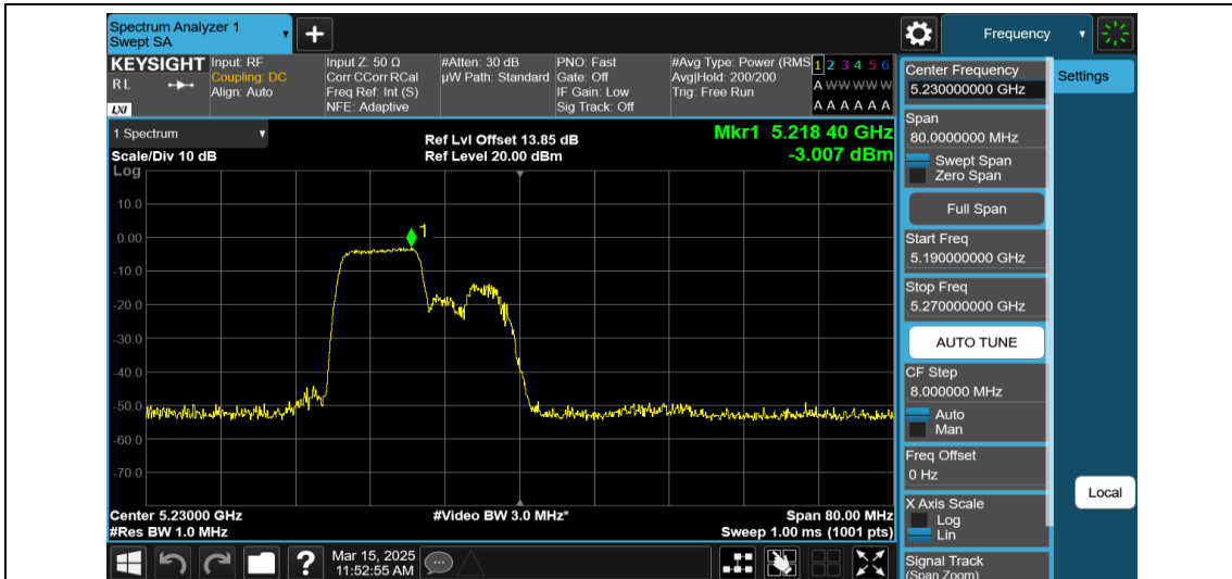
11AX40MIMO-Ant2-5230-106Tone-RU53-PASS
