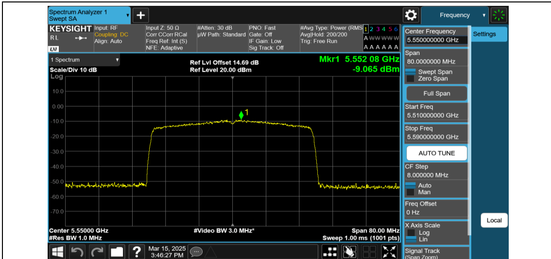
11AX40MIMO-Ant1-5550-484Tone-RU65-PASS
