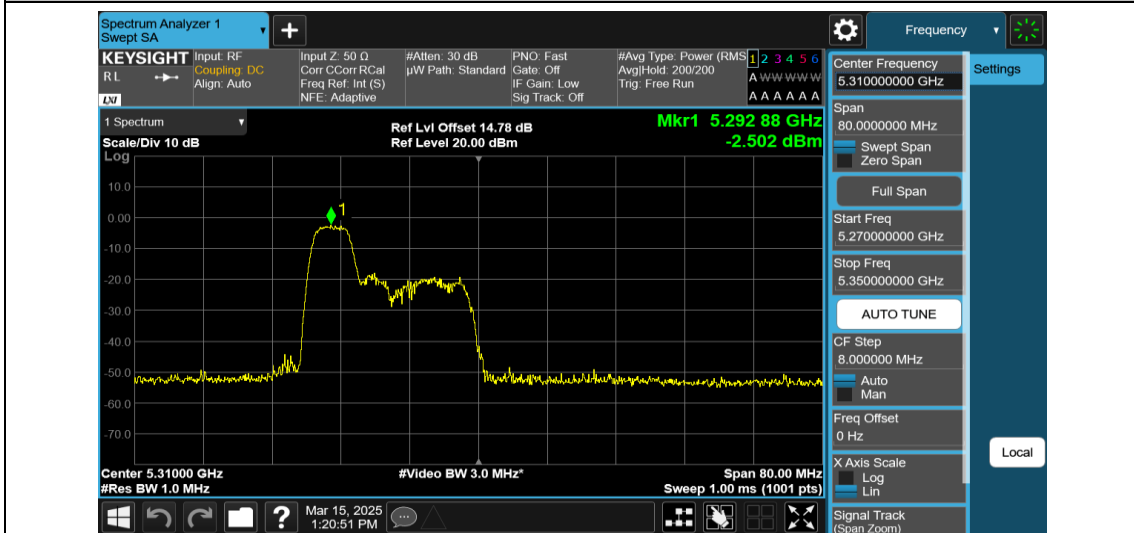
11AX40MIMO-Ant1-5310-52Tone-RU37-PASS
