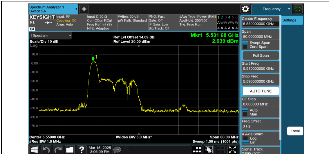
11AX40MIMO-Ant1-5550-26Tone-RU0-PASS
