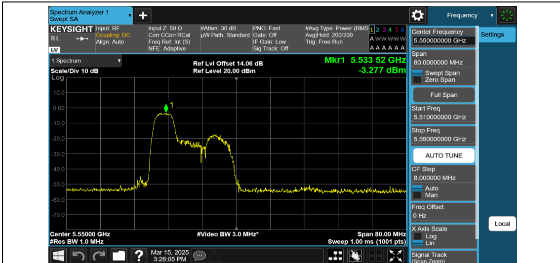
11AX40MIMO-Ant2-5550-52Tone-RU37-PASS
