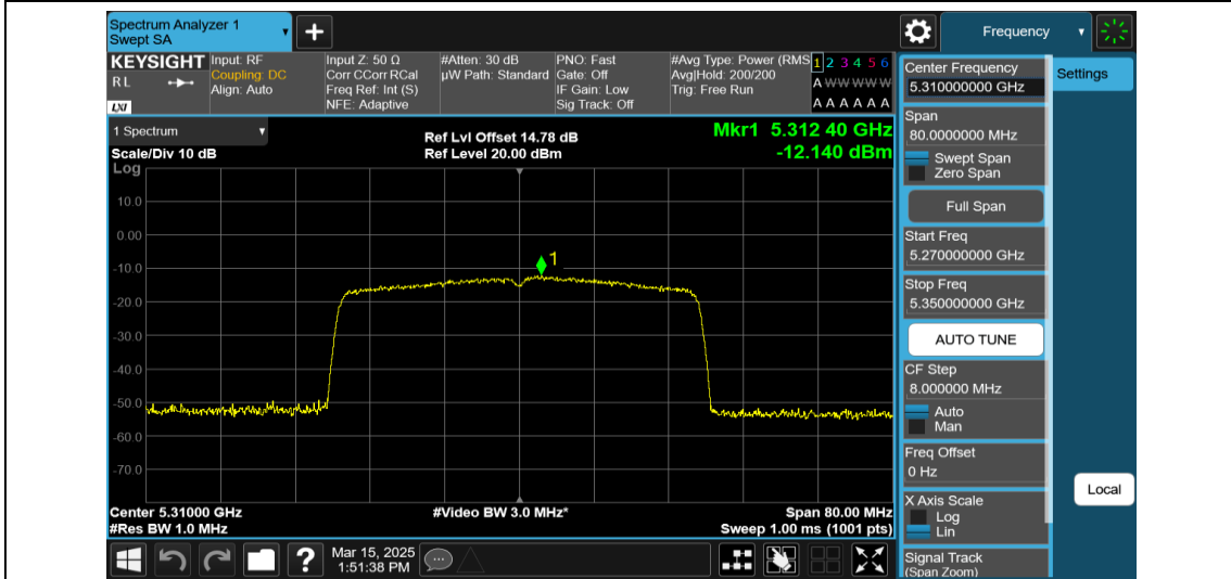
11AX40MIMO-Ant1-5310-484Tone-RU65-PASS
