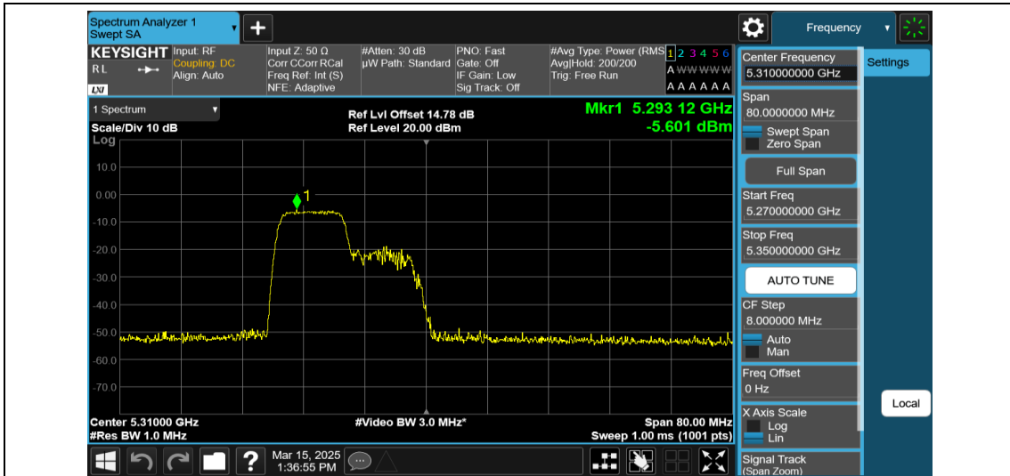
11AX40MIMO-Ant1-5310-106Tone-RU53-PASS
