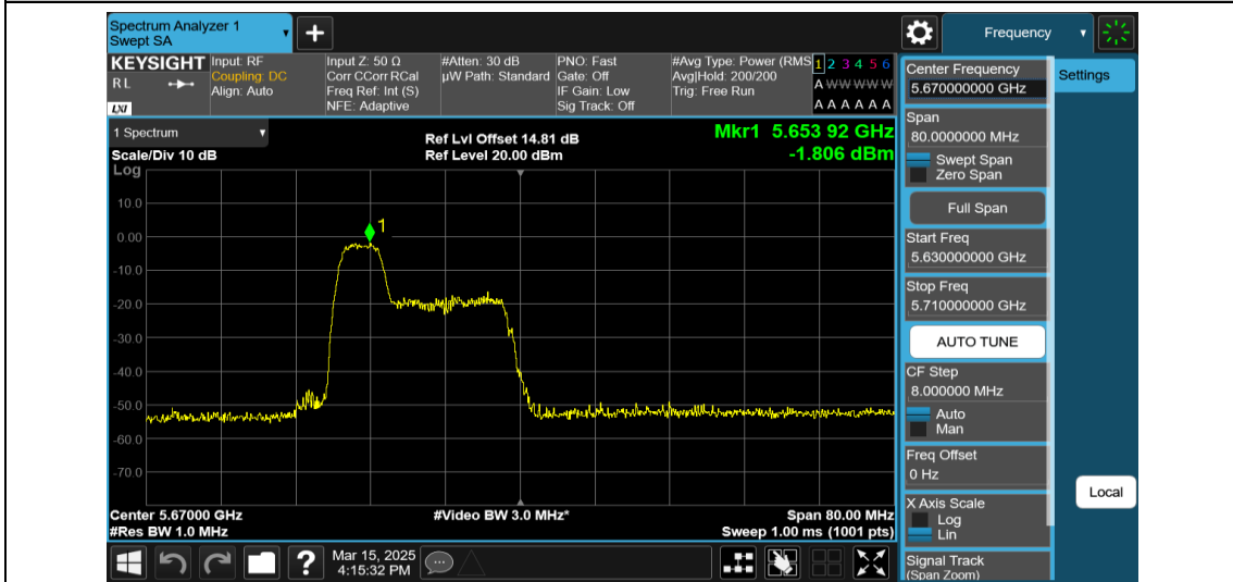
11AX40MIMO-Ant1-5670-52Tone-RU37-PASS
