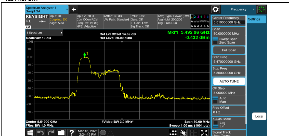
11AX40MIMO-Ant1-5510-52Tone-RU37-PASS
