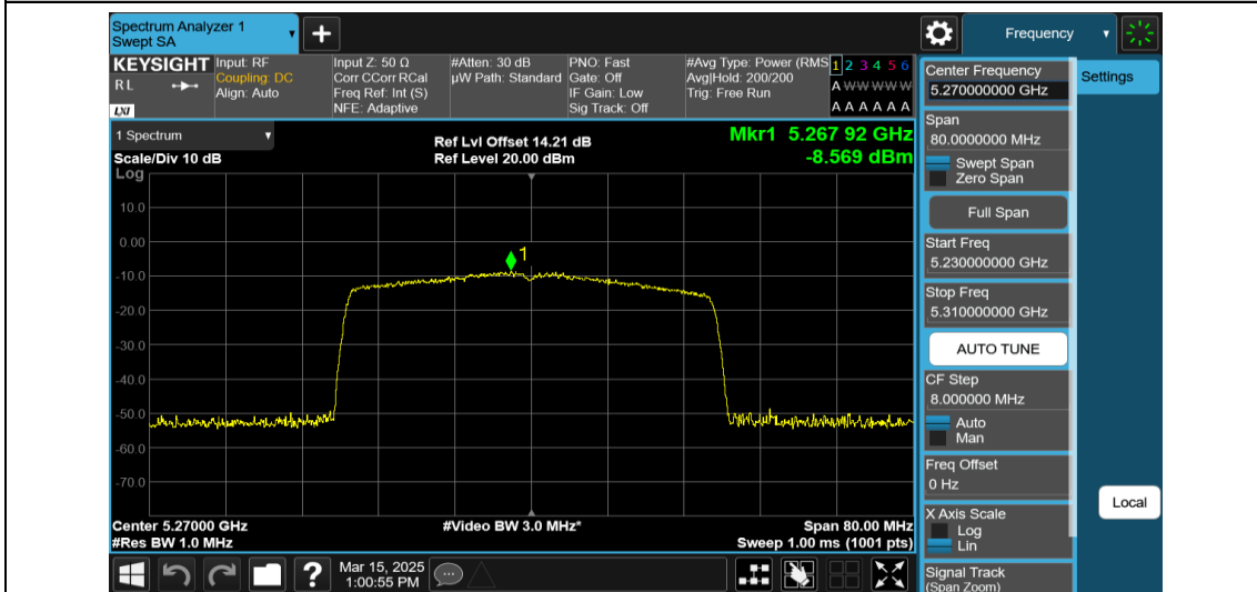
11AX40MIMO-Ant2-5270-484Tone-RU65-PASS
