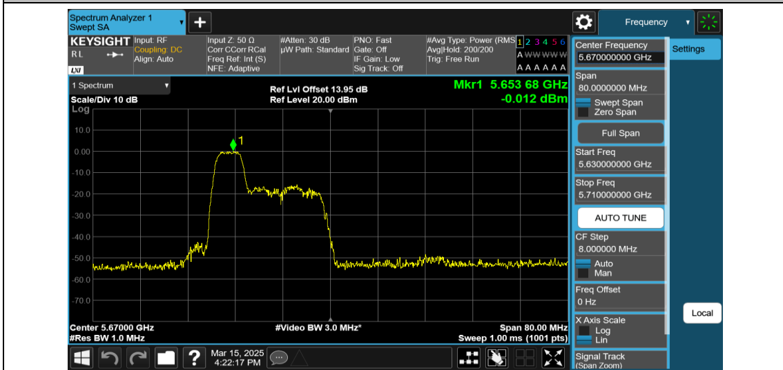
11AX40MIMO-Ant2-5670-52Tone-RU37-PASS
