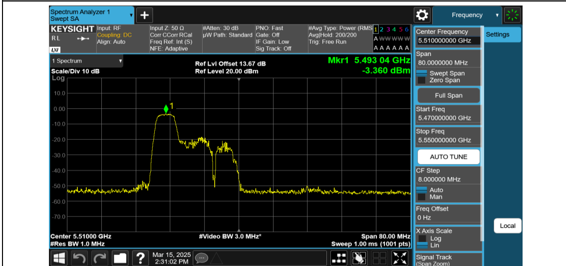
11AX40MIMO-Ant2-5510-52Tone-RU37-PASS
