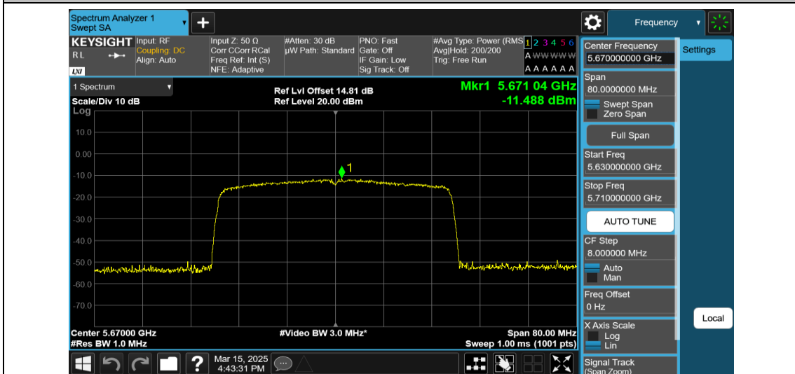
11AX40MIMO-Ant1-5670-484Tone-RU65-PASS
