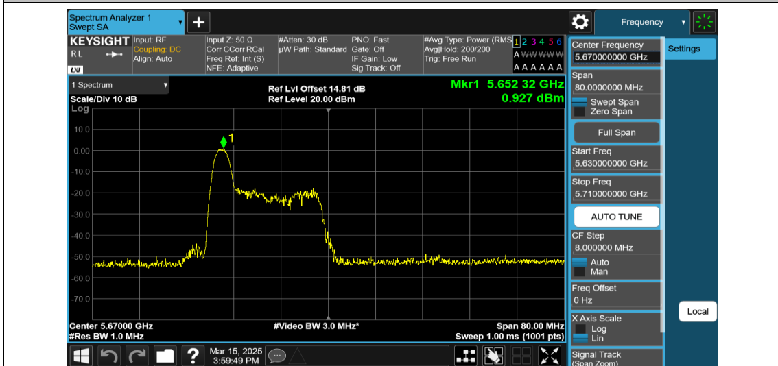
11AX40MIMO-Ant1-5670-26Tone-RU0-PASS
