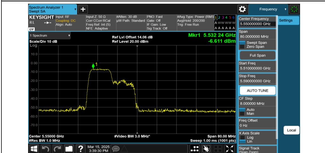
11AX40MIMO-Ant2-5550-106Tone-RU53-PASS
