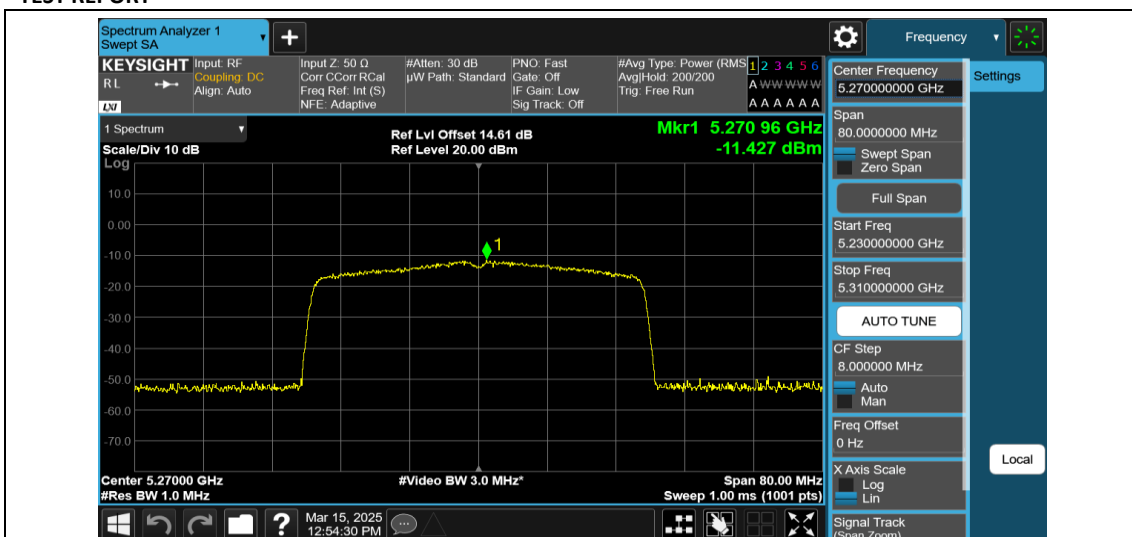
11AX40MIMO-Ant1-5270-484Tone-RU65-PASS
