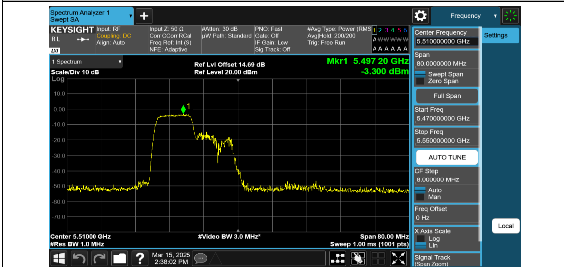
11AX40MIMO-Ant1-5510-106Tone-RU53-PASS
