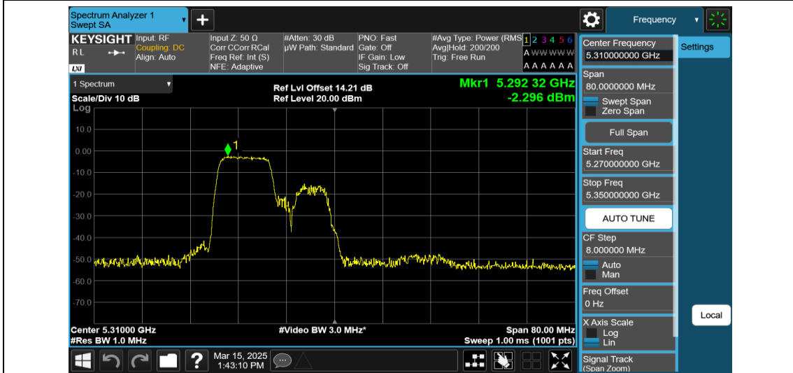
11AX40MIMO-Ant2-5310-106Tone-RU53-PASS
