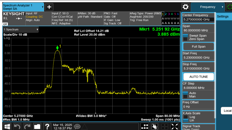
11AX40MIMO-Ant2-5270-26Tone-RU0-PASS
