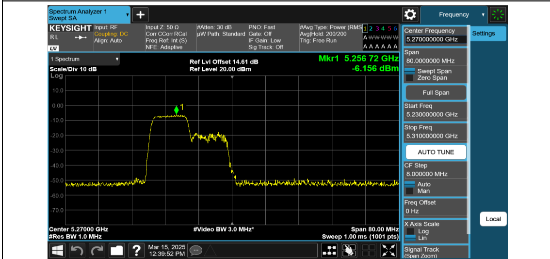
11AX40MIMO-Ant1-5270-106Tone-RU53-PASS
