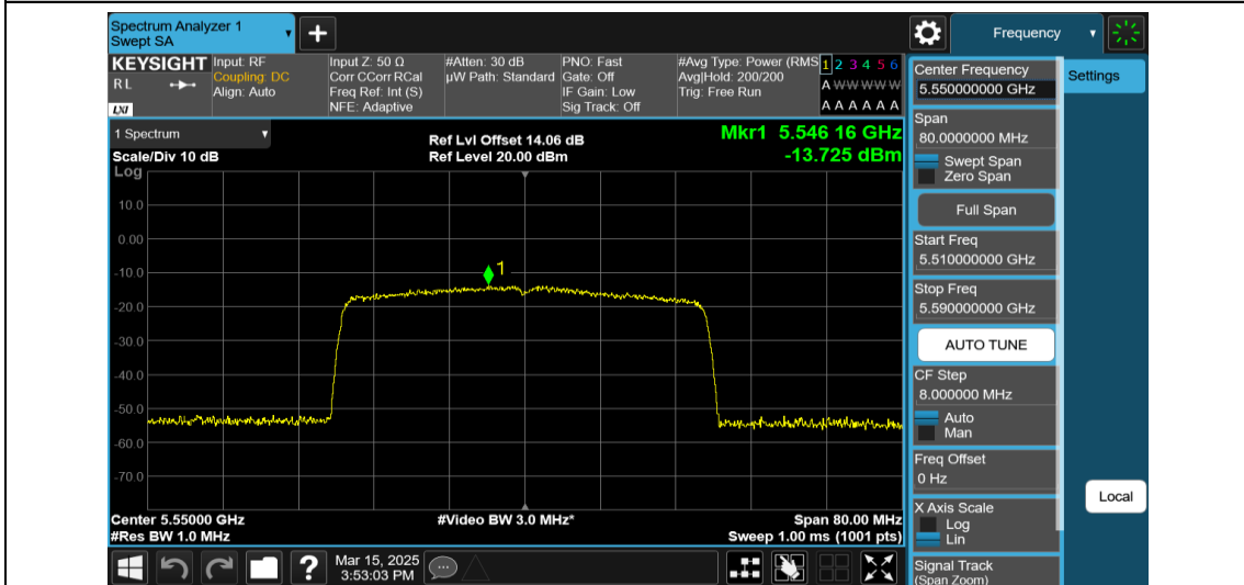
11AX40MIMO-Ant2-5550-484Tone-RU65-PASS
