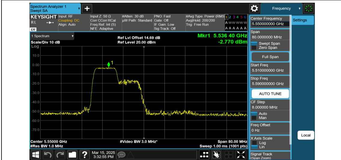
11AX40MIMO-Ant1-5550-106Tone-RU53-PASS
