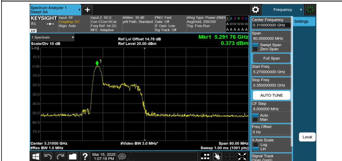
11AX40MIMO-Ant1-5310-26Tone-RU0-PASS
