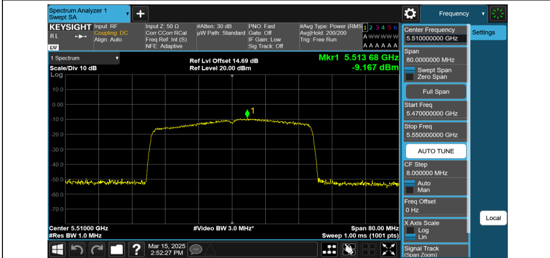
11AX40MIMO-Ant1-5510-484Tone-RU65-PASS
