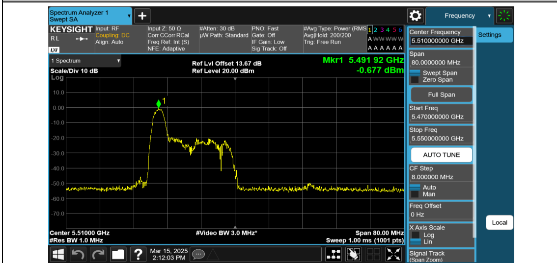
11AX40MIMO-Ant2-5510-26Tone-RU0-PASS
