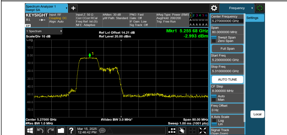
11AX40MIMO-Ant2-5270-106Tone-RU53-PASS
