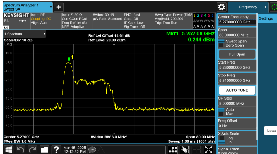
11AX40MIMO-Ant1-5270-26Tone-RU0-PASS
