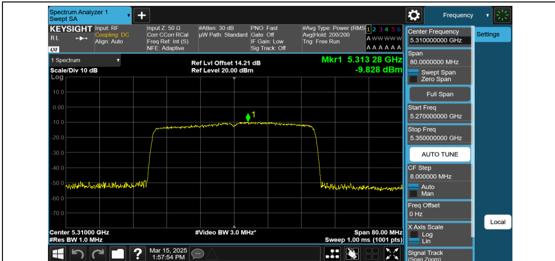
11AX40MIMO-Ant2-5310-484Tone-RU65-PASS
