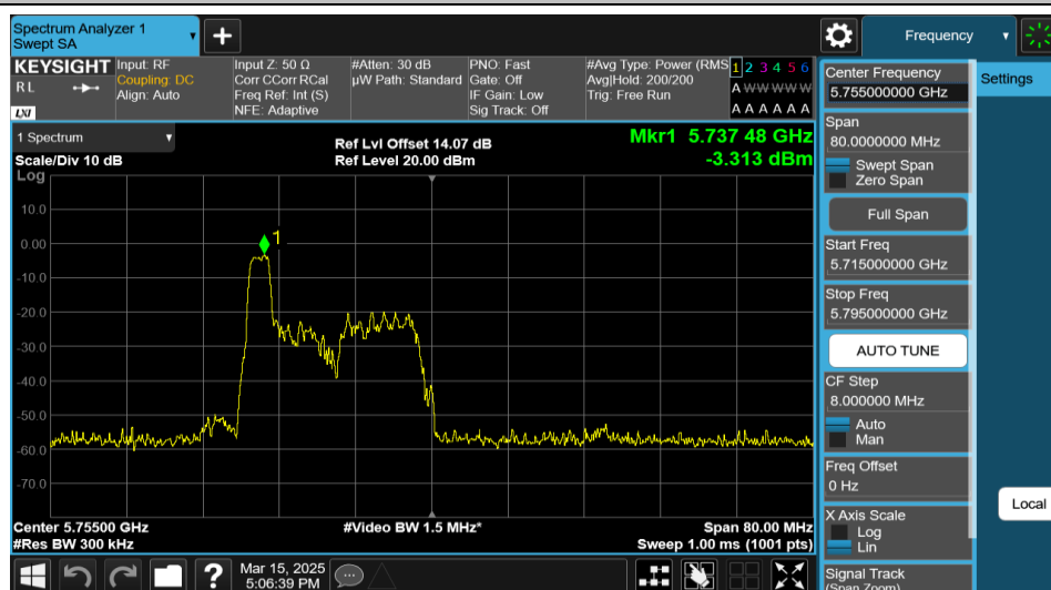
11AX40MIMO-Ant2-5755-26Tone-RU0-PASS
