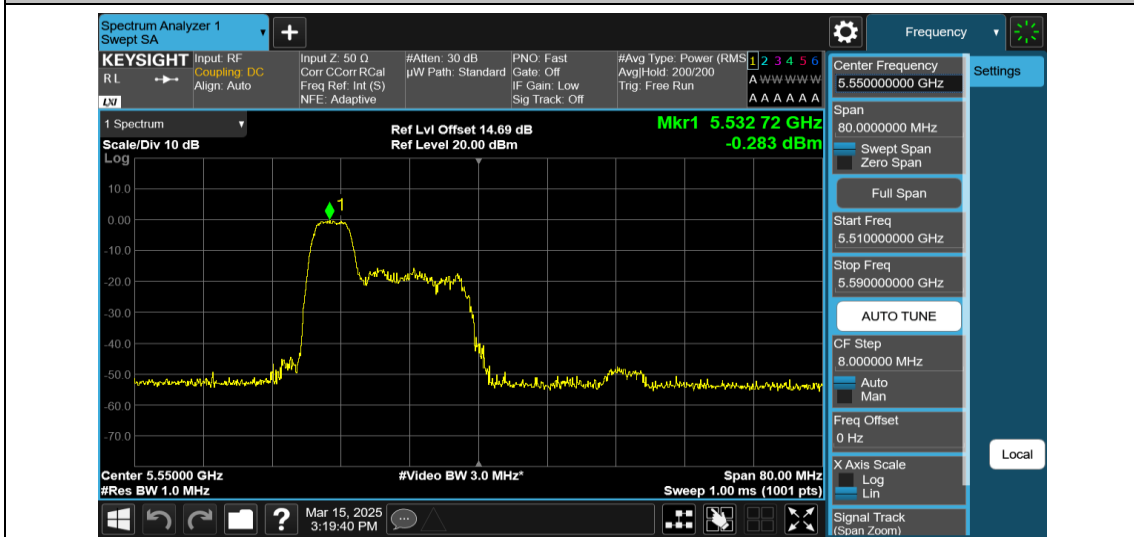
11AX40MIMO-Ant1-5550-52Tone-RU37-PASS
