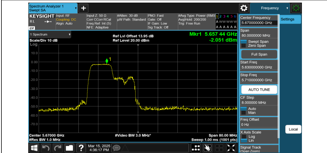
11AX40MIMO-Ant2-5670-106Tone-RU53-PASS
