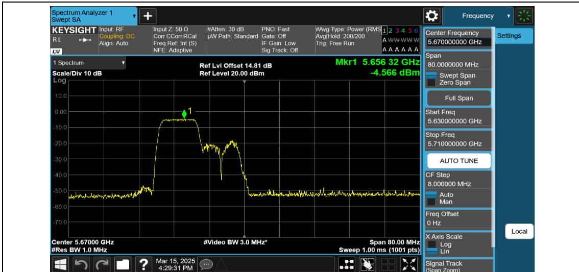
11AX40MIMO-Ant1-5670-106Tone-RU53-PASS
