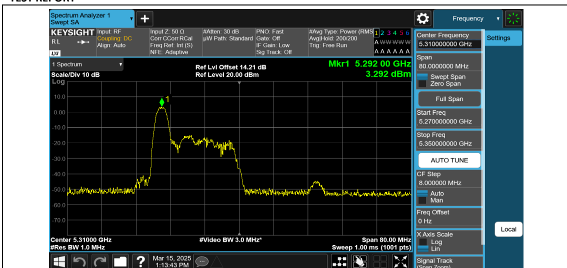
11AX40MIMO-Ant2-5310-26Tone-RU0-PASS
