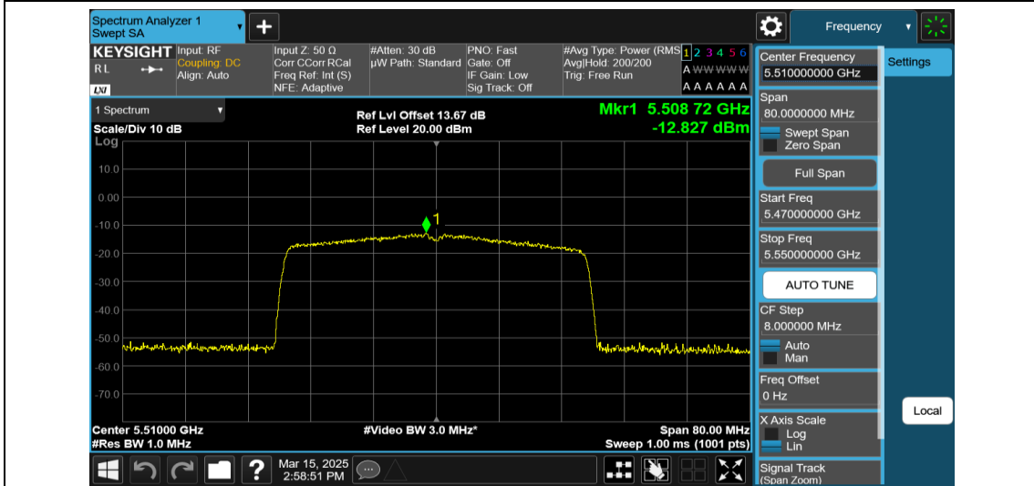
11AX40MIMO-Ant2-5510-484Tone-RU65-PASS
