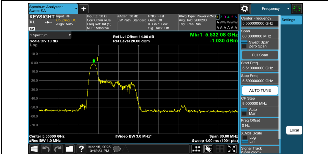
11AX40MIMO-Ant2-5550-26Tone-RU0-PASS
