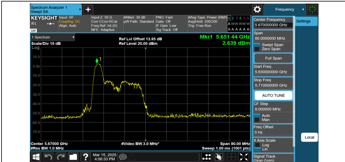
11AX40MIMO-Ant2-5670-26Tone-RU0-PASS
