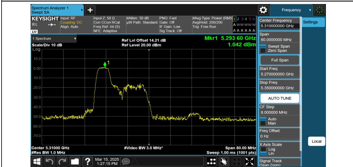
11AX40MIMO-Ant2-5310-52Tone-RU37-PASS
