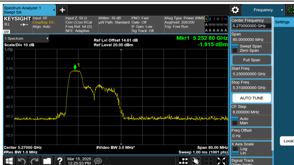
11AX40MIMO-Ant1-5270-52Tone-RU37-PASS
