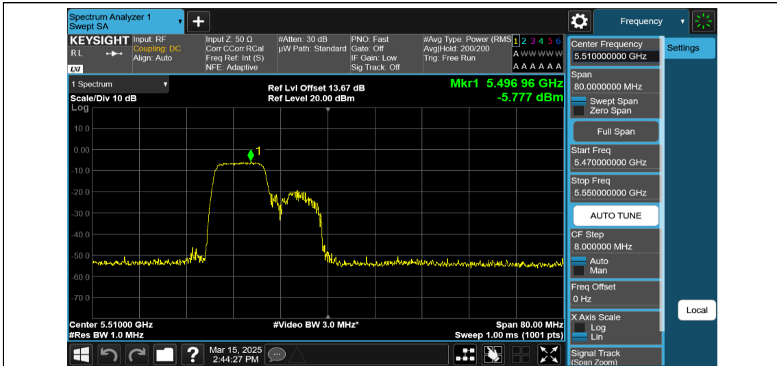
11AX40MIMO-Ant2-5510-106Tone-RU53-PASS
