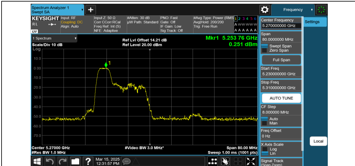
11AX40MIMO-Ant2-5270-52Tone-RU37-PASS
