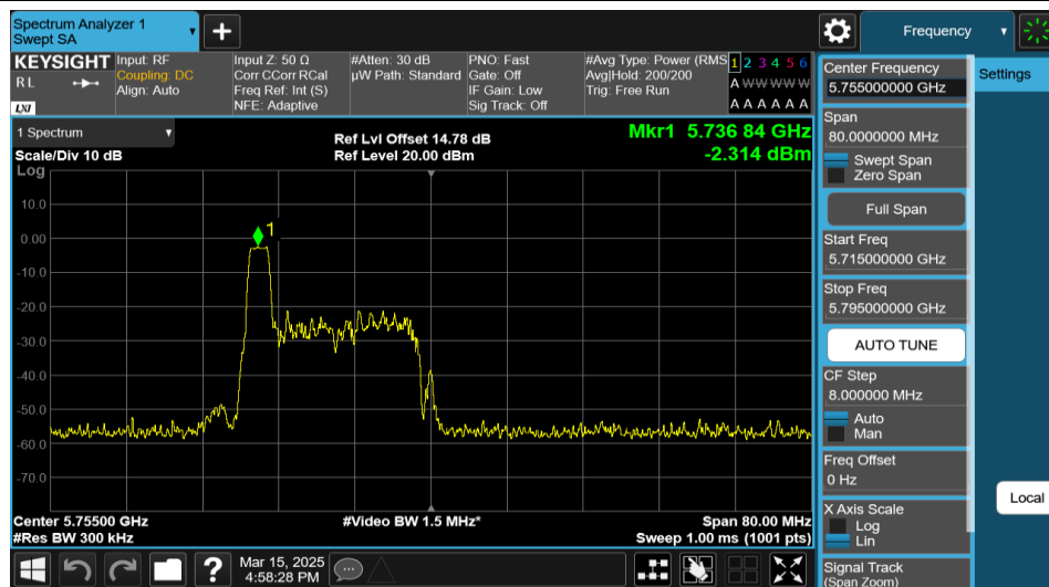
11AX40MIMO-Ant1-5755-26Tone-RU0-PASS
