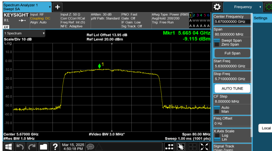
11AX40MIMO-Ant2-5670-484Tone-RU65-PASS
