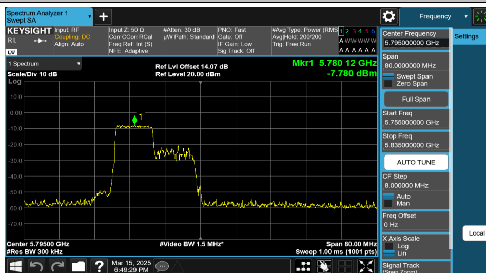
11AX40MIMO-Ant2-5795-106Tone-RU53-PASS
