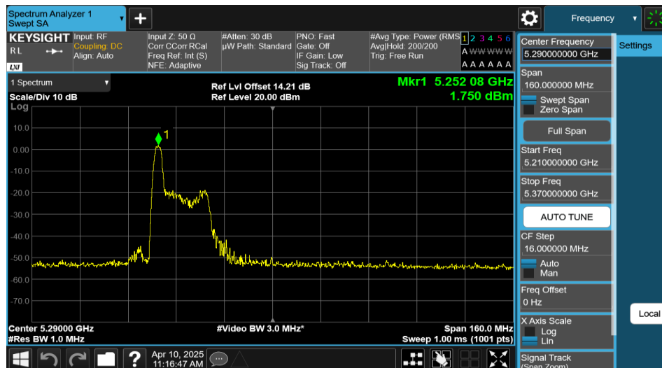
11AX80MIMO-Ant2-5290-26Tone-RU0-PASS
