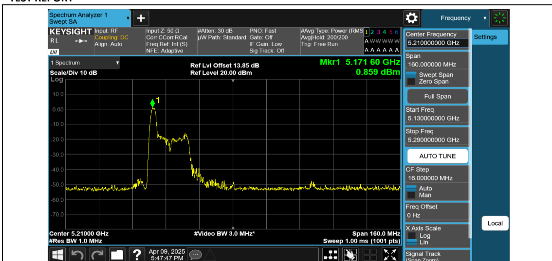
11AX80MIMO-Ant2-5210-26Tone-RU0-PASS
