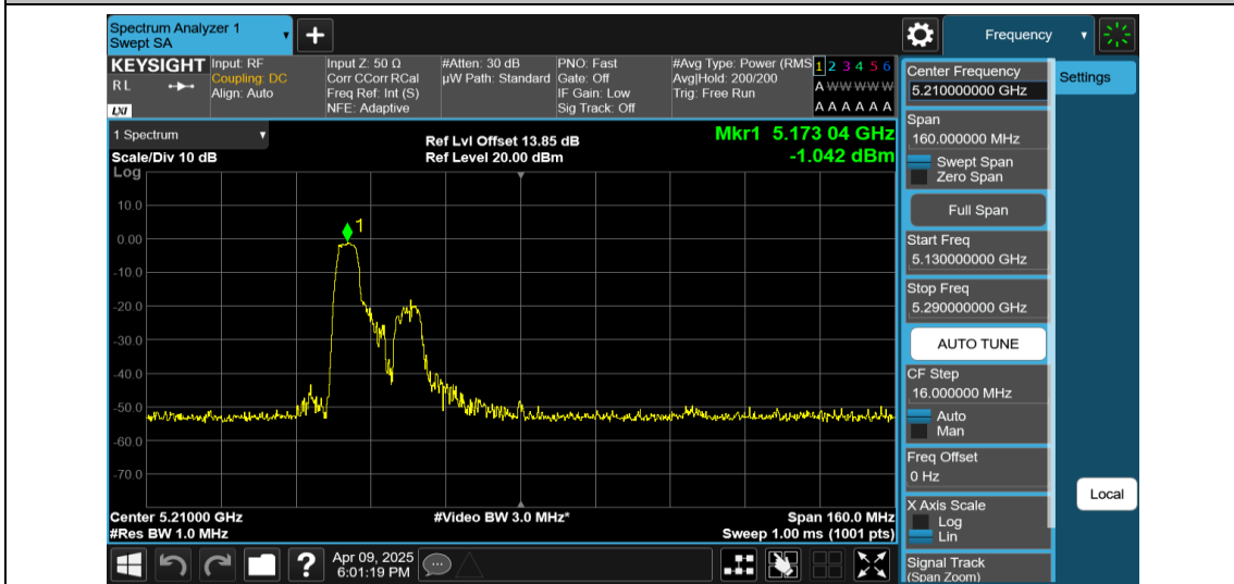
11AX80MIMO-Ant2-5210-52Tone-RU37-PASS
