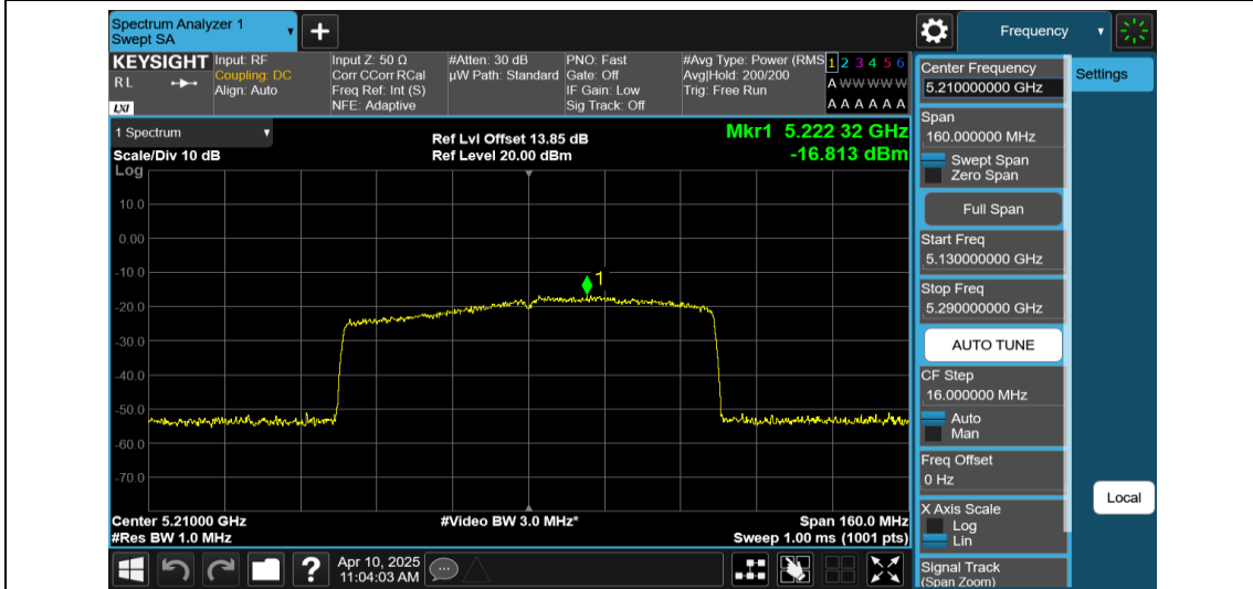
11AX80MIMO-Ant2-5210-996Tone-RU67-PASS
