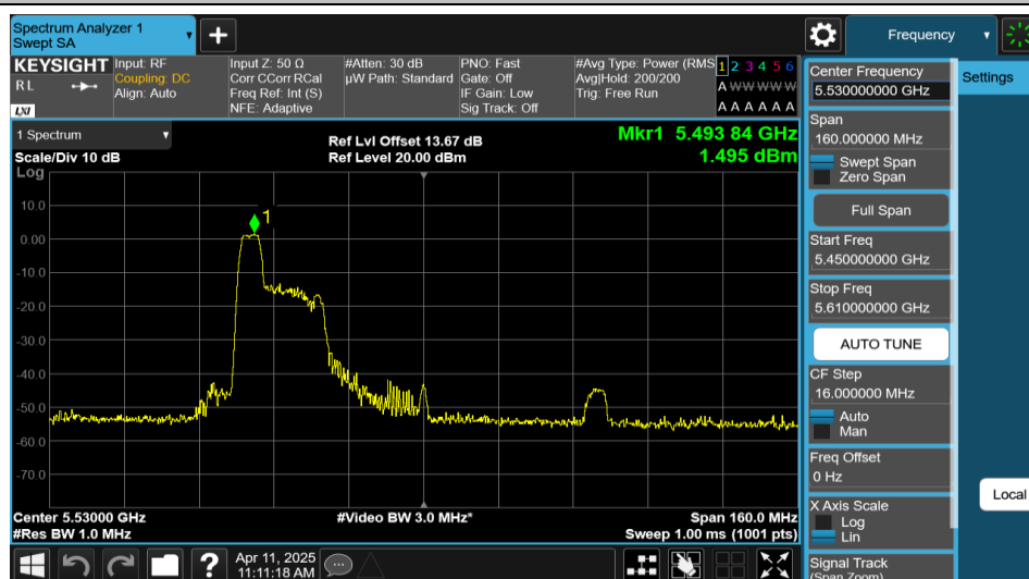
11AX80MIMO-Ant2-5530-52Tone-RU37-PASS
