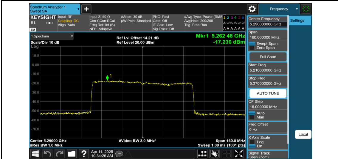
11AX80MIMO-Ant2-5290-996Tone-RU67-PASS
