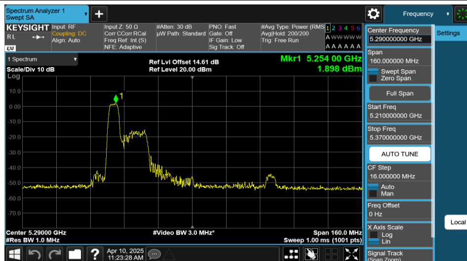
11AX80MIMO-Ant1-5290-52Tone-RU37-PASS
