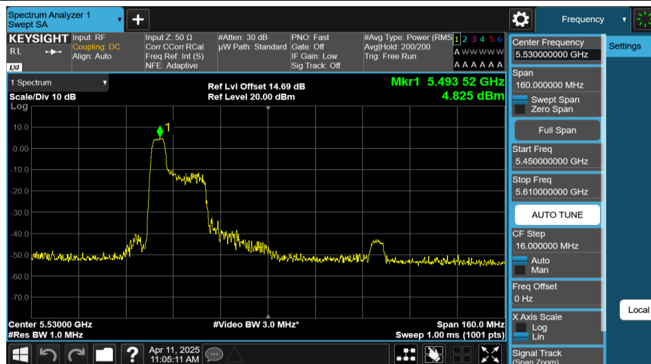
11AX80MIMO-Ant1-5530-52Tone-RU37-PASS
