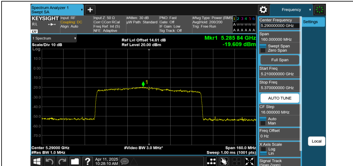
11AX80MIMO-Ant1-5290-996Tone-RU67-PASS
