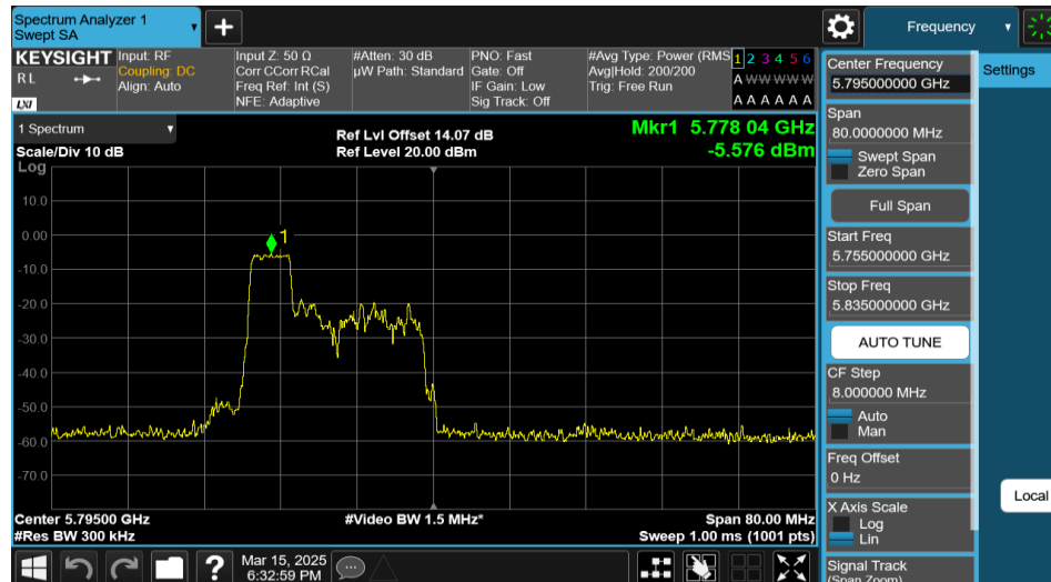
11AX40MIMO-Ant2-5795-52Tone-RU37-PASS
