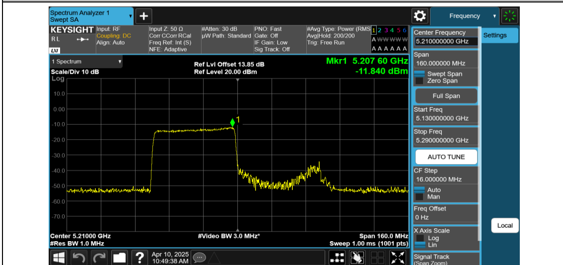
11AX80MIMO-Ant2-5210-484Tone-RU65-PASS
