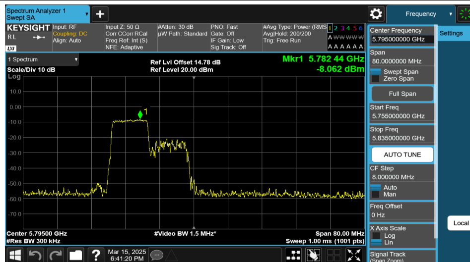
11AX40MIMO-Ant1-5795-106Tone-RU53-PASS
