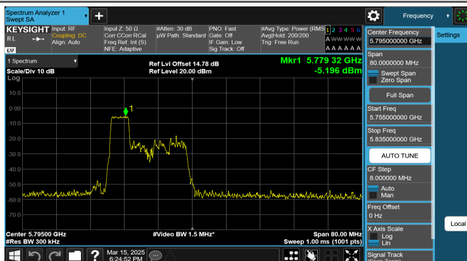
11AX40MIMO-Ant1-5795-52Tone-RU37-PASS
