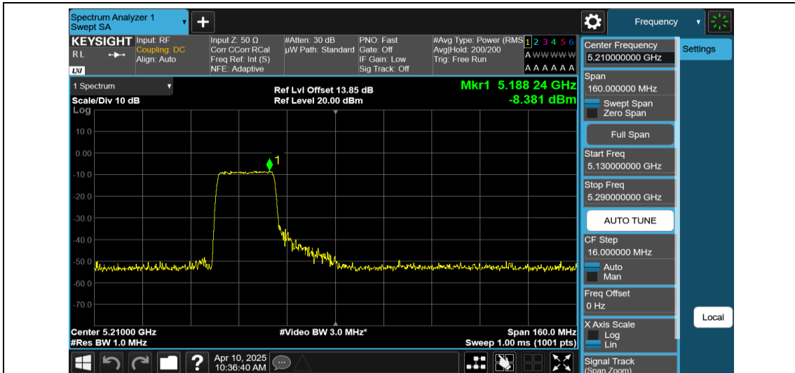
11AX80MIMO-Ant2-5210-242Tone-RU61-PASS
