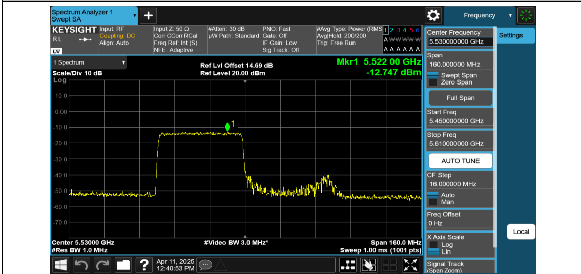
11AX80MIMO-Ant1-5530-484Tone-RU65-PASS
