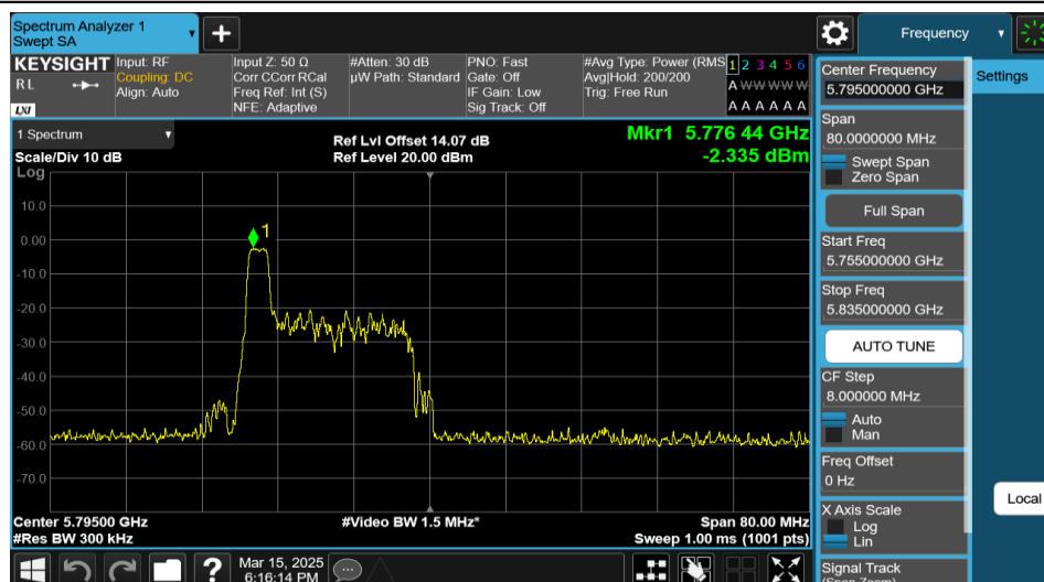
11AX40MIMO-Ant2-5795-26Tone-RU0-PASS
