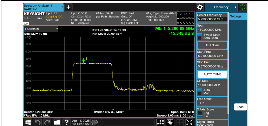
11AX80MIMO-Ant1-5290-484Tone-RU65-PASS
