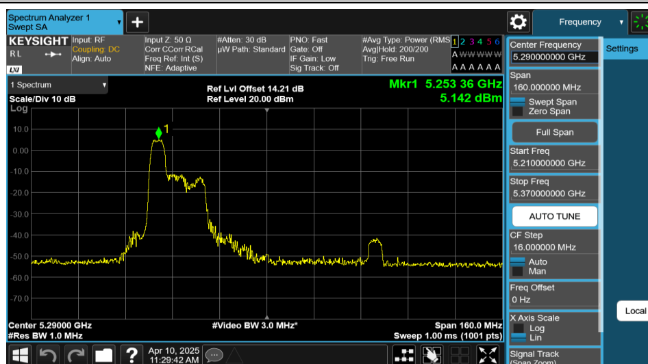
11AX80MIMO-Ant2-5290-52Tone-RU37-PASS
