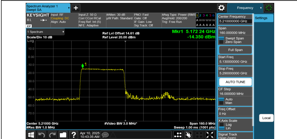
11AX80MIMO-Ant1-5210-484Tone-RU65-PASS
