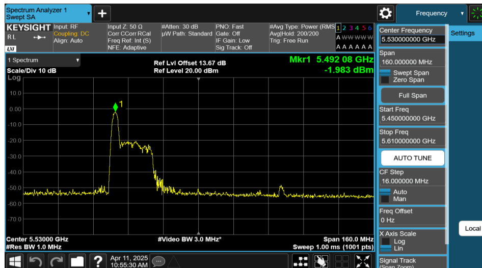
11AX80MIMO-Ant2-5530-26Tone-RU0-PASS
