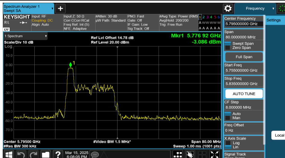
11AX40MIMO-Ant1-5795-26Tone-RU0-PASS
