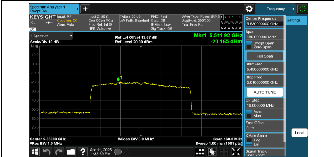
11AX80MIMO-Ant2-5530-996Tone-RU67-PASS
