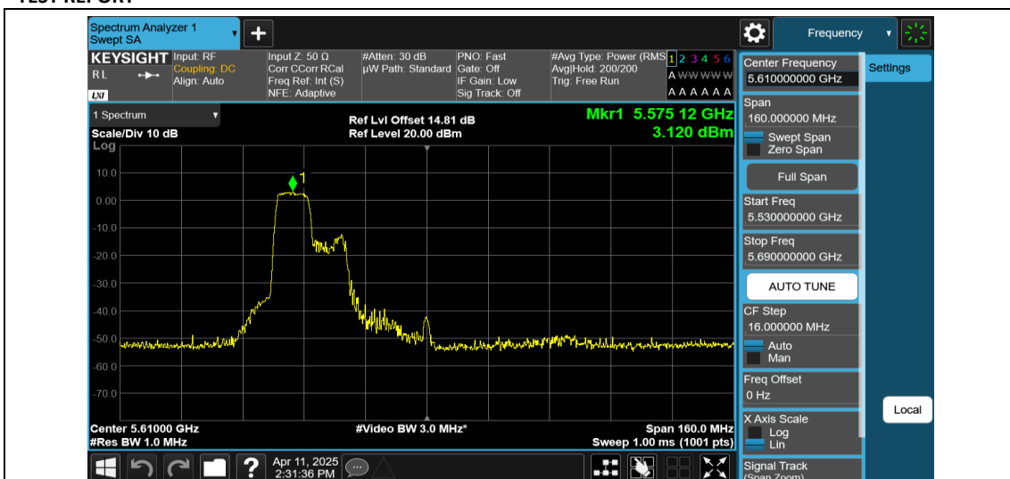
11AX80MIMO-Ant1-5610-106Tone-RU53-PASS
