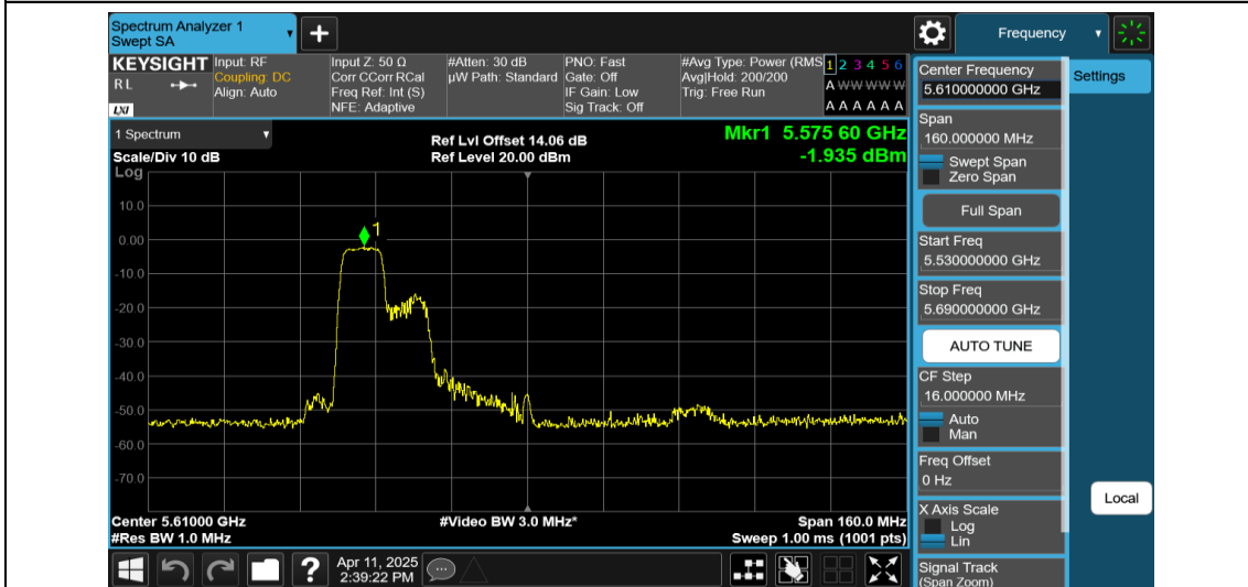
11AX80MIMO-Ant2-5610-106Tone-RU53-PASS
