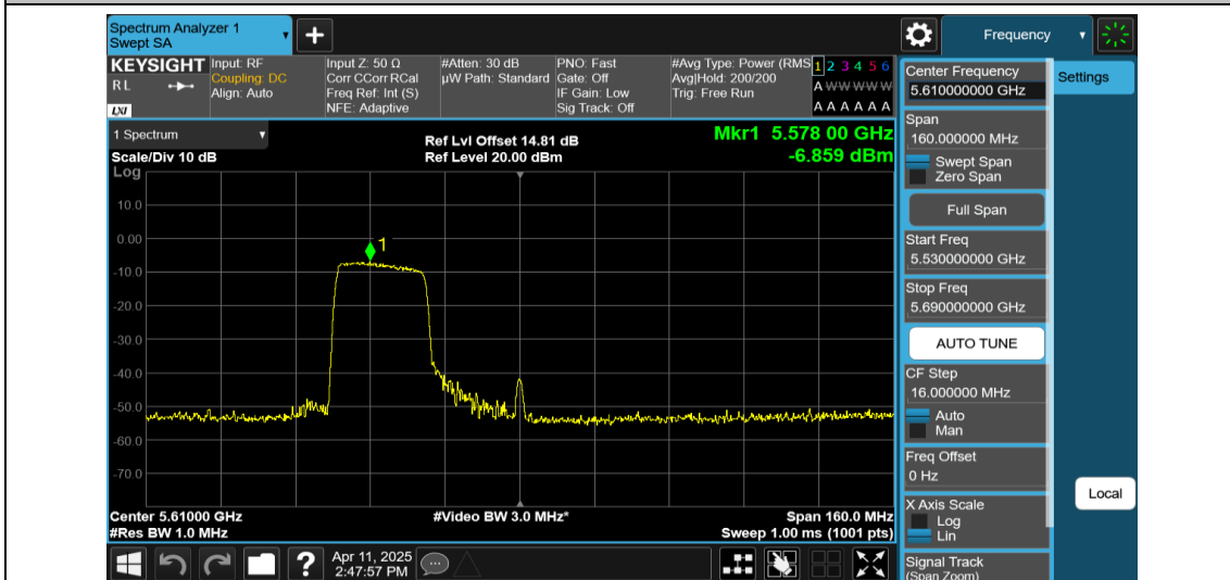
11AX80MIMO-Ant1-5610-242Tone-RU61-PASS
