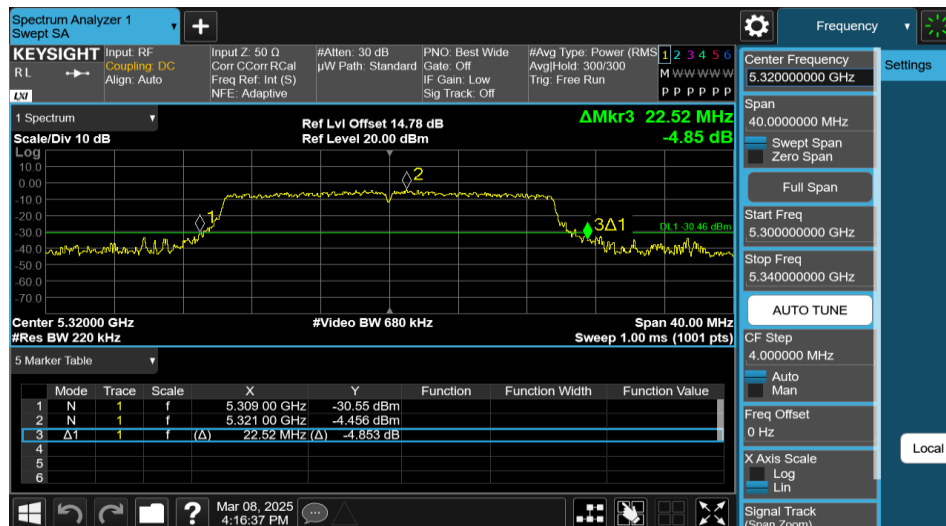
11AX20MIMO-Ant1-5320-242Tone-RU61
