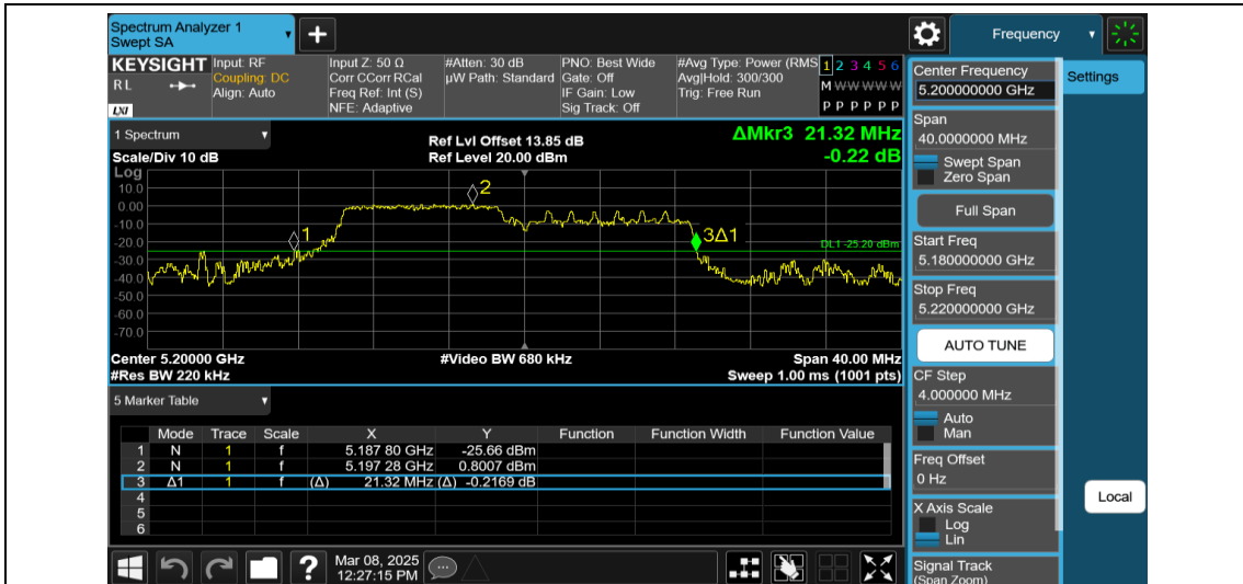
11AX20MIMO-Ant2-5200-106Tone-RU53
