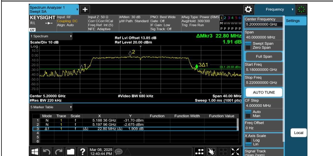
11AX20MIMO-Ant2-5200-242Tone-RU61
