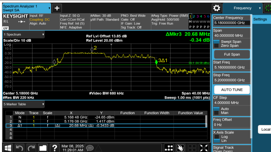
11AX20MIMO-Ant2-5180-106Tone-RU53
