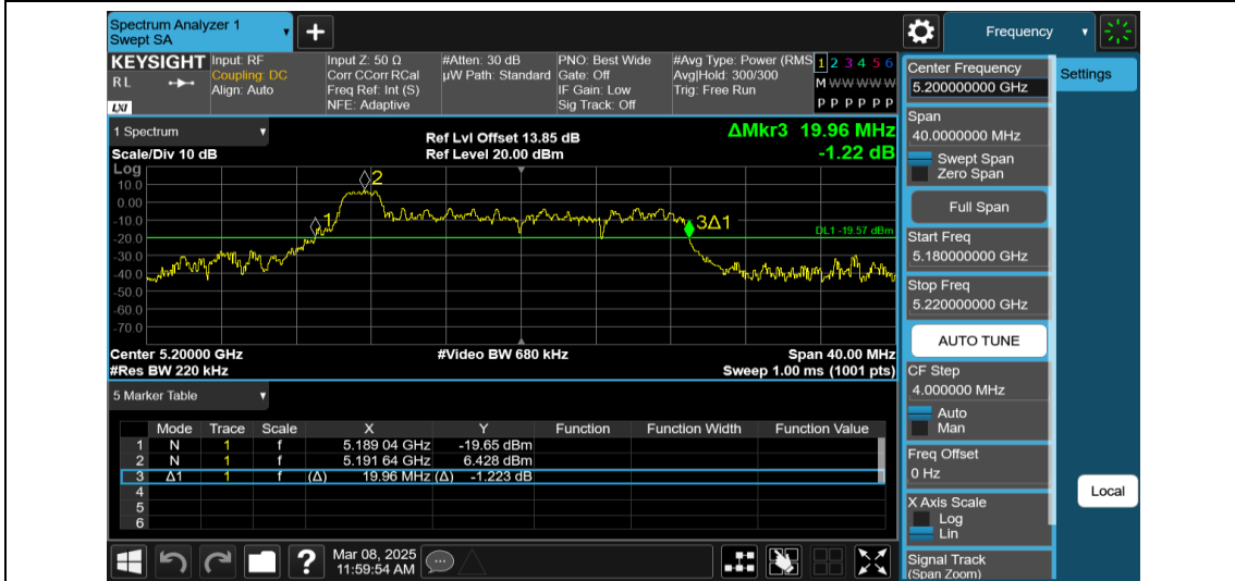
11AX20MIMO-Ant2-5200-26Tone-RU0
