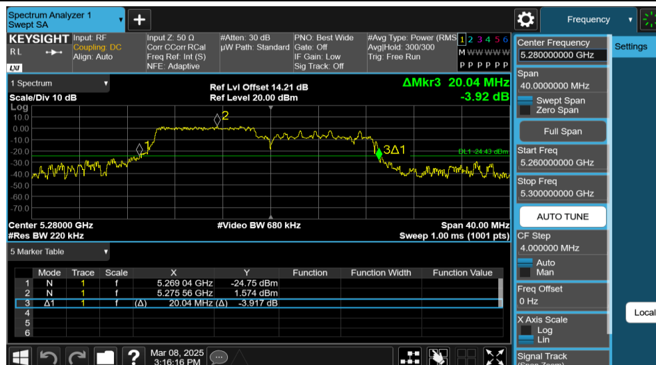
11AX20MIMO-Ant2-5280-106Tone-RU53
