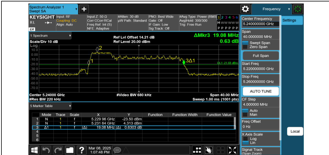
11AX20MIMO-Ant2-5240-52Tone-RU37
