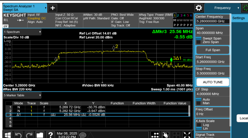
11AX20MIMO-Ant1-5280-242Tone-RU61
