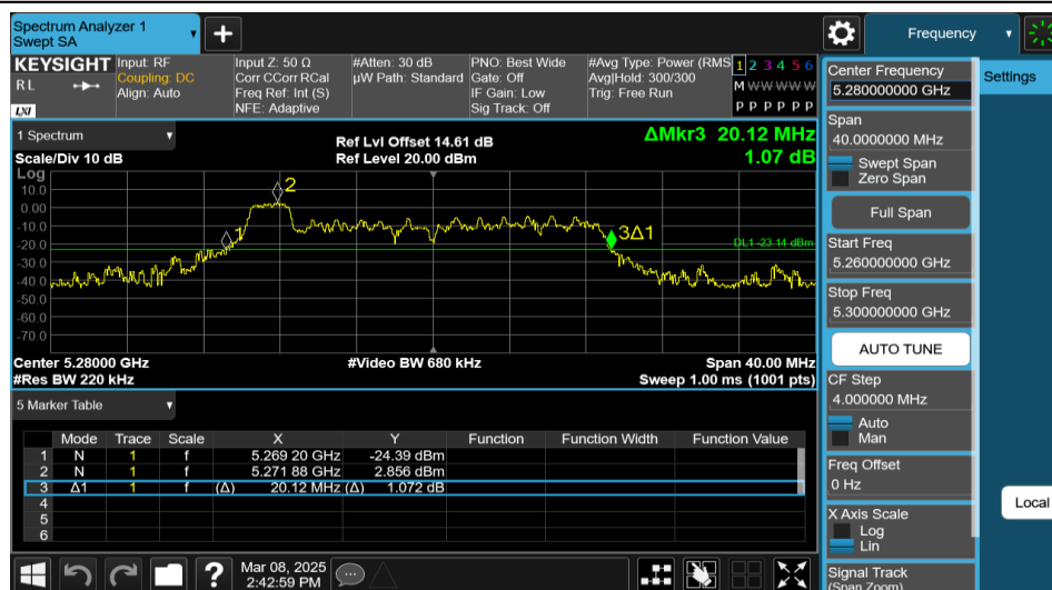
11AX20MIMO-Ant1-5280-26Tone-RU0
