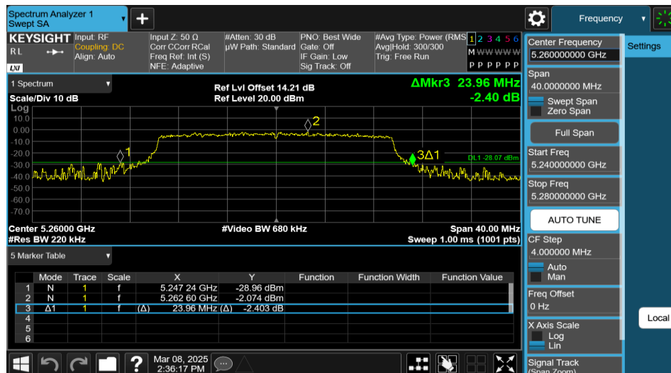
11AX20MIMO-Ant2-5260-242Tone-RU61
