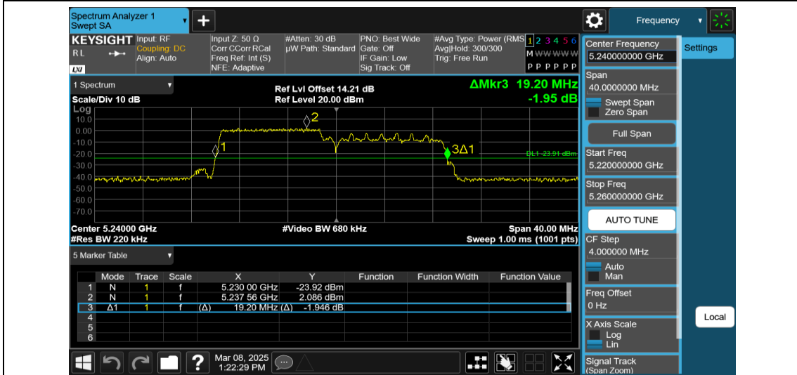
11AX20MIMO-Ant2-5240-106Tone-RU53
