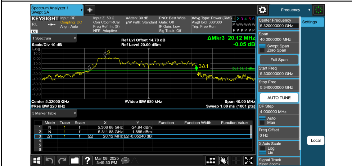
11AX20MIMO-Ant1-5320-52Tone-RU37
