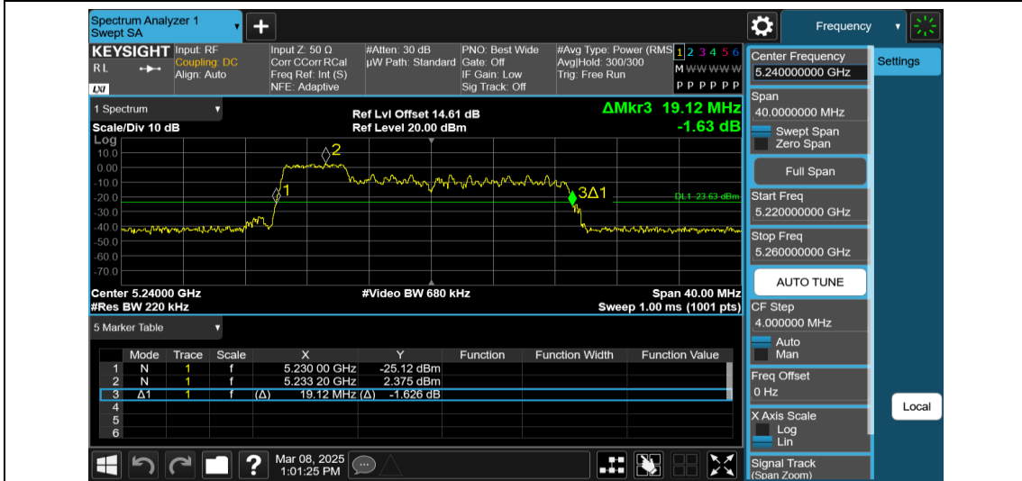
11AX20MIMO-Ant1-5240-52Tone-RU37
