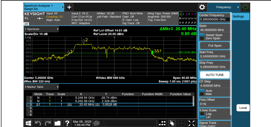
11AX20MIMO-Ant1-5260-52Tone-RU37
