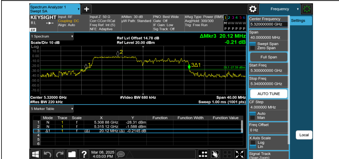
11AX20MIMO-Ant1-5320-106Tone-RU53
