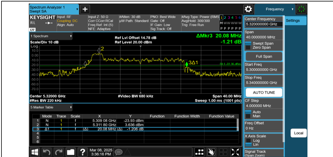
11AX20MIMO-Ant1-5320-26Tone-RU0
