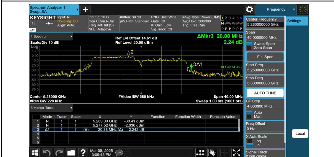
11AX20MIMO-Ant1-5280-106Tone-RU53
