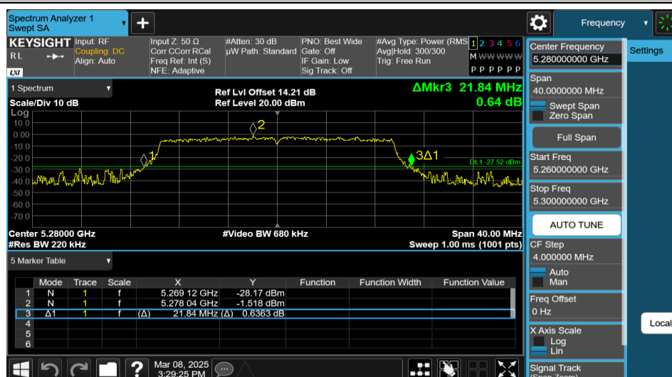
11AX20MIMO-Ant2-5280-242Tone-RU61
