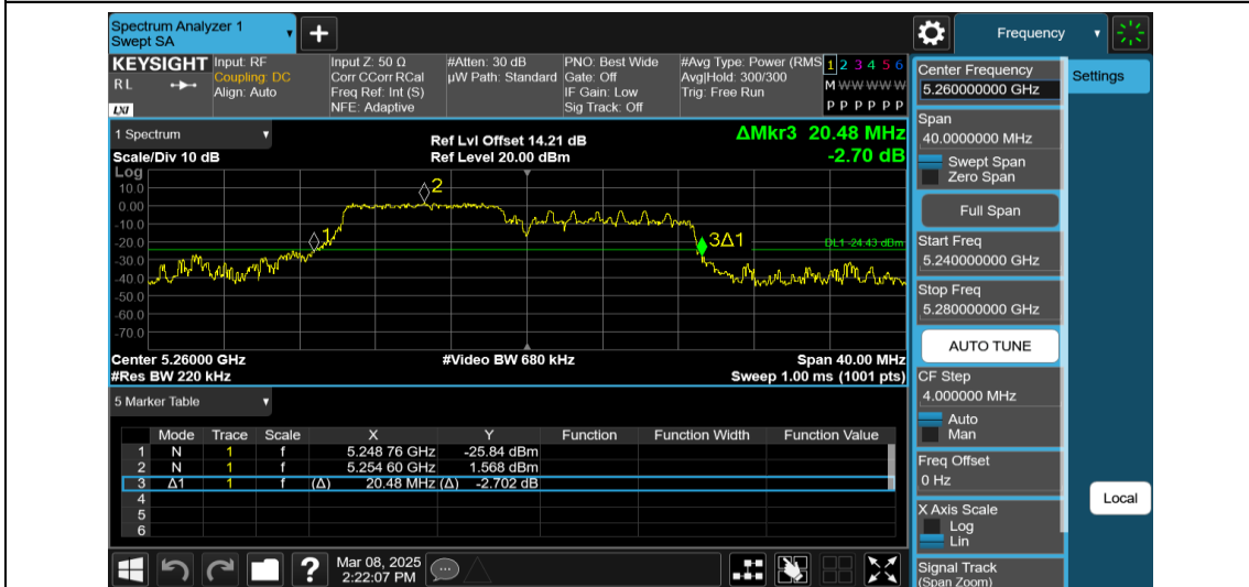
11AX20MIMO-Ant2-5260-106Tone-RU53
