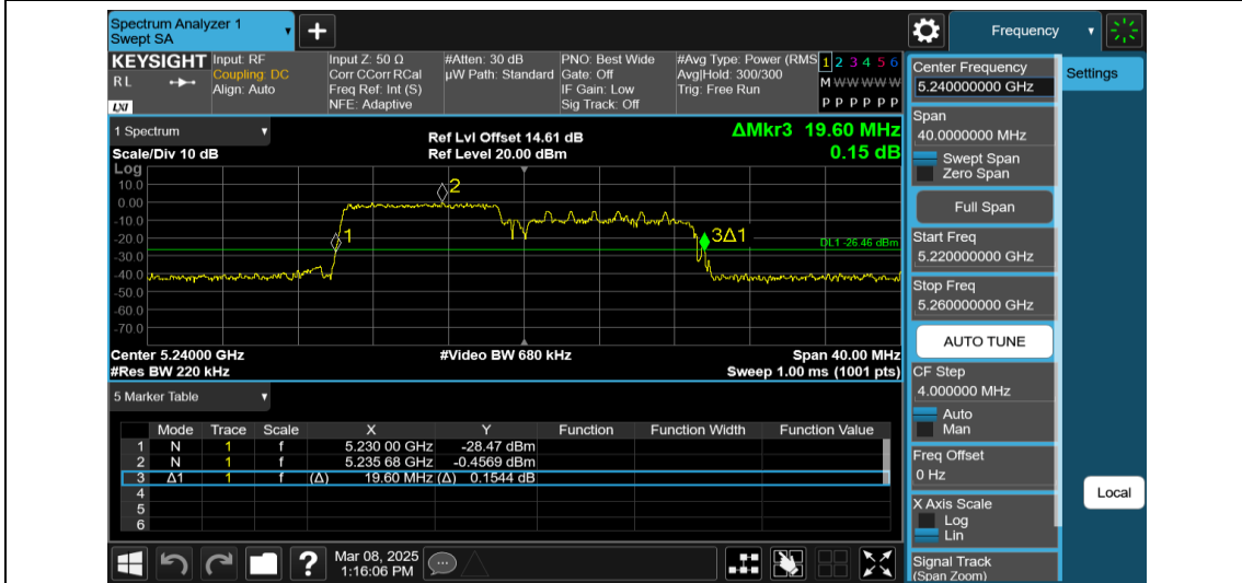
11AX20MIMO-Ant1-5240-106Tone-RU53
