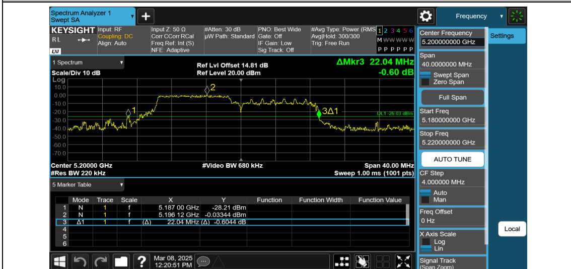
11AX20MIMO-Ant1-5200-106Tone-RU53
