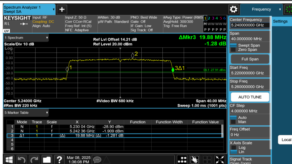
11AX20MIMO-Ant2-5240-242Tone-RU61
