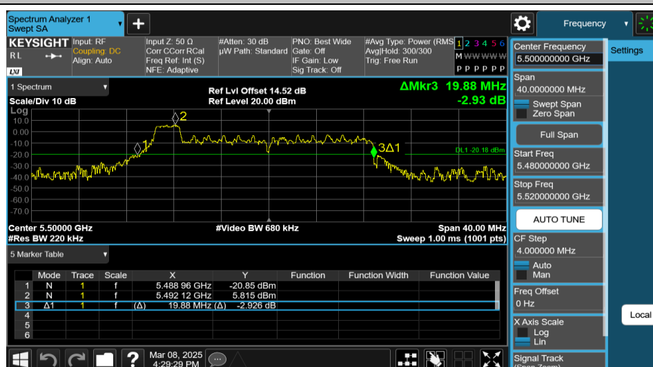
11AX20MIMO-Ant1-5500-26Tone-RU0
