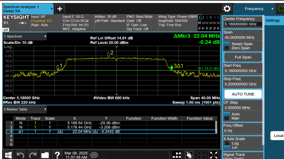
11AX20MIMO-Ant1-5180-242Tone-RU61
