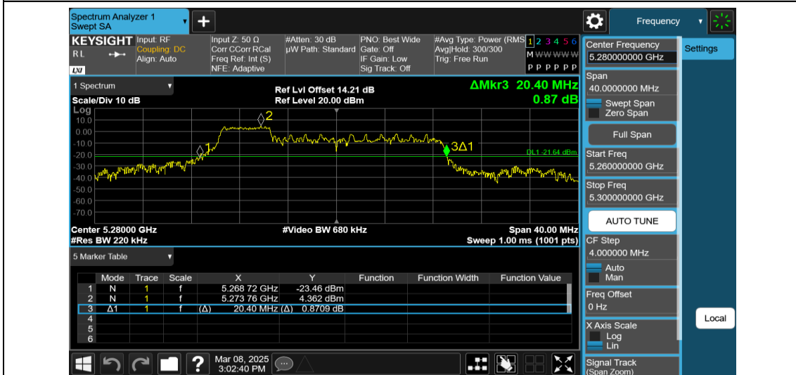
11AX20MIMO-Ant2-5280-52Tone-RU37
