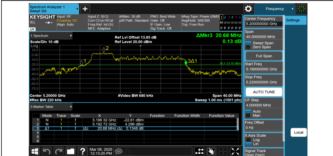
11AX20MIMO-Ant2-5200-52Tone-RU37
