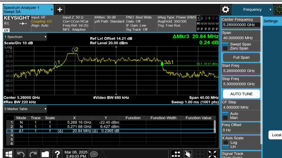
11AX20MIMO-Ant2-5280-26Tone-RU0
