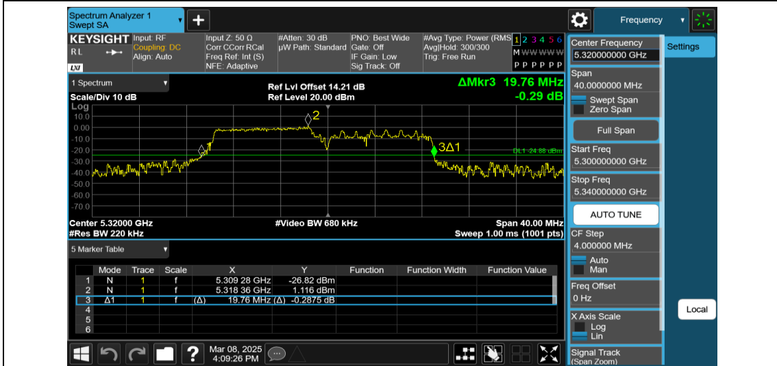
11AX20MIMO-Ant2-5320-106Tone-RU53
