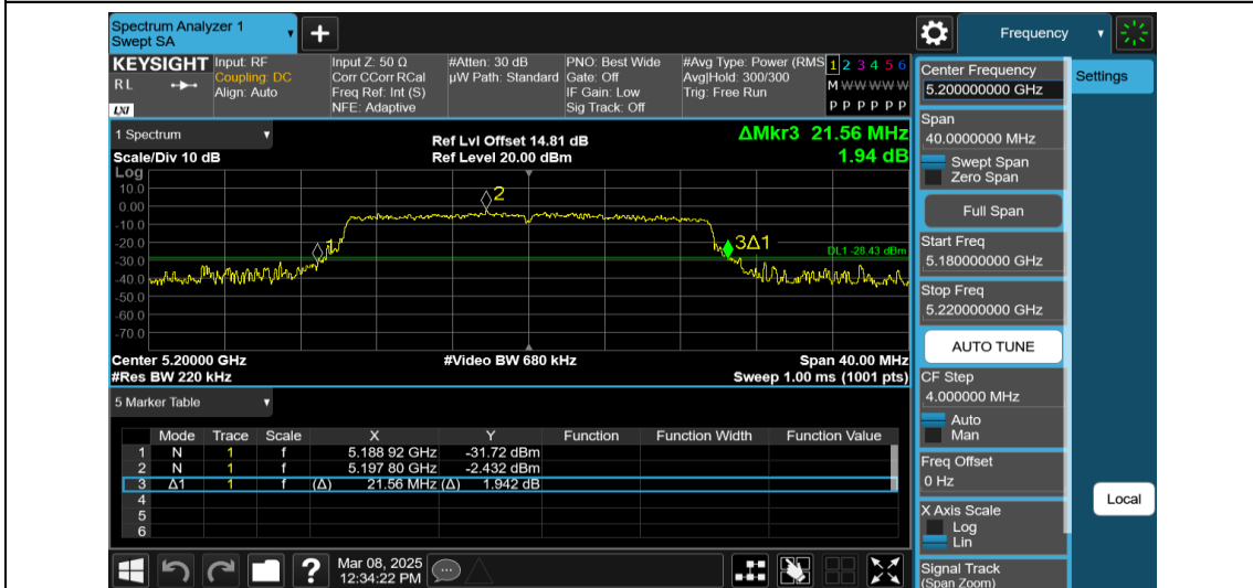
11AX20MIMO-Ant1-5200-242Tone-RU61
