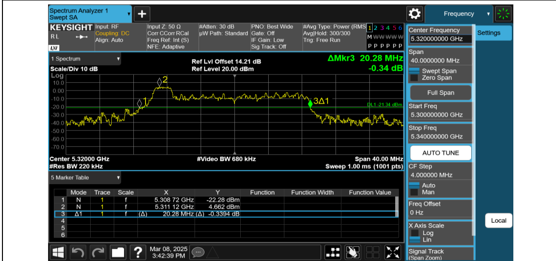
11AX20MIMO-Ant2-5320-26Tone-RU0
