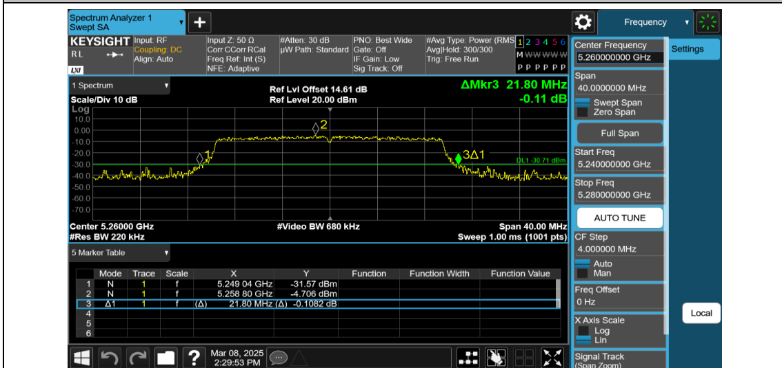
11AX20MIMO-Ant1-5260-242Tone-RU61
