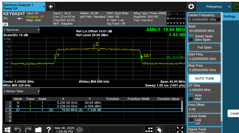
11AX20MIMO-Ant1-5240-242Tone-RU61
