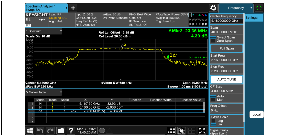
11AX20MIMO-Ant2-5180-242Tone-RU61
