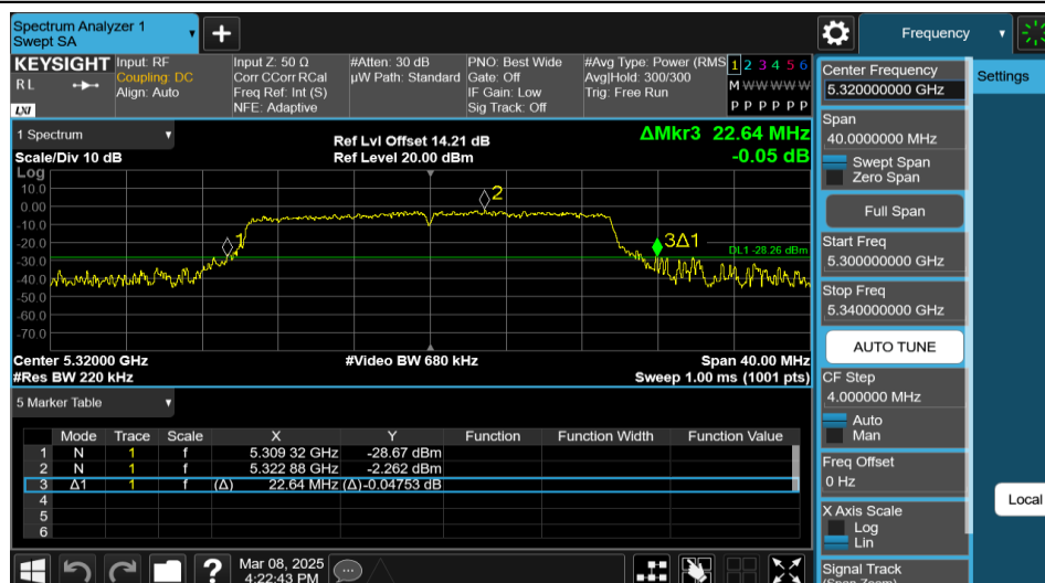
11AX20MIMO-Ant2-5320-242Tone-RU61
