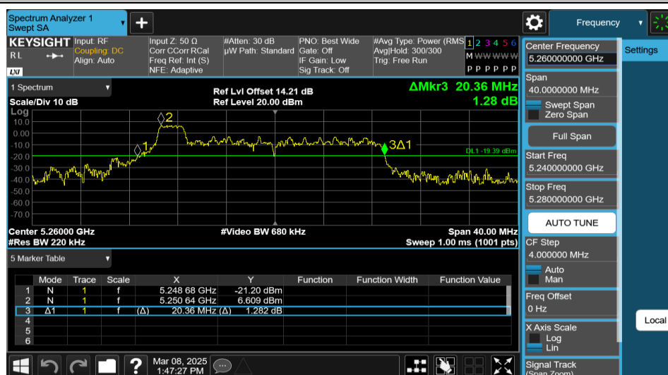
11AX20MIMO-Ant2-5260-26Tone-RU0
