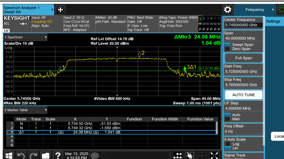
11AX20MIMO-Ant1-5745-242Tone-RU61
