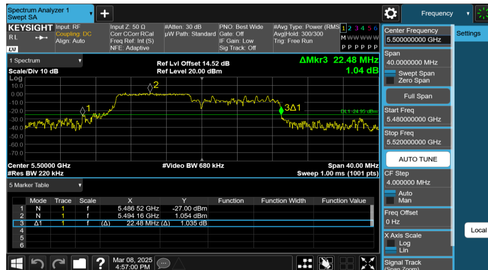
11AX20MIMO-Ant1-5500-106Tone-RU53
