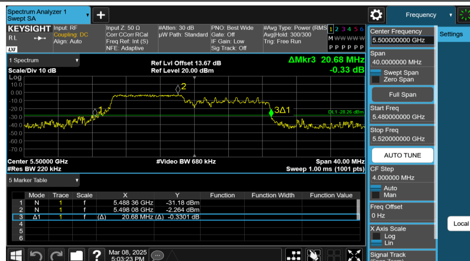
11AX20MIMO-Ant2-5500-106Tone-RU53
