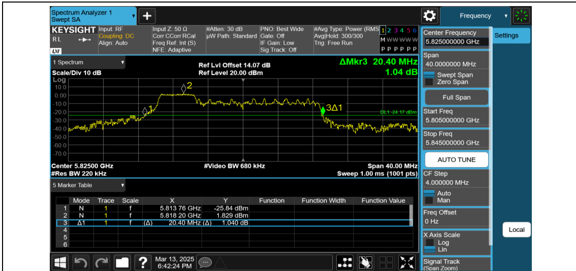
11AX20MIMO-Ant2-5825-52Tone-RU37
