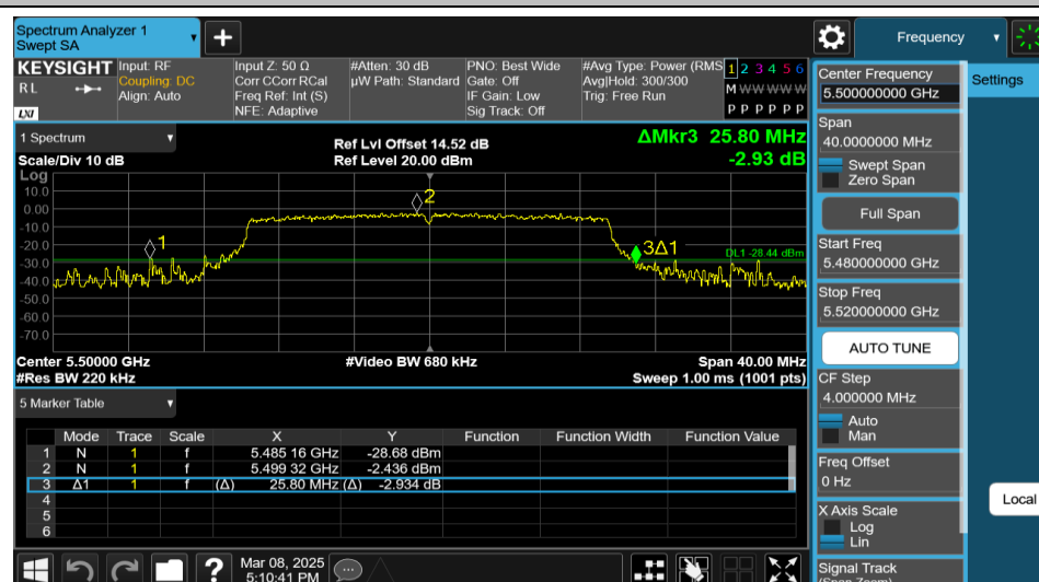
11AX20MIMO-Ant1-5500-242Tone-RU61
