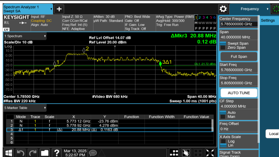
11AX20MIMO-Ant2-5785-52Tone-RU37
