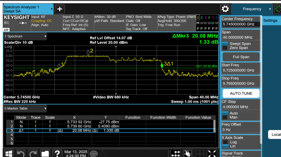
11AX20MIMO-Ant2-5745-106Tone-RU53
