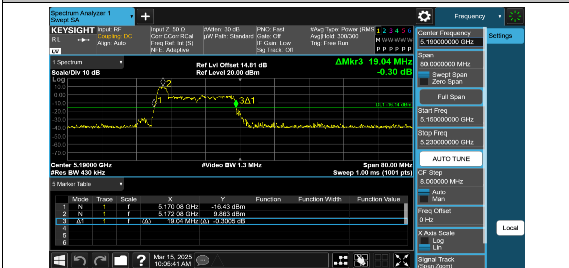
11AX40MIMO-Ant1-5190-26Tone-RU0
