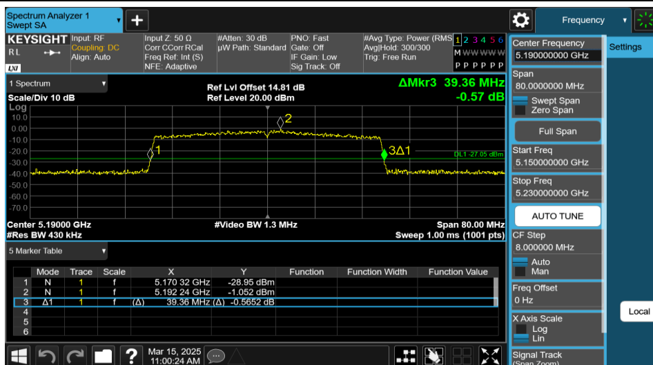
11AX40MIMO-Ant1-5190-484Tone-RU65
