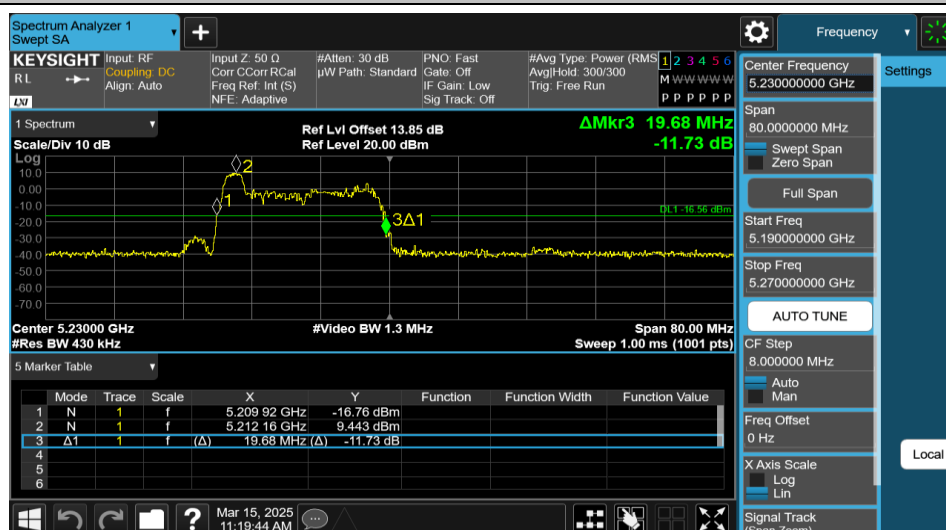
11AX40MIMO-Ant2-5230-26Tone-RU0
