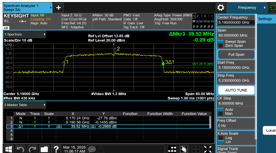
11AX40MIMO-Ant2-5190-484Tone-RU65
