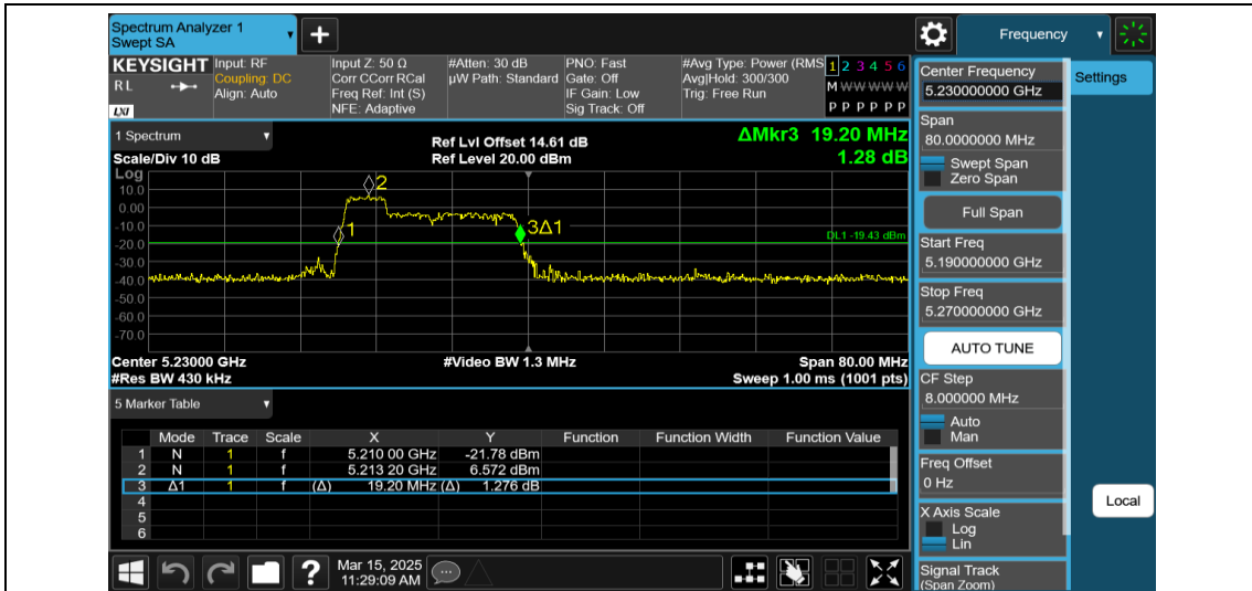
11AX40MIMO-Ant1-5230-52Tone-RU37
