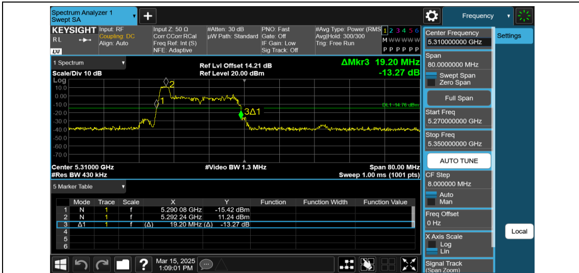
11AX40MIMO-Ant2-5310-26Tone-RU0
