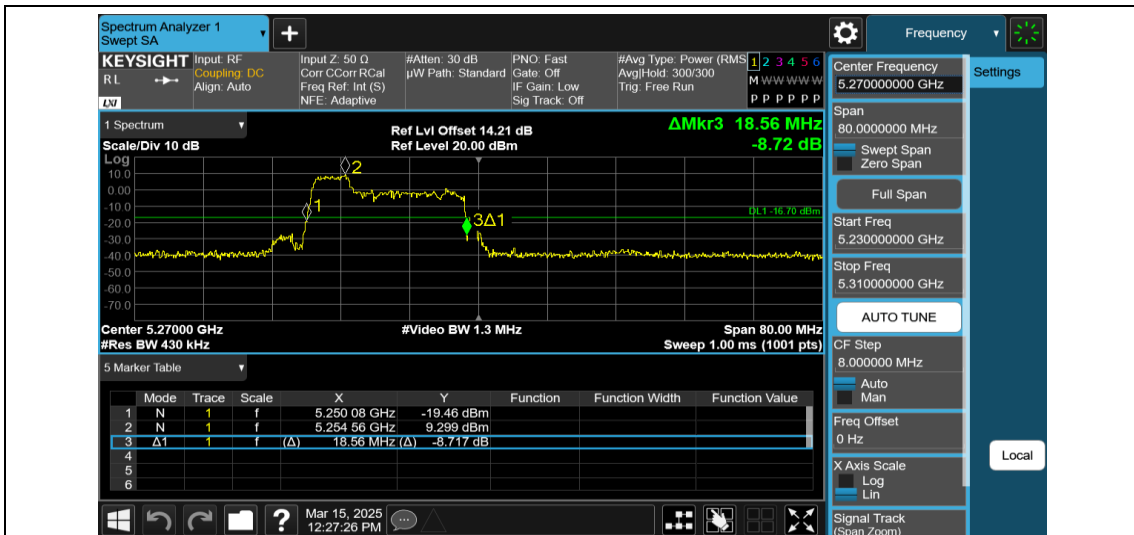
11AX40MIMO-Ant2-5270-52Tone-RU37
