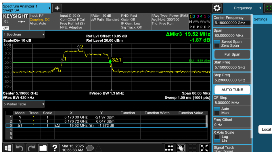
11AX40MIMO-Ant2-5190-106Tone-RU53
