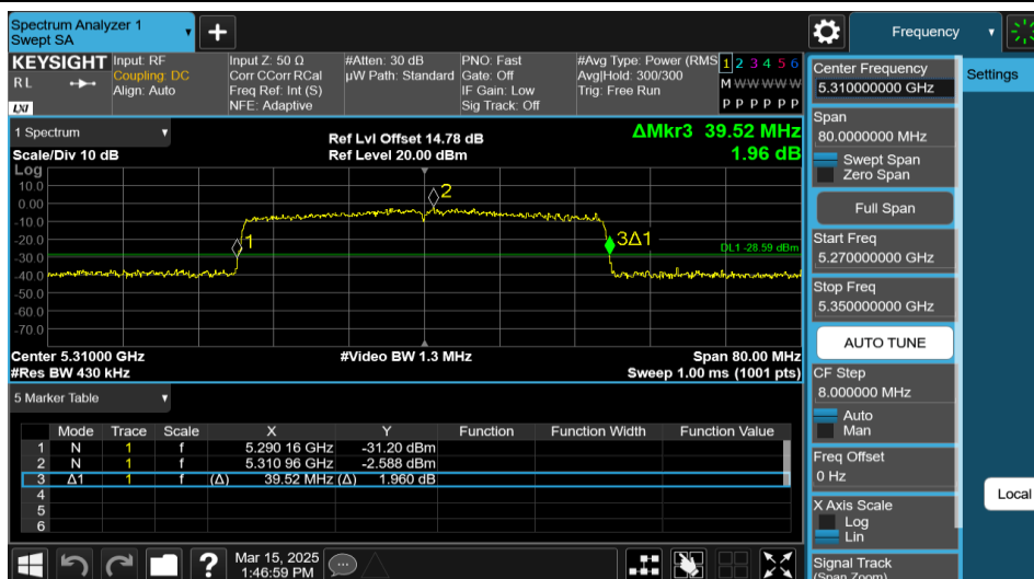
11AX40MIMO-Ant1-5310-484Tone-RU65
