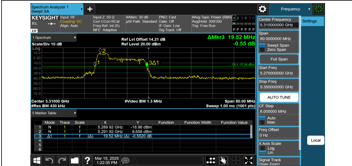
11AX40MIMO-Ant2-5310-52Tone-RU37
