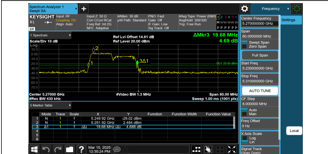
11AX40MIMO-Ant1-5270-106Tone-RU53
