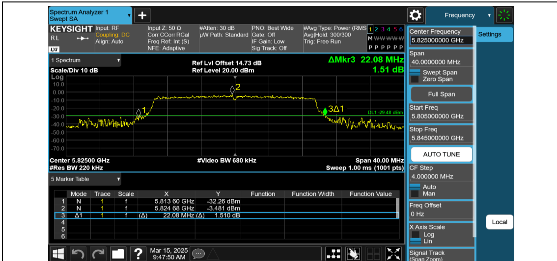
11AX20MIMO-Ant1-5825-242Tone-RU61
