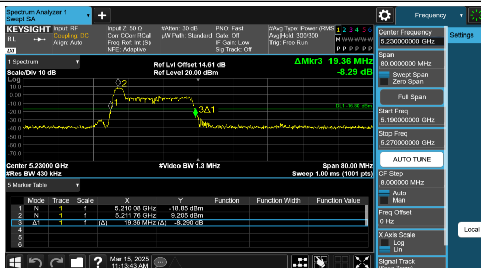
11AX40MIMO-Ant1-5230-26Tone-RU0
