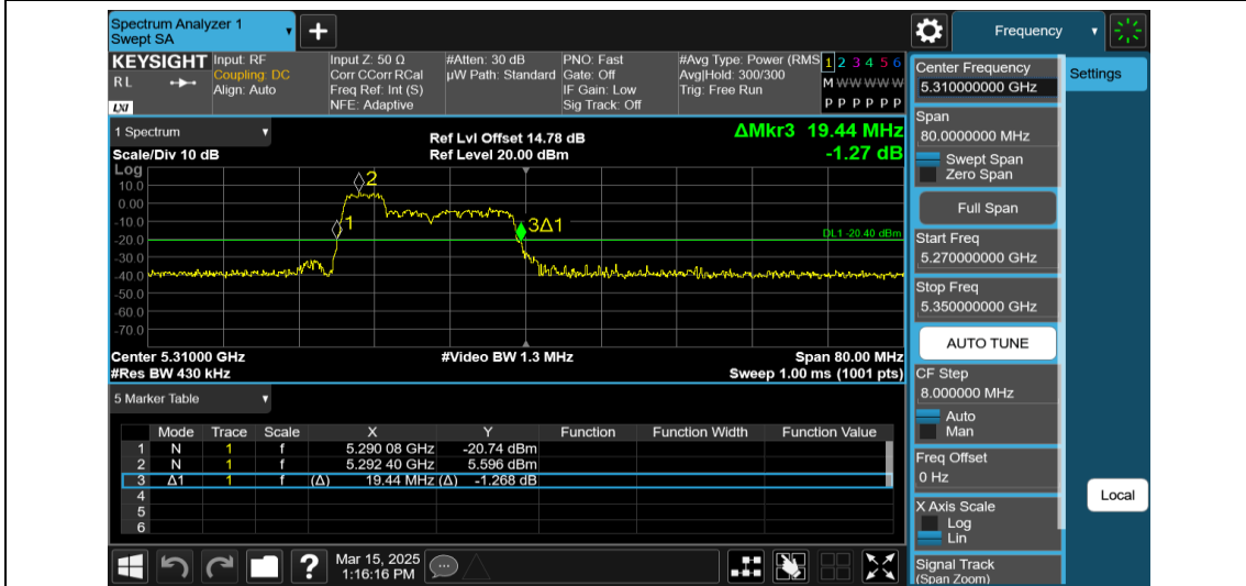
11AX40MIMO-Ant1-5310-52Tone-RU37
