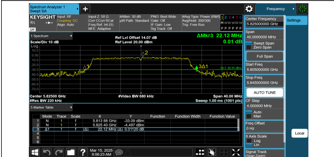
11AX20MIMO-Ant2-5825-242Tone-RU61
