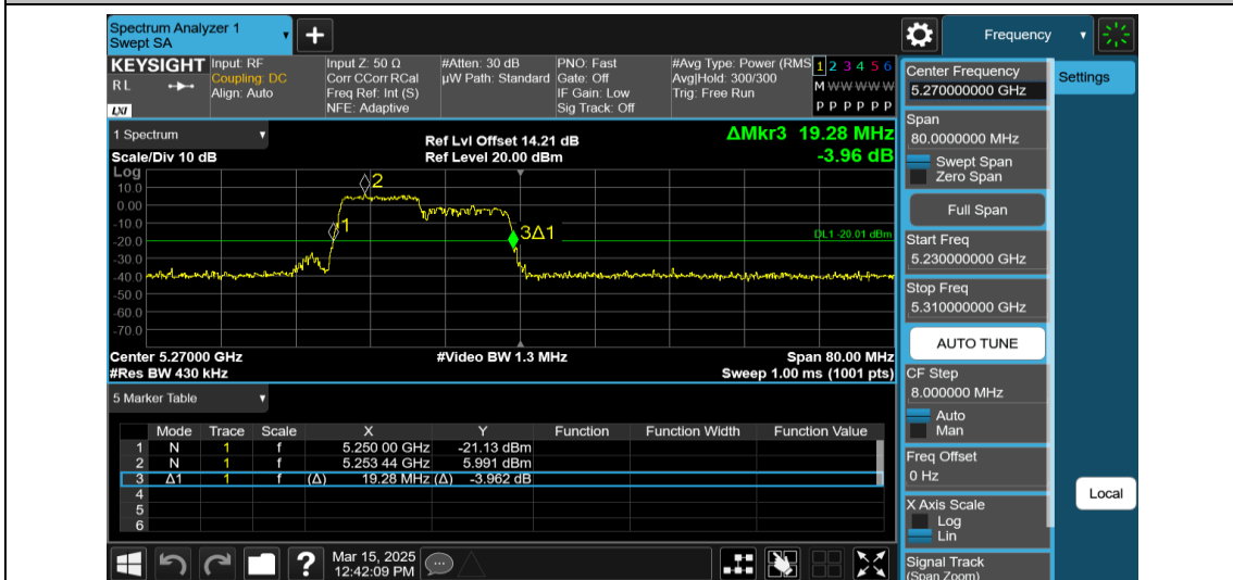
11AX40MIMO-Ant2-5270-106Tone-RU53
