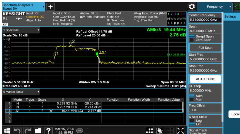
11AX40MIMO-Ant1-5310-106Tone-RU53
