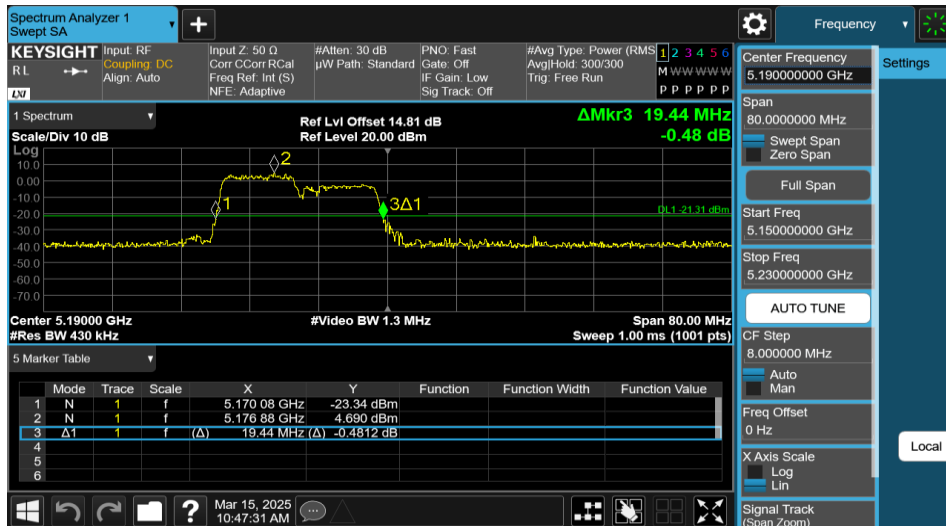
11AX40MIMO-Ant1-5190-106Tone-RU53
