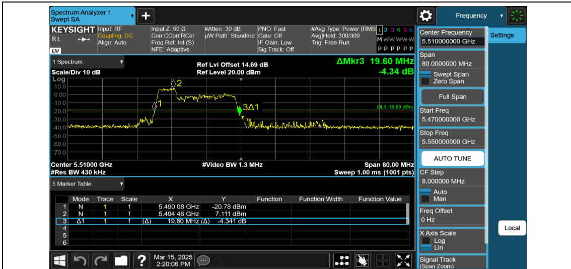
11AX40MIMO-Ant1-5510-52Tone-RU37
