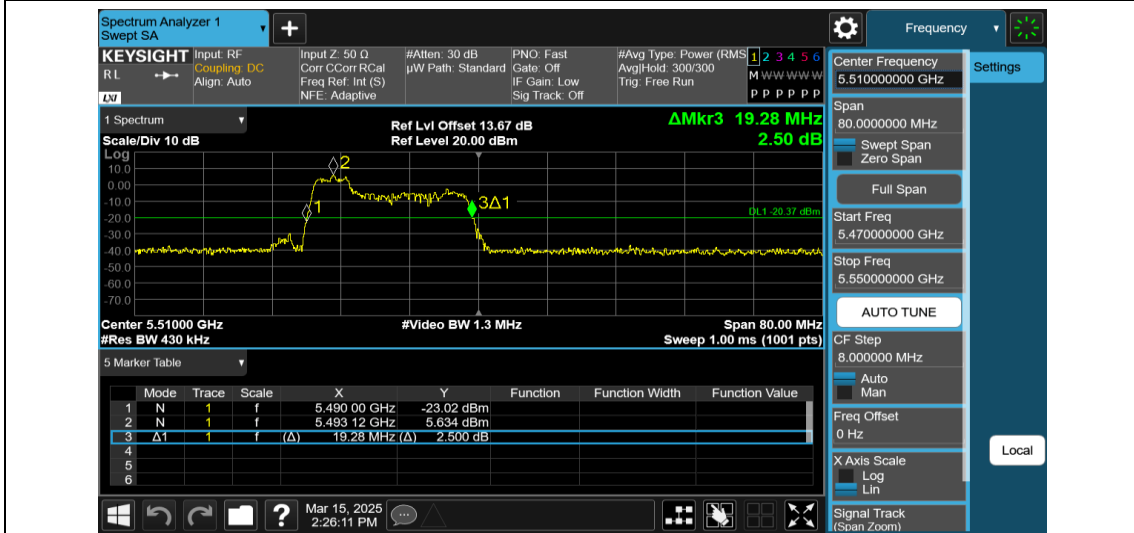
11AX40MIMO-Ant2-5510-52Tone-RU37
