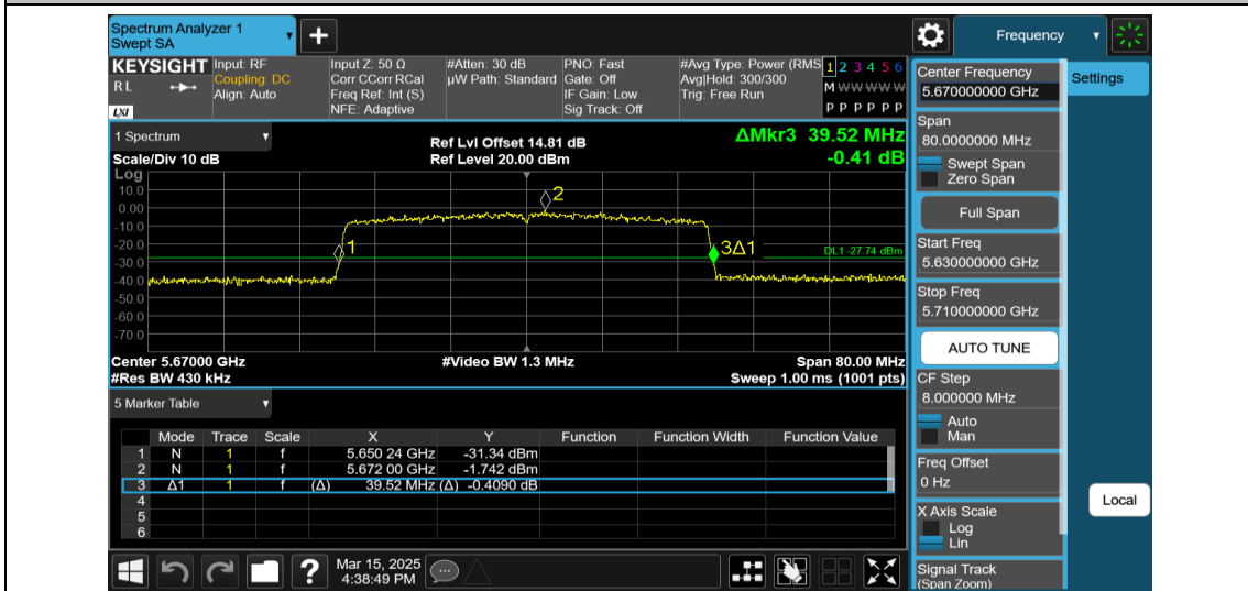
11AX40MIMO-Ant1-5670-484Tone-RU65
