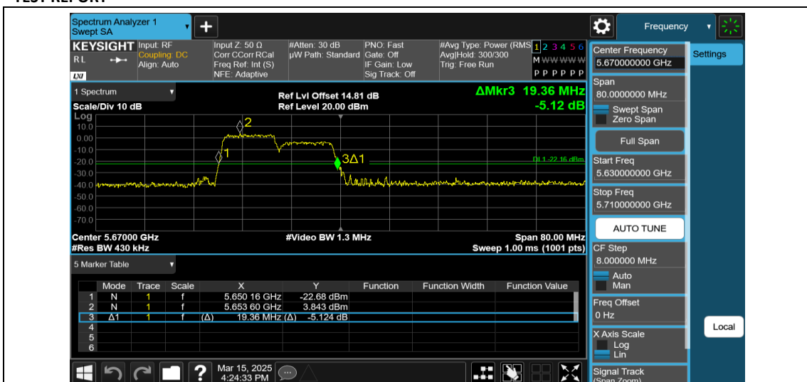
11AX40MIMO-Ant1-5670-106Tone-RU53
