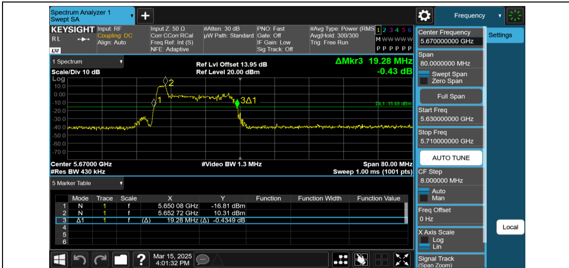
11AX40MIMO-Ant2-5670-26Tone-RU0
