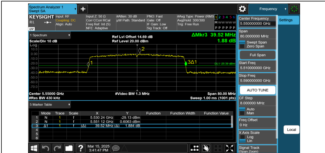
11AX40MIMO-Ant1-5550-484Tone-RU65
