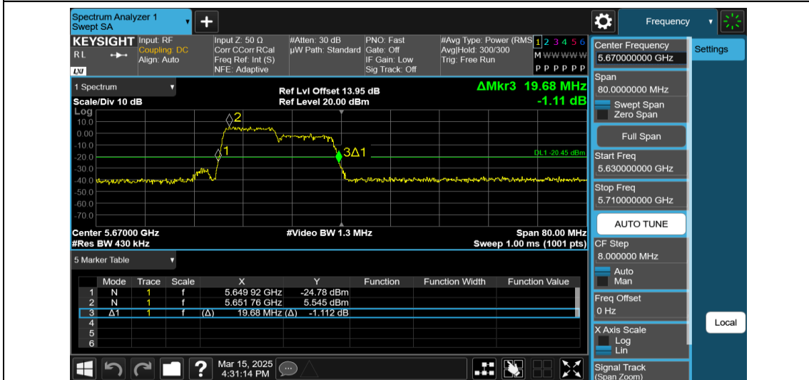
11AX40MIMO-Ant2-5670-106Tone-RU53
