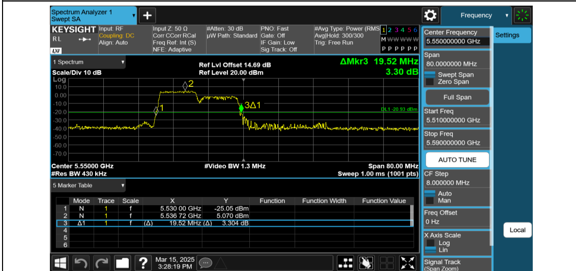
11AX40MIMO-Ant1-5550-106Tone-RU53
