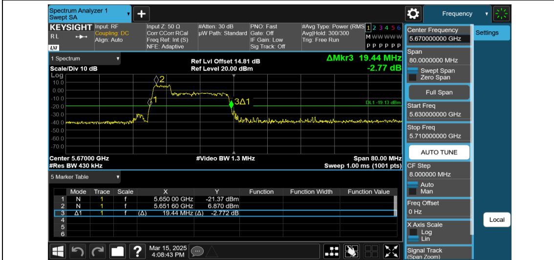
11AX40MIMO-Ant1-5670-52Tone-RU37
