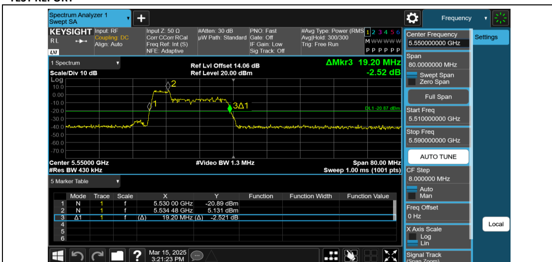
11AX40MIMO-Ant2-5550-52Tone-RU37
