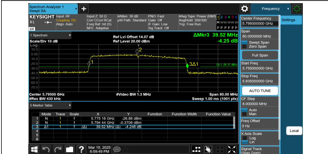
11AX40MIMO-Ant2-5795-484Tone-RU65
