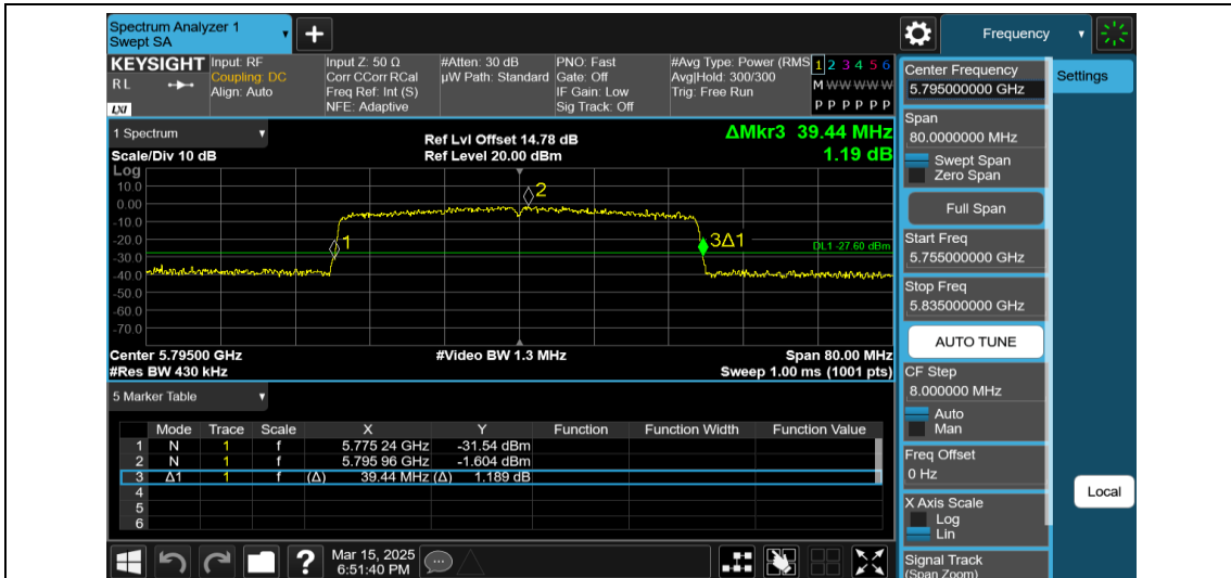
11AX40MIMO-Ant1-5795-484Tone-RU65
