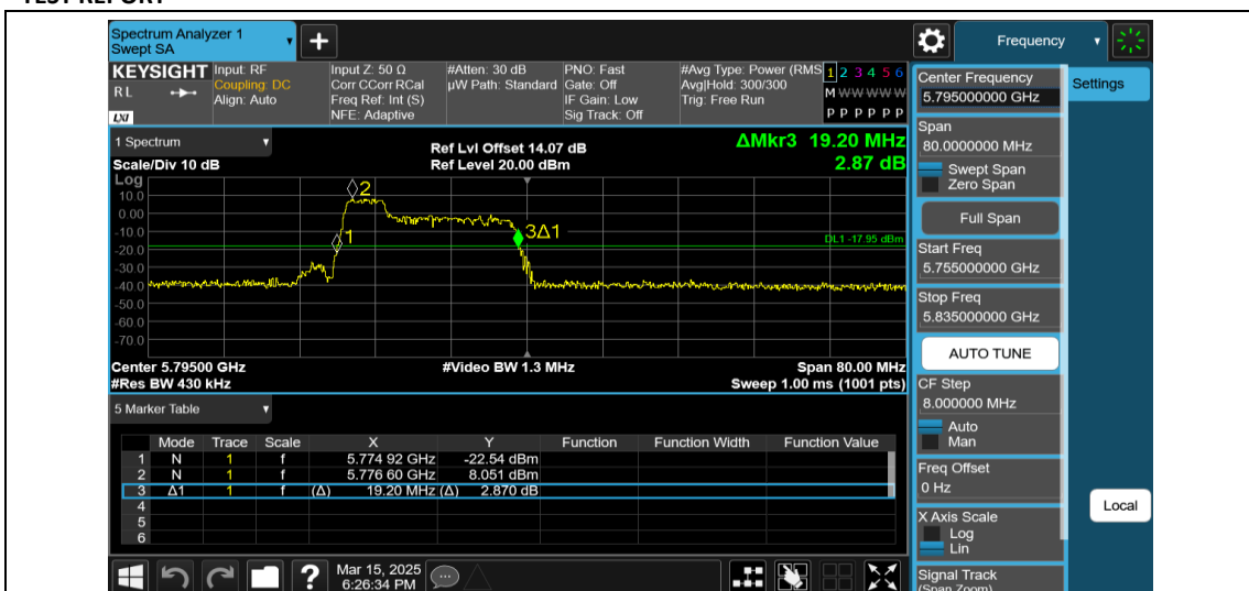
11AX40MIMO-Ant2-5795-52Tone-RU37
