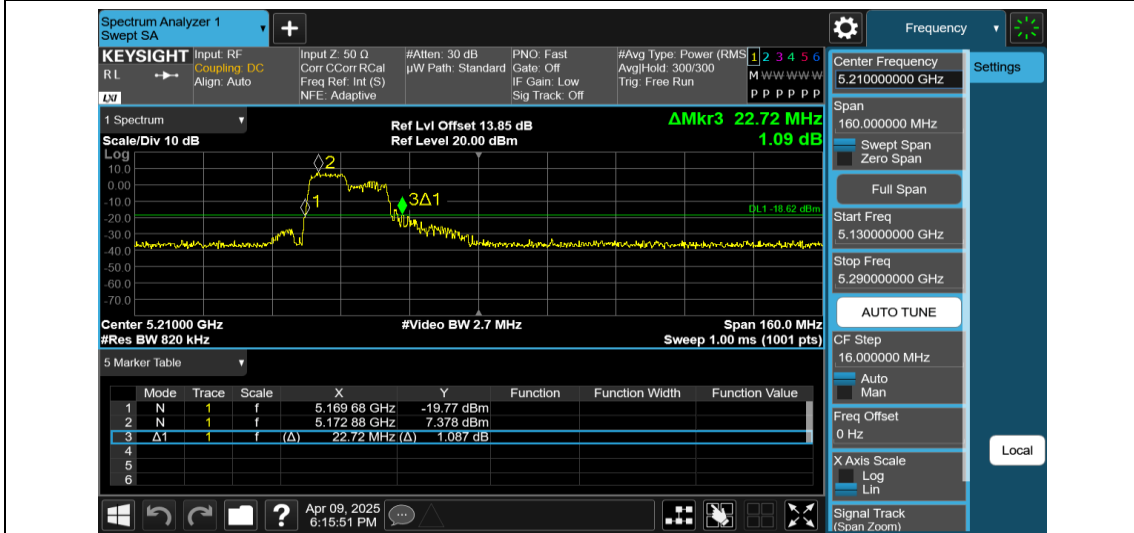
11AX80MIMO-Ant2-5210-106Tone-RU53
