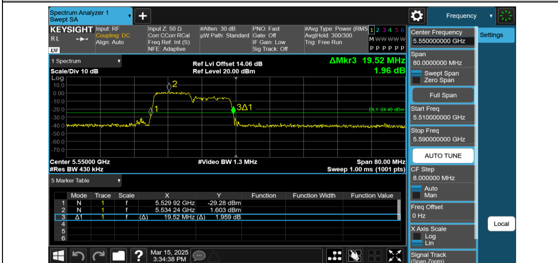
11AX40MIMO-Ant2-5550-106Tone-RU53
