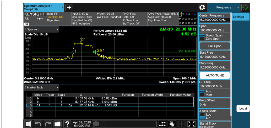
11AX80MIMO-Ant1-5210-106Tone-RU53
