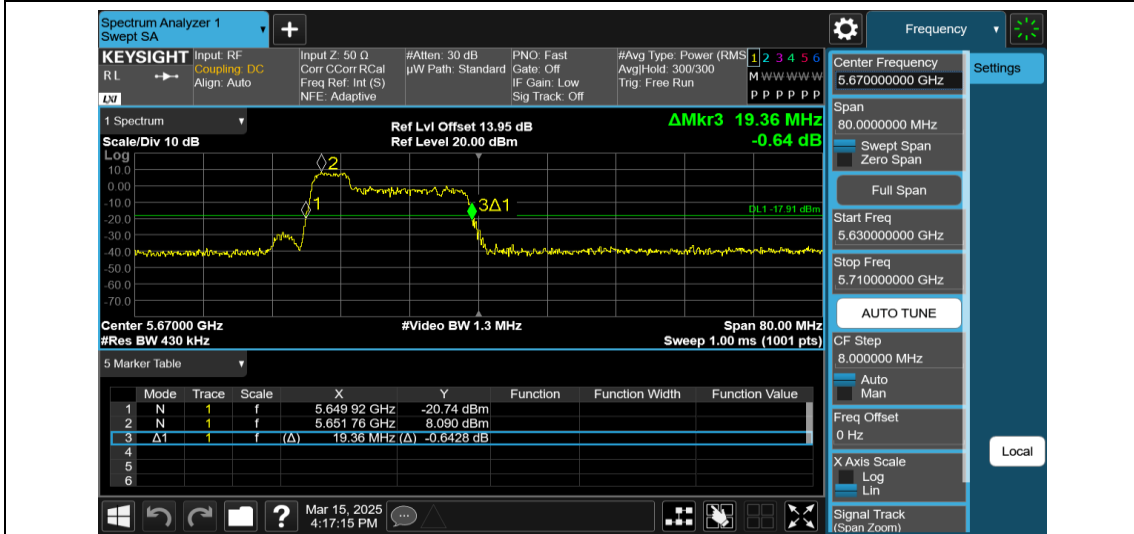
11AX40MIMO-Ant2-5670-52Tone-RU37
