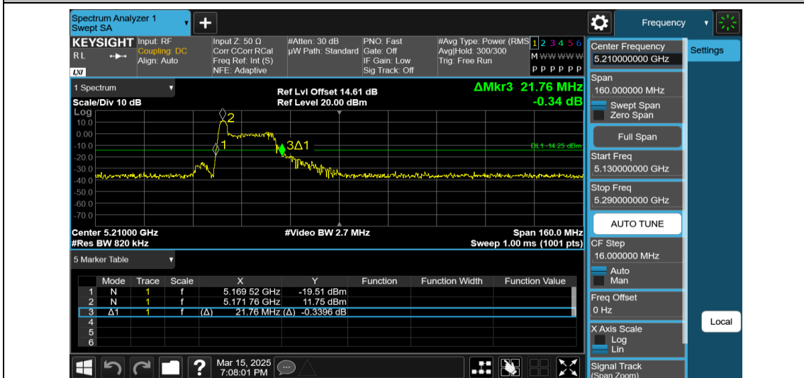
11AX80MIMO-Ant1-5210-26Tone-RU0
