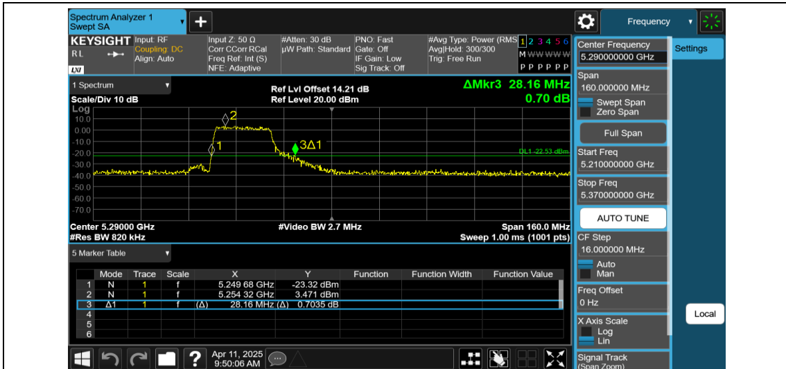
11AX80MIMO-Ant2-5290-242Tone-RU61
