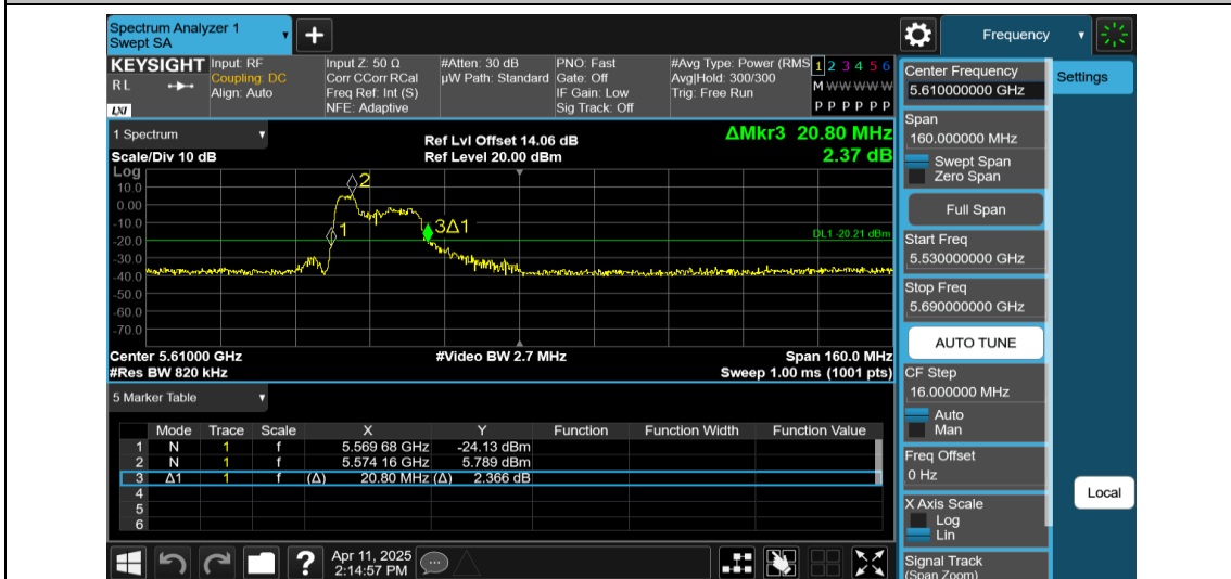
11AX80MIMO-Ant2-5610-52Tone-RU37
