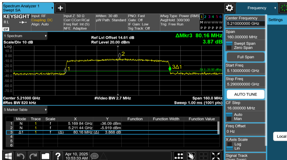
11AX80MIMO-Ant1-5210-996Tone-RU67
