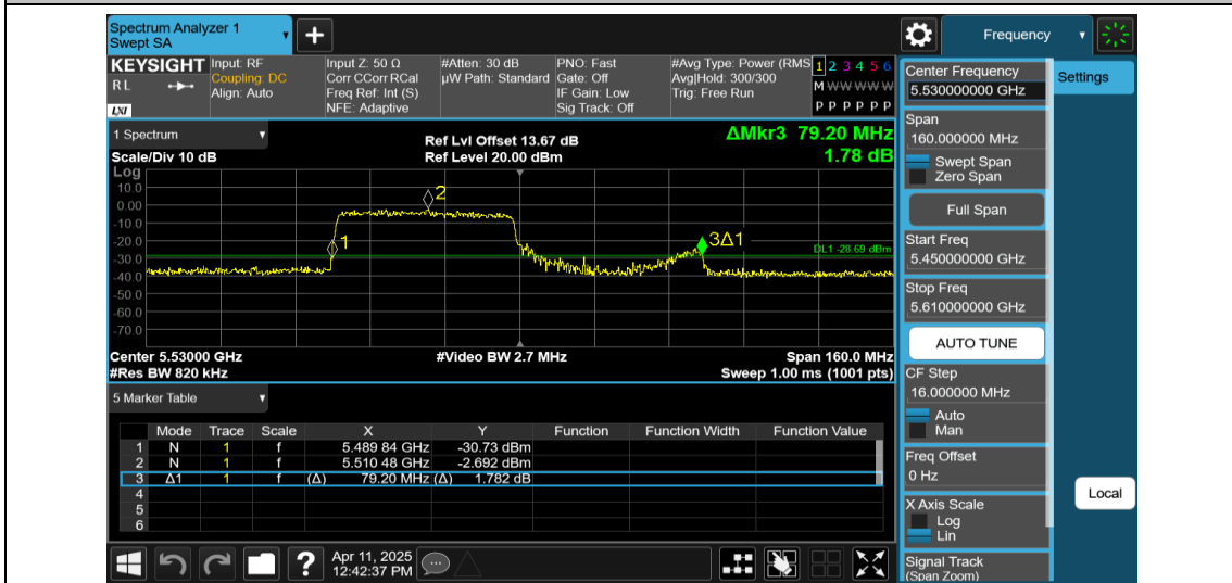
11AX80MIMO-Ant2-5530-484Tone-RU65
