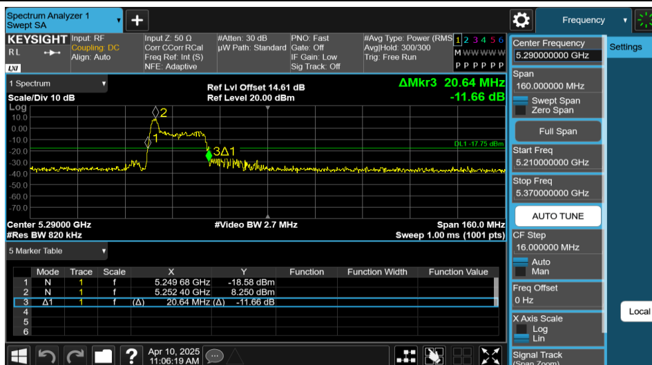
11AX80MIMO-Ant1-5290-26Tone-RU0
