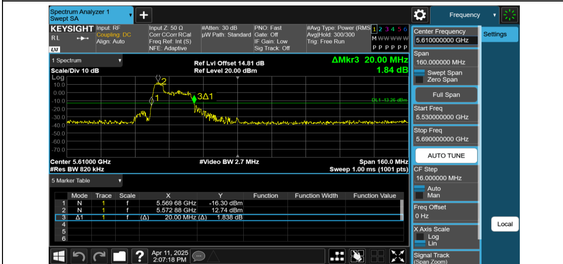
11AX80MIMO-Ant1-5610-52Tone-RU37
