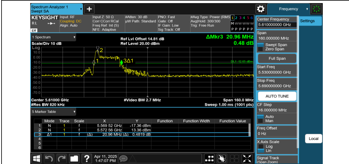
11AX80MIMO-Ant1-5610-26Tone-RU0
