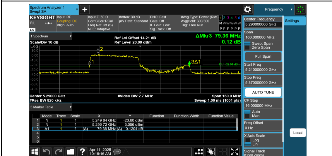
11AX80MIMO-Ant2-5290-484Tone-RU65
