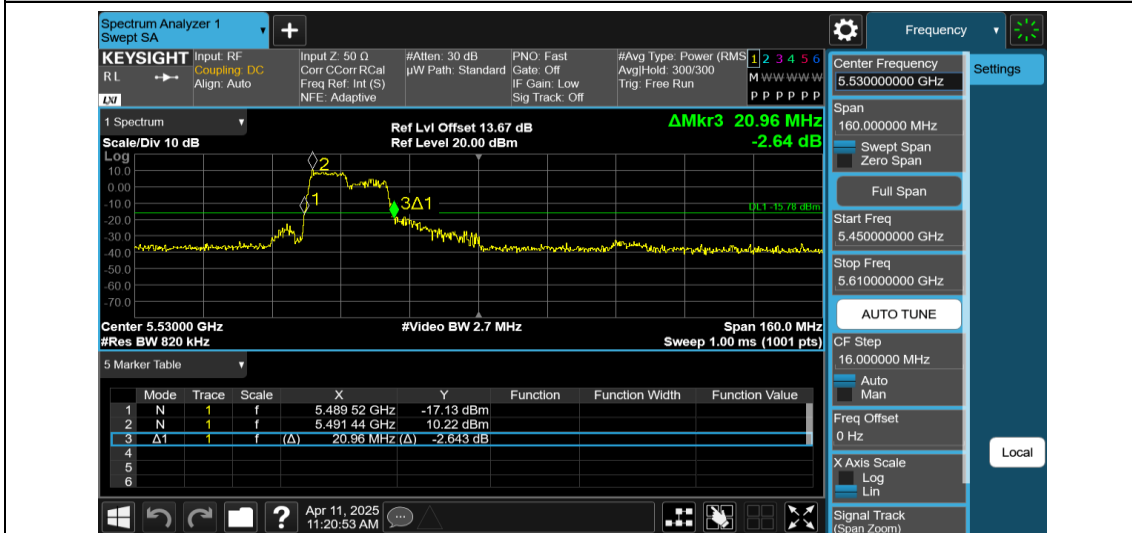
11AX80MIMO-Ant2-5530-106Tone-RU53
