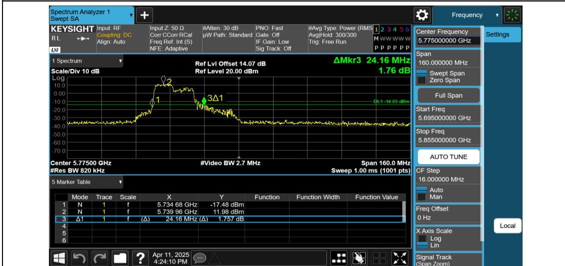
11AX80MIMO-Ant2-5775-106Tone-RU53
