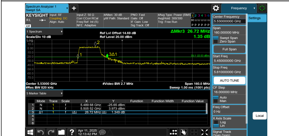
11AX80MIMO-Ant1-5530-242Tone-RU61
