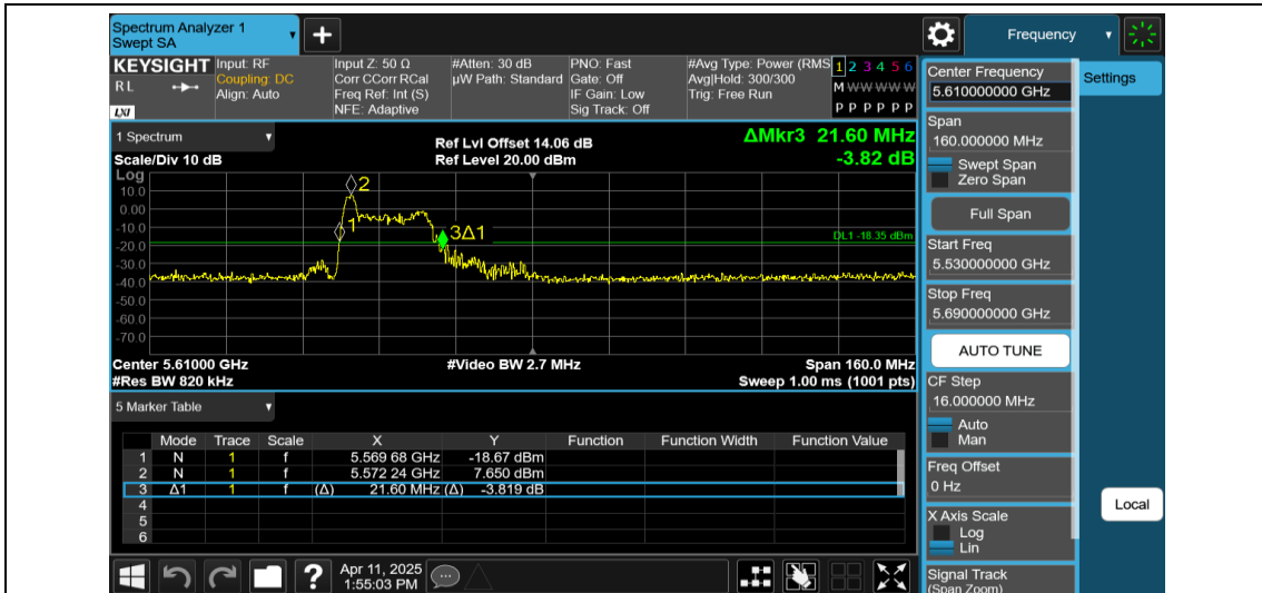
11AX80MIMO-Ant2-5610-26Tone-RU0
