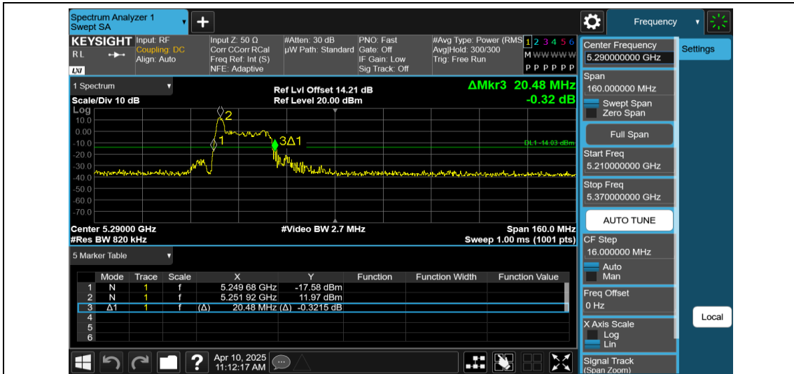
11AX80MIMO-Ant2-5290-26Tone-RU0
