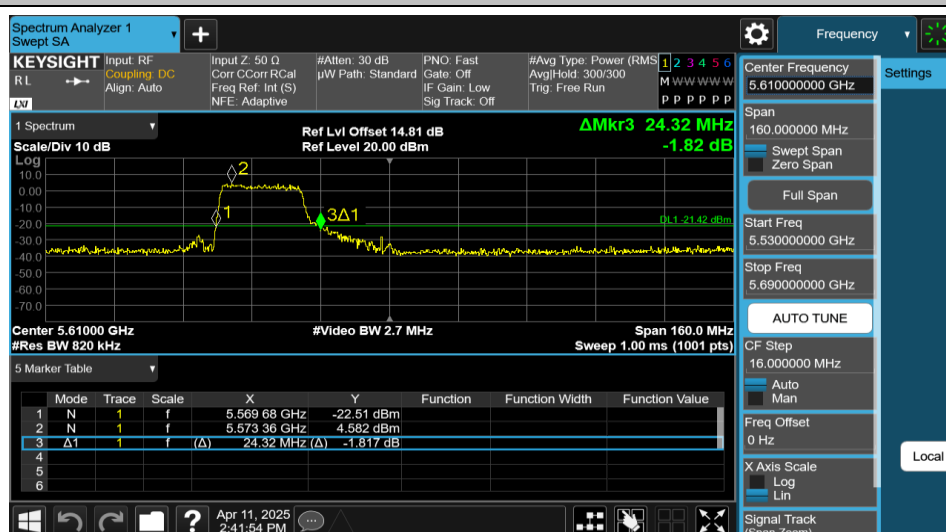
11AX80MIMO-Ant1-5610-242Tone-RU61
