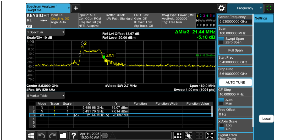
11AX80MIMO-Ant2-5530-26Tone-RU0
