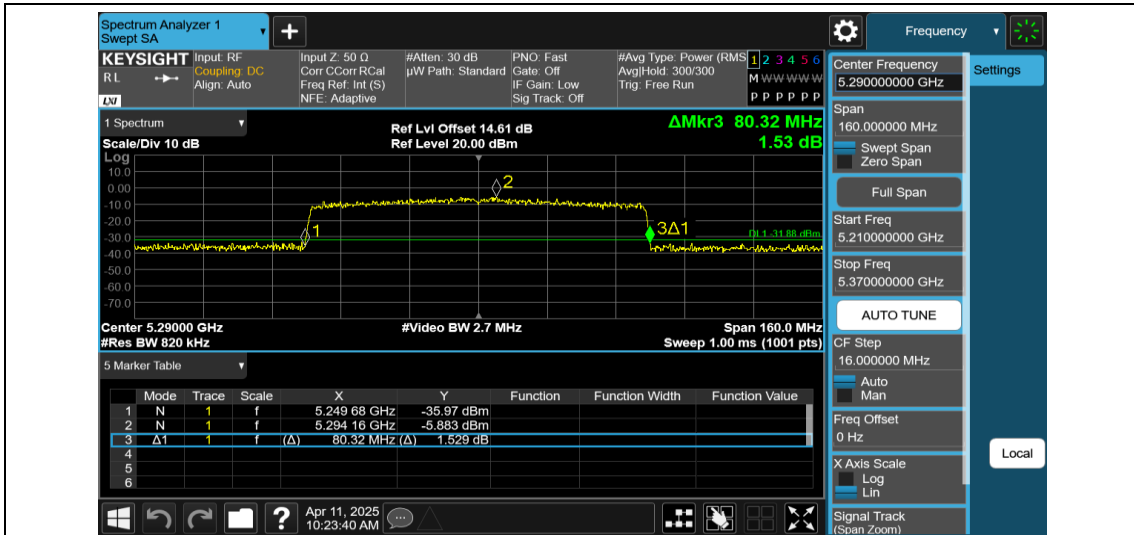
11AX80MIMO-Ant1-5290-996Tone-RU67
