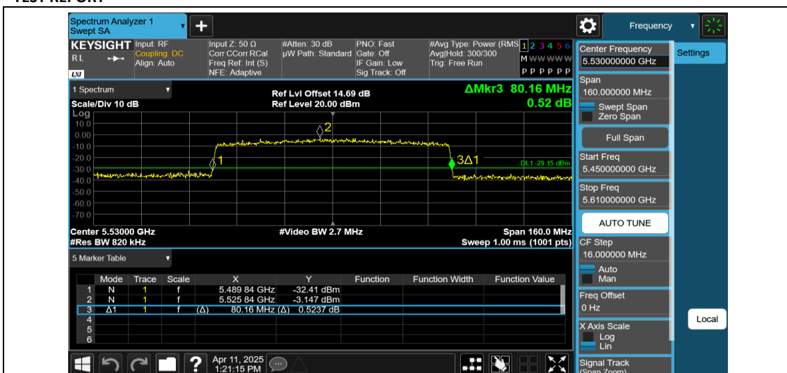
11AX80MIMO-Ant1-5530-996Tone-RU67
