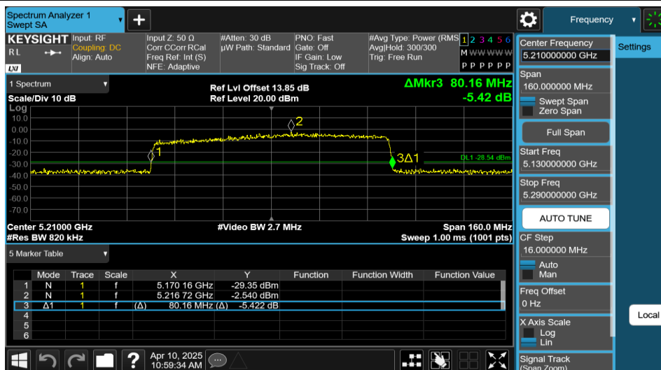
11AX80MIMO-Ant2-5210-996Tone-RU67
