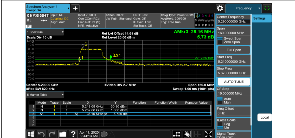
11AX80MIMO-Ant1-5290-242Tone-RU61
