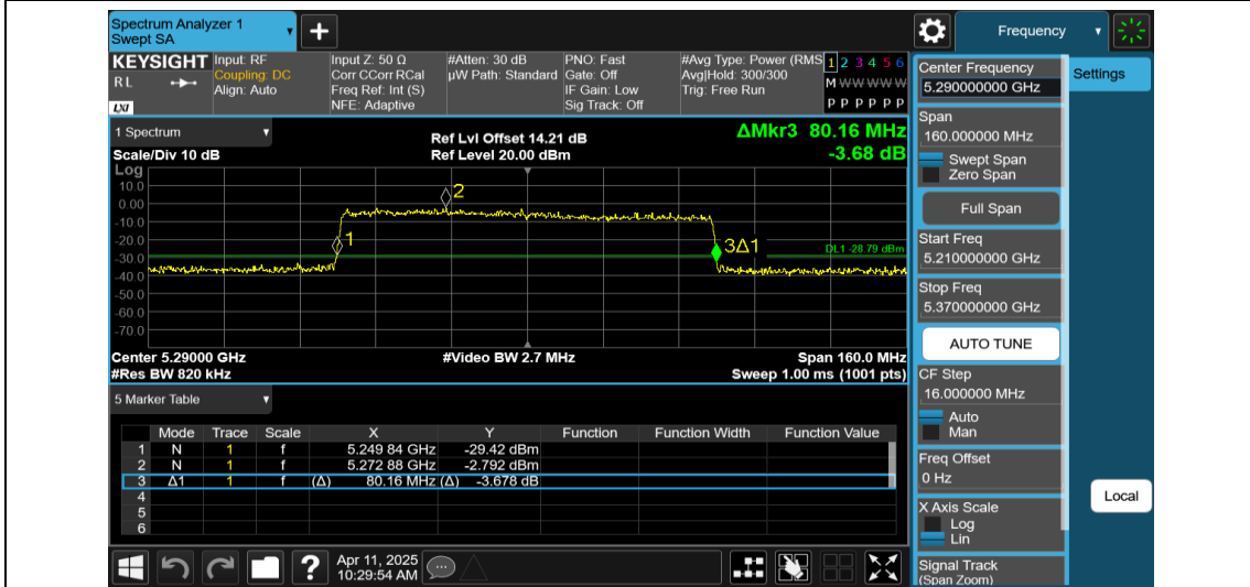
11AX80MIMO-Ant2-5290-996Tone-RU67
