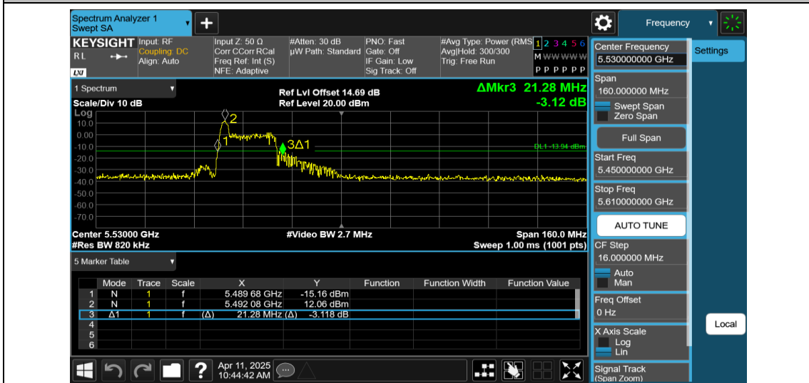
11AX80MIMO-Ant1-5530-26Tone-RU0
