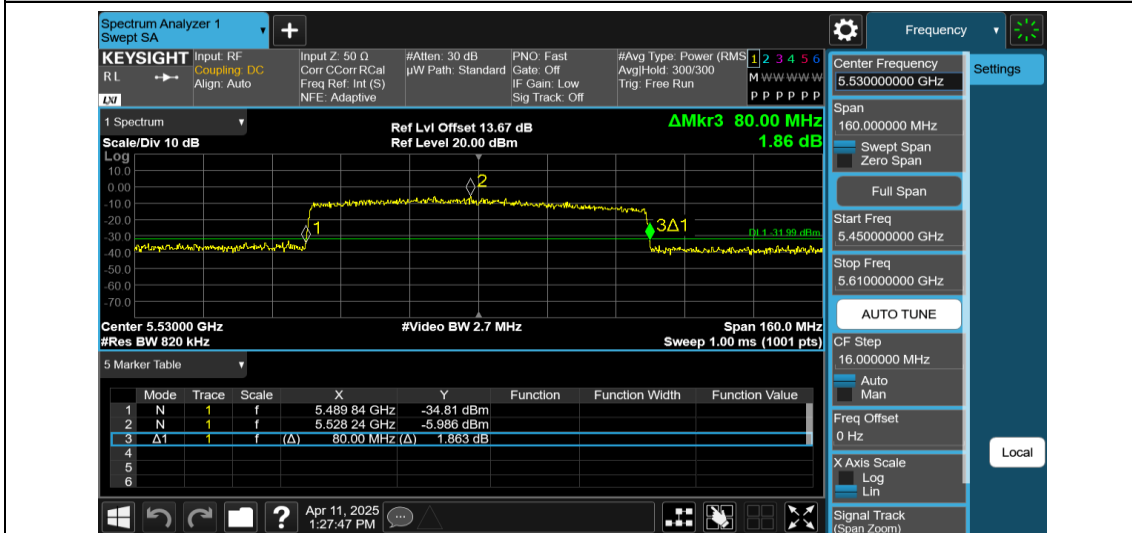
11AX80MIMO-Ant2-5530-996Tone-RU67
