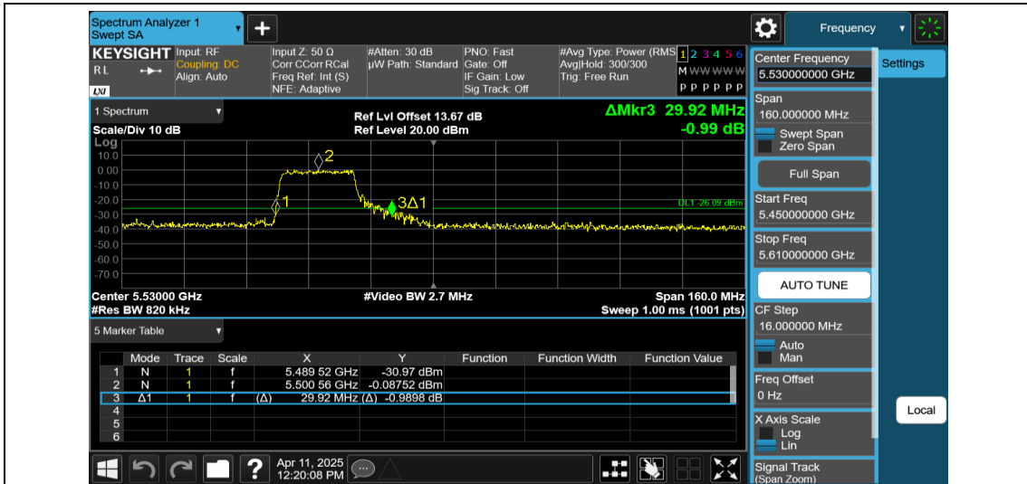
11AX80MIMO-Ant2-5530-242Tone-RU61
