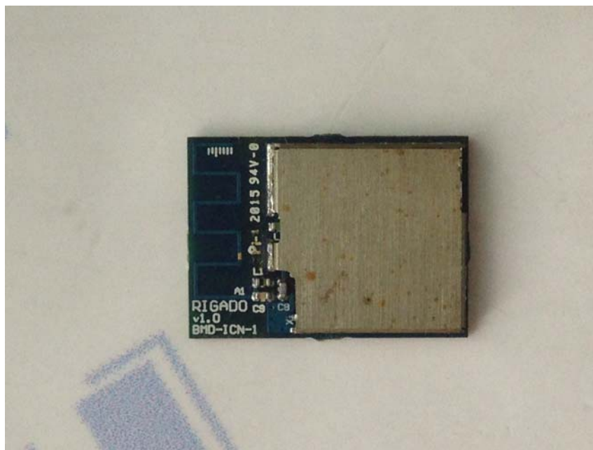
Module view side 1
