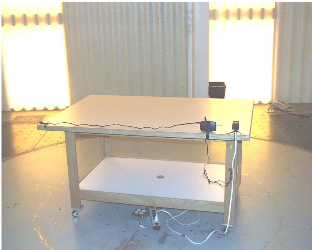
Rear View Radiated Emission Configuration (Horizontal Orientation)
