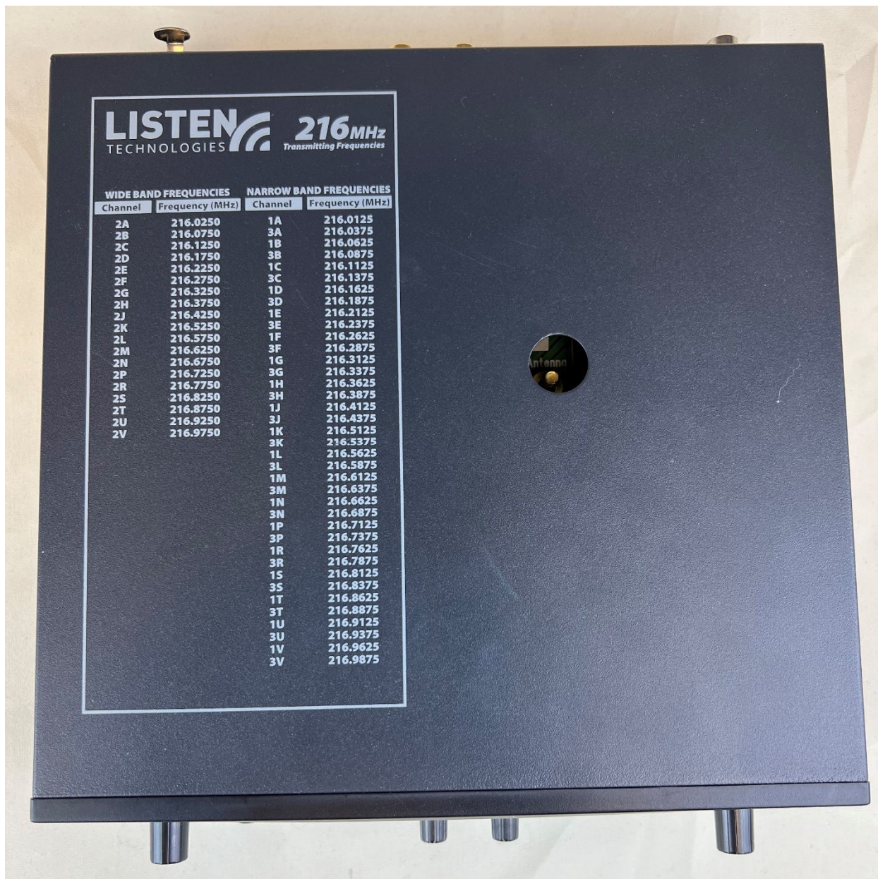
Figure 4 - External Top View
