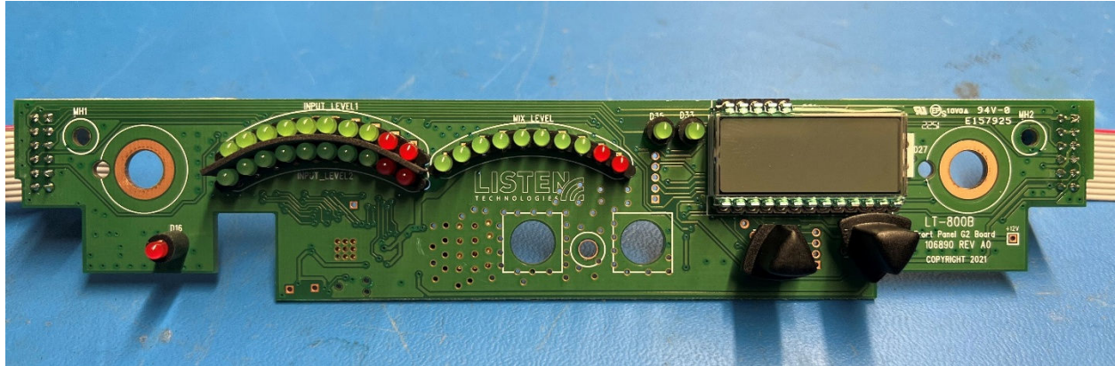
Figure 4 - Front Panel PCB - Top
