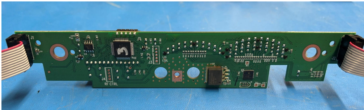
Figure 5 - Front Panel PCB - Rear
