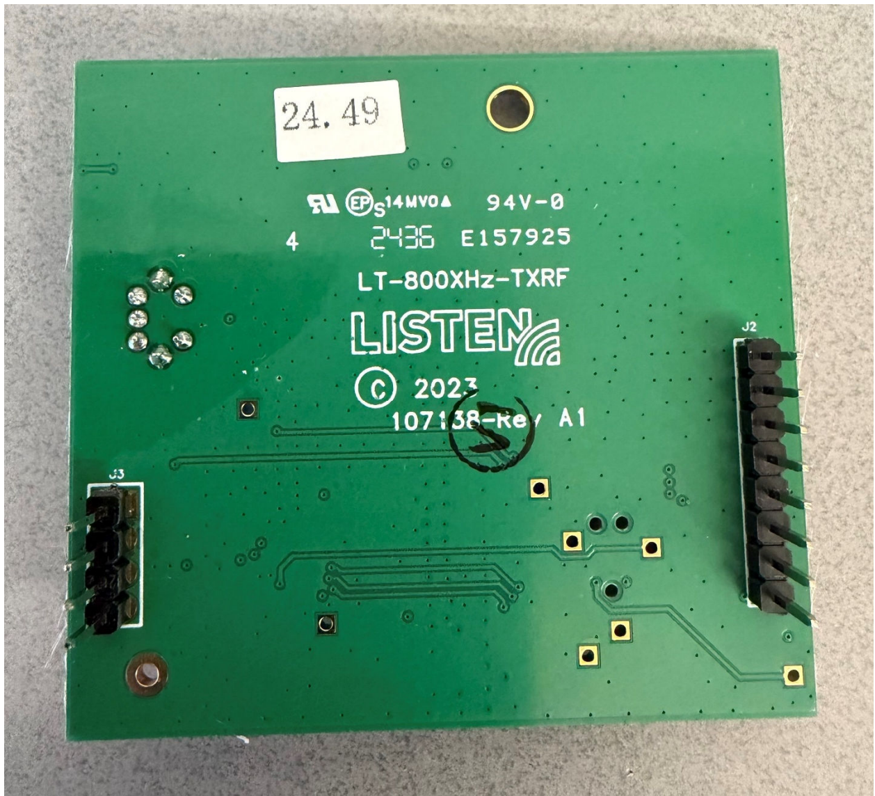
Figure 7 - RF Card - Bottom
