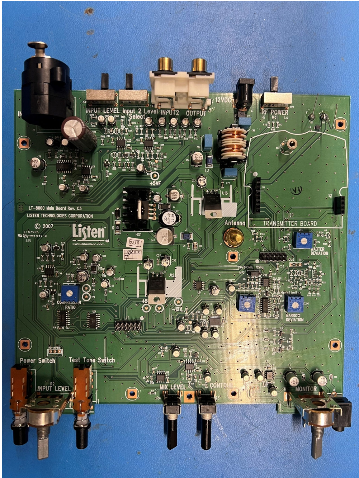
Figure 2 - Top of Main Board
