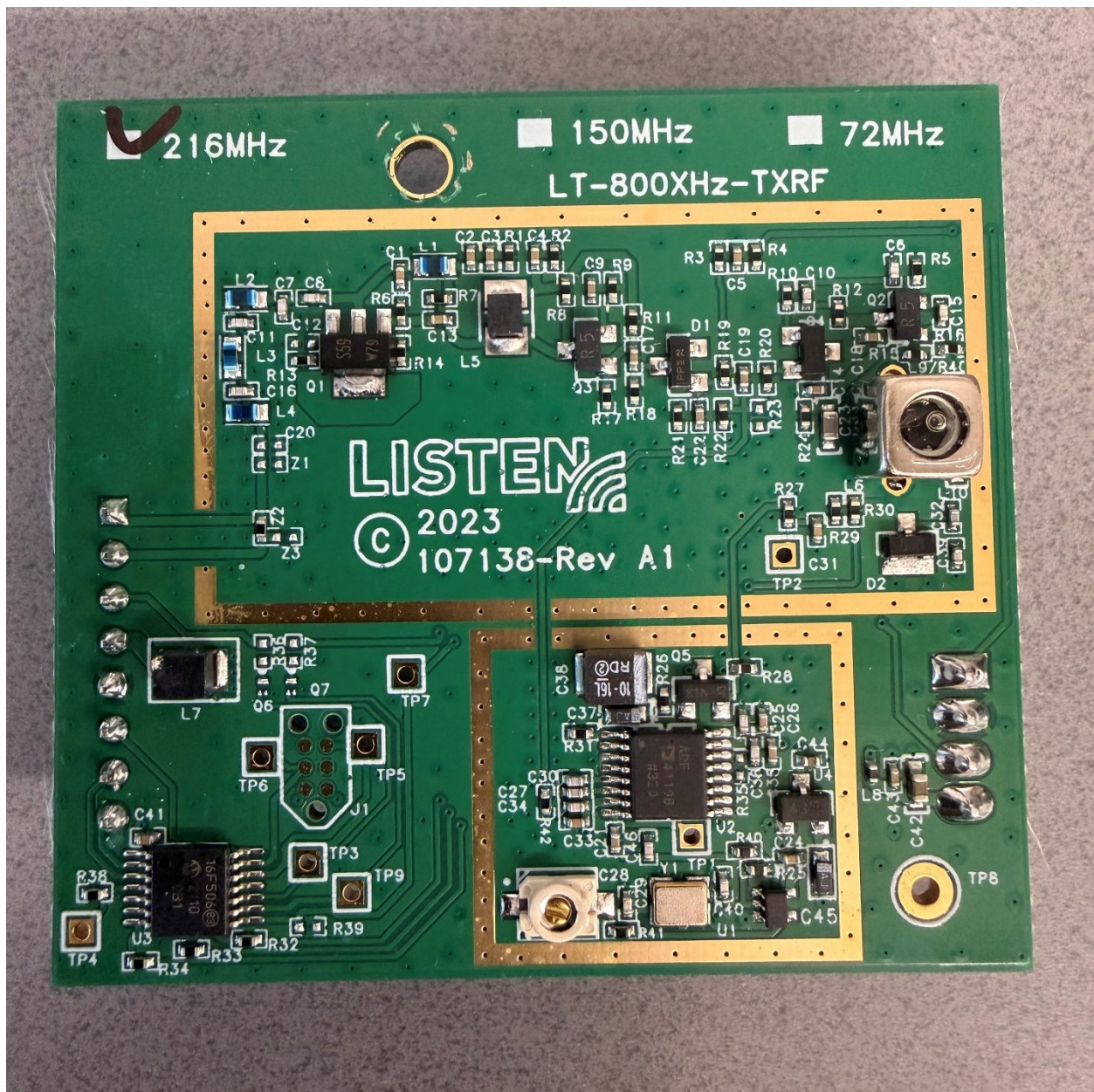
Figure 6 - RF Card - Top
