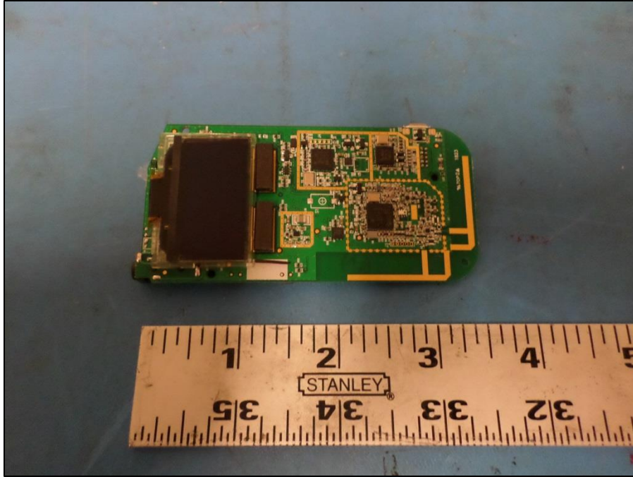
LKR-11 PCB Component Side
