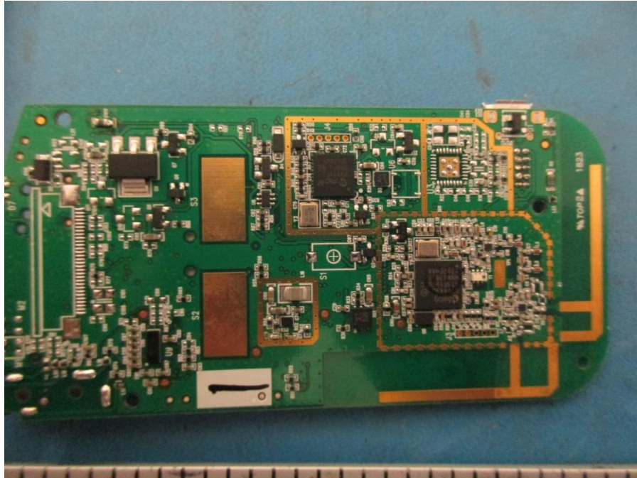
LKR-12 PCB Component Side
