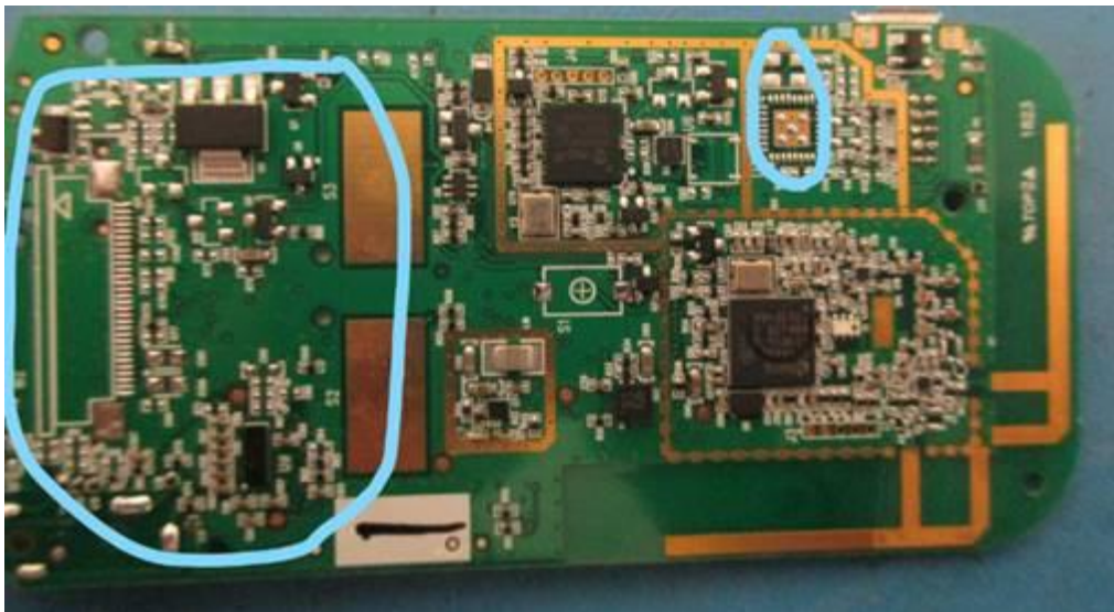
LKR-12 PCB Removed components circled
