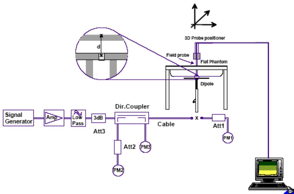
Figure 6: System performance check components
