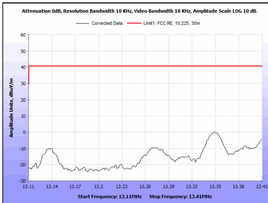
Plot 4. Spurious Emissions Within the Band 13.110 – 13.410 MHz
