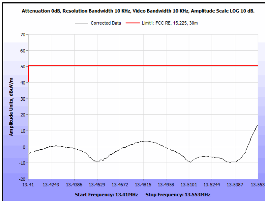
Plot 2. Spurious Emissions Within the Band 13.410 – 13.553 MHz
