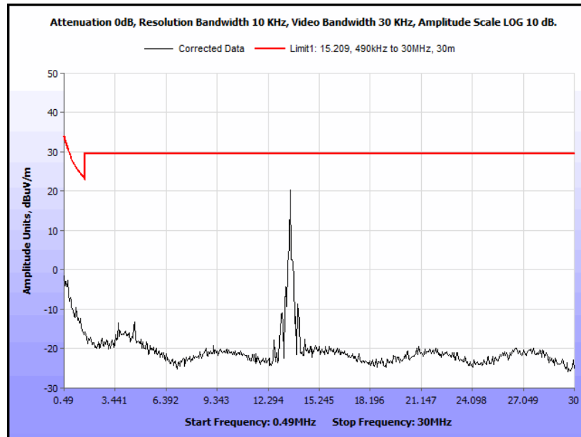
Plot 7. Spurious Emissions, Outside the Bands 13.110 - 14.010 MHz, 490KHz – 30MHz
