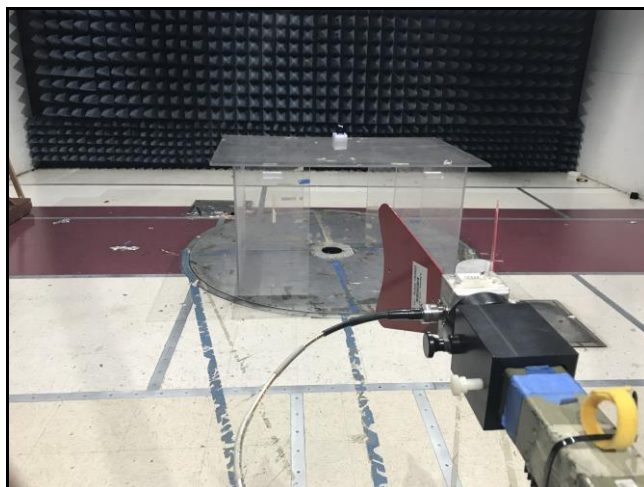
Photograph 4. Spurious Emissions, Outside the Bands, 1GHz - 18GHz Setup
