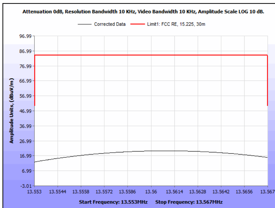
Plot 1. Spurious Emissions Within the Band 13.553 – 13.567 MHz
