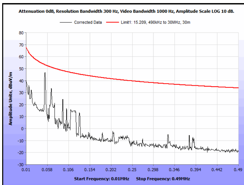
Plot 6. Spurious Emissions, Outside the Bands 13.110 - 14.010 MHz, 10KHz – 490KHz
