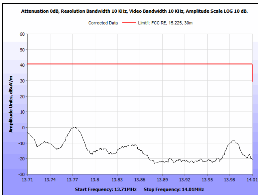
Plot 5. Spurious Emissions Within the Band 13.710 – 14.010 MHz
