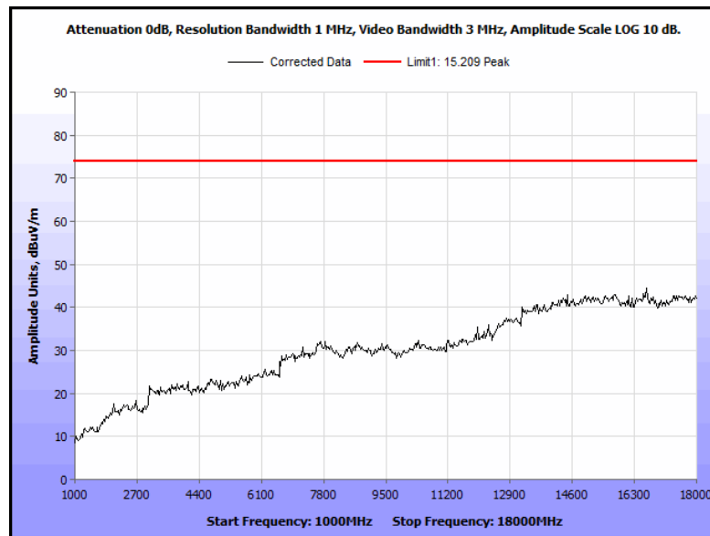
Plot 10. Spurious Emissions, Outside the Bands, 13.110 - 14.010 MHz, 1Ghz – 18GHz Peak
