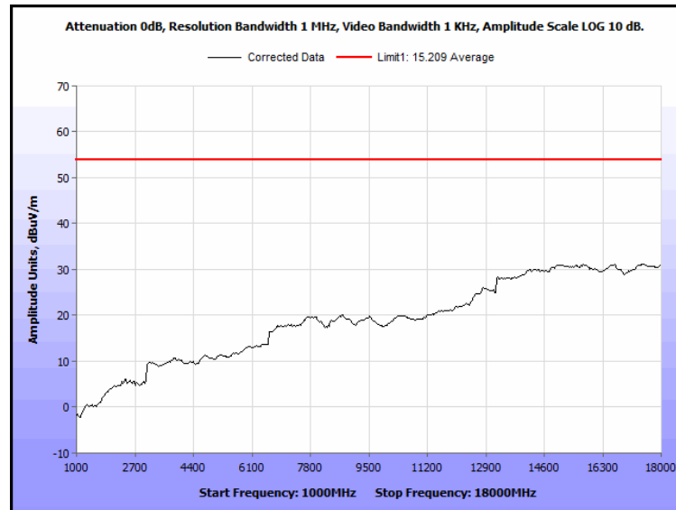
Plot 9 Spurious Emissions, Outside the Bands, 13.110 - 14.010 MHz, 1GHz – 18GHz AVG
