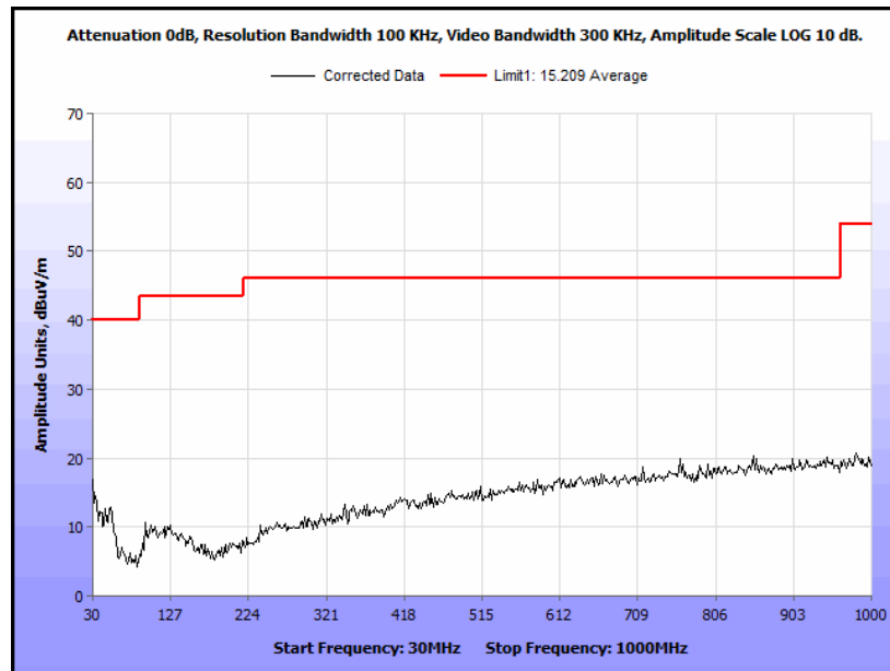
Plot 8. Spurious Emissions, Outside the Bands, 13.110 - 14.010 MHz, 30MHz - 1GHz
