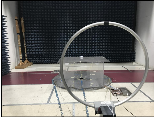
Photograph 2. Spurious Emissions, Outside the Bands, 10KHz - 30MHz Setup
