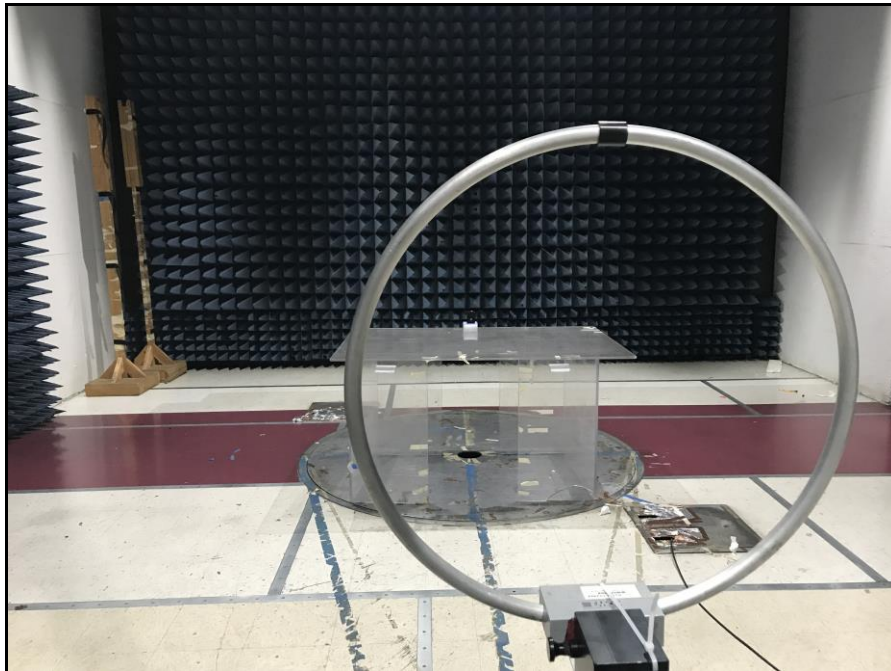
Photograph 1. Spurious Emissions Within the Band 13.553 – 13.567 MHz, 10KHz - 30MHz Setup
