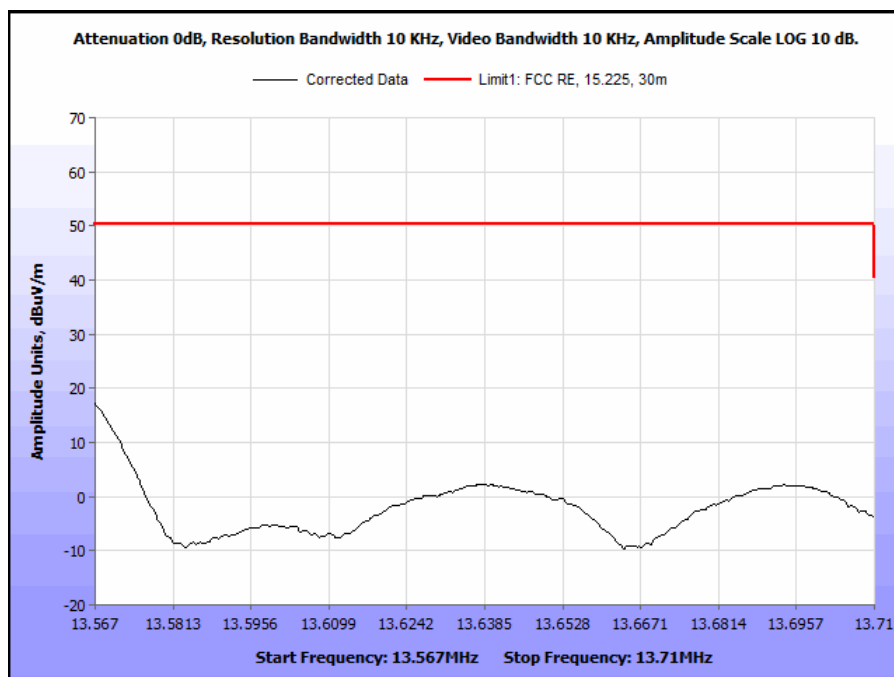
Plot 3. Spurious Emissions Within the Band 13.567 – 13.710 MHz
