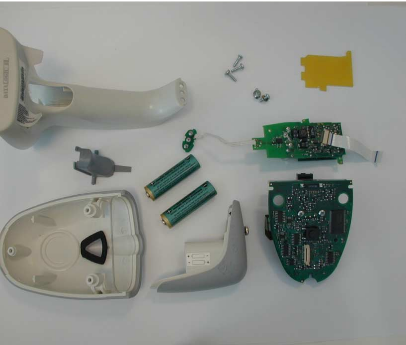
Gryphon m200 internal view
