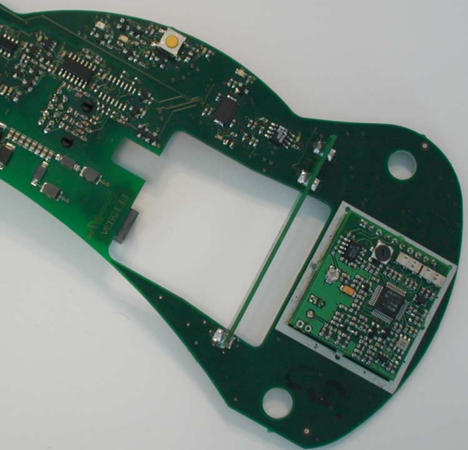
ELECTRONIC BOARD SIDE 2
