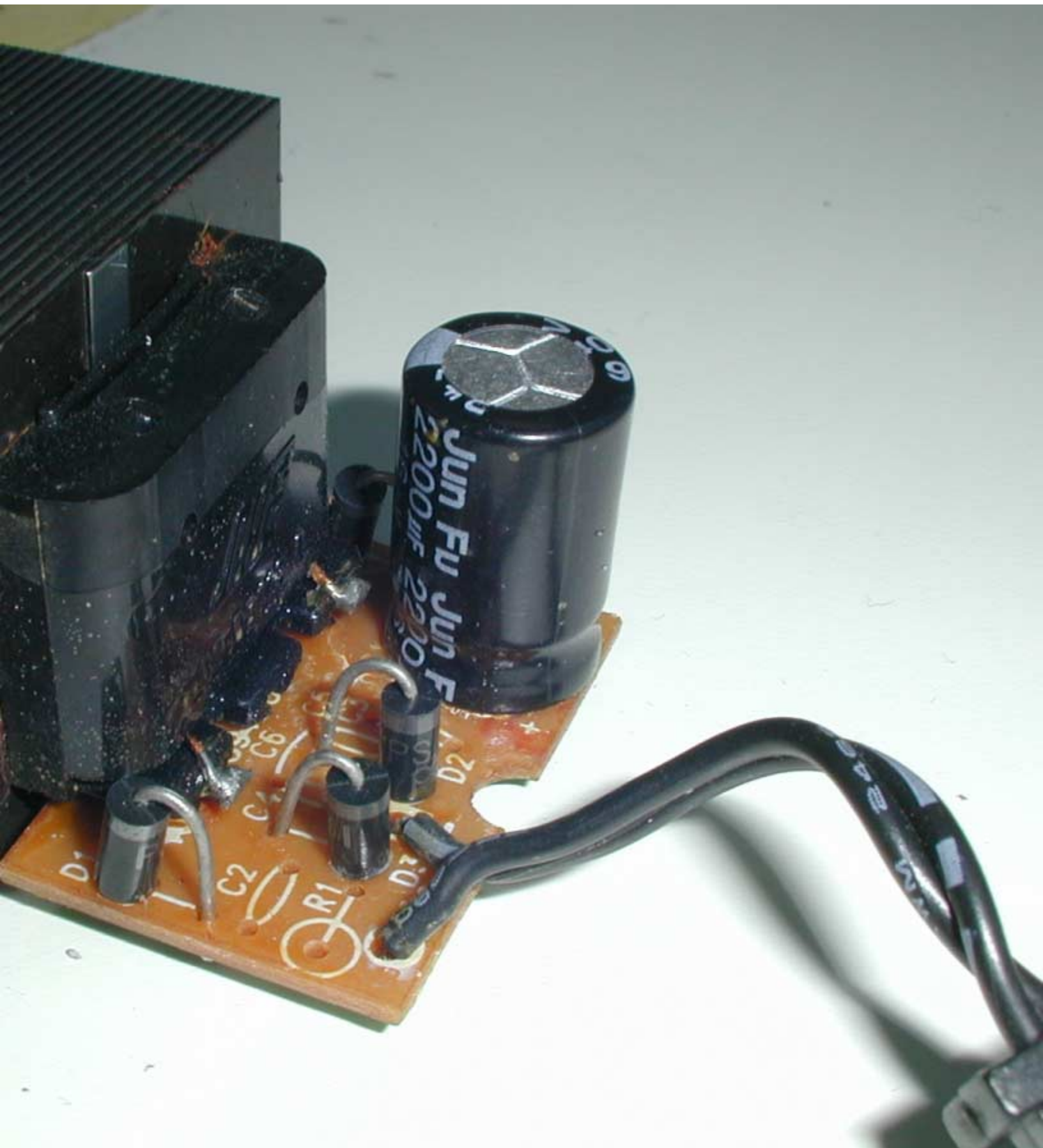
GENERAL VIEW – POWER SUPPLY
