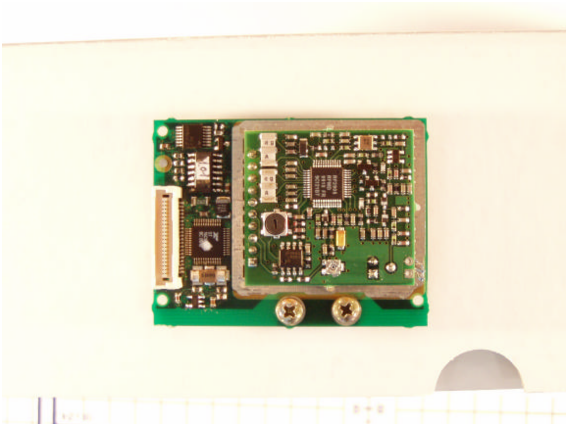
GEL2372 BOARD PLUS TRANSCEIVER
