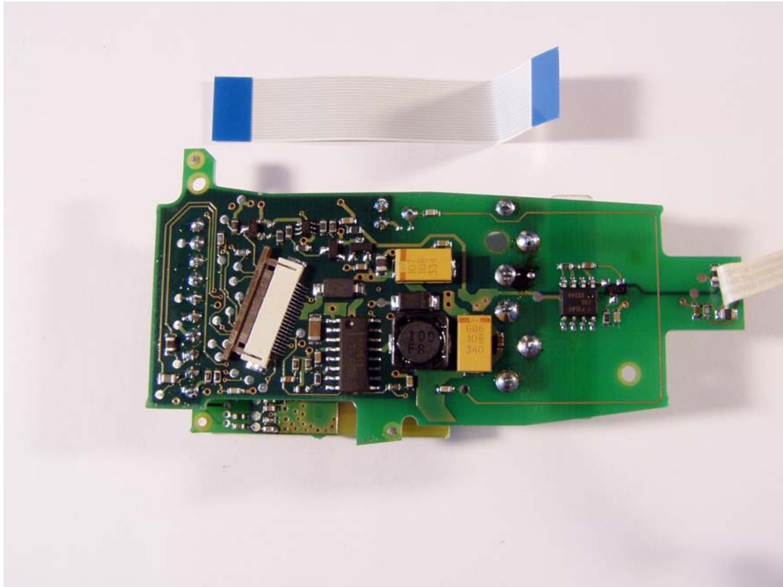
Fig. 12.7 Handle board – foil side
