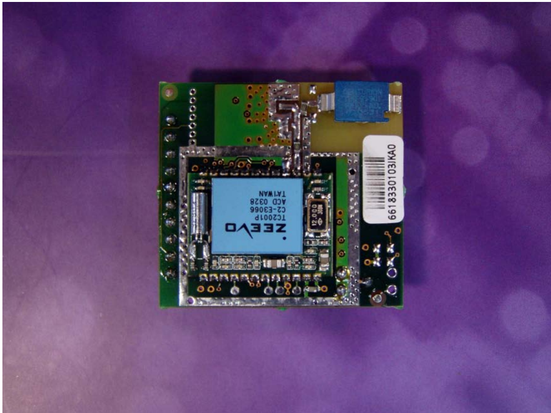
Fig. 12.8 Tranceiver module – upper side
