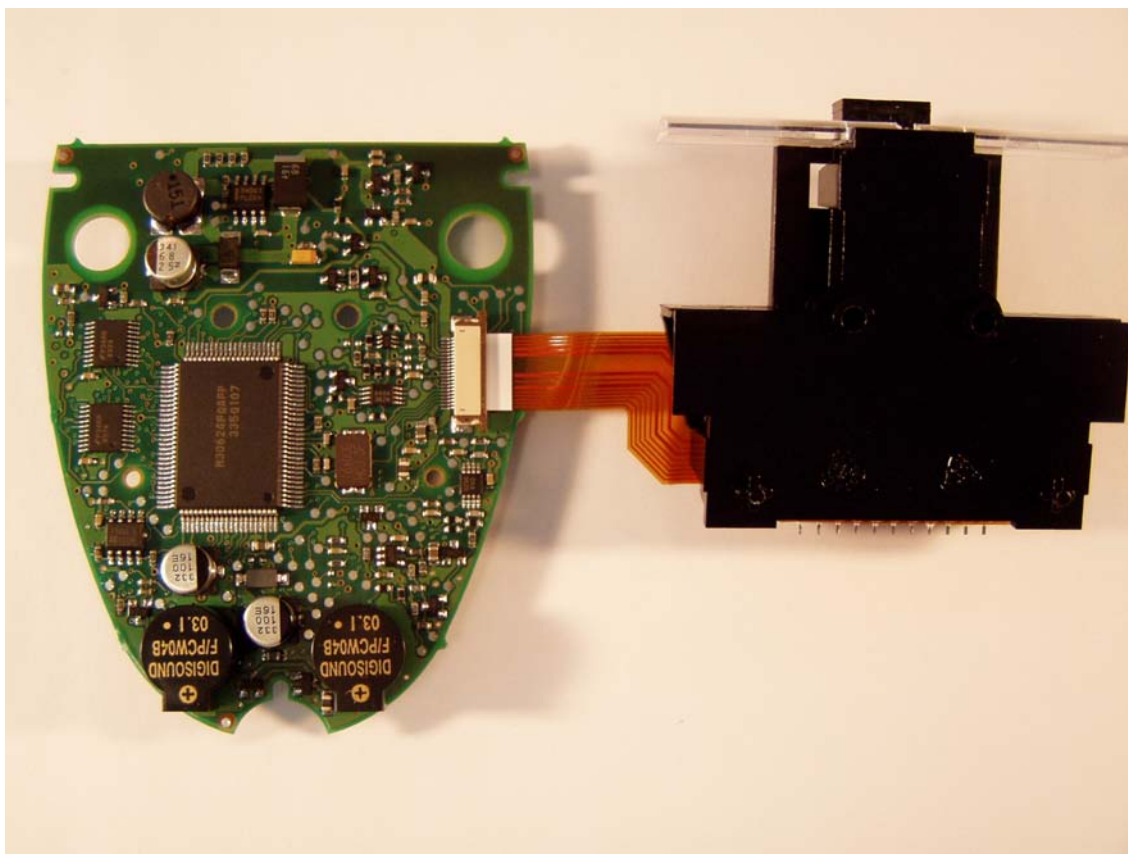
Fig. 12.3 Mother board – side 1
