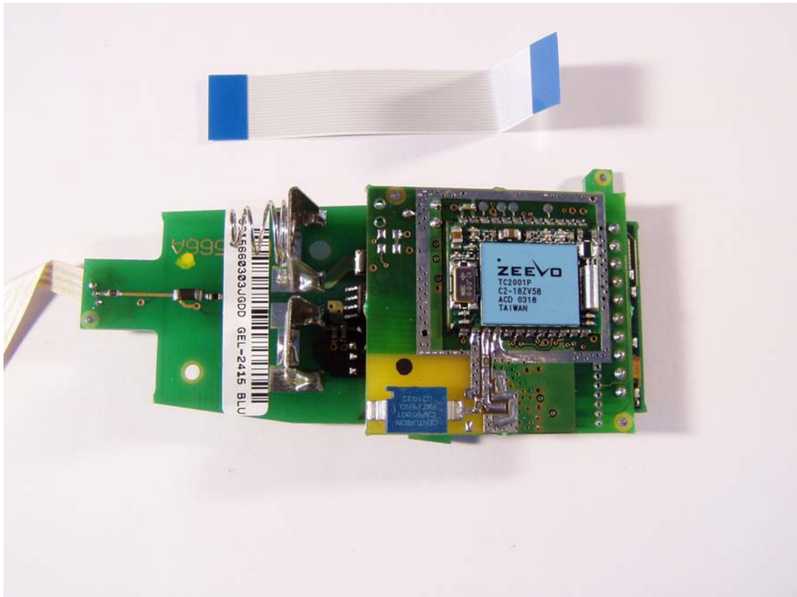
Fig. 12.5 Handle board – components side (with transceiver mounted)
