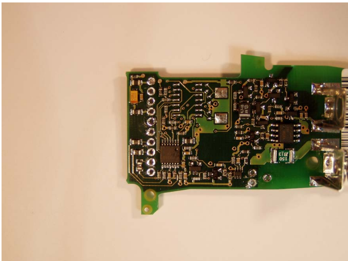
Fig. 12.6 Handle board – components side (without transceiver)
