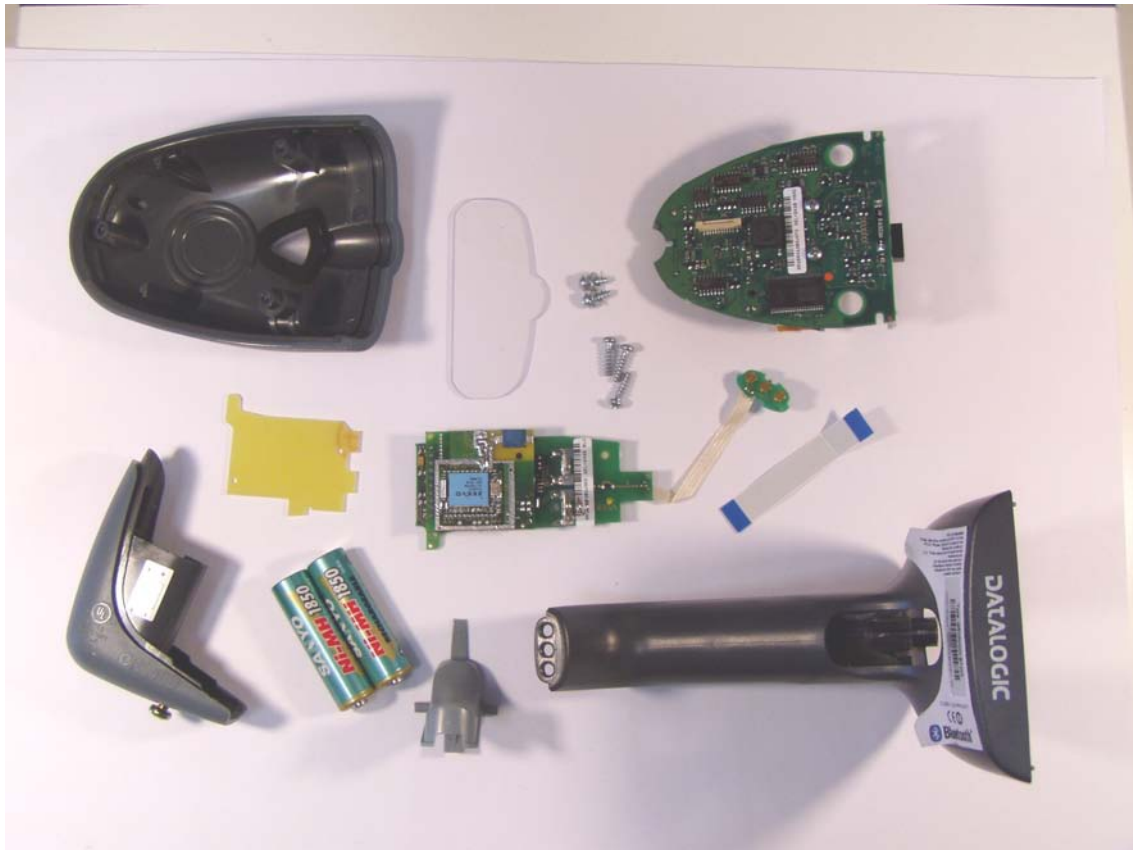
Fig. 12.2 Mother board + CCD
