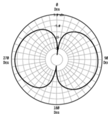
Free Space Elevation Pattern PHI=0
