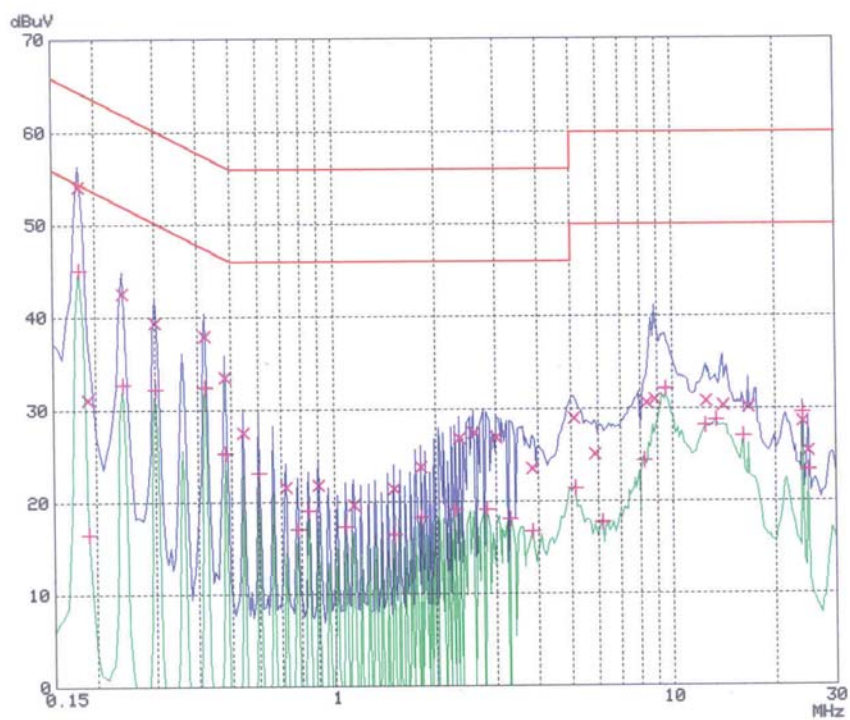
< Neutral line >
