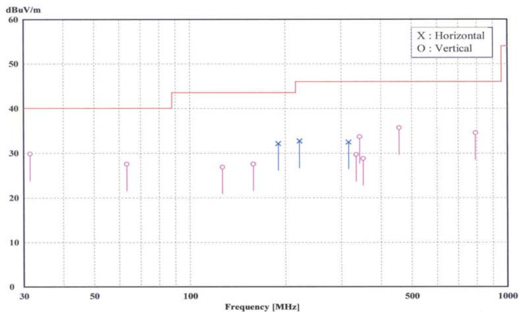
< Fig 6-1. Radiated emission result >
