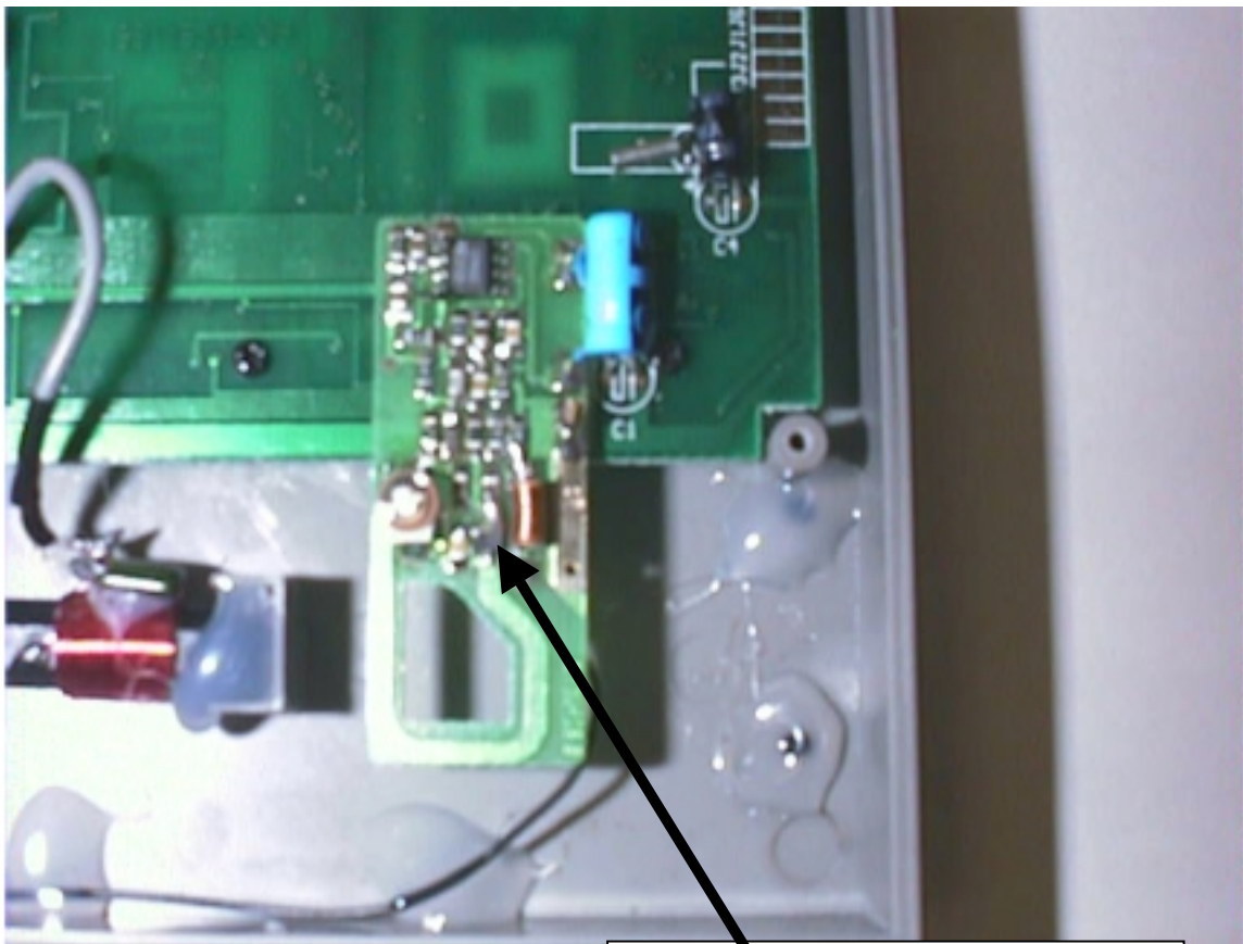
HFS 301-WS Receiver PC Board Sub Assembly
