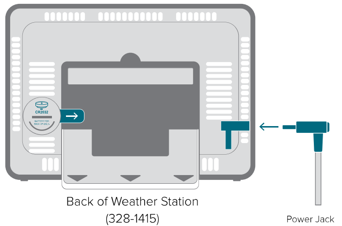
Power Jack
