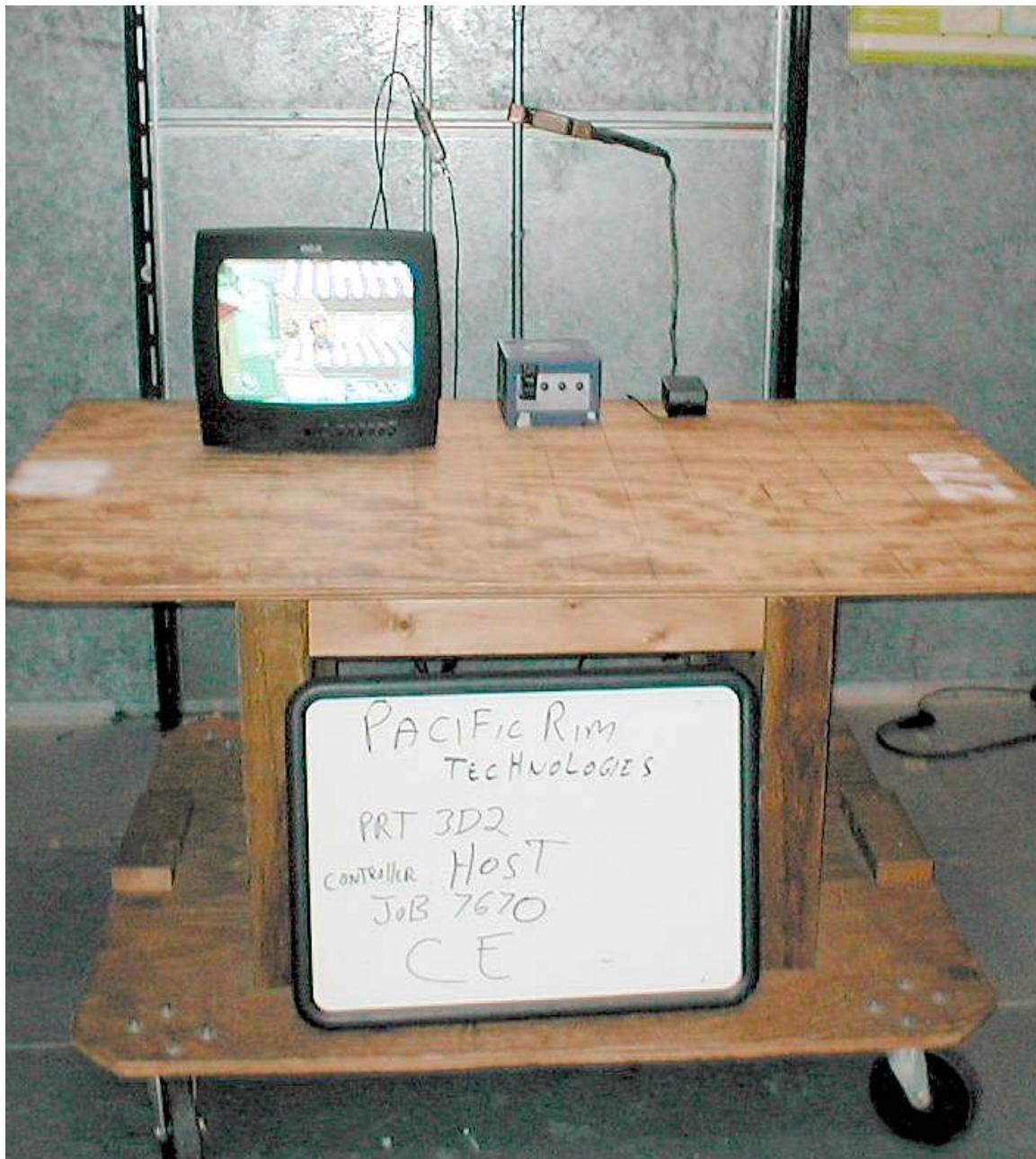
Conducted Spurious Emissions Test Setup, Front
