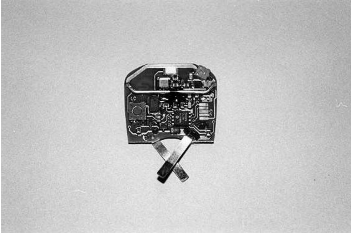
Fig. 2 Controller Board - Components side
