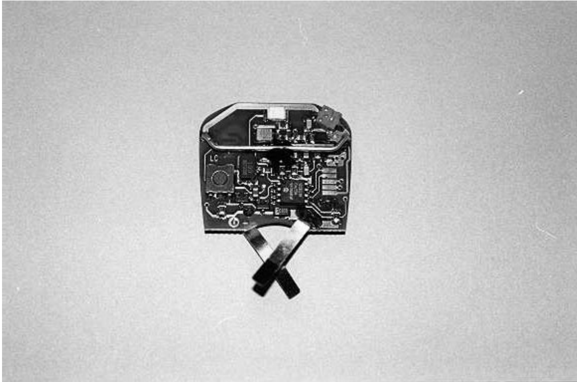
Fig. 1 Controller Board - Components side
